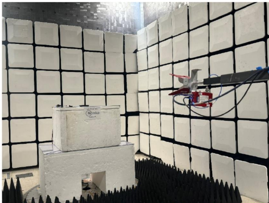
Figure 9.1-2: Radiated emissions setup (1 – 5 GHz): Front view photo.
