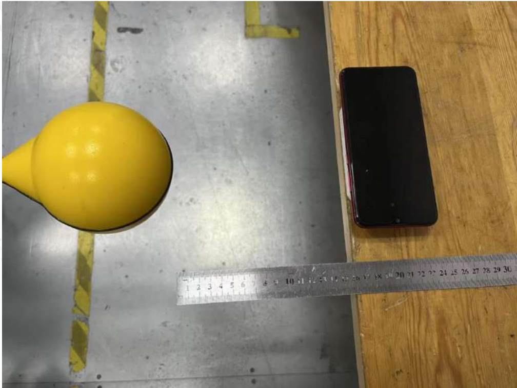
Test Position D(16cm) - Exposure photo from side edge surface-Front(TM1)
