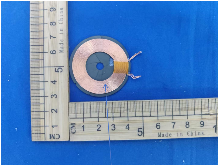
ANT_Earphone
