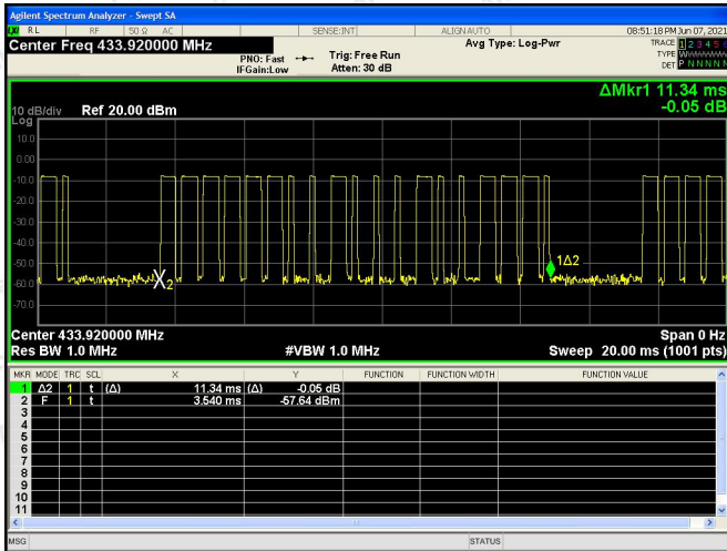
T on(ms)
