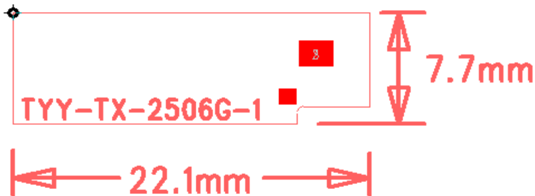
Chart 1 TYY-TX2506G-1 Product size
