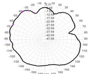
5790.0MHz Total(E1), Max= 0.62dBi
