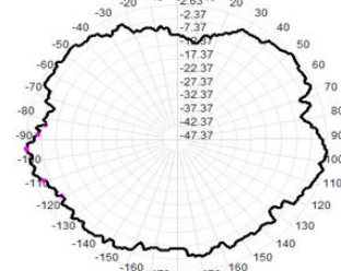
5790.0MHz Total(E2), Max= 2.63dBi
