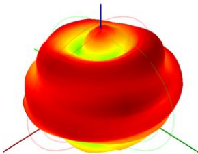
5790.0MHz H+V, Eff: 66.3%
