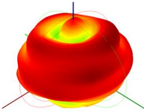
2470.0MHz H+V, Eff: 70.4%
