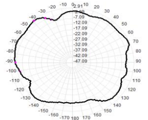
2470.0MHz Total(E2), Max= 2.29dBi
