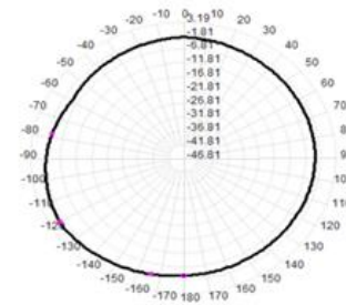
2400.0MHz Total(H), Max= -1.62dBi
