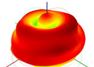
2470.0MHz H+V, Eff. 70.4%
