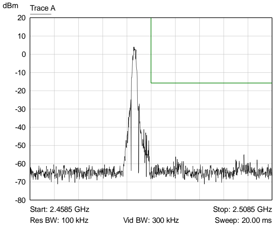
Graph 8: Upper Band Edge Plot
