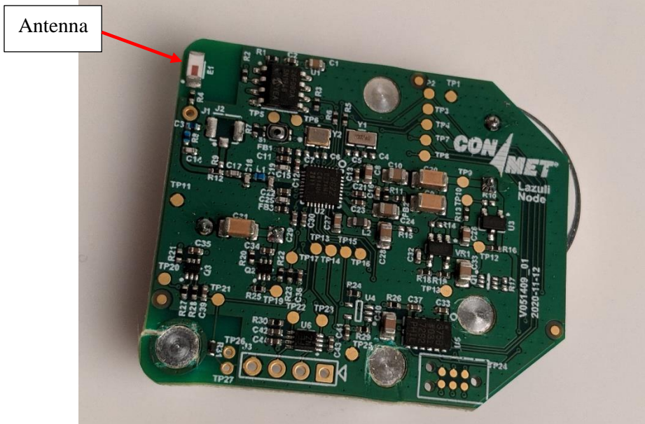
Photograph 11: Top side of the PCB
