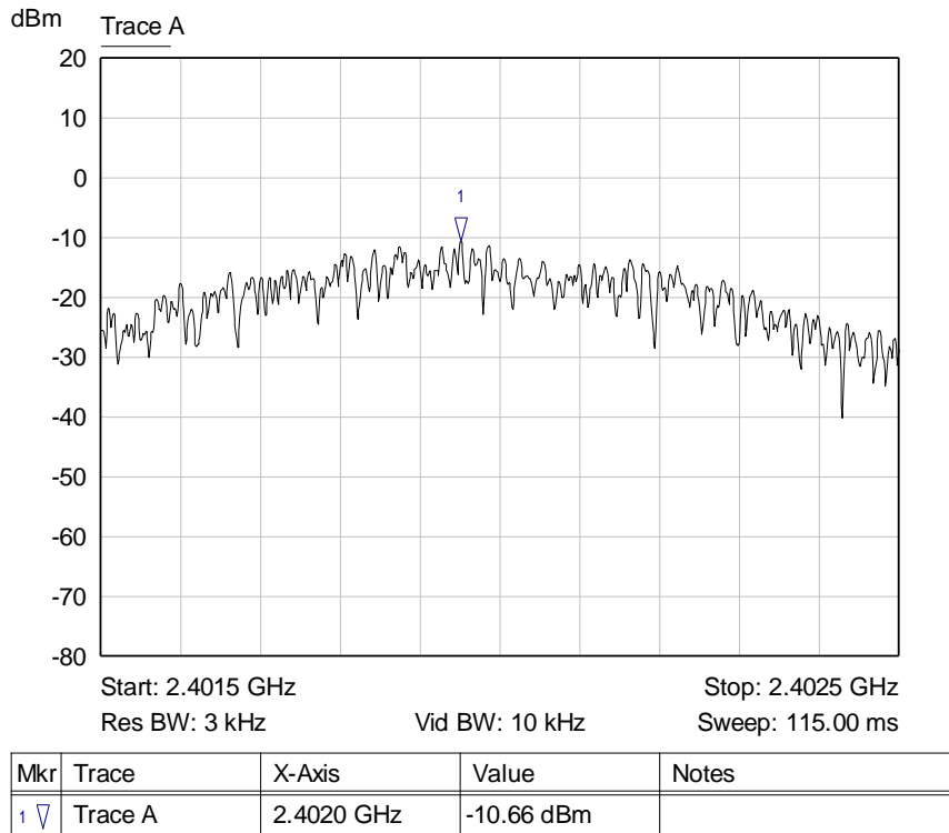
Graph 11: Lowest Channel 3 kHz PSD Plot
