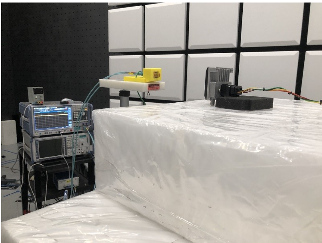
Radiated Emissions Test Setup (220 GHz to 243GHz)
