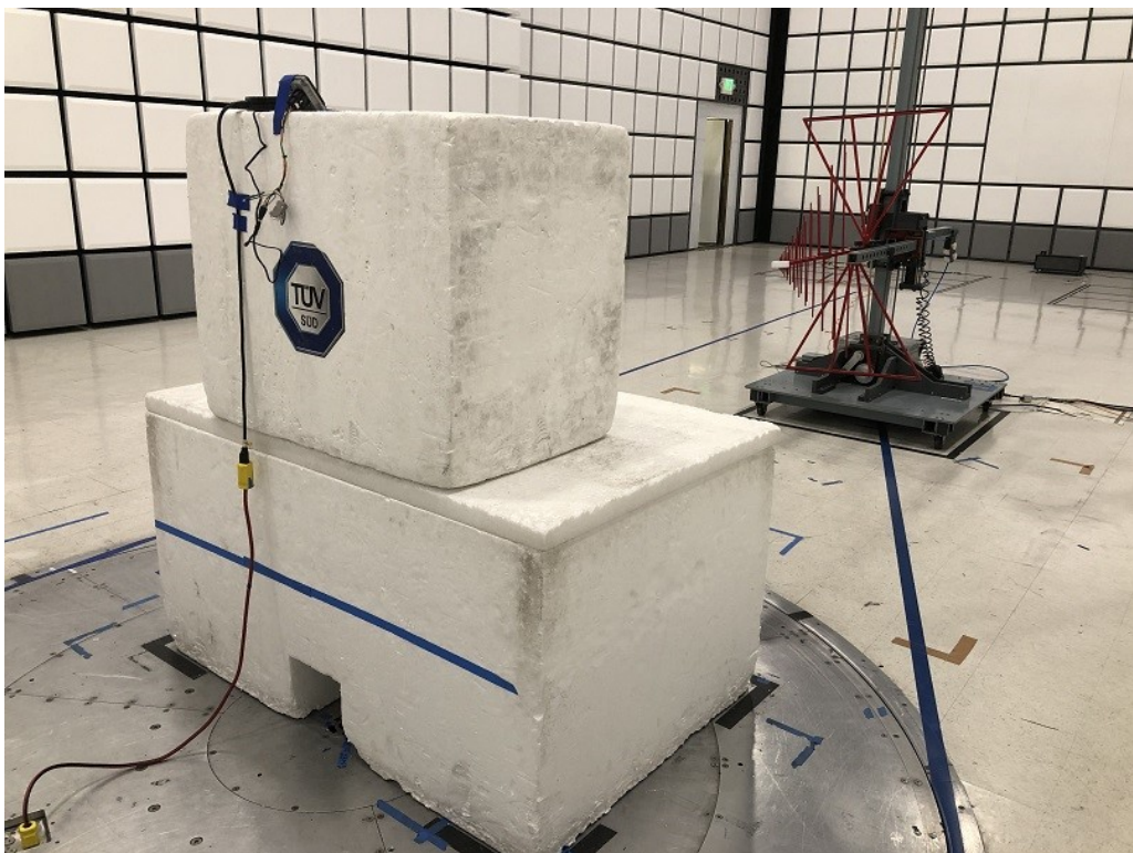
Radiated Emissions Test Setup (30 MHz to 1 GHz)
