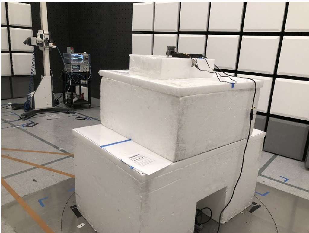
Radiated Emissions Test Setup (18 GHz to 81GHz)
