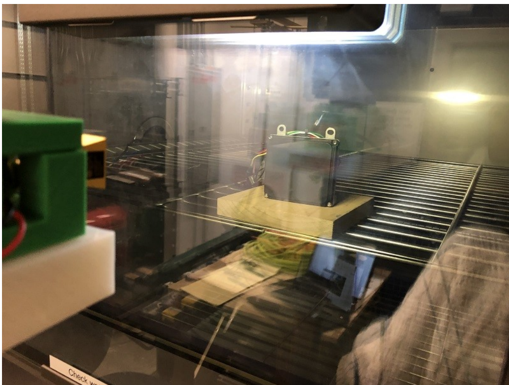
Extreme Condition Test Setup (220 GHz to 243GHz)
