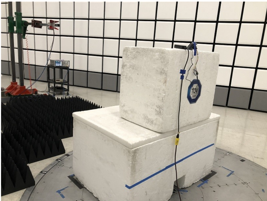
Radiated Emissions Test Setup (1 GHz to 18 GHz)
