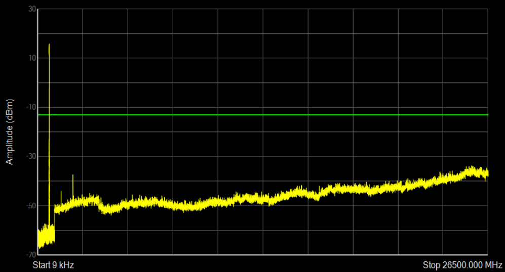
Band71 QAM16 BW=5MHz Channel=133447 RB Size=25 Position=#0
