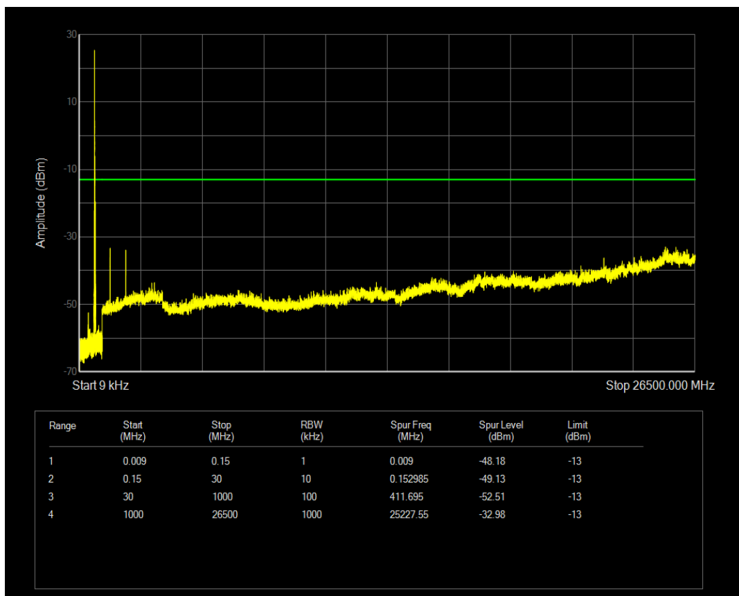
Band71 QAM16 BW=20MHz Channel=133297 RB Size=100 Position=#0
