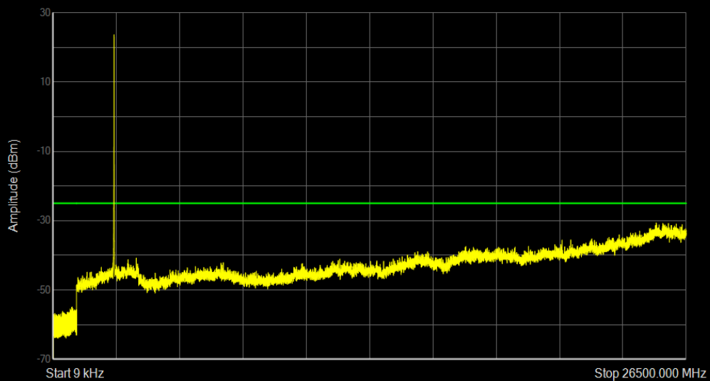
Band7 QPSK BW=5MHz Channel=21425 RB Size=25 Position=#0
