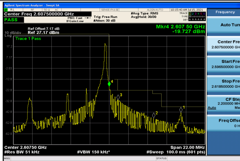
Band41-5MHz-QPSK-40740-1RB#24
