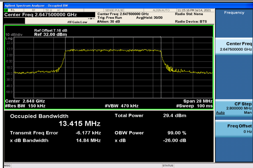
Band41-15MHz-16QAM-41165-75RB#0-13.415
