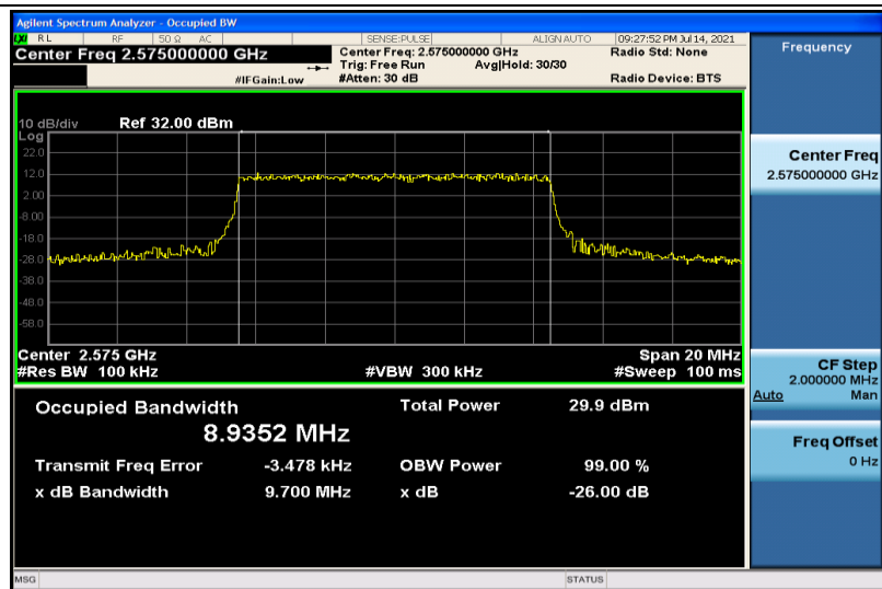
Band38-10MHz-16QAM-37800-50RB#0-8.9352
