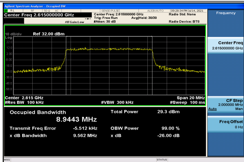
Band38-10MHz-16QAM-38200-50RB#0-8.9443
