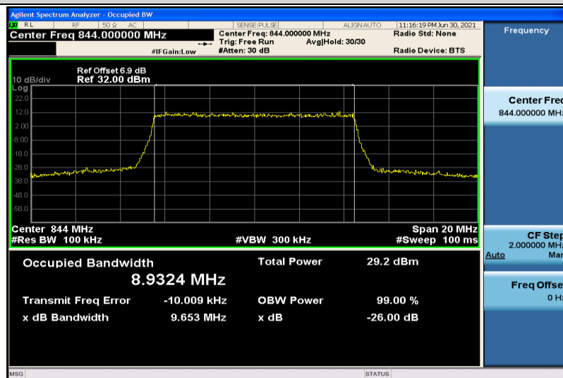
Band5-10MHz-16QAM-20600-50RB#0-8.9324
