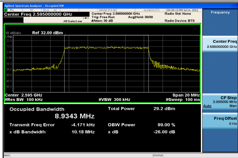
Band38-10MHz-16QAM-38000-50RB#0-8.9343
