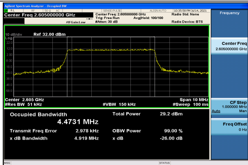
Band41-5MHz-16QAM-40740-25RB#0-4.4731
