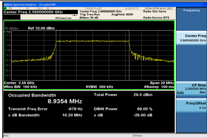
Band41-10MHz-16QAM-40290-50RB#0-8.9354
