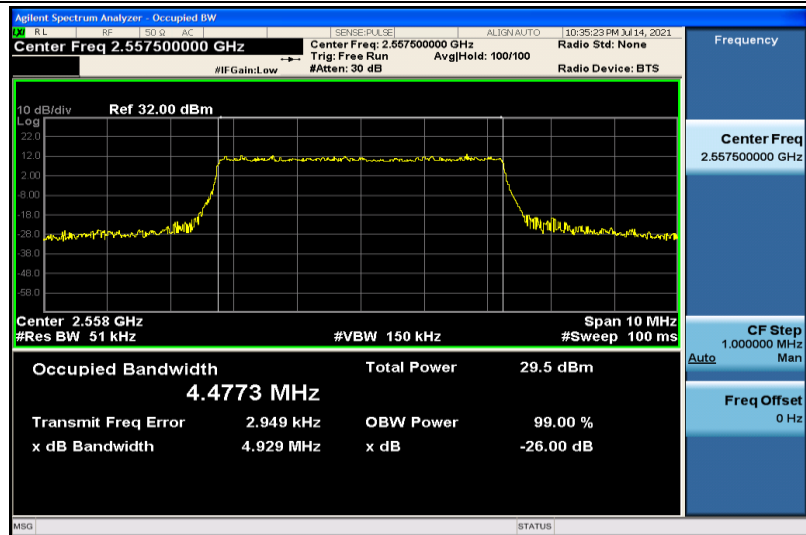
Band41-5MHz-16QAM-40265-25RB#0-4.4773
