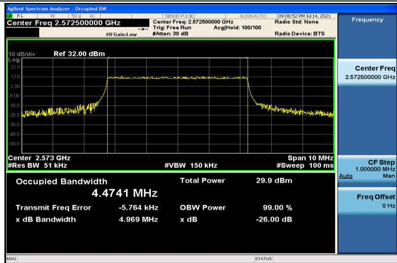
Band38-5MHz-16QAM-37775-25RB#0-4.4741
