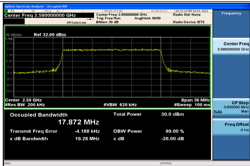
Band38-20MHz-16QAM-37850-100RB#0-17.872
