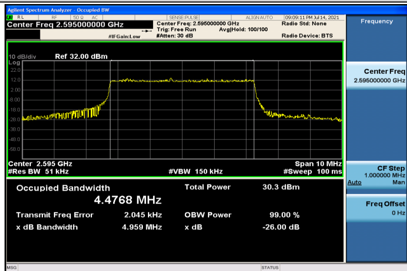
Band38-5MHz-QPSK-38000-25RB#0-4.4768
