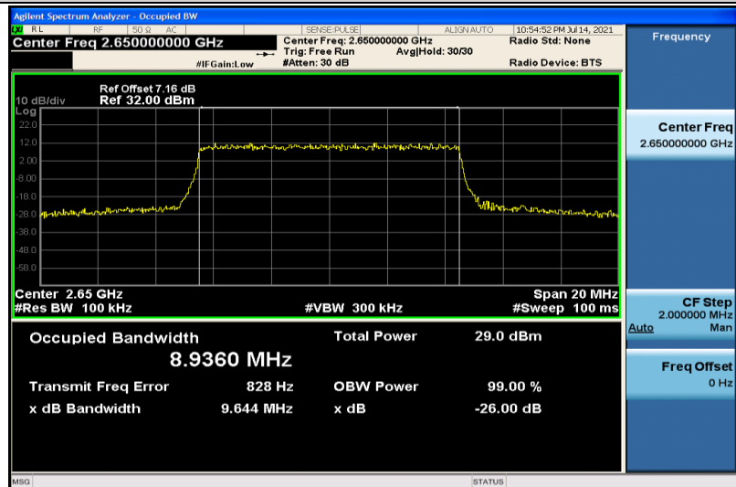
Band41-10MHz-16QAM-41190-50RB#0-8.9360
