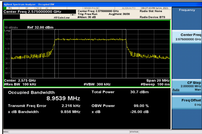
Band38-10MHz-QPSK-37800-50RB#0-8.9539
