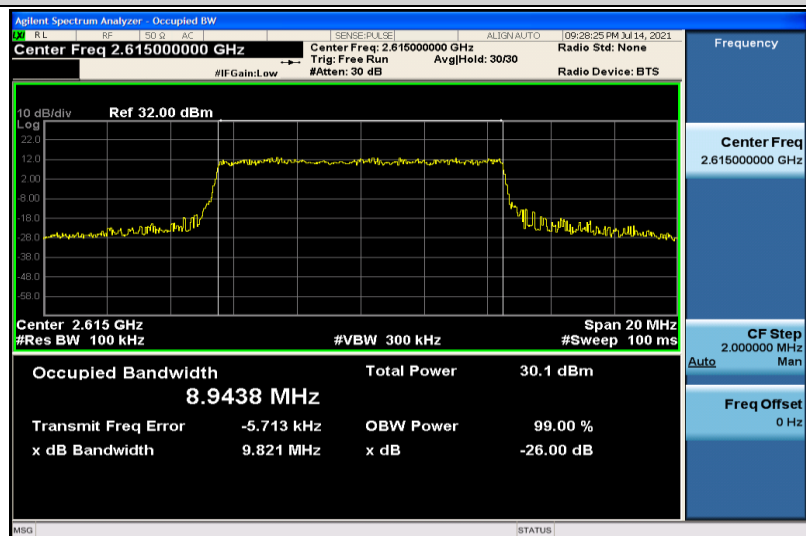
Band38-10MHz-QPSK-38200-50RB#0-8.9438
