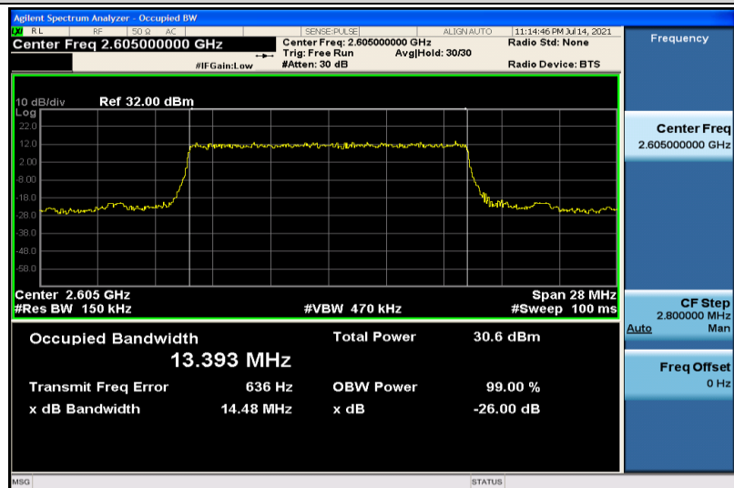
Band41-15MHz-QPSK-40740-75RB#0-13.393
