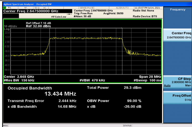
Band41-15MHz-QPSK-41165-75RB#0-13.434
