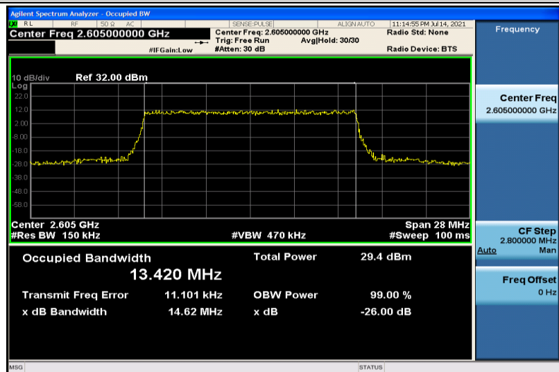
Band41-15MHz-16QAM-40740-75RB#0-13.420
