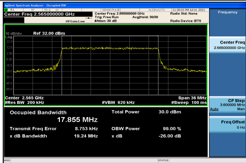
Band41-20MHz-16QAM-40340-100RB#0-17.855
