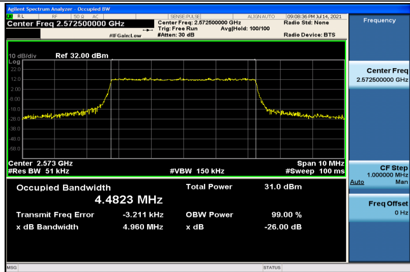
Band38-5MHz-QPSK-37775-25RB#0-4.4823
