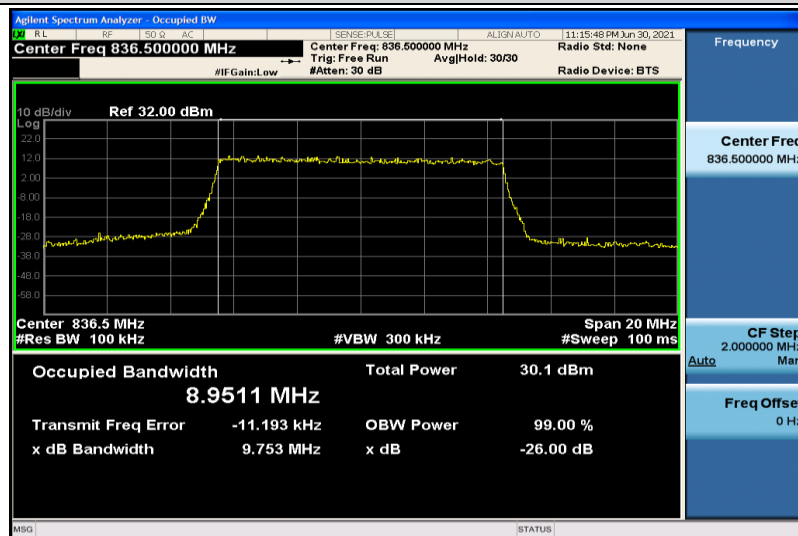
Band5-10MHz-QPSK-20525-50RB#0-8.9511
