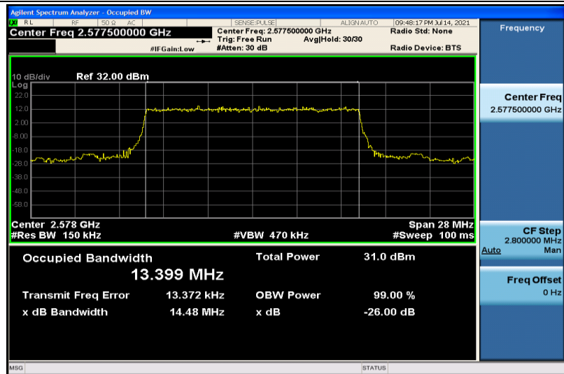
Band38-15MHz-QPSK-37825-75RB#0-13.399
