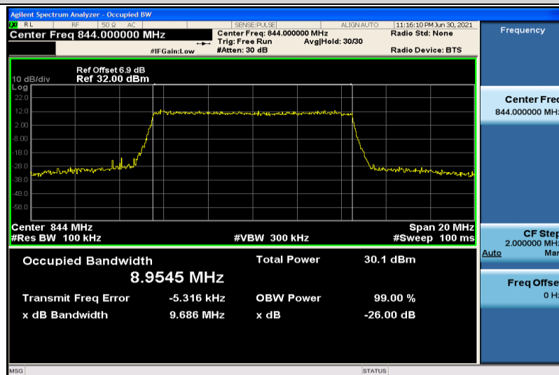
Band5-10MHz-QPSK-20600-50RB#0-8.9545
