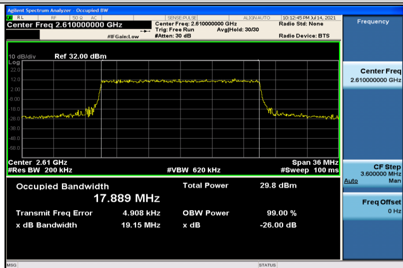
Band38-20MHz-QPSK-38150-100RB#0-17.889
