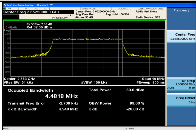
Band41-5MHz-QPSK-41215-25RB#0-4.4818
