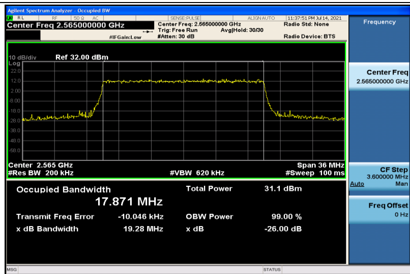
Band41-20MHz-QPSK-40340-100RB#0-17.871
