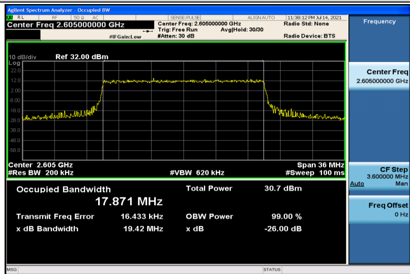
Band41-20MHz-QPSK-40740-100RB#0-17.871
