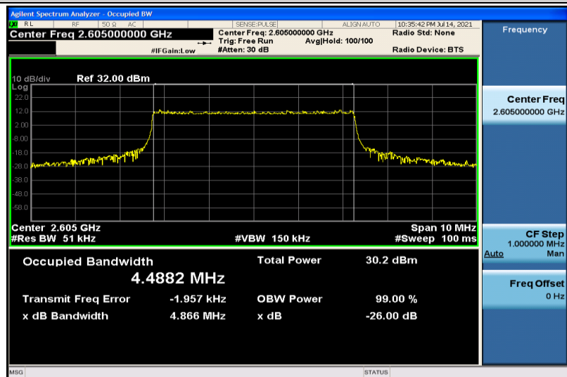
Band41-5MHz-QPSK-40740-25RB#0-4.4882
