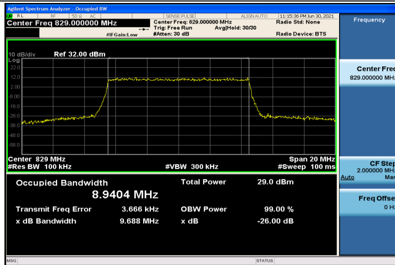
Band5-10MHz-16QAM-20450-50RB#0-8.9404
