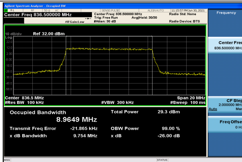
Band5-10MHz-16QAM-20525-50RB#0-8.9649
