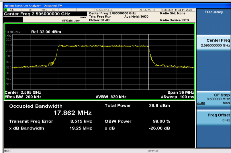
Band38-20MHz-16QAM-38000-100RB#0-17.862
