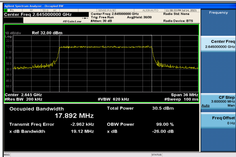
Band41-20MHz-QPSK-41140-100RB#0-17.892
