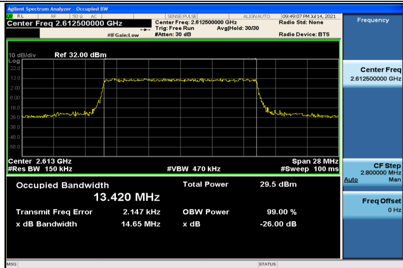
Band38-15MHz-16QAM-38175-75RB#0-13.420
