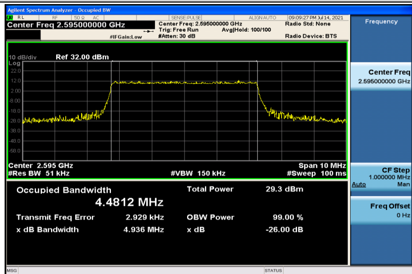
Band38-5MHz-16QAM-38000-25RB#0-4.4812
