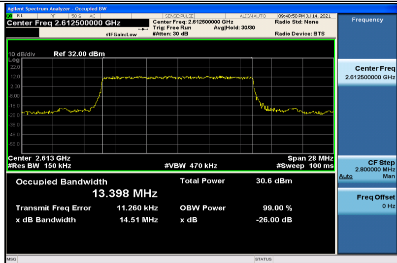
Band38-15MHz-QPSK-38175-75RB#0-13.398
