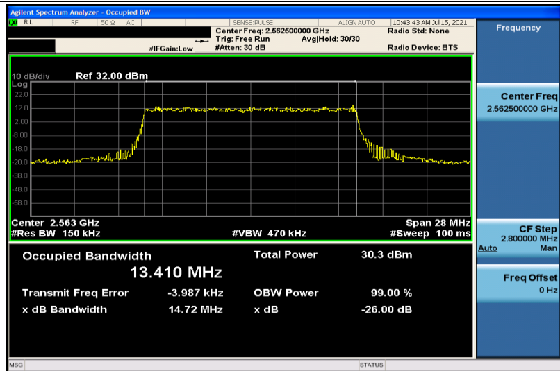
Band41-15MHz-16QAM-40315-75RB#0-13.410
