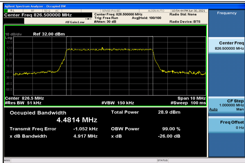
Band5-5MHz-16QAM-20425-25RB#0-4.4814
