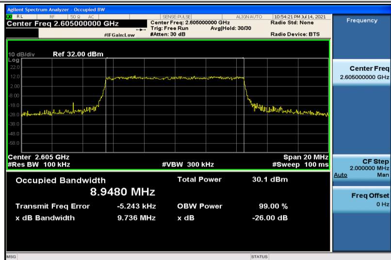
Band41-10MHz-QPSK-40740-50RB#0-8.9480
