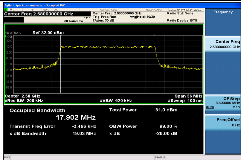
Band38-20MHz-QPSK-37850-100RB#0-17.902
