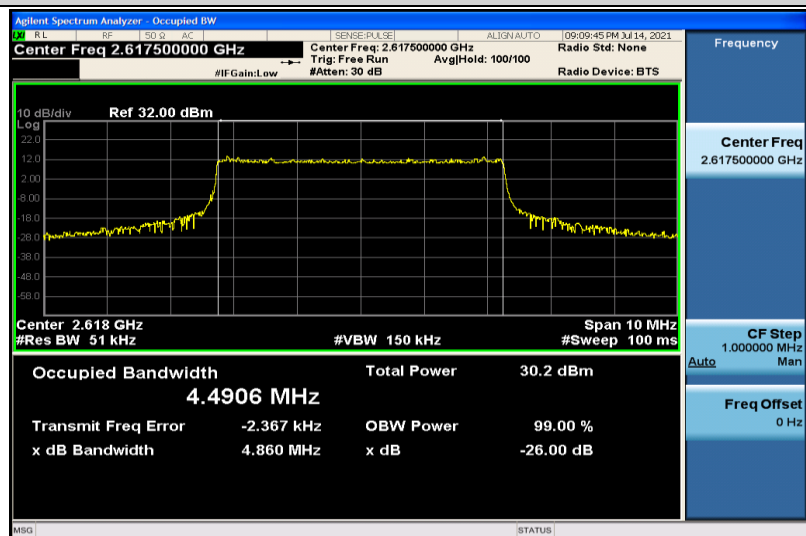
Band38-5MHz-QPSK-38225-25RB#0-4.4906
