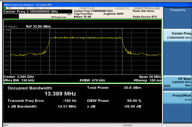
Band38-15MHz-QPSK-38000-75RB#0-13.389
