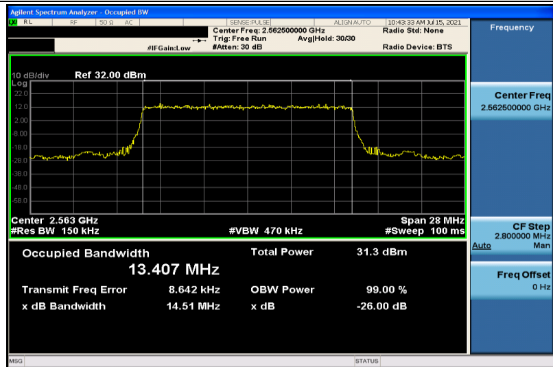
Band41-15MHz-QPSK-40315-75RB#0-13.407
