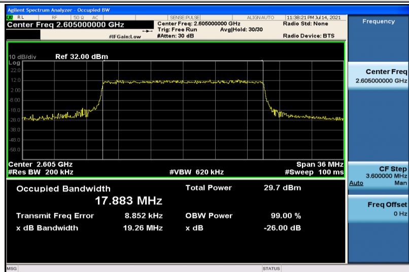
Band41-20MHz-16QAM-40740-100RB#0-17.883
