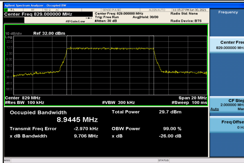
Band5-10MHz-QPSK-20450-50RB#0-8.9445
