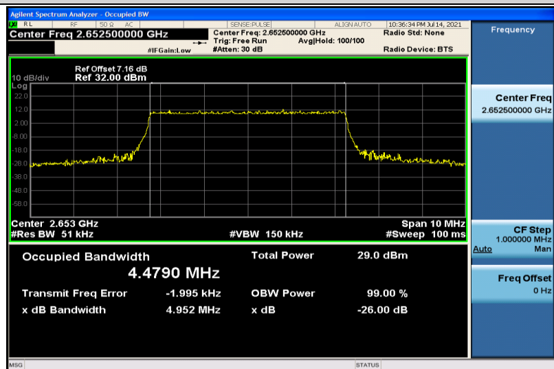
Band41-5MHz-16QAM-41215-25RB#0-4.4790
