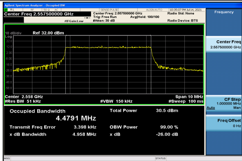
Band41-5MHz-QPSK-40265-25RB#0-4.4791
