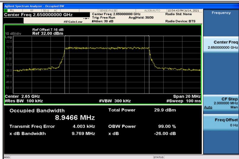
Band41-10MHz-QPSK-41190-50RB#0-8.9466
