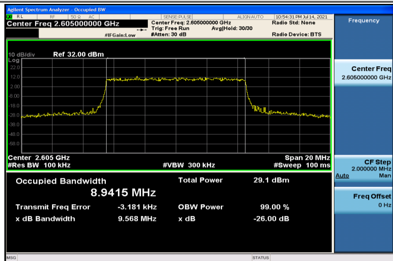
Band41-10MHz-16QAM-40740-50RB#0-8.9415
