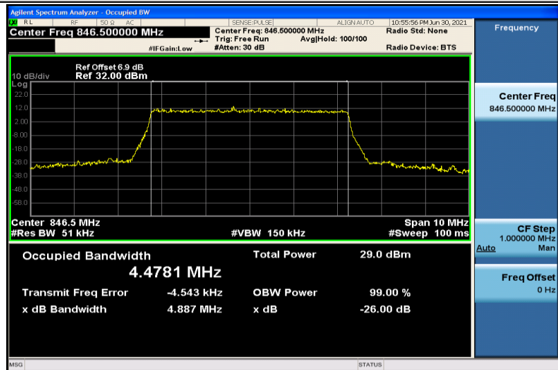
Band5-5MHz-16QAM-20625-25RB#0-4.4781
