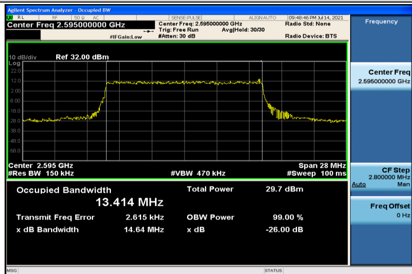
Band38-15MHz-16QAM-38000-75RB#0-13.414
