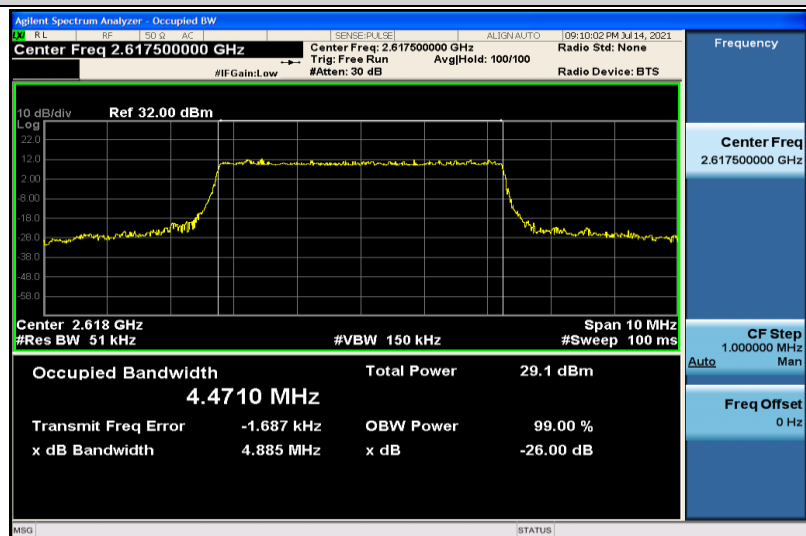
Band38-5MHz-16QAM-38225-25RB#0-4.4710
