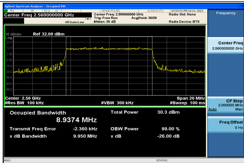
Band41-10MHz-QPSK-40290-50RB#0-8.9374
