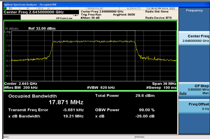
Band41-20MHz-16QAM-41140-100RB#0-17.871
