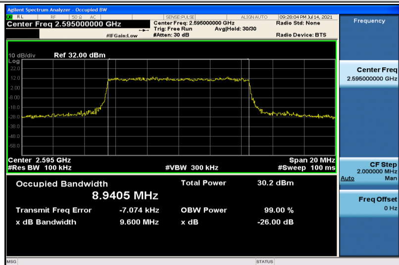
Band38-10MHz-QPSK-38000-50RB#0-8.9405
