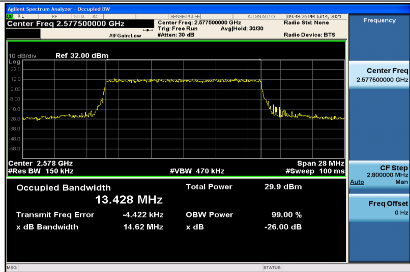
Band38-15MHz-16QAM-37825-75RB#0-13.428
