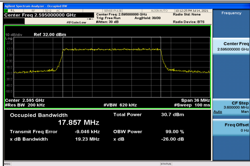
Band38-20MHz-QPSK-38000-100RB#0-17.857
