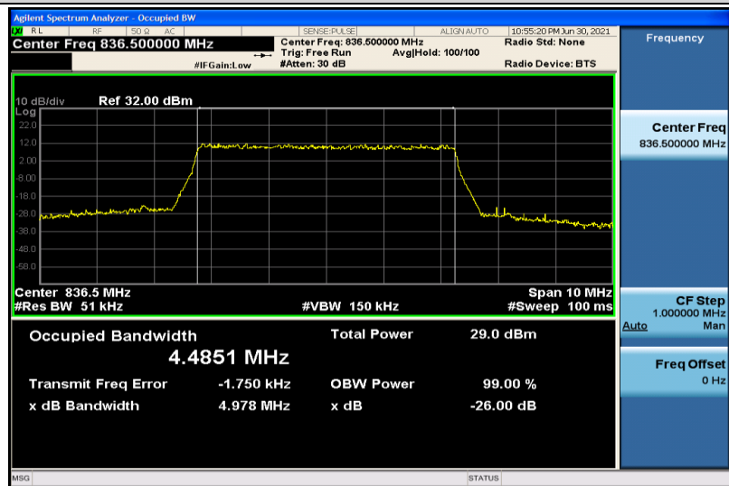
Band5-5MHz-16QAM-20525-25RB#0-4.4851
