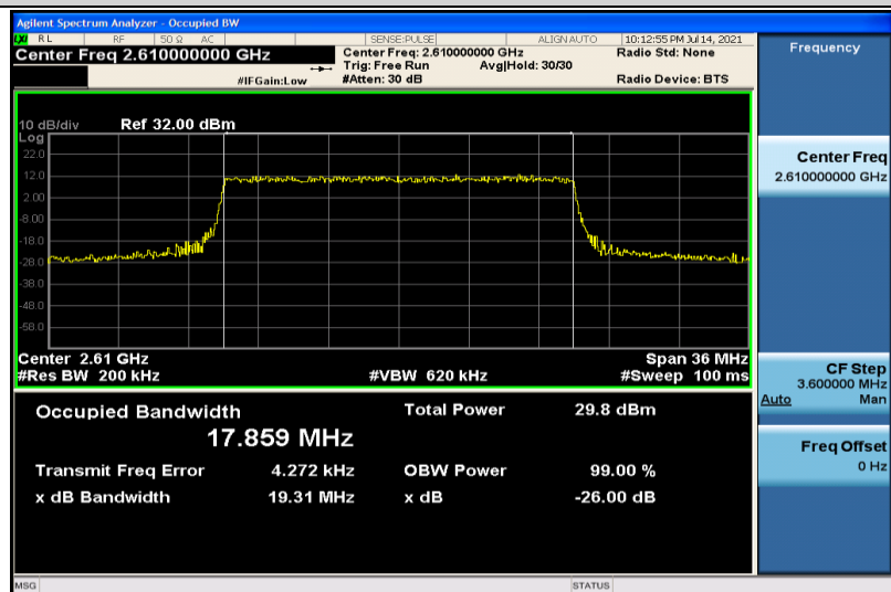
Band38-20MHz-16QAM-38150-100RB#0-17.859
