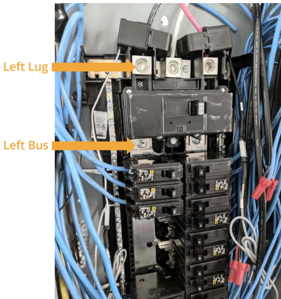
Figure C – Typical Main Breaker Electrical Panel
