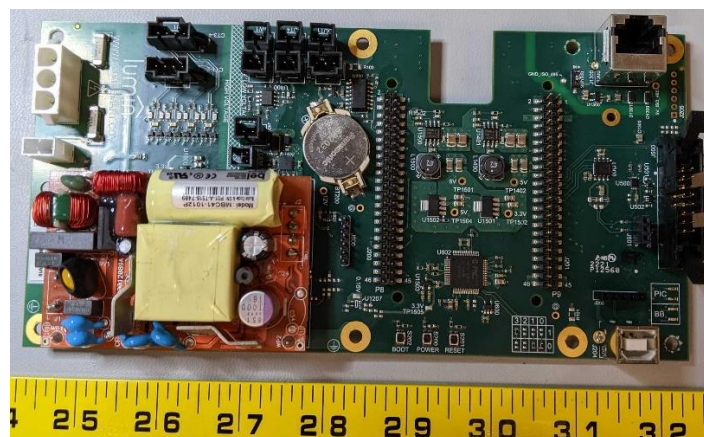
FRONT OF MAIN BOARD
