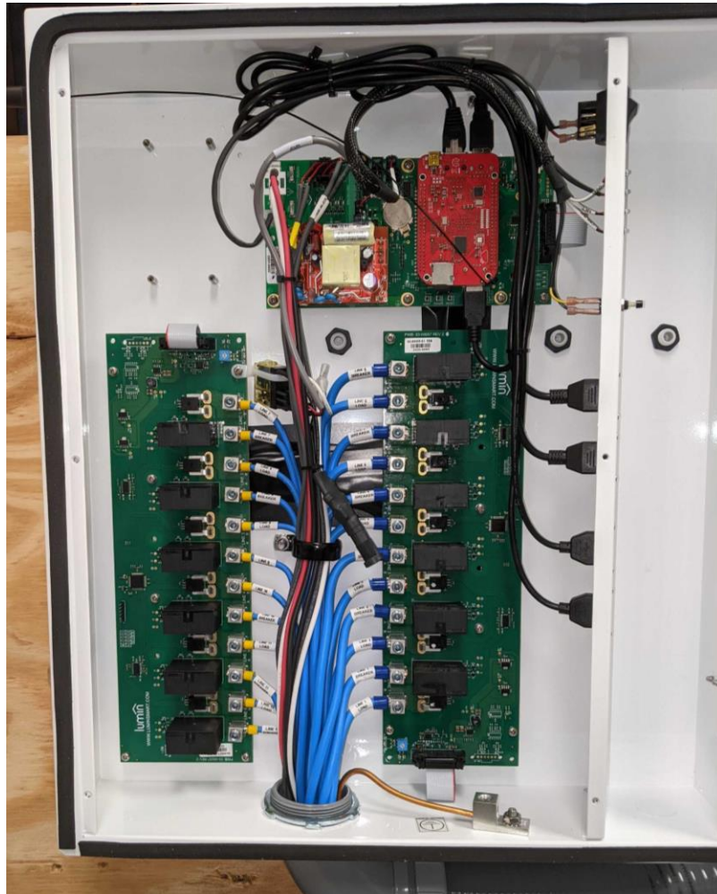
INTERNAL FRONT VIEW
