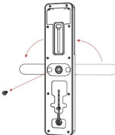
2. Adjust the door handle direction and Tighten the screws
