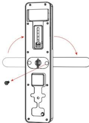
2. Adjust the door handle direction and Tighten the screws
