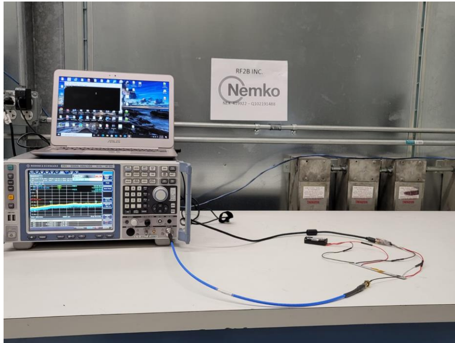
Figure 9 - Conducted emissions setup using a spectrum analyzer.
