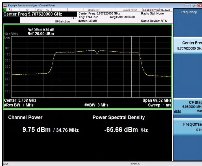
11N40SISO_Ant1_5710_UNII-2C
