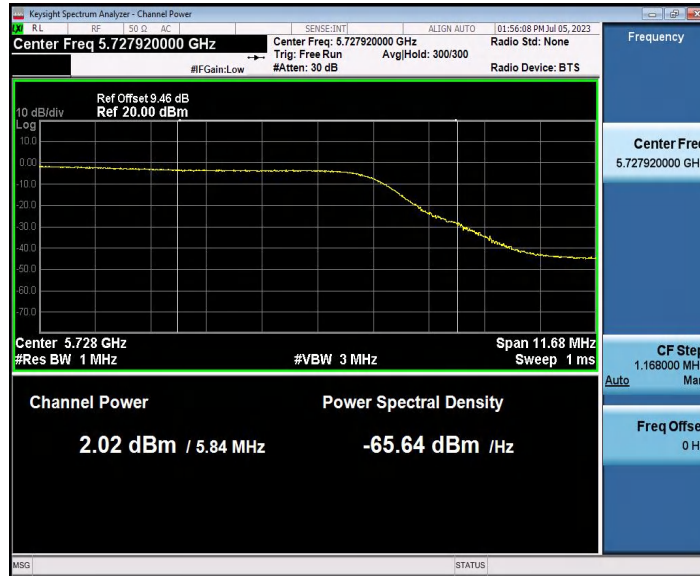
11N20SISO_Ant1_5720_UNII-3
