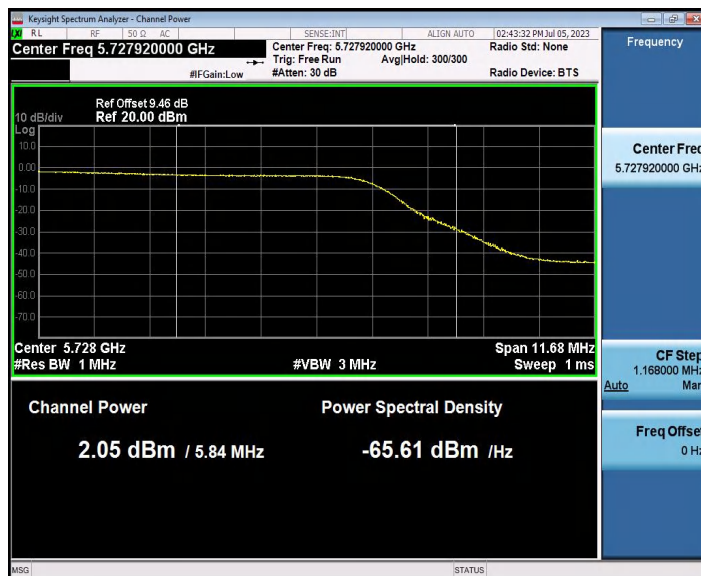
11AC20SISO_Ant1_5720_UNII-3
