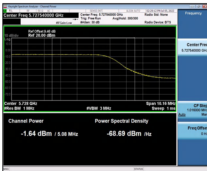
11N40SISO_Ant1_5710_UNII-3
