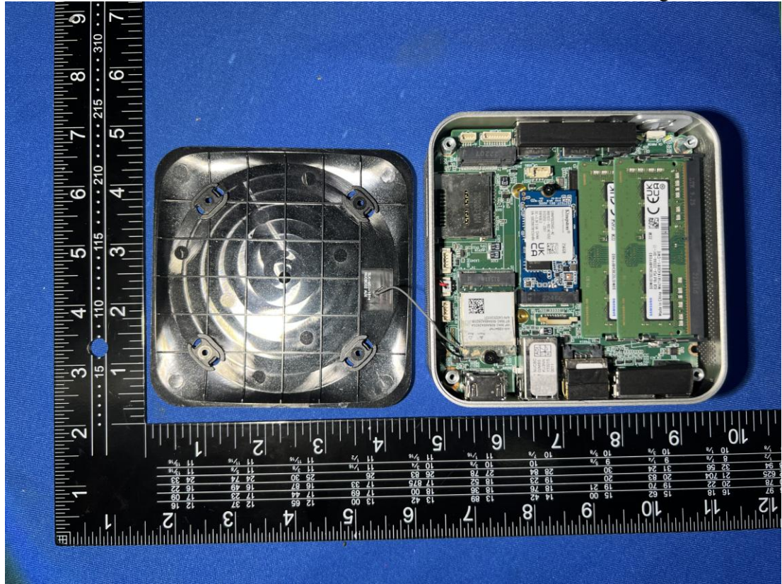
Metal appearance Figure 9 Inside Configuration of the EUT
