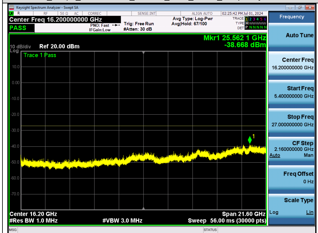
Test Graph 802.11ax160 Chain A 5250 MCS0 Frequency Band 4
