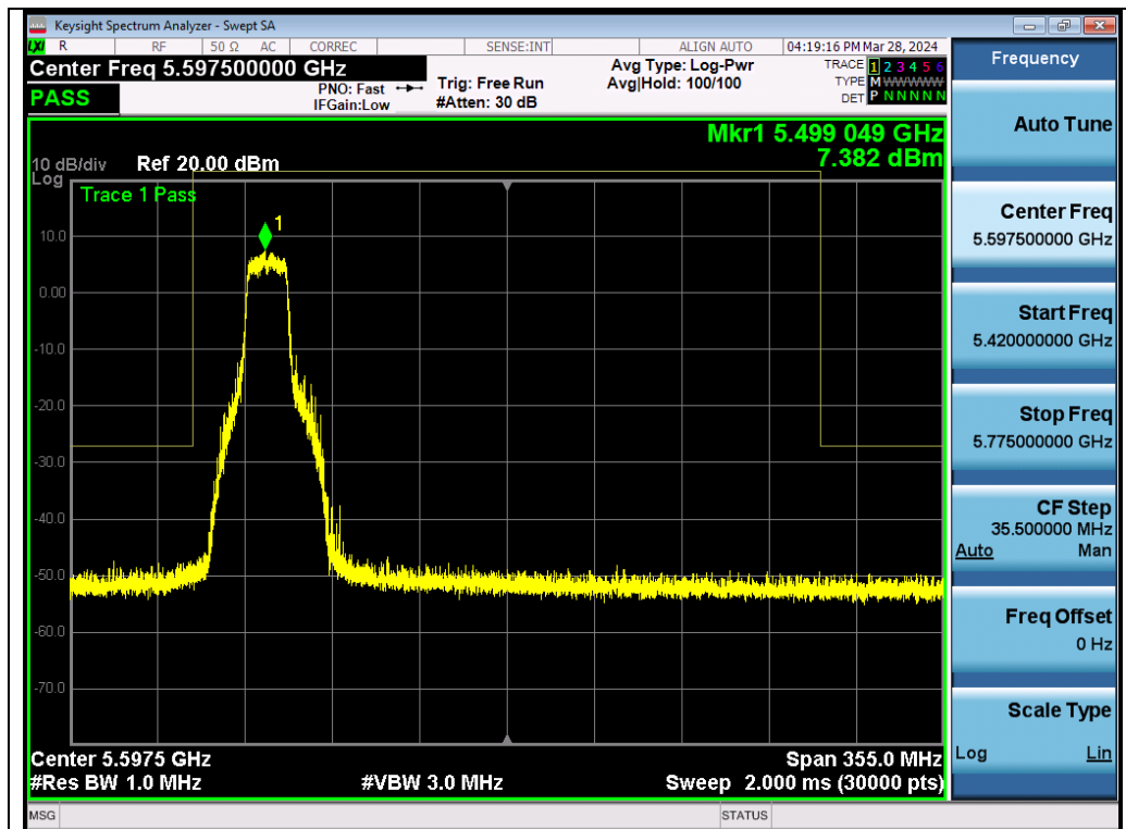
Test_Graph_802.11a_Chain B_5500_6Mbps_Frequency Band 3
