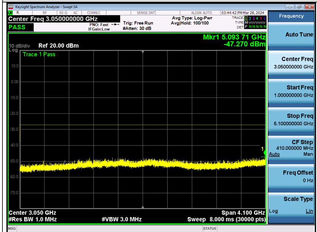
Test_Graph_802.11n40_Chain B_5310_MCS0_Frequency Band 2
