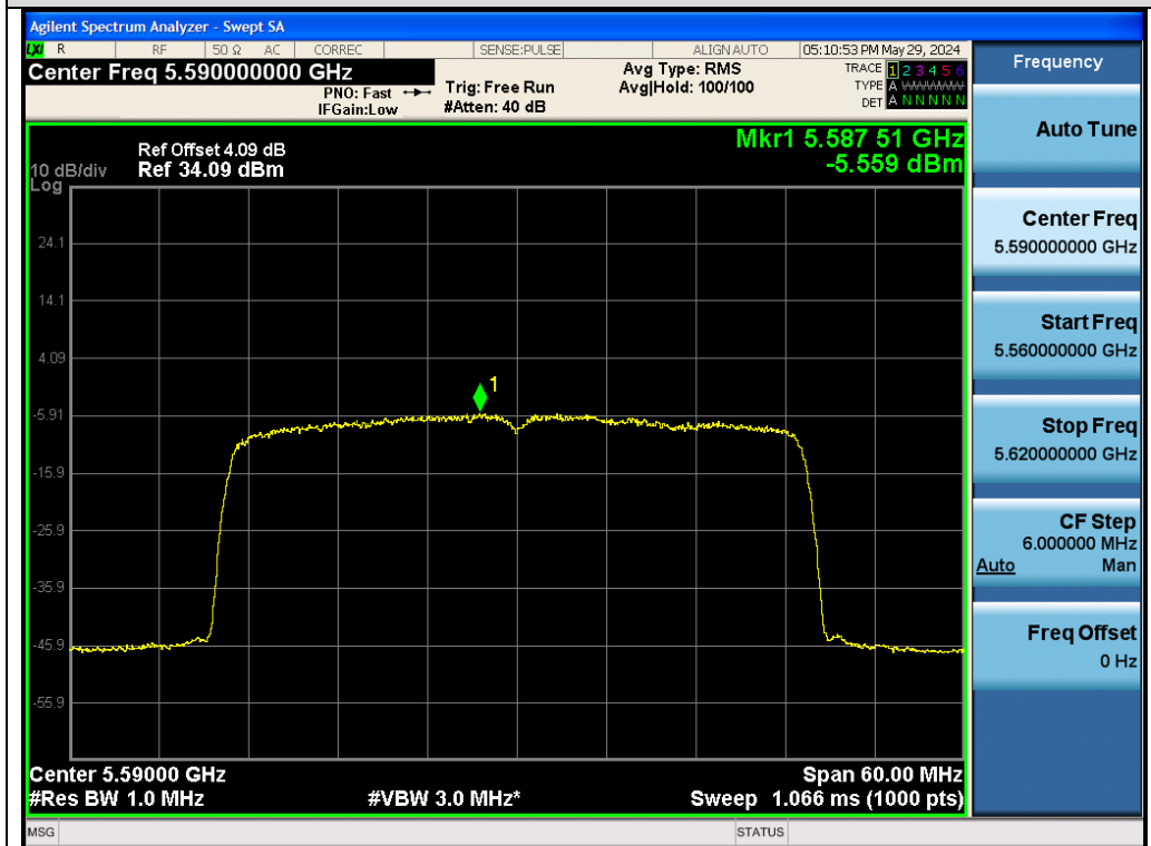
Test_Graph_802.11ax40_Chain A_5590_MCS0_PSD
