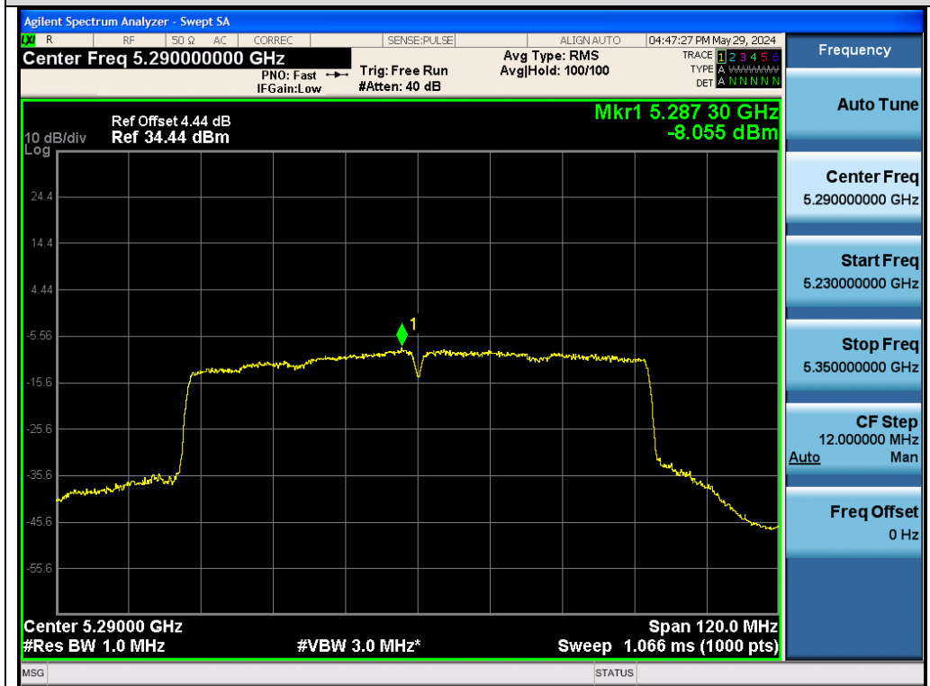
Test_Graph_802.11ac80_Chain A_5290_MCS0_PSD
