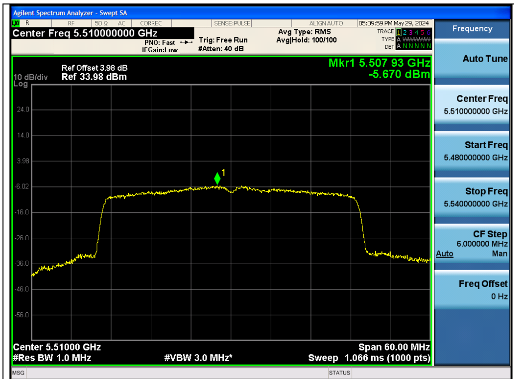
Test_Graph_802.11ax40_Chain A_5510_MCS0_PSD
