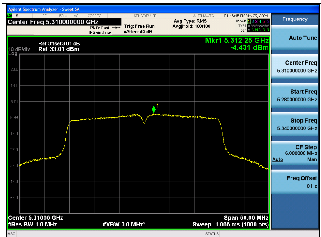
Test_Graph_802.11ac40_Chain A_5310_MCS0_PSD
