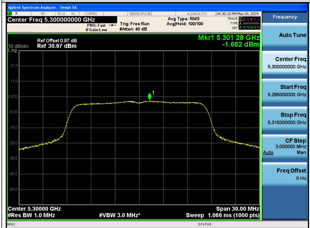
Test_Graph_802.11a_Chain A_5300_6Mbps_PSD
