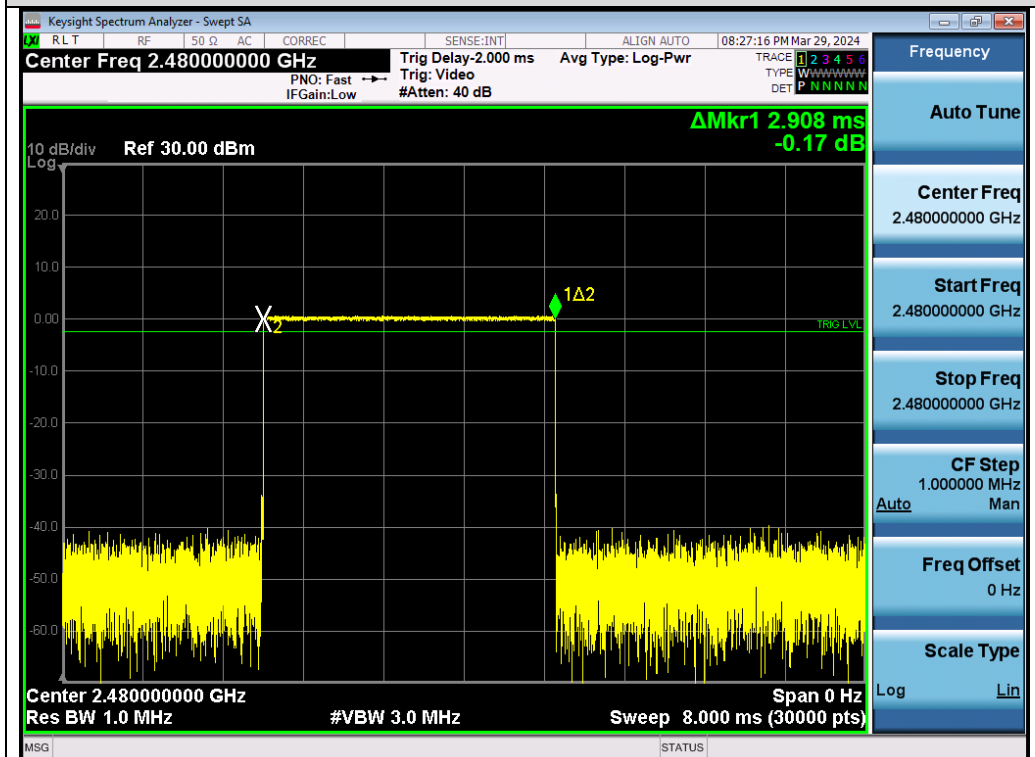
Test_Graph_BR_HOP_Chain A_NA_1Mbps_2480_Time per Burst
