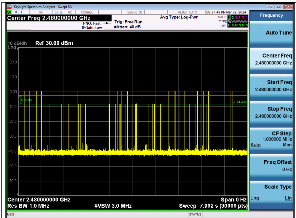
Test_Graph_BR_HOP_Chain A_NA_1Mbps_2480_Number of Burst
