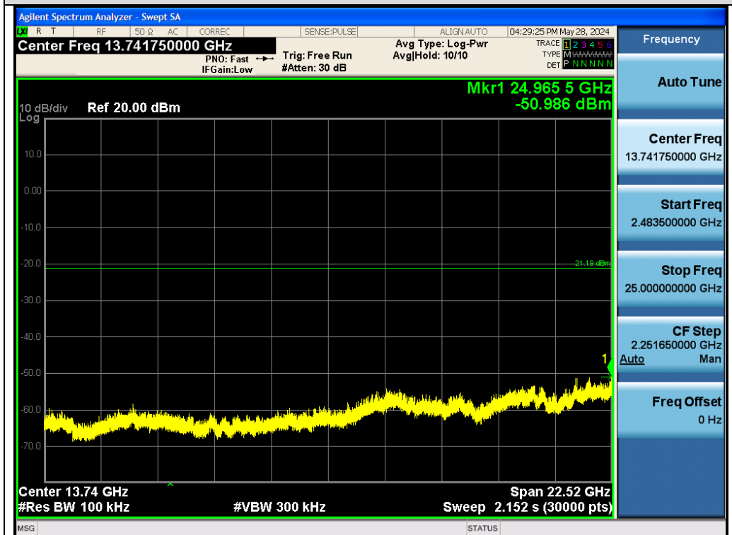
Test_Graph_EDR_Chain A_2441_3Mbps_Higher Band Emissions
