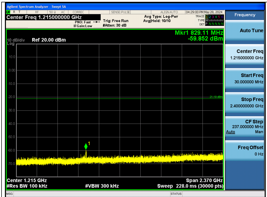
Test_Graph_EDR_Chain A_2441_3Mbps_Lower Band Emissions
