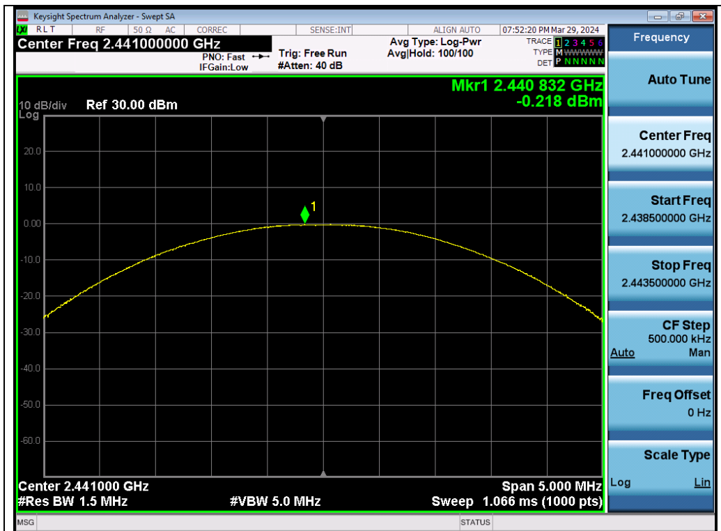
Test_Graph_EDR_Chain A_2441_2Mbps_Peak Power
