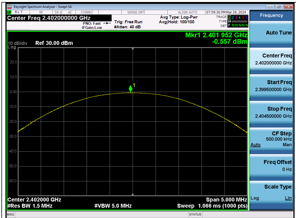
Test_Graph_EDR_Chain A_2402_3Mbps_Peak Power
