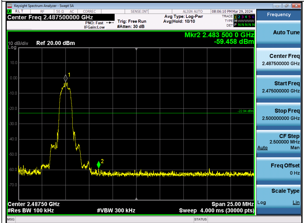
Test_Graph_EDR_Chain A_2480_3Mbps_Higher Band Edge Emissions
