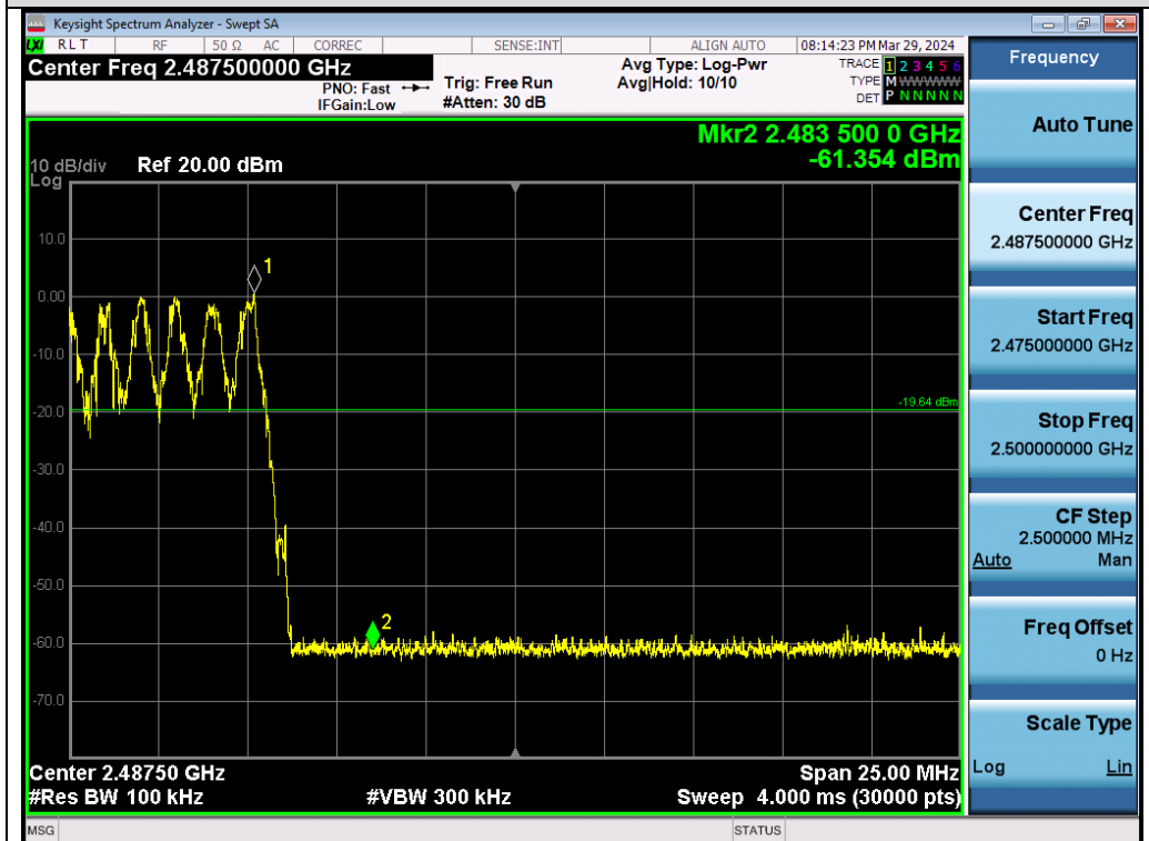
Test_Graph_BR_HOP_Chain A_NA_1Mbps_Higher Band Edge Emissions
