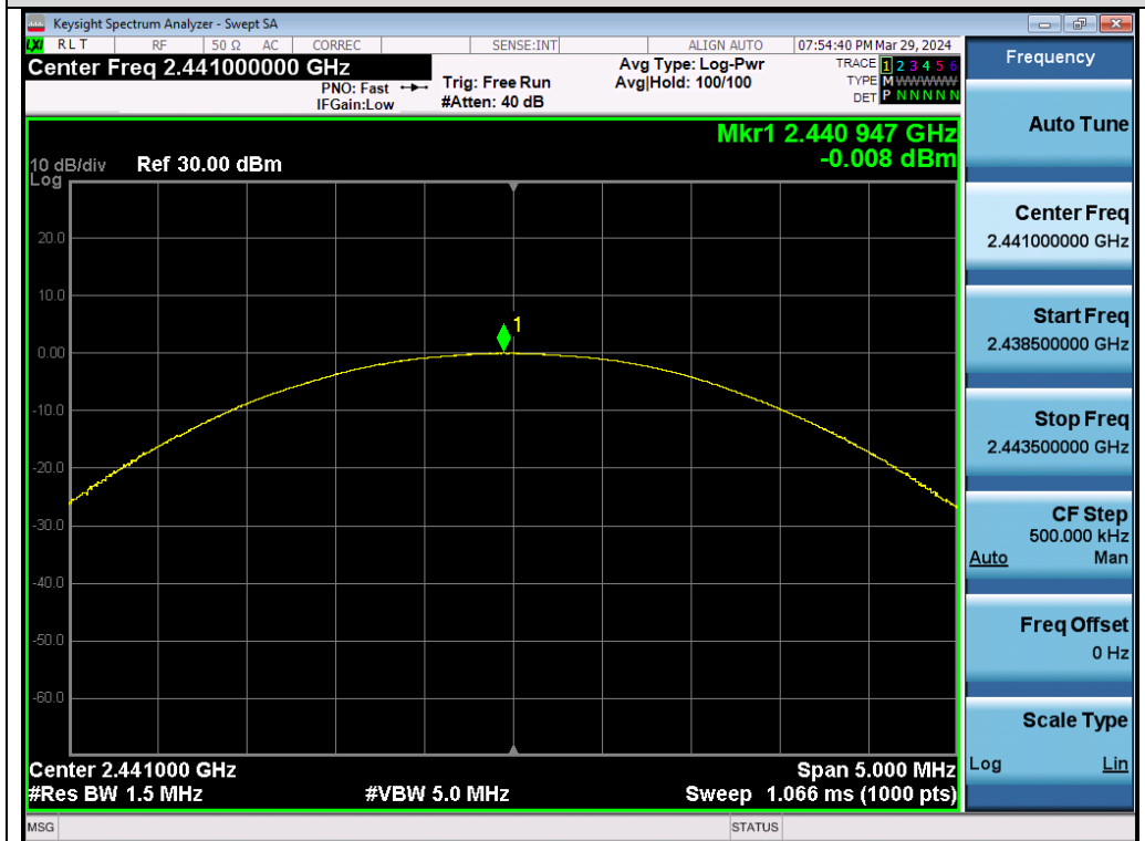
Test_Graph_EDR_Chain A_2441_3Mbps_Peak Power
