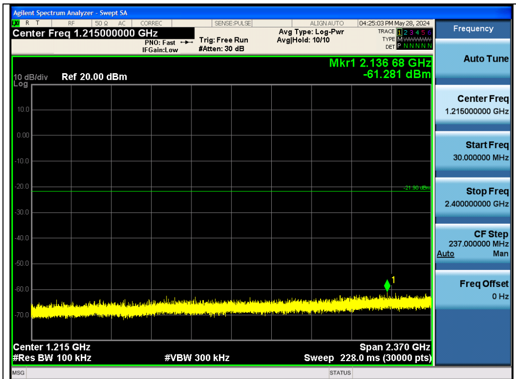
Test_Graph_EDR_Chain A_2480_2Mbps_Lower Band Emissions
