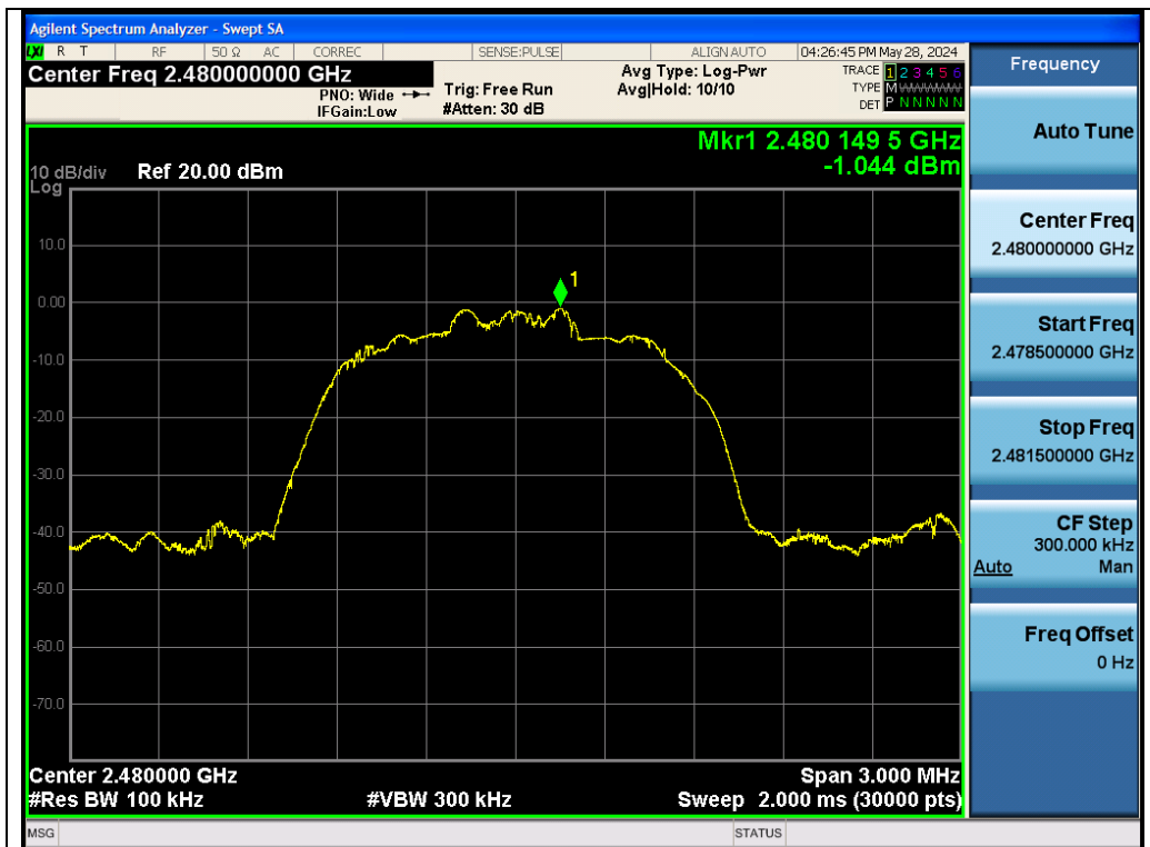
Test_Graph_EDR_Chain A_2480_3Mbps_Reference Level
