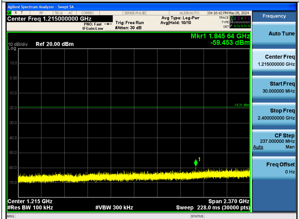
Test_Graph_BR_Chain A_2480_1Mbps_Lower Band Emissions
