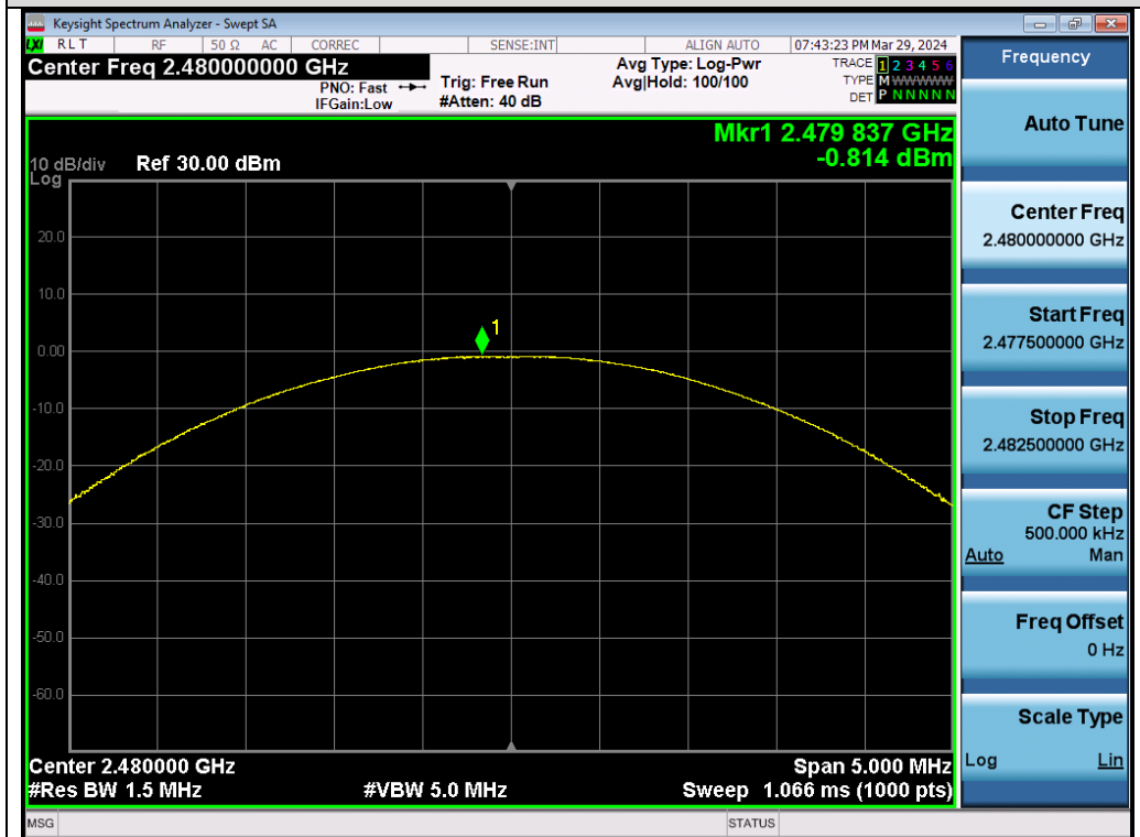
Test_Graph_EDR_Chain A_2480_2Mbps_Peak Power
