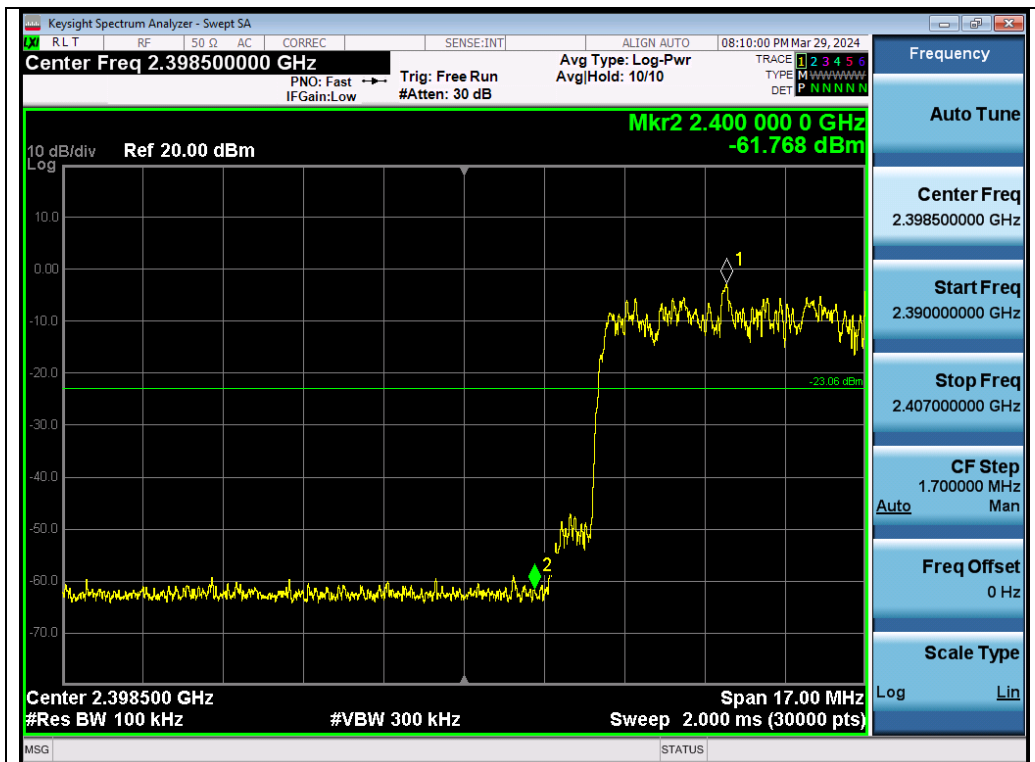
Test_Graph_EDR_HOP_Chain A_NA_3Mbps_Lower Band Edge Emissions
