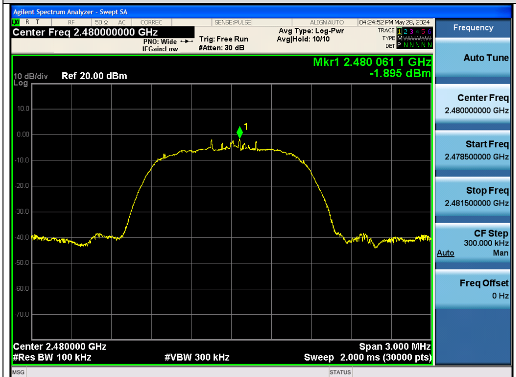
Test_Graph_EDR_Chain A_2480_2Mbps_Reference Level
