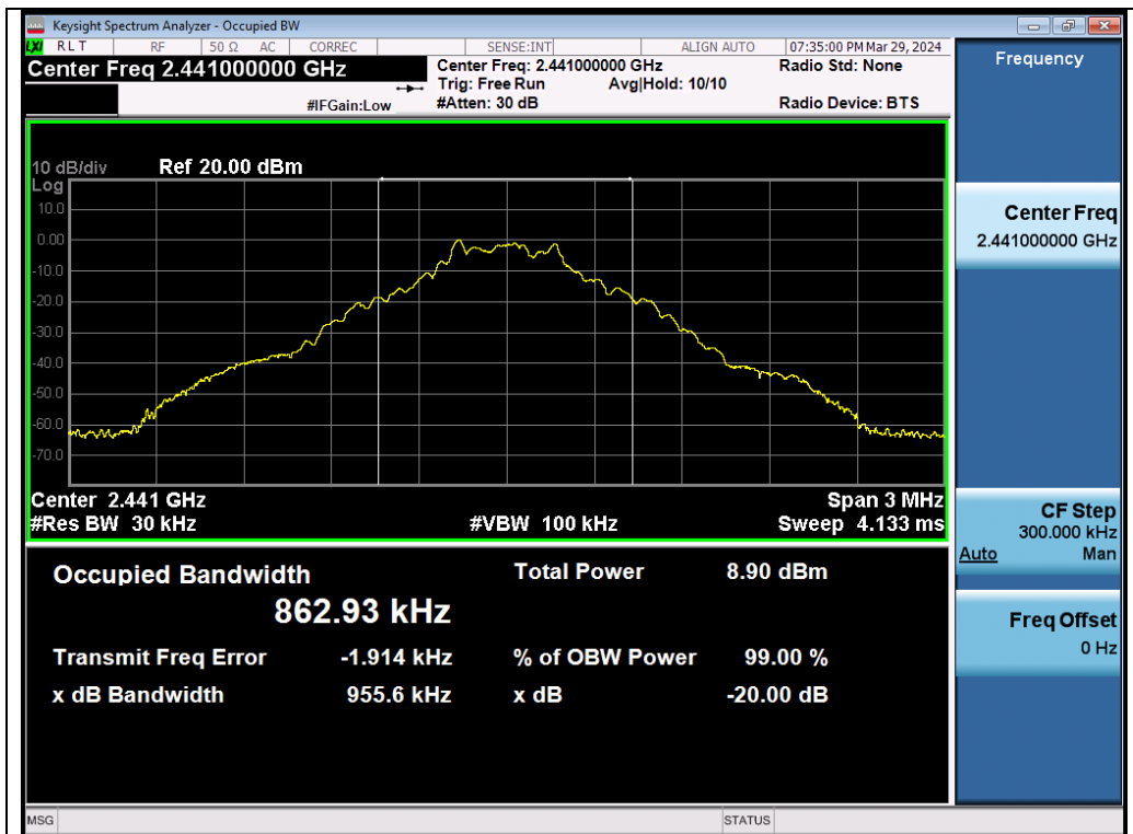
Test_Graph_BR_Chain A_2441_1Mbps_OBW
