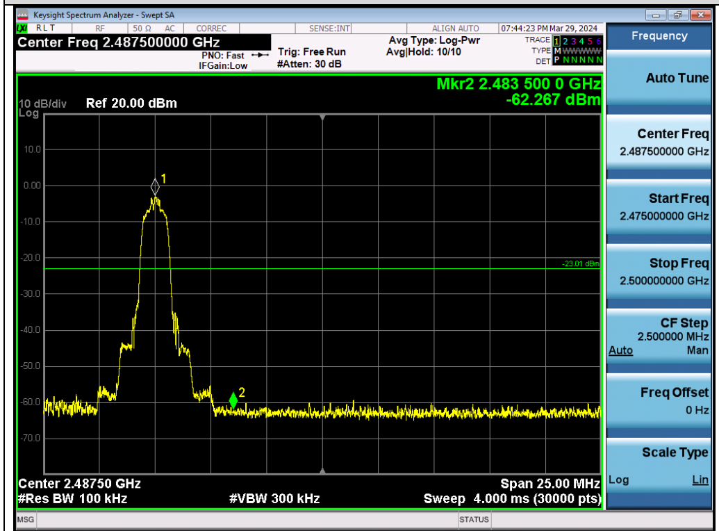
Test_Graph_EDR_Chain A_2480_2Mbps_Higher Band Edge Emissions
