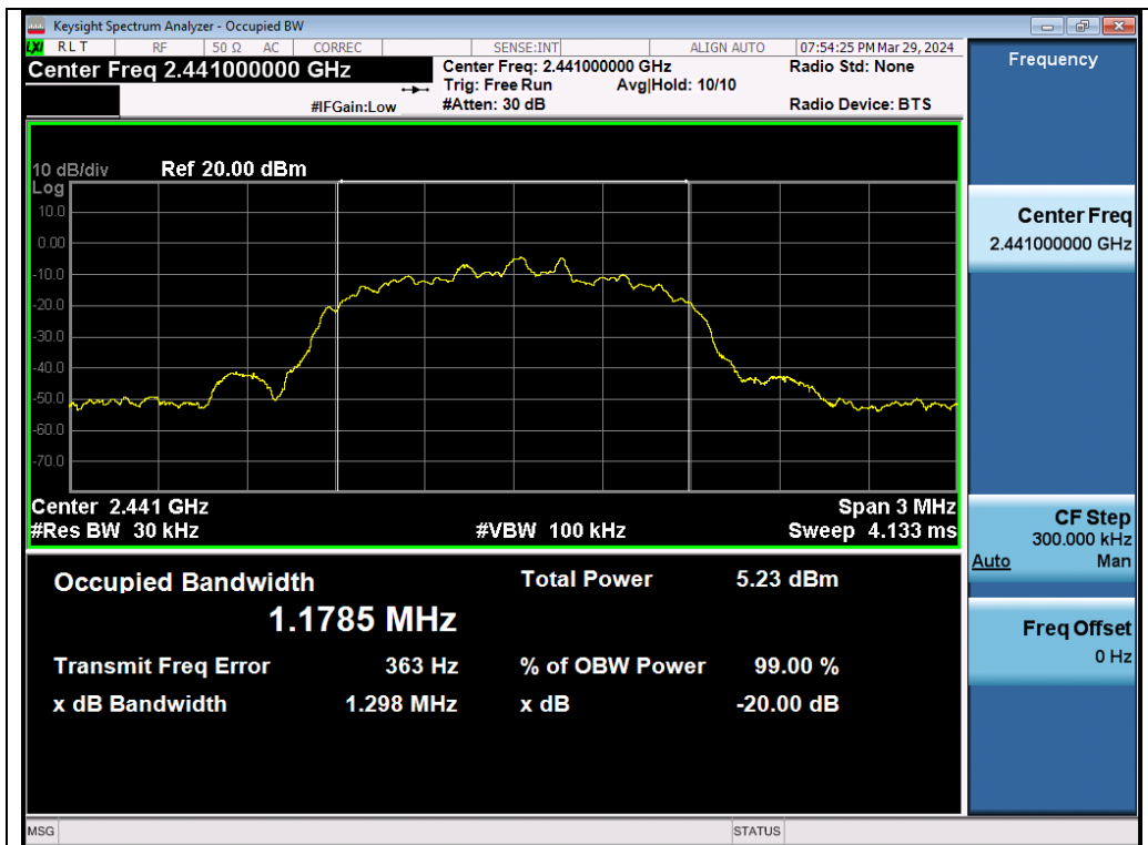
Test_Graph_EDR_Chain A_2441_3Mbps_OBW
