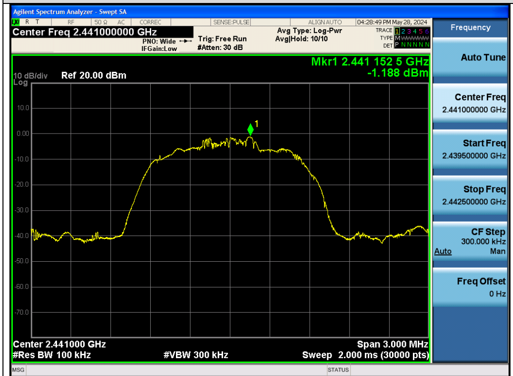
Test_Graph_EDR_Chain A_2441_3Mbps_Reference Level
