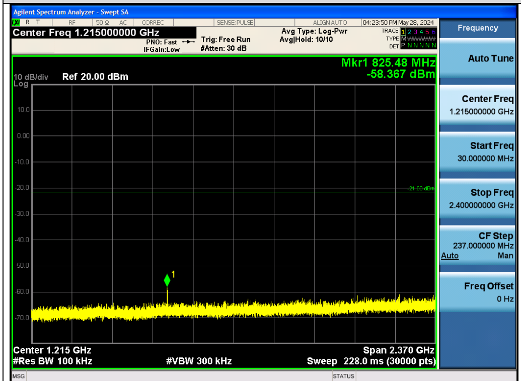
Test_Graph_EDR_Chain A_2441_2Mbps_Lower Band Emissions
