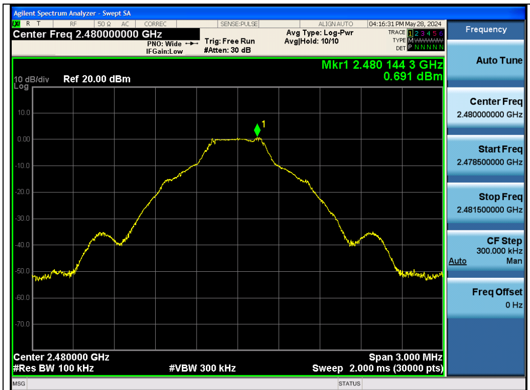
Test_Graph_BR_Chain A_2480_1Mbps_Reference Level
