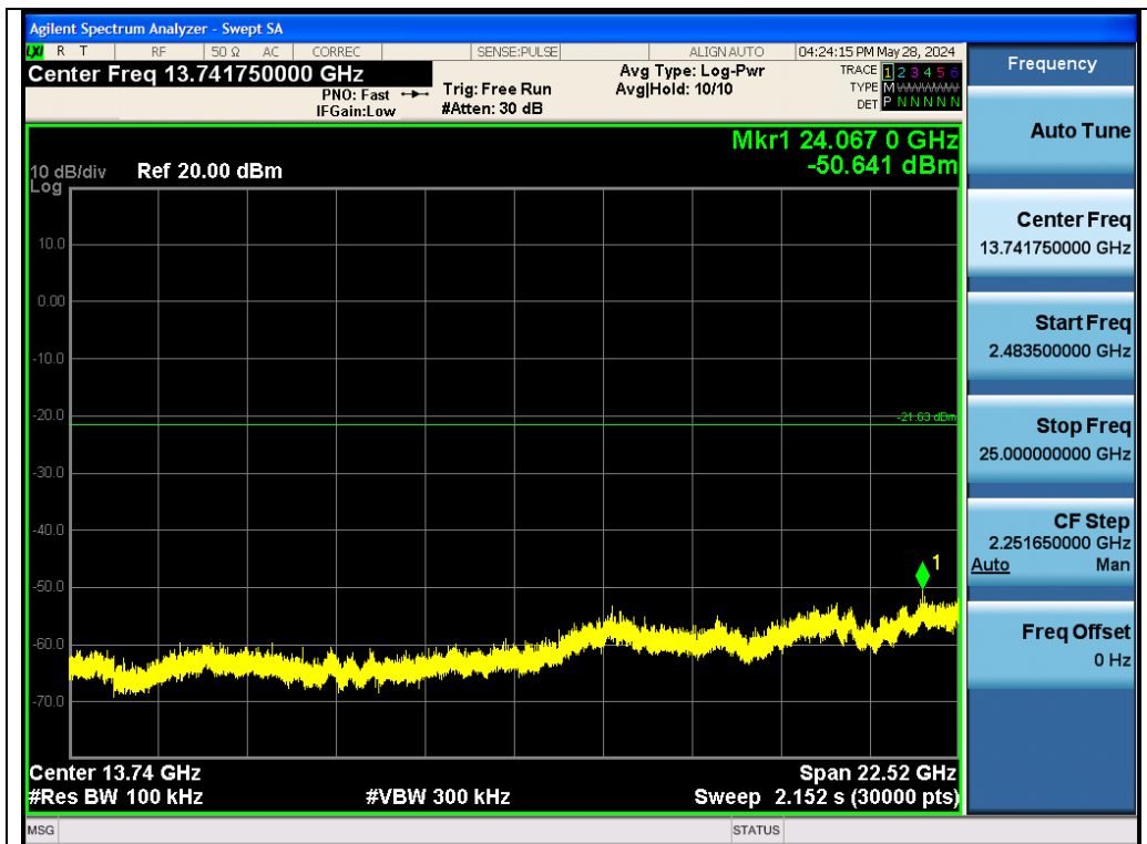
Test_Graph_EDR_Chain A_2441_2Mbps_Higher Band Emissions
