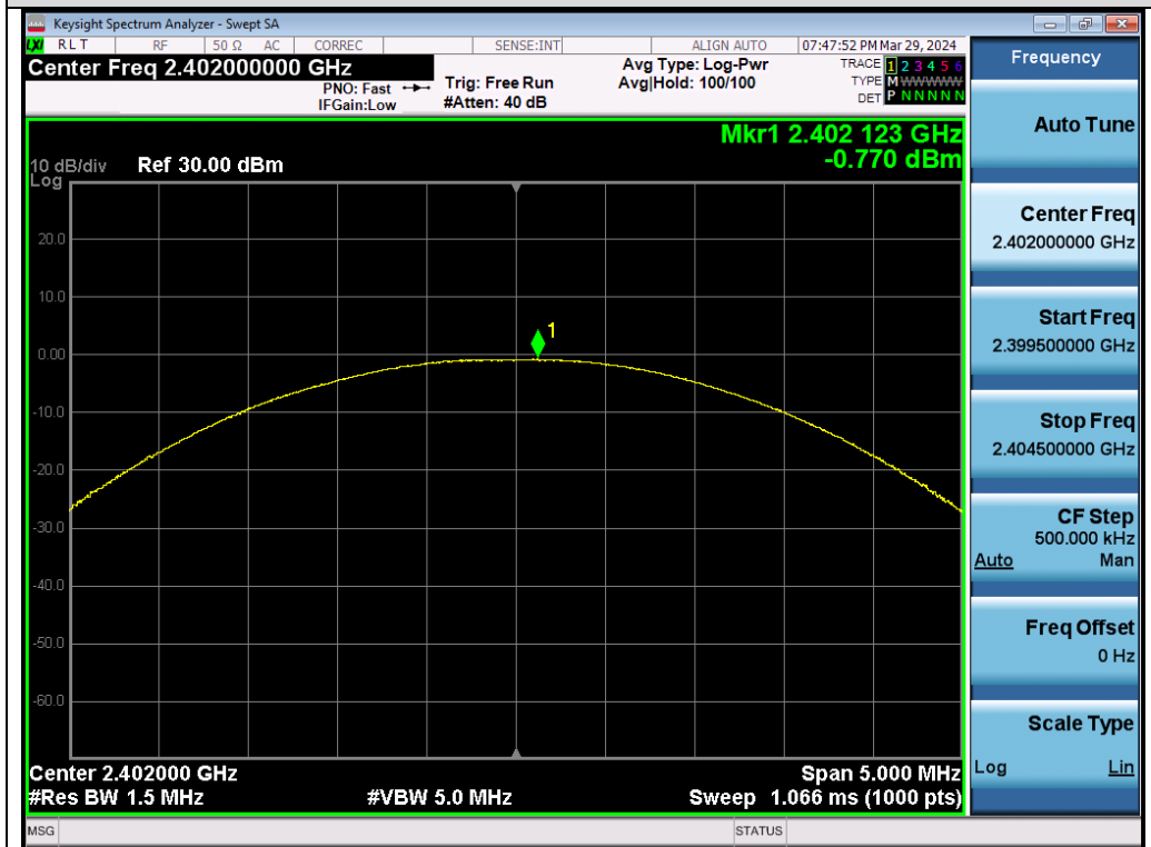
Test_Graph_EDR_Chain A_2402_2Mbps_Peak Power
