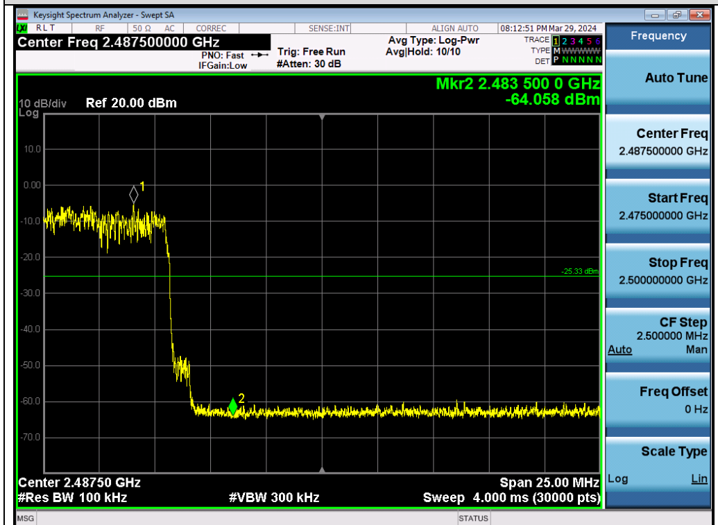
Test_Graph_EDR_HOP_Chain A_NA_2Mbps_Higher Band Edge Emissions
