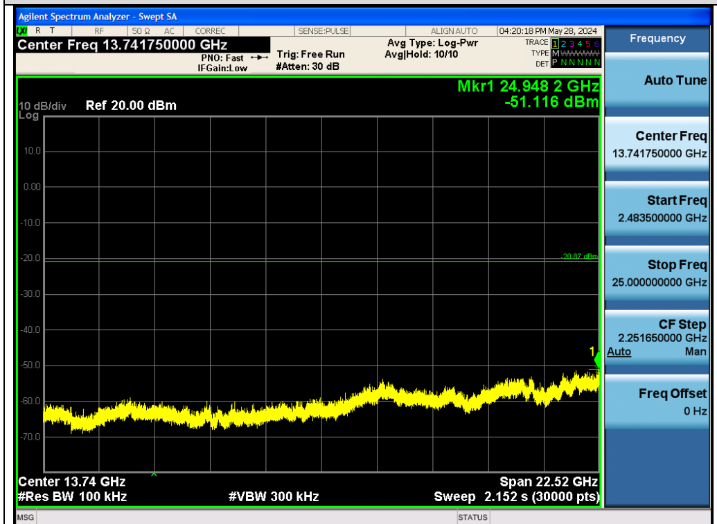
Test_Graph_EDR_Chain A_2402_2Mbps_Higher Band Emissions
