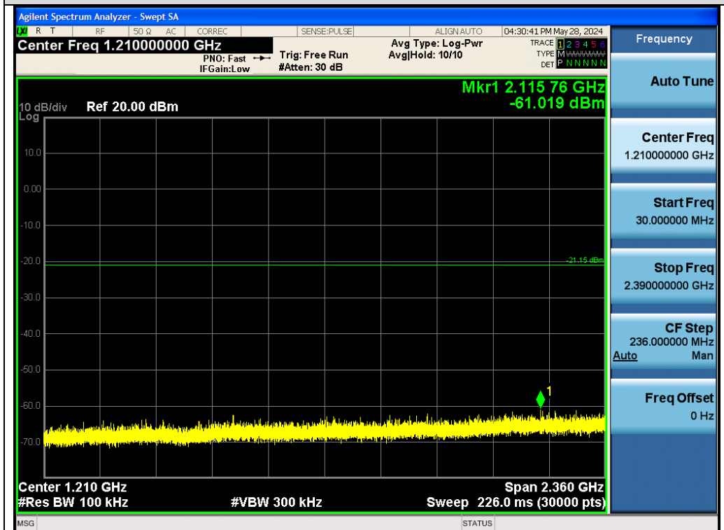
Test_Graph_EDR_Chain A_2402_3Mbps_Lower Band Emissions
