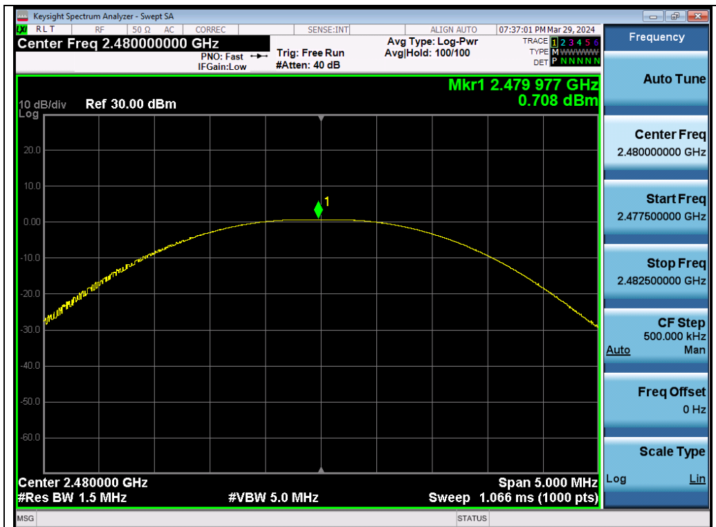
Test_Graph_BR_Chain A_2480_1Mbps_Peak Power
