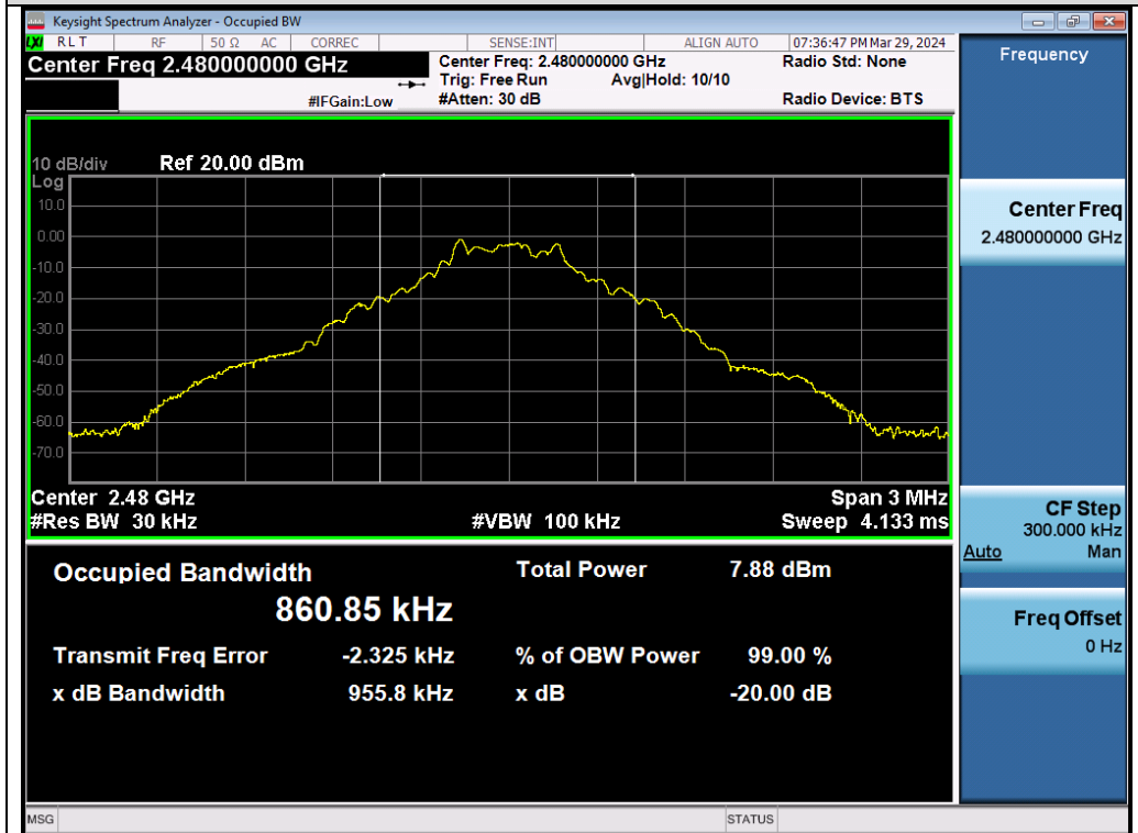
Test_Graph_BR_Chain A_2480_1Mbps_OBW
