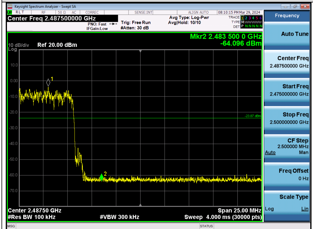
Test_Graph_EDR_HOP_Chain A_NA_3Mbps_Higher Band Edge Emissions
