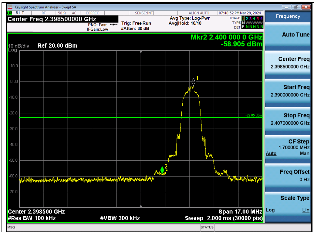
Test_Graph_EDR_Chain A_2402_2Mbps_Lower Band Edge Emissions
