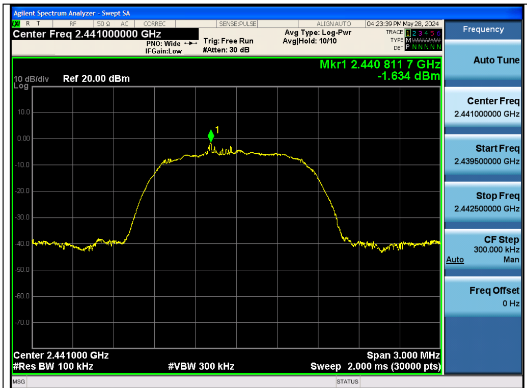
Test_Graph_EDR_Chain A_2441_2Mbps_Reference Level
