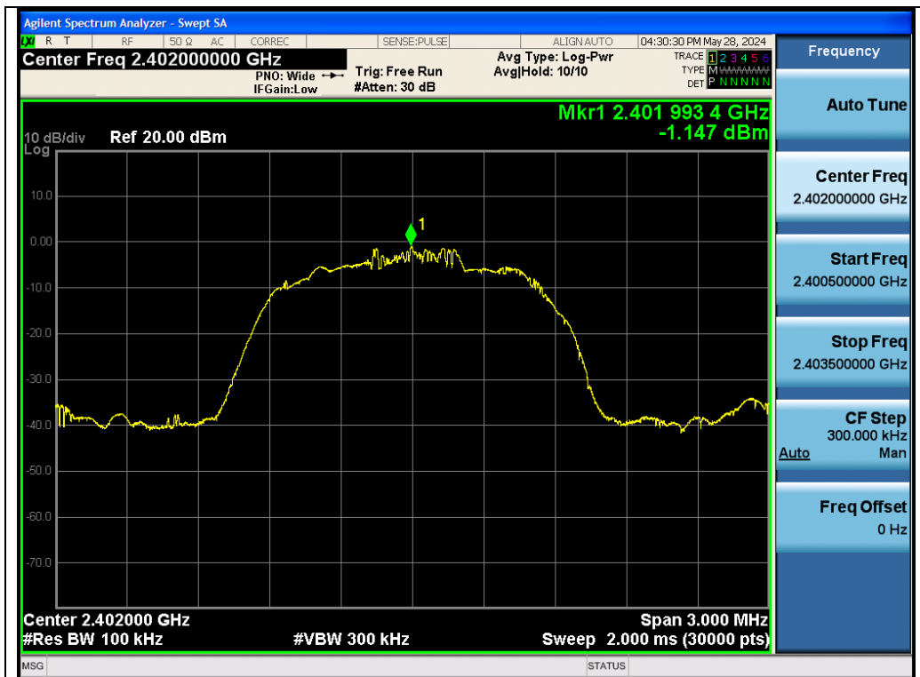
Test_Graph_EDR_Chain A_2402_3Mbps_Reference Level
