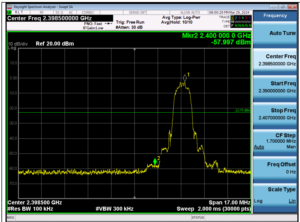
Test_Graph_EDR_Chain A_2402_3Mbps_Lower Band Edge Emissions
