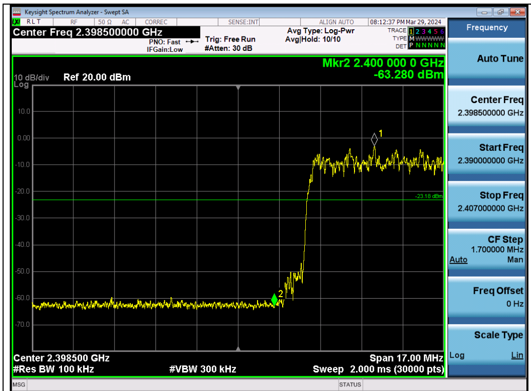
Test_Graph_EDR_HOP_Chain A_NA_2Mbps_Lower Band Edge Emissions
