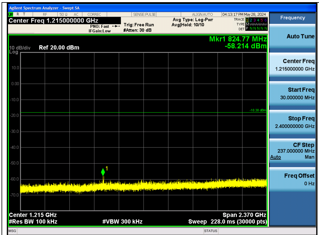
Test_Graph_BR_Chain A_2441_1Mbps_Lower Band Emissions
