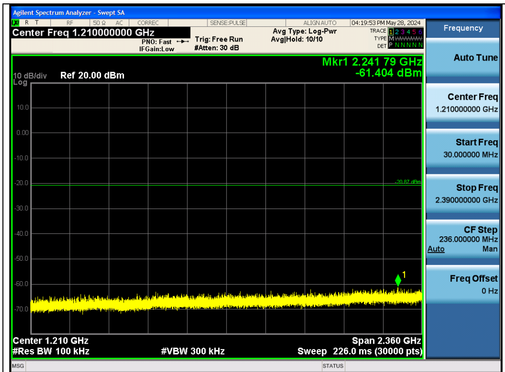
Test_Graph_EDR_Chain A_2402_2Mbps_Lower Band Emissions
