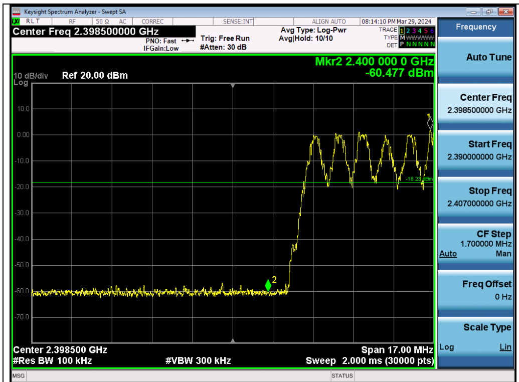
Test_Graph_BR_HOP_Chain A_NA_1Mbps_Lower Band Edge Emissions
