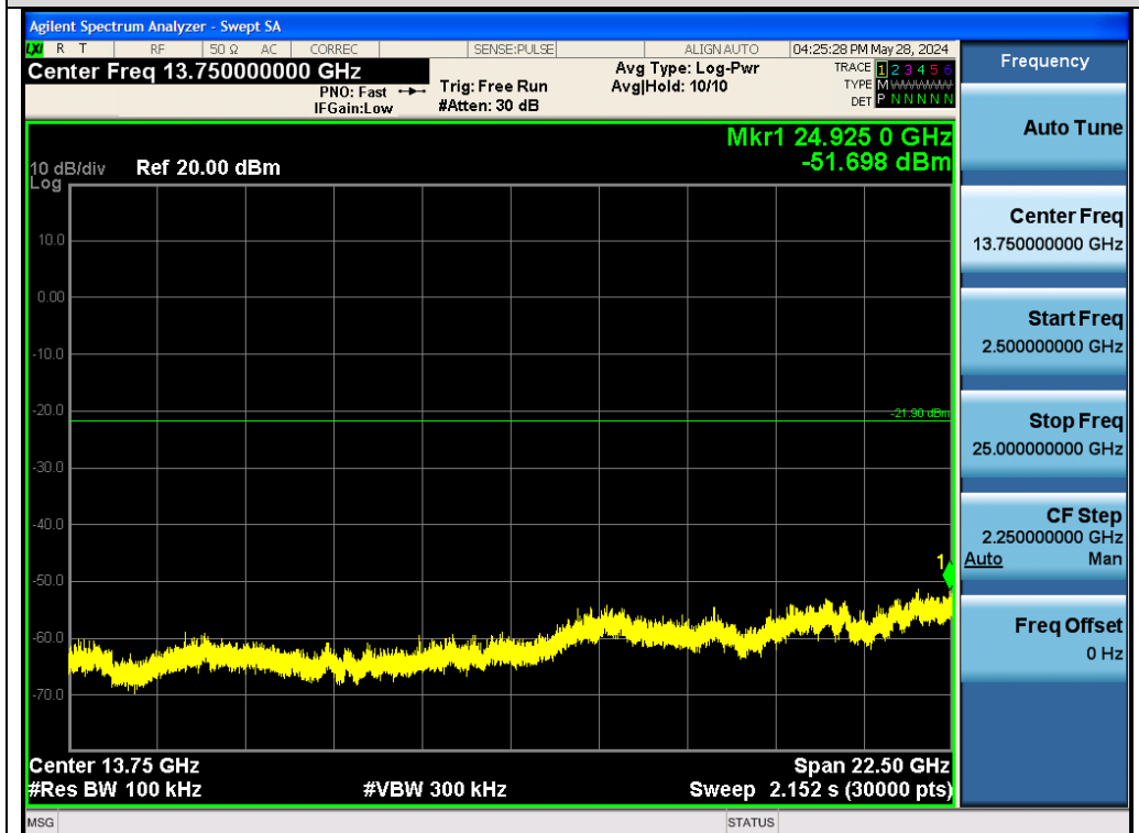
Test_Graph_EDR_Chain A_2480_2Mbps_Higher Band Emissions
