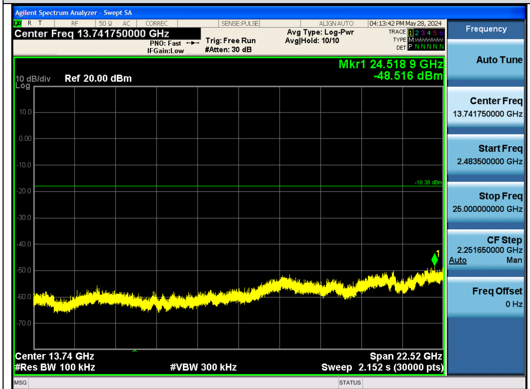
Test_Graph_BR_Chain A_2441_1Mbps_Higher Band Emissions
