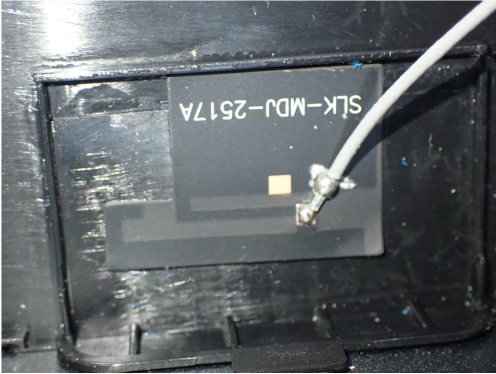
BT&2.4GWIFI&5GWIFI ANTENNA
