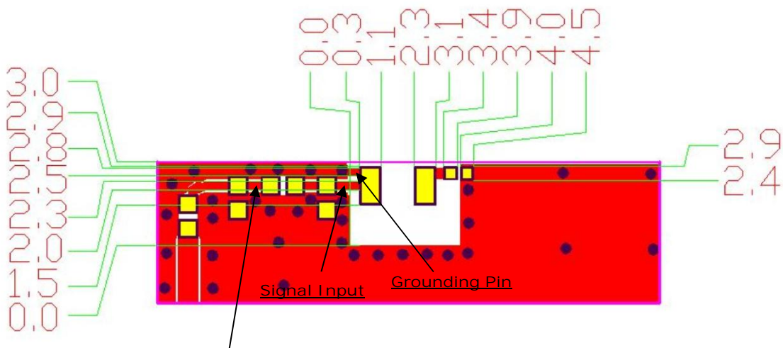
Transmission Line with 50 \Omega Impedance Characteristic
