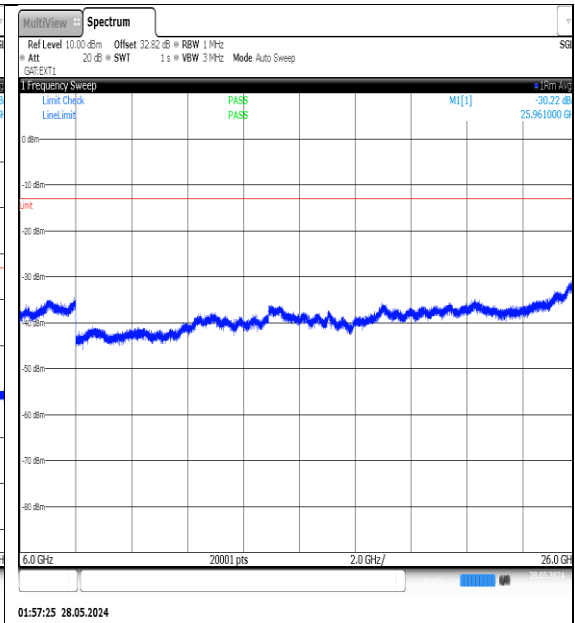
NTVN-N77-3450-3550-PC3-30-30-H-DFT-QPSK-Edge_1RB_Left-6000-26000-Ant1-PASS
