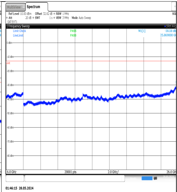
NTNV-N77-3450-3550-PC3-30-25-M-DFT-QPSK- Edge_1RB_Left-6000-26000-Ant1-PASS
