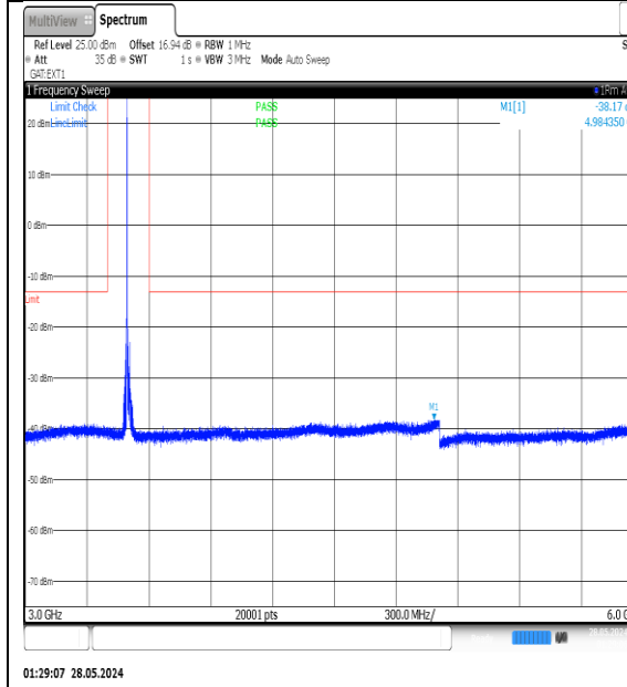
NTNV-N77-3450-3550-PC3-30-15-M-DFT-QPSK-Edge_1RB_Left-3000-6000-Ant1-PASS
