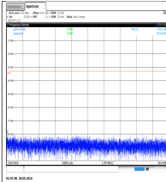
NTNV-N77-3450-3550-PC3-30-25-H-DFT-QPSK- Edge_1RB_Left-0.15-30-Ant1-PASS
