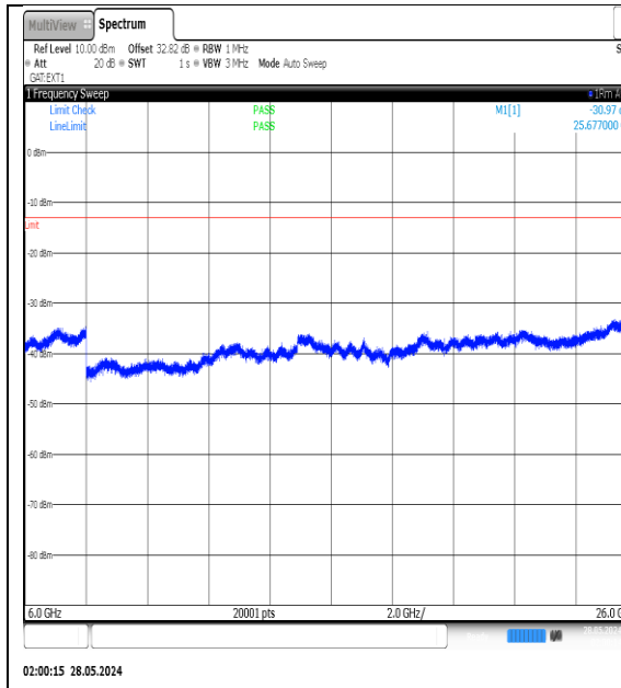
NTNV-N77-3450-3550-PC3-30-40-L-DFT-QPSK-Edge_1RB_Left-6000-26000-Ant1-PASS
