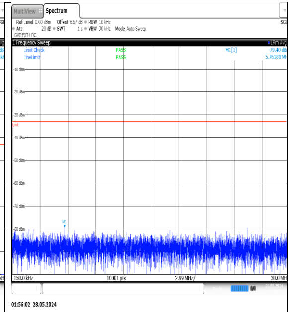
NTNV-N77-3450-3550-PC3-30-30-H-DFT-QPSK-Edge_1RB_Left-0.15-30-Ant1-PASS
