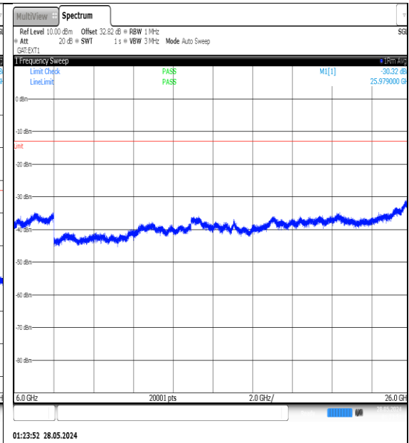
NTVN-N77-3450-3550-PC3-30-10-H-DFT-QPSK-Edge_1RB_Left-6000-26000-Ant1-PASS
