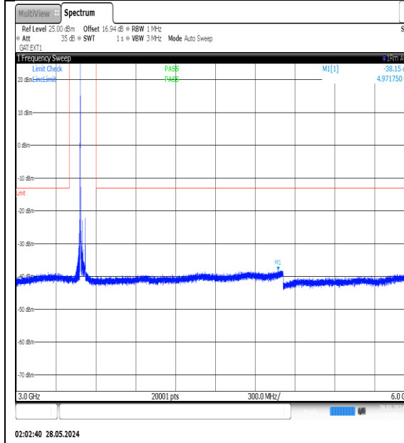
NTNV-N77-3450-3550-PC3-30-40-M-DFT-QPSK-Edge_1RB_Left-3000-6000-Ant1-PASS
