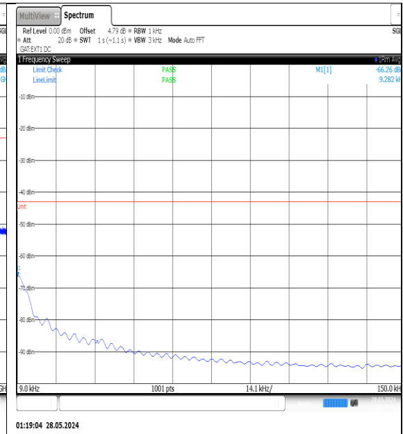
N77-3450-3550-PC3-30-10-M-DFT-QPSK- Edge_1RB_Left-0.009-0.15-Ant1-PASS
