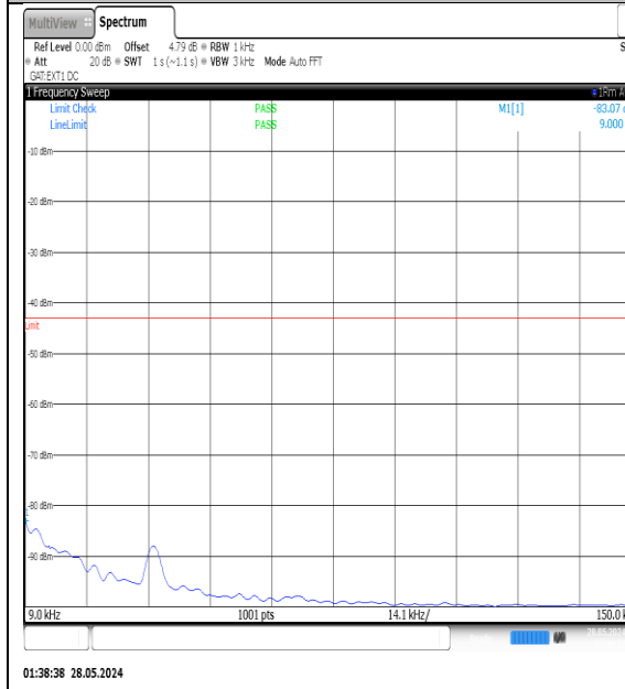
NTNV-N77-3450-3550-PC3-30-20-H-DFT-QPSK-Edge_1RB_Left-0.009-0.15-Ant1-PASS
