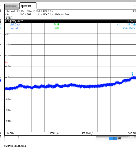
NTNV-N41-PC3-30-100-M-DFT-QPSK- Edge_1RB_Left-18000-26500-Ant1-PASS
