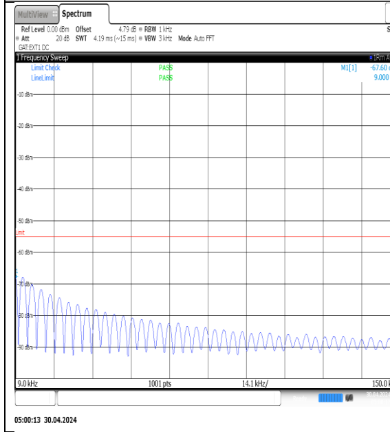
NTVN-N41-PC3-30-90-H-DFT-QPSK-Edge_1RB_Left-0.009-0.15-Ant1-PASS
