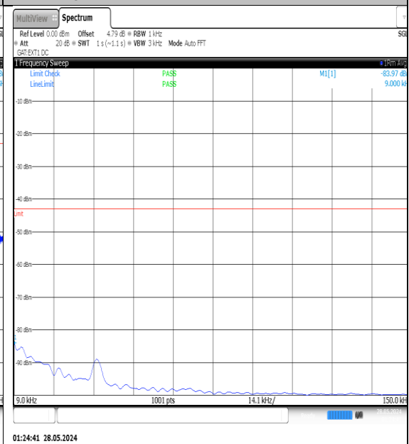
NTVN-N77-3450-3550-PC3-30-15-L-DFT-QPSK-Edge_1RB_Left-0.009-0.15-Ant1-PASS
