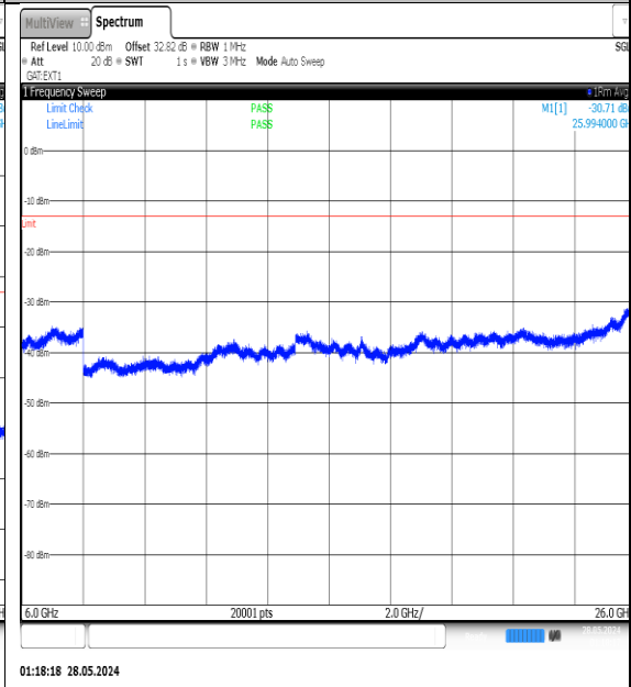
NTNV-N77-3450-3550-PC3-30-10-L-DFT-QPSK-Edge_1RB_Left-6000-26000-Ant1-PASS
