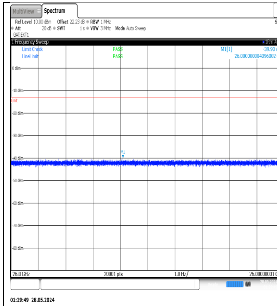
NTVN-N77-3450-3550-PC3-30-15-M-DFT-QPSK-Edge_1RB_Left-26000-40000-Ant1-PASS
