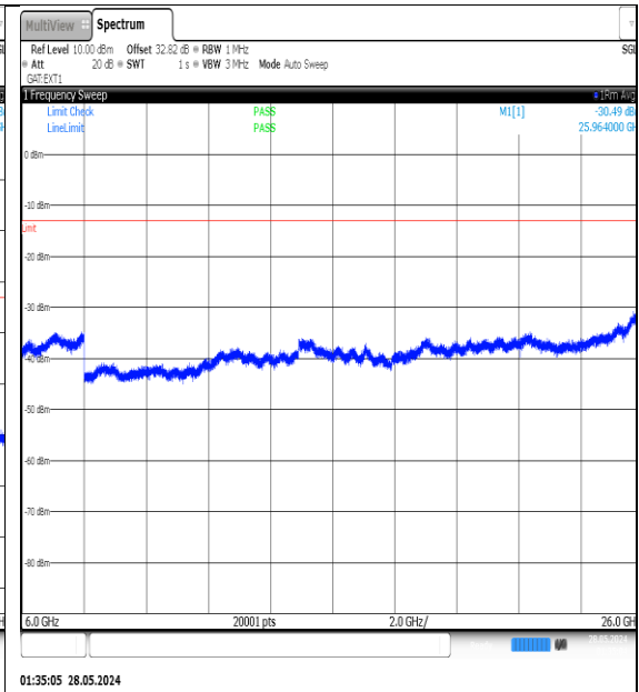
NTNV-N77-3450-3550-PC3-30-20-L-DFT-QPSK- Edge_1RB_Left-6000-26000-Ant1-PASS
