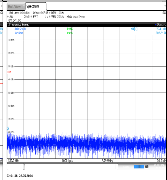
NTNV-N77-3450-3550-PC3-30-40-M-DFT-QPSK-Edge_1RB_Left-0.15-30-Ant1-PASS
