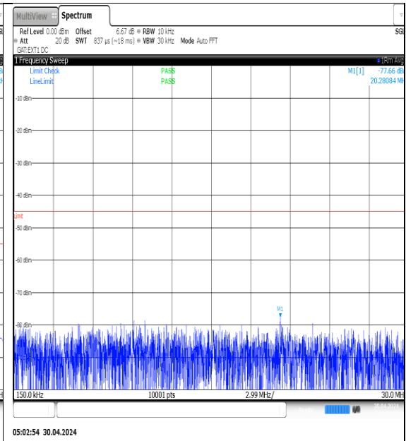
NTVN-N41-PC3-30-100-L-DFT-QPSK- Edge_1RB_Left-0.15-30-Ant1-PASS
