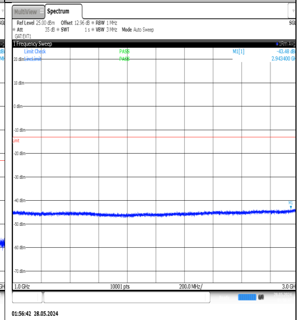
NTNV-N77-3450-3550-PC3-30-30-H-DFT-QPSK-Edge_1RB_Left-1000-3000-Ant1-PASS
