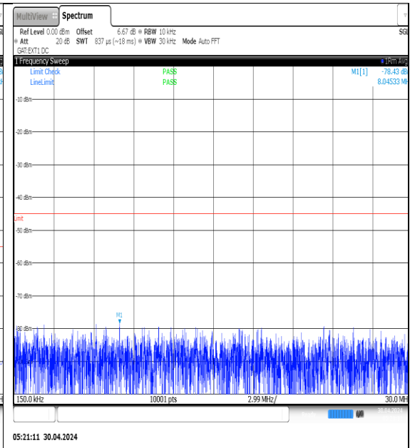
NTV-N41-PC3-30-100-H-DFT-QPSK- Edge_1RB_Left-0.15-30-Ant1-PASS
