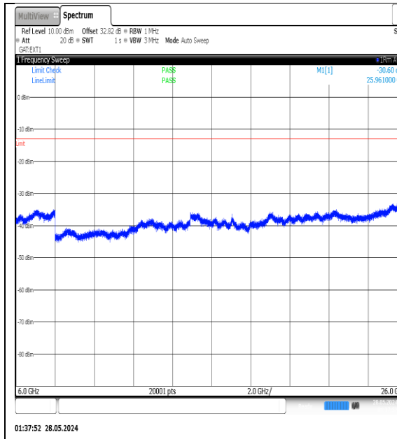
NTNV-N77-3450-3550-PC3-30-20-M-DFT-QPSK-Edge_1RB_Left-6000-26000-Ant1-PASS
