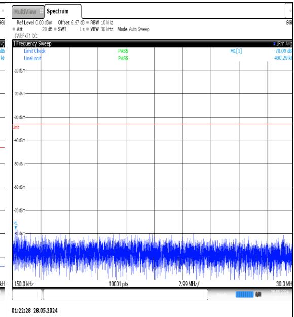
NTNV-N77-3450-3550-PC3-30-10-H-DFT-QPSK- Edge_1RB_Left-0.15-30-Ant1-PASS
