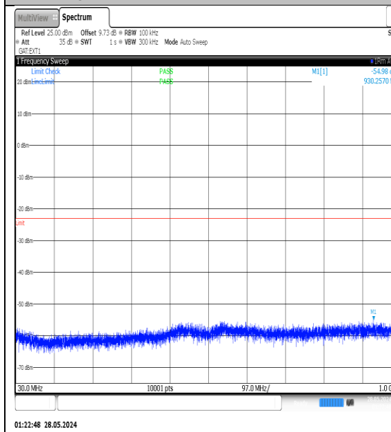
NTNV-N77-3450-3550-PC3-30-10-H-DFT-QPSK- Edge_1RB_Left-30-1000-Ant1-PASS
