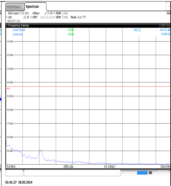
NTNV-N77-3450-3550-PC3-30-25-L-DFT-QPSK-Edge_1RB_Left-0.009-0.15-Ant1-PASS
