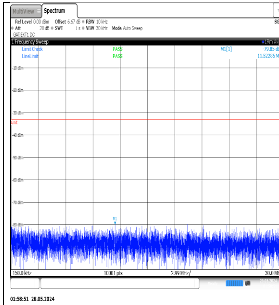
NTNV-N77-3450-3550-PC3-30-40-L-DFT-QPSK- Edge_1RB_Left-0.15-30-Ant1-PASS
