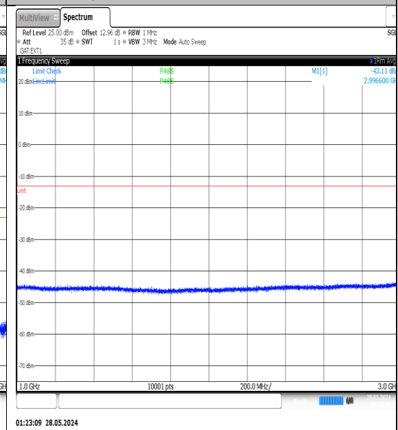
NTNV-N77-3450-3550-PC3-30-10-H-DFT-QPSK- Edge_1RB_Left-1000-3000-Ant1-PASS
