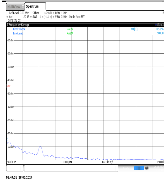
NTNV-N77-3450-3550-PC3-30-30-L-DFT-QPSK- Edge_1RB_Left-0.009-0.15-Ant1-PASS
