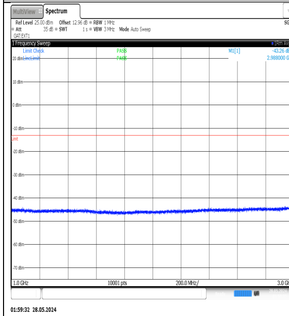
NTNV-N77-3450-3550-PC3-30-40-L-DFT-QPSK- Edge_1RB_Left-1000-3000-Ant1-PASS
