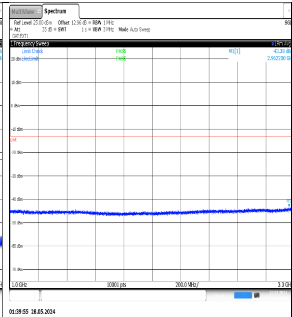
NTNV-N77-3450-3550-PC3-30-20-H-DFT-QPSK- Edge_1RB_Left-1000-3000-Ant1-PASS
