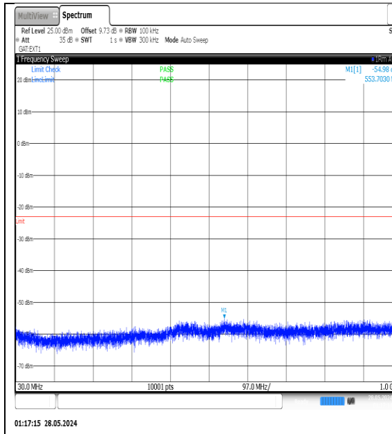
NTNV-N77-3450-3550-PC3-30-10-L-DFT-QPSK-Edge_1RB_Left-30-1000-Ant1-PASS
