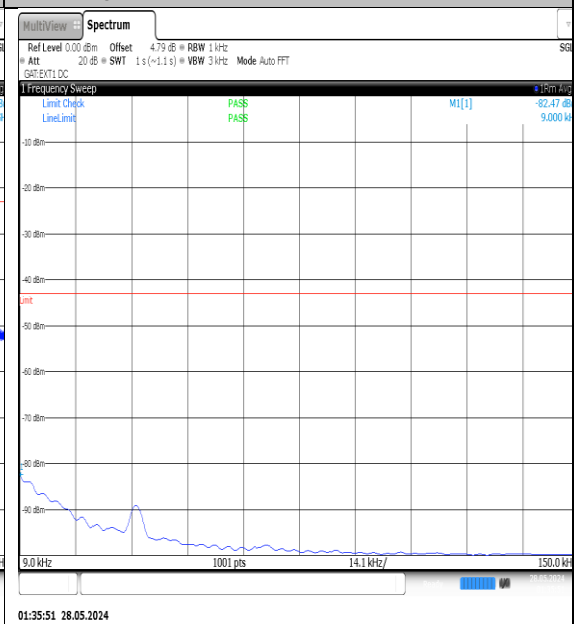
NTNV-N77-3450-3550-PC3-30-20-M-DFT-QPSK- Edge_1RB_Left-0.009-0.15-Ant1-PASS
