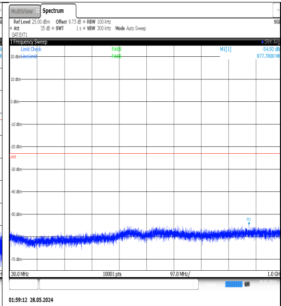
NTNV-N77-3450-3550-PC3-30-40-L-DFT-QPSK- Edge_1RB_Left-30-1000-Ant1-PASS
