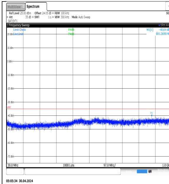
NTNV-N41-PC3-30-100-M-DFT-QPSK- Edge_1RB_Left-30-100-Ant1-PASS
