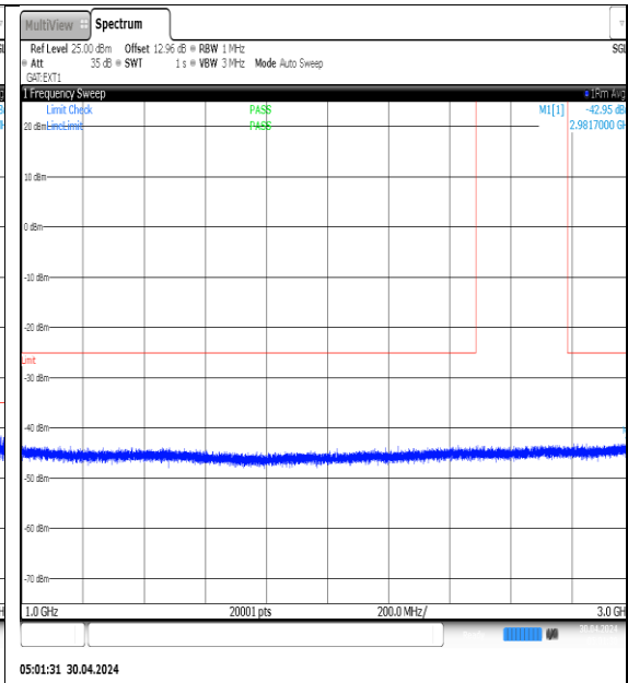
NTNV-N41-PC3-30-90-H-DFT-QPSK- Edge_1RB_Left-1000-3000-Ant1-PASS
