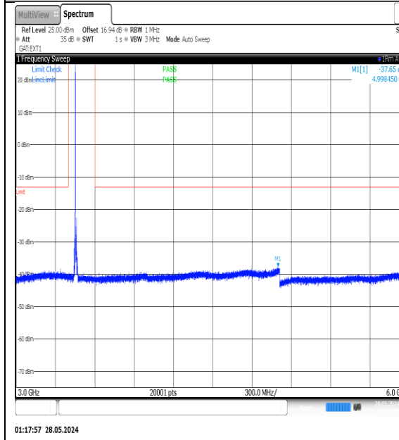
NTNV-N77-3450-3550-PC3-30-10-L-DFT-QPSK-Edge_1RB_Left-3000-6000-Ant1-PASS
