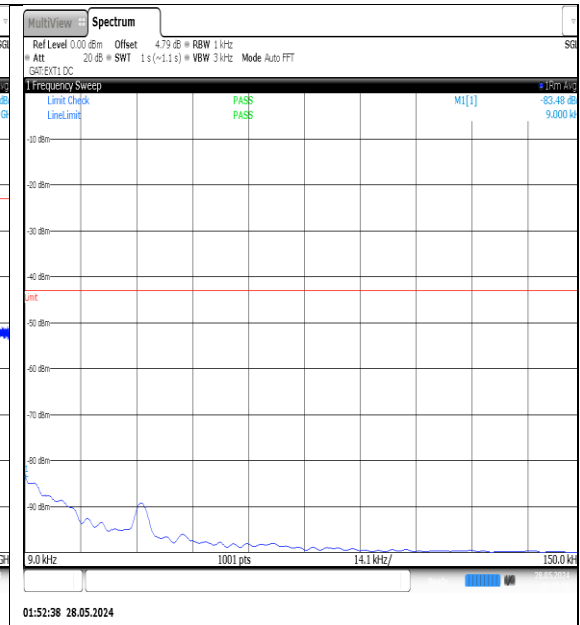
N77-3450-3550-PC3-30-30-M-DFT-QPSK- Edge_1RB_Left-0.009-0.15-Ant1-PASS
