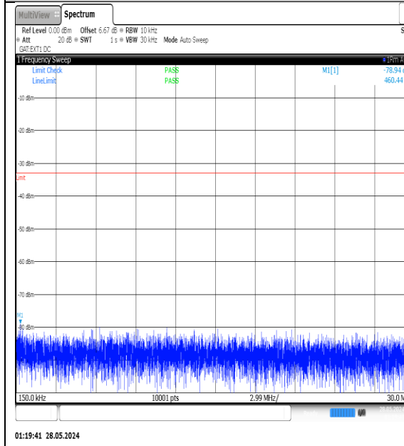
N77-3450-3550-PC3-30-10-M-DFT-QPSK- Edge_1RB_Left-0.15-30-Ant1-PASS
