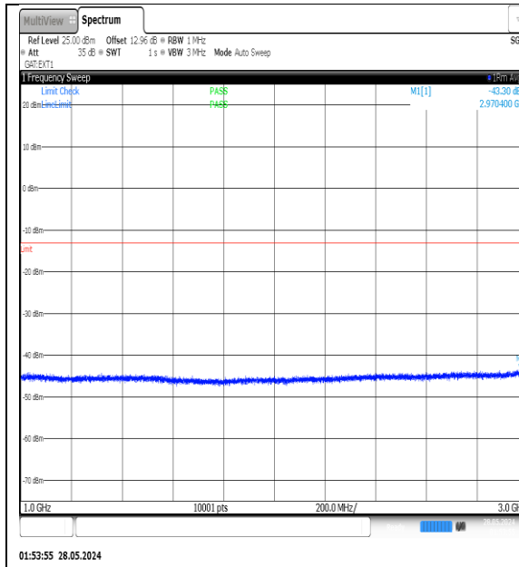
NTNV-N77-3450-3550-PC3-30-30-M-DFT-QPSK-Edge_1RB_Left-1000-3000-Ant1-PASS
