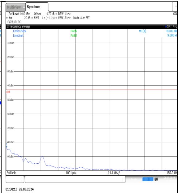
NTVN-N77-3450-3550-PC3-30-15-H-DFT-QPSK-Edge_1RB_Left-0.009-0.15-Ant1-PASS
