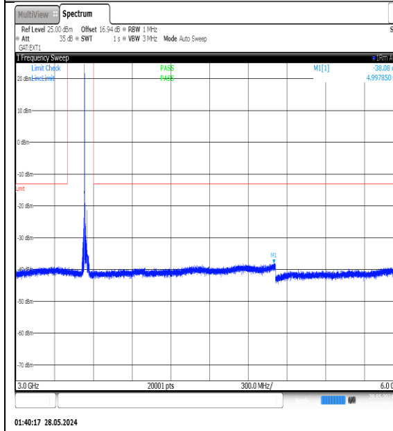
NTNV-N77-3450-3550-PC3-30-20-H-DFT-QPSK- Edge_1RB_Left-3000-6000-Ant1-PASS
