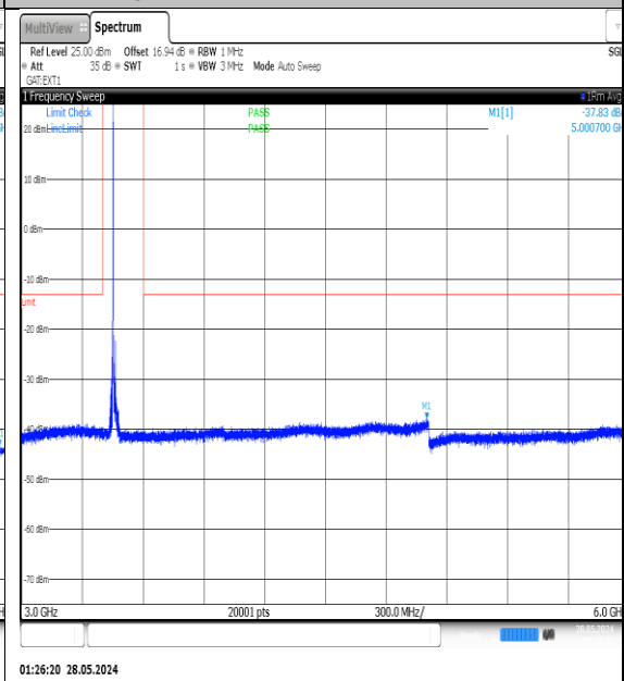
NTNV-N77-3450-3550-PC3-30-15-L-DFT-QPSK- Edge_1RB_Left-3000-6000-Ant1-PASS
