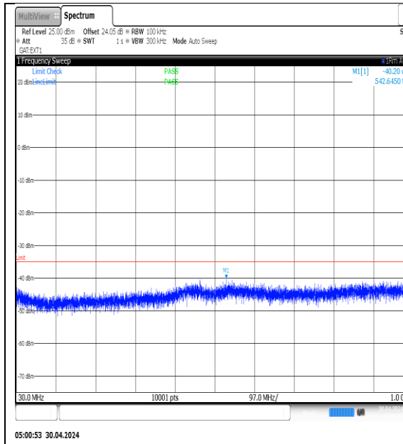
NTNV-N41-PC3-30-90-H-DFT-QPSK- Edge_1RB_Left-30-1000-Ant1-PASS
