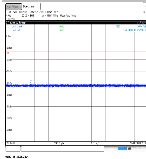
NTVN-N77-3450-3550-PC3-30-30-H-DFT-QPSK-Edge_1RB_Left-26000-40000-Ant1-PASS
