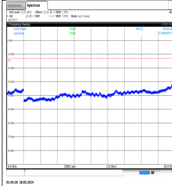
NTNV-N77-3450-3550-PC3-30-25-L-DFT-QPSK- Edge_1RB_Left-6000-26000-Ant1-PASS
