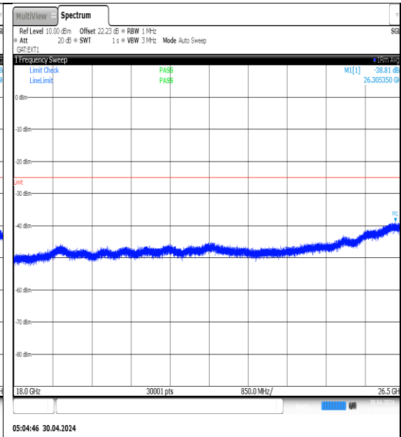
NTVN-N41-PC3-30-100-L-DFT-QPSK- Edge_1RB_Left-18000-26500-Ant1-PASS
