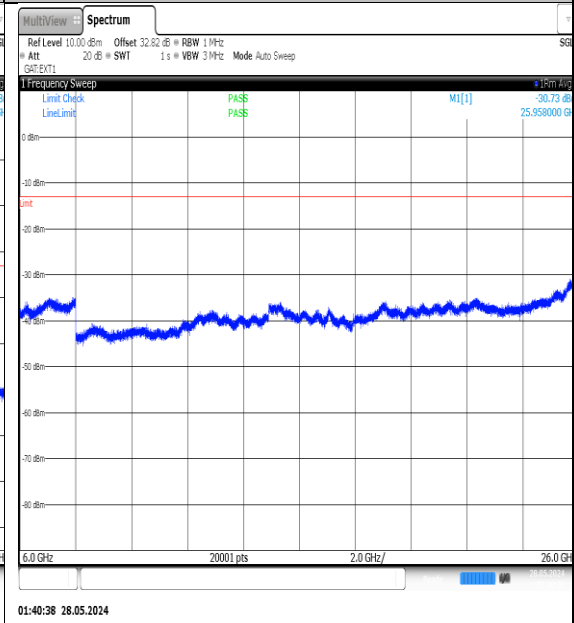
NTNV-N77-3450-3550-PC3-30-20-H-DFT-QPSK- Edge_1RB_Left-6000-26000-Ant1-PASS
