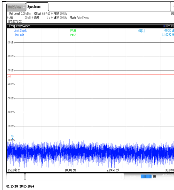
NTNV-N77-3450-3550-PC3-30-15-L-DFT-QPSK- Edge_1RB_Left-0.15-30-Ant1-PASS
