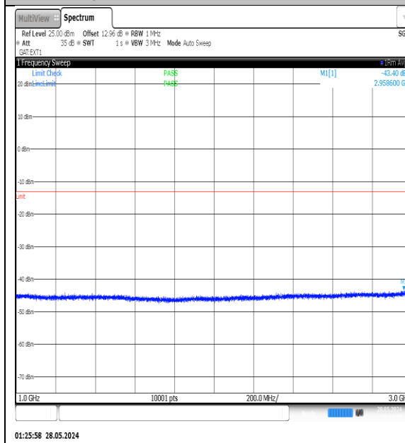
NTNV-N77-3450-3550-PC3-30-15-L-DFT-QPSK- Edge_1RB_Left-1000-3000-Ant1-PASS
