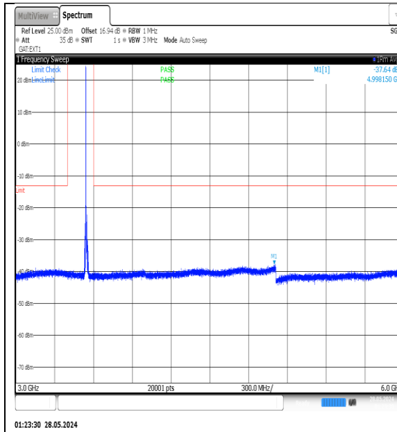
NTVN-N77-3450-3550-PC3-30-10-H-DFT-QPSK-Edge_1RB_Left-3000-6000-Ant1-PASS
