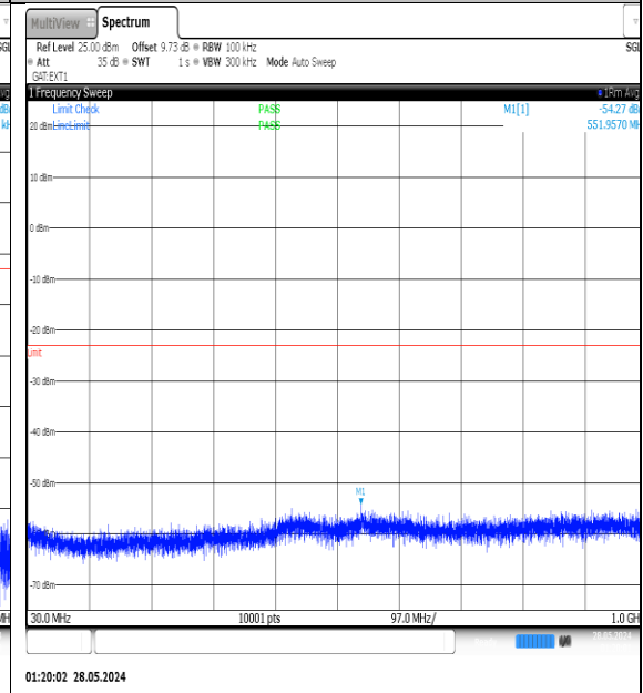
N77-3450-3550-PC3-30-10-M-DFT-QPSK- Edge_1RB_Left-30-1000-Ant1-PASS
