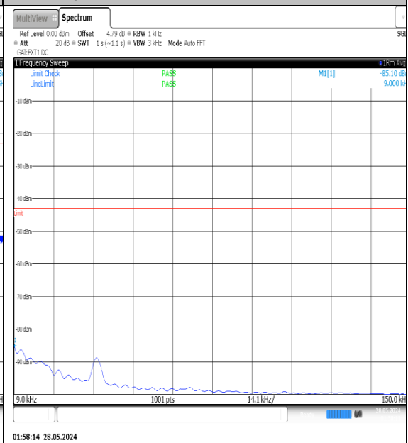
NTVN-N77-3450-3550-PC3-30-40-L-DFT-QPSK-Edge_1RB_Left-0.009-0.15-Ant1-PASS
