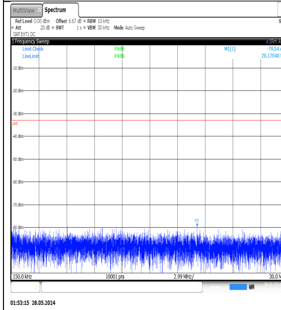
N77-3450-3550-PC3-30-30-M-DFT-QPSK- Edge_1RB_Left-0.15-30-Ant1-PASS
