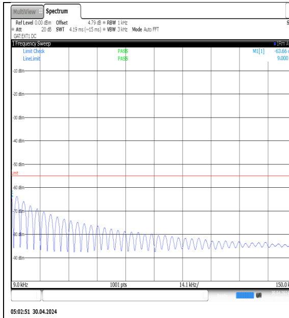
NTVN-N41-PC3-30-100-L-DFT-QPSK- Edge_1RB_Left-0.009-0.15-Ant1-PASS
