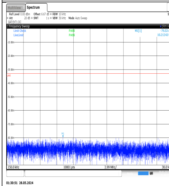
NTVN-N77-3450-3550-PC3-30-15-H-DFT-QPSK-Edge_1RB_Left-0.15-30-Ant1-PASS
