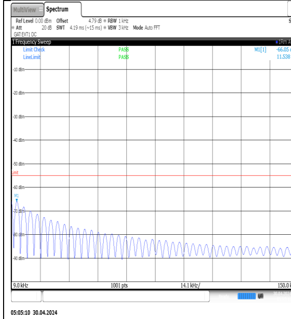
NTVN-N41-PC3-30-100-M-DFT-QPSK- Edge_1RB_Left-0.009-0.15-Ant1-PASS
