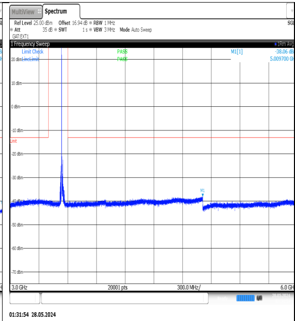
NTNV-N77-3450-3550-PC3-30-15-H-DFT-QPSK-Edge_1RB_Left-3000-6000-Ant1-PASS
