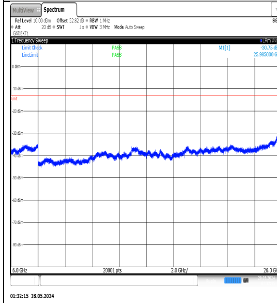
NTNV-N77-3450-3550-PC3-30-15-H-DFT-QPSK-Edge_1RB_Left-6000-26000-Ant1-PASS
