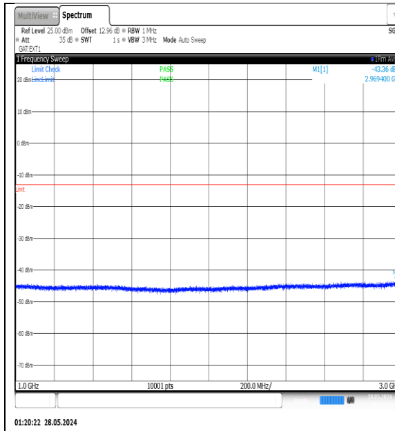
NTNV-N77-3450-3550-PC3-30-10-M-DFT-QPSK-Edge_1RB_Left-1000-3000-Ant1-PASS
