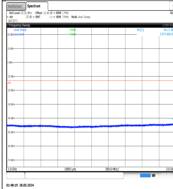
NTNV-N77-3450-3550-PC3-30-25-H-DFT-QPSK- Edge_1RB_Left-1000-3000-Ant1-PASS
