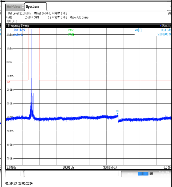
NTNV-N77-3450-3550-PC3-30-40-L-DFT-QPSK- Edge_1RB_Left-3000-6000-Ant1-PASS
