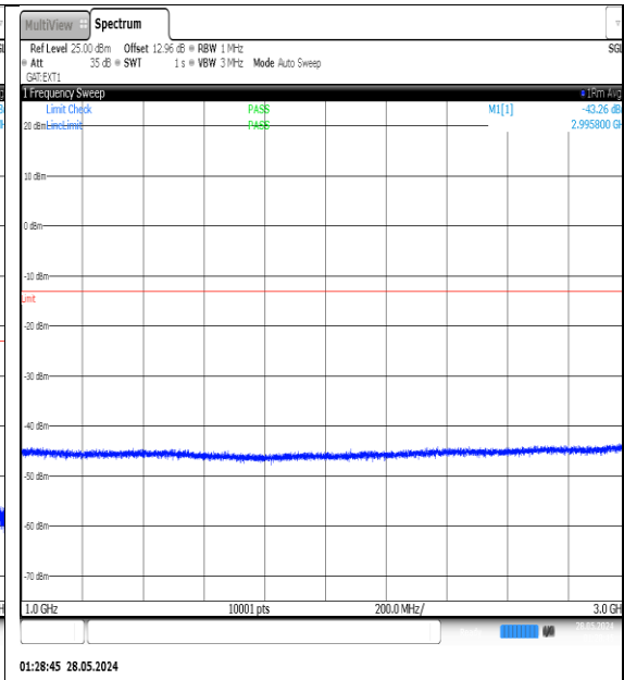
NTNV-N77-3450-3550-PC3-30-15-M-DFT-QPSK-Edge_1RB_Left-1000-3000-Ant1-PASS
