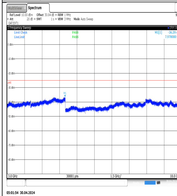
NTNV-N41-PC3-30-90-H-DFT-QPSK- Edge_1RB_Left-3000-18000-Ant1-PASS
