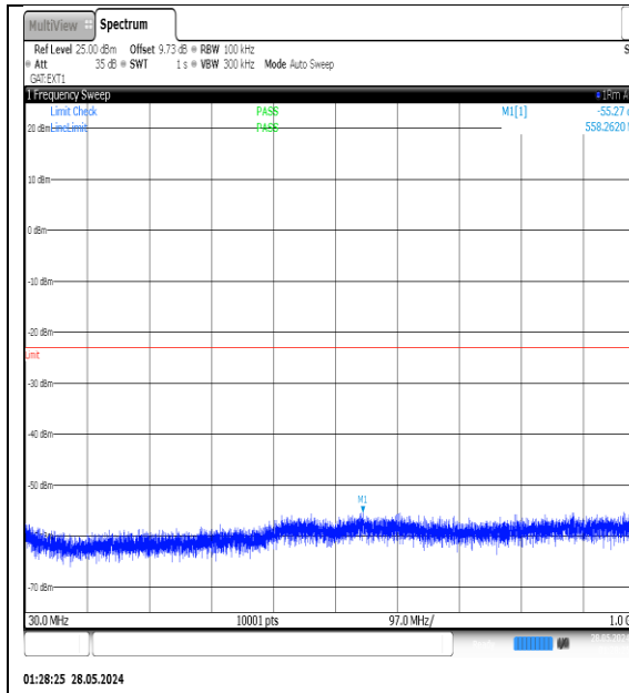
NTNV-N77-3450-3550-PC3-30-15-M-DFT-QPSK-Edge_1RB_Left-30-1000-Ant1-PASS
