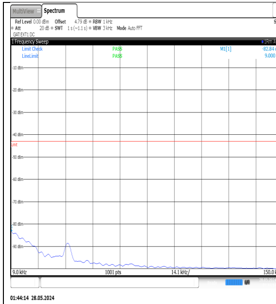
NTVN-N77-3450-3550-PC3-30-25-M-DFT-QPSK-Edge_1RB_Left-0.009-0.15-Ant1-PASS
