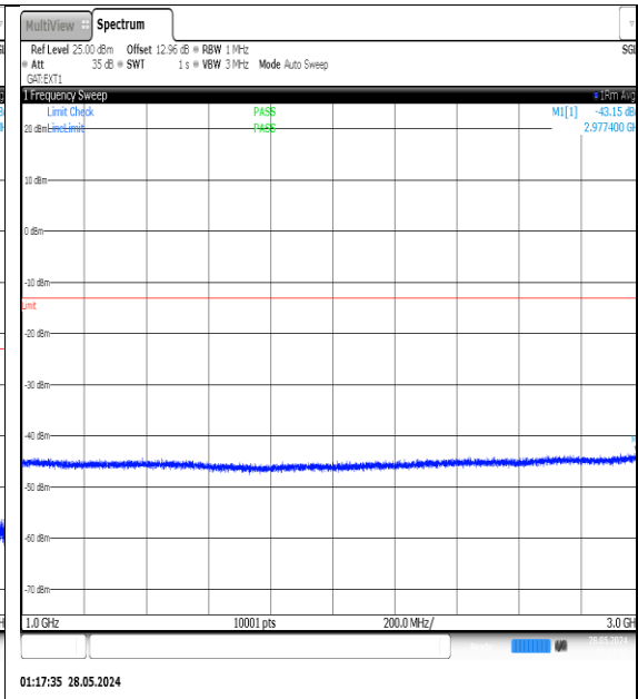
NTNV-N77-3450-3550-PC3-30-10-L-DFT-QPSK-Edge_1RB_Left-1000-3000-Ant1-PASS
