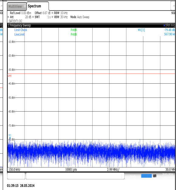
NTNV-N77-3450-3550-PC3-30-20-H-DFT-QPSK-Edge_1RB_Left-0.15-30-Ant1-PASS
