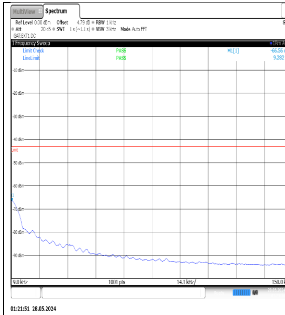
NTNV-N77-3450-3550-PC3-30-10-H-DFT-QPSK- Edge_1RB_Left-0.009-0.15-Ant1-PASS
