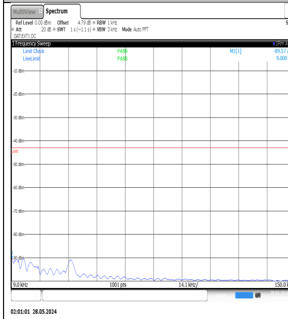
NTNV-N77-3450-3550-PC3-30-40-M-DFT-QPSK-Edge_1RB_Left-0.009-0.15-Ant1-PASS
