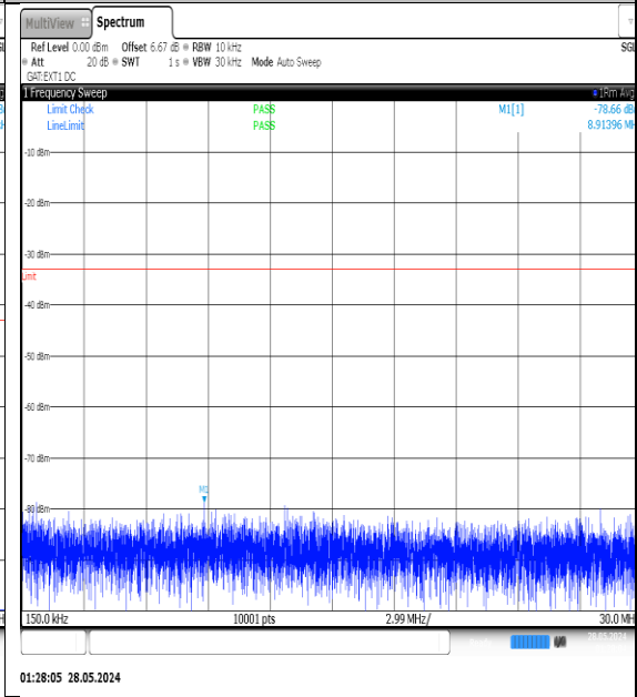
NTNV-N77-3450-3550-PC3-30-15-M-DFT-QPSK-Edge_1RB_Left-0.15-30-Ant1-PASS
