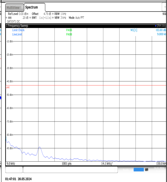
NTNV-N77-3450-3550-PC3-30-25-H-DFT-QPSK- Edge_1RB_Left-0.009-0.15-Ant1-PASS
