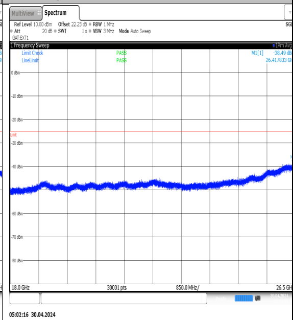
NTNV-N41-PC3-30-90-H-DFT-QPSK- Edge_1RB_Left-18000-26500-Ant1-PASS
