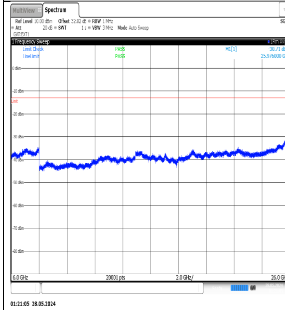
NTNV-N77-3450-3550-PC3-30-10-M-DFT-QPSK-Edge_1RB_Left-6000-26000-Ant1-PASS
