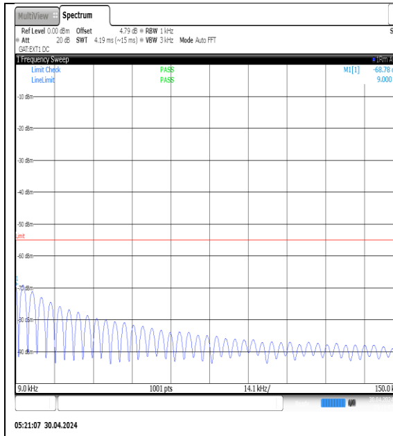
NTV-N41-PC3-30-100-H-DFT-QPSK- Edge_1RB_Left-0.009-0.15-Ant1-PASS
