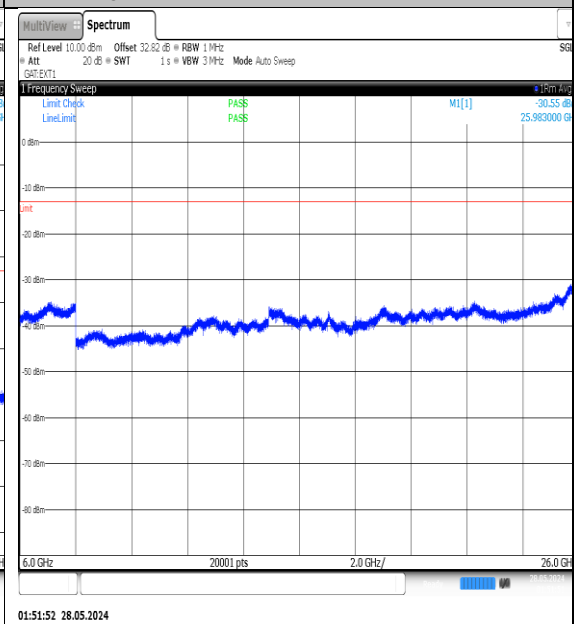
NTNV-N77-3450-3550-PC3-30-30-L-DFT-QPSK- Edge_1RB_Left-6000-26000-Ant1-PASS
