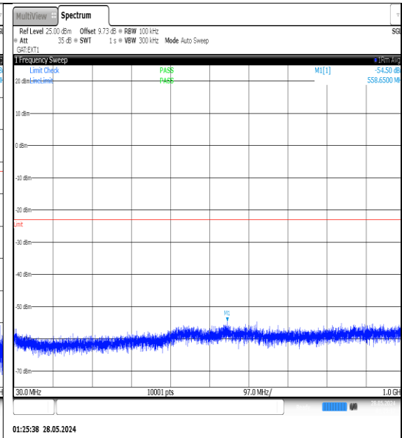
NTNV-N77-3450-3550-PC3-30-15-L-DFT-QPSK- Edge_1RB_Left-30-1000-Ant1-PASS
