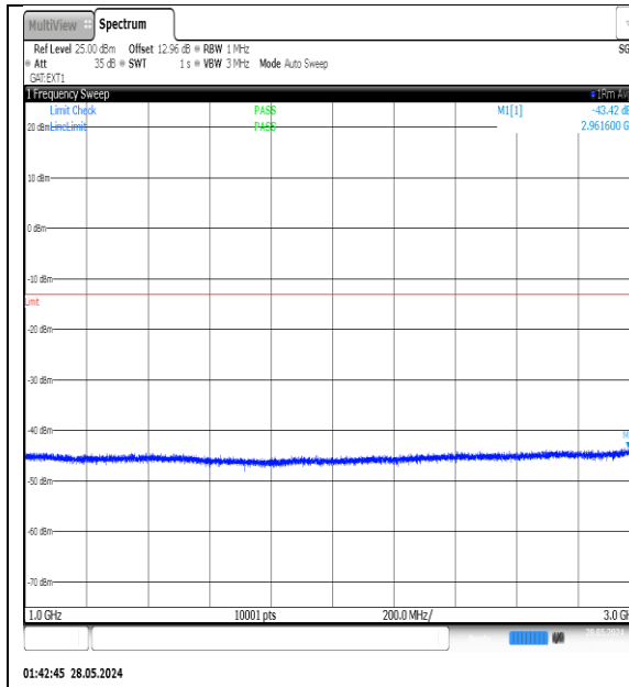
NTNV-N77-3450-3550-PC3-30-25-L-DFT-QPSK- Edge_1RB_Left-1000-3000-Ant1-PASS
