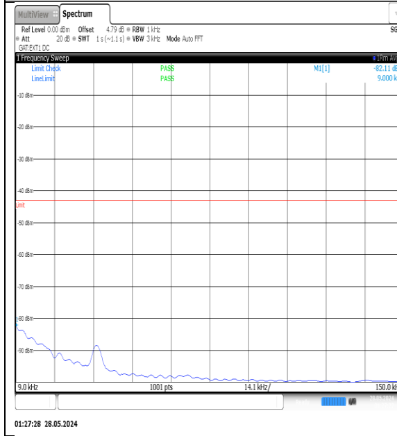
NTNV-N77-3450-3550-PC3-30-15-M-DFT-QPSK-Edge_1RB_Left-0.009-0.15-Ant1-PASS
