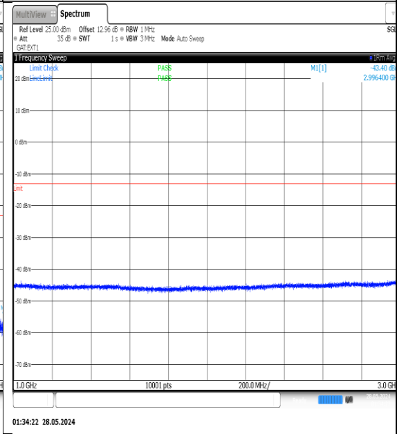
NTNV-N77-3450-3550-PC3-30-20-L-DFT-QPSK- Edge_1RB_Left-1000-3000-Ant1-PASS
