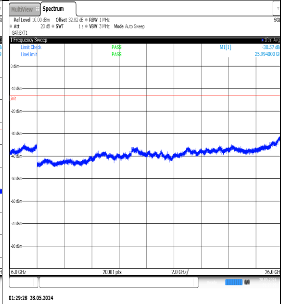
NTNV-N77-3450-3550-PC3-30-15-M-DFT-QPSK-Edge_1RB_Left-6000-26000-Ant1-PASS
