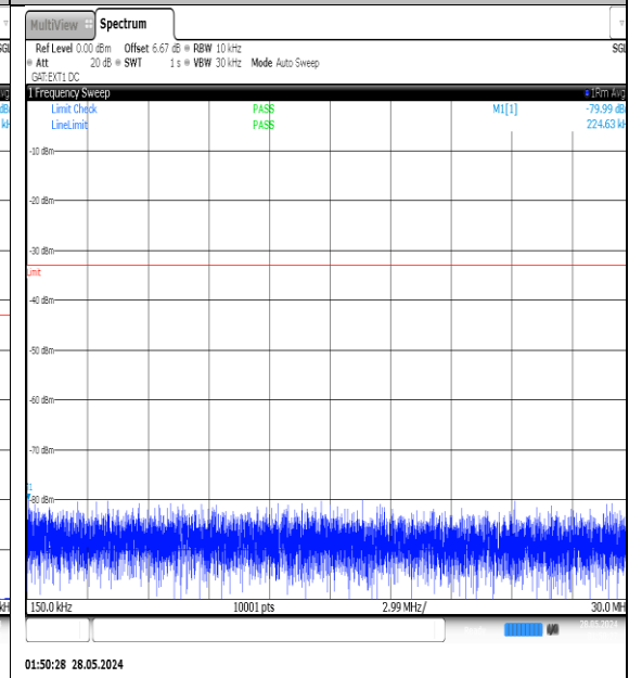
NTNV-N77-3450-3550-PC3-30-30-L-DFT-QPSK- Edge_1RB_Left-0.15-30-Ant1-PASS
