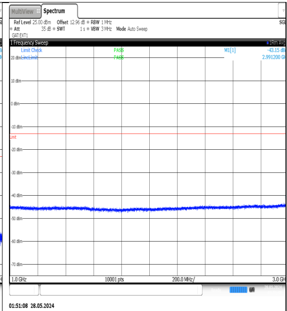
NTNV-N77-3450-3550-PC3-30-30-L-DFT-QPSK- Edge_1RB_Left-1000-3000-Ant1-PASS
