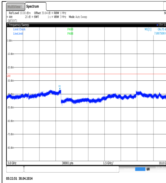
NTV-N41-PC3-30-100-H-DFT-QPSK- Edge_1RB_Left-3000-18000-Ant1-PASS
