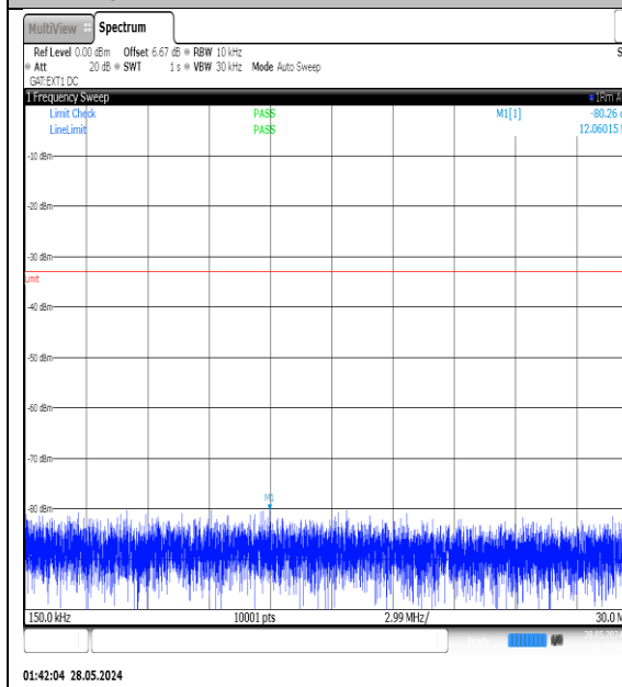
NTNV-N77-3450-3550-PC3-30-25-L-DFT-QPSK-Edge_1RB_Left-0.15-30-Ant1-PASS
