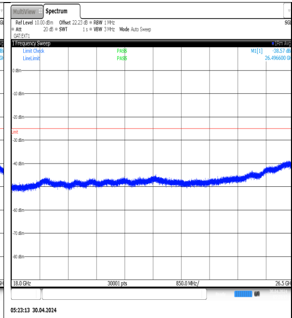
NTV-N41-PC3-30-100-H-DFT-QPSK- Edge_1RB_Left-18000-26500-Ant1-PASS
