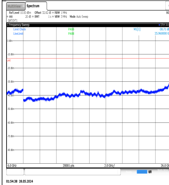
NTNV-N77-3450-3550-PC3-30-30-M-DFT-QPSK-Edge_1RB_Left-6000-26000-Ant1-PASS
