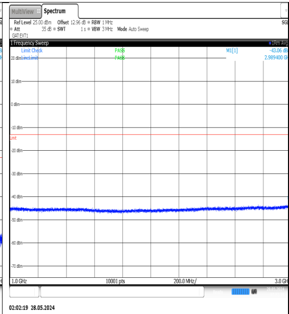
NTNV-N77-3450-3550-PC3-30-40-M-DFT-QPSK-Edge_1RB_Left-1000-3000-Ant1-PASS
