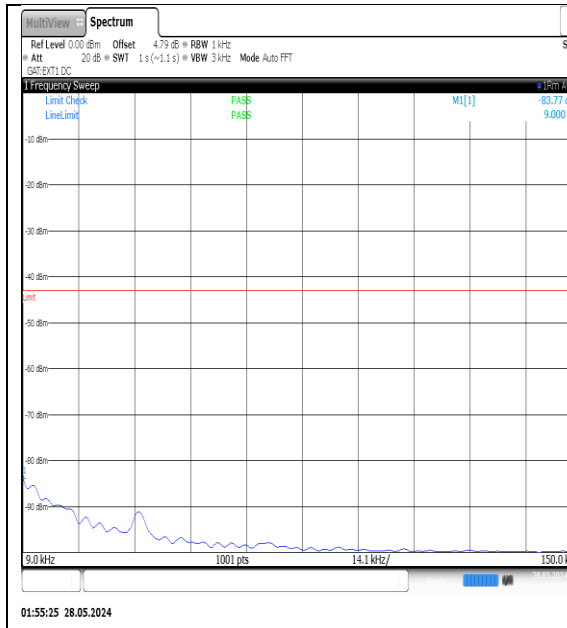
NTNV-N77-3450-3550-PC3-30-30-H-DFT-QPSK-Edge_1RB_Left-0.009-0.15-Ant1-PASS
