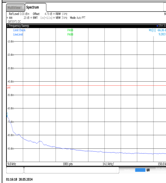
NTV-N77-3450-3550-PC3-30-10-L-DFT-QPSK- Edge_1RB_Left-0.009-0.15-Ant1-PASS
