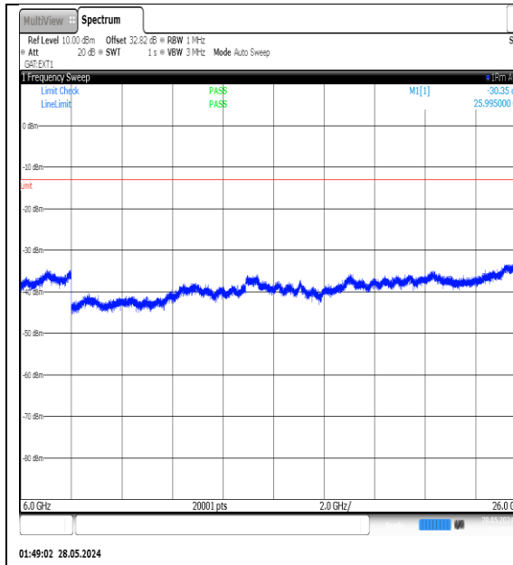
NTNV-N77-3450-3550-PC3-30-25-H-DFT-QPSK- Edge_1RB_Left-6000-26000-Ant1-PASS
