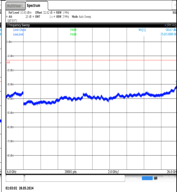
NTNV-N77-3450-3550-PC3-30-40-M-DFT-QPSK-Edge_1RB_Left-6000-26000-Ant1-PASS
