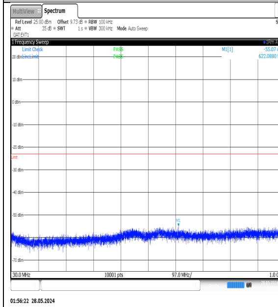
NTNV-N77-3450-3550-PC3-30-30-H-DFT-QPSK-Edge_1RB_Left-30-1000-Ant1-PASS
