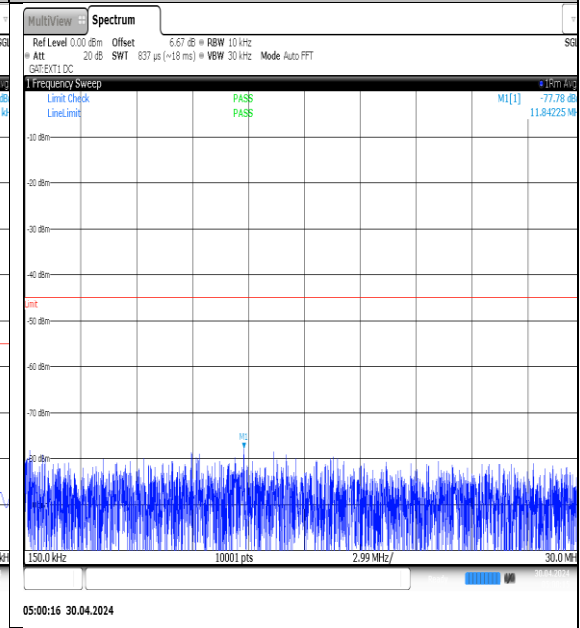
NTVN-N41-PC3-30-90-H-DFT-QPSK-Edge_1RB_Left-0.15-30-Ant1-PASS
