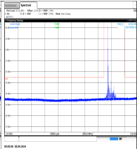
NTNV-N41-PC3-30-100-M-DFT-QPSK- Edge_1RB_Left-1000-3000-Ant1-PASS
