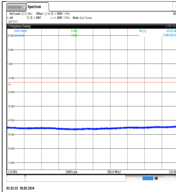
NTNV-N77-3450-3550-PC3-30-15-H-DFT-QPSK-Edge_1RB_Left-1000-3000-Ant1-PASS
