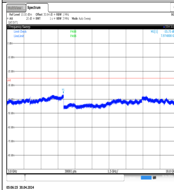
NTNV-N41-PC3-30-100-M-DFT-QPSK- Edge_1RB_Left-3000-18000-Ant1-PASS
