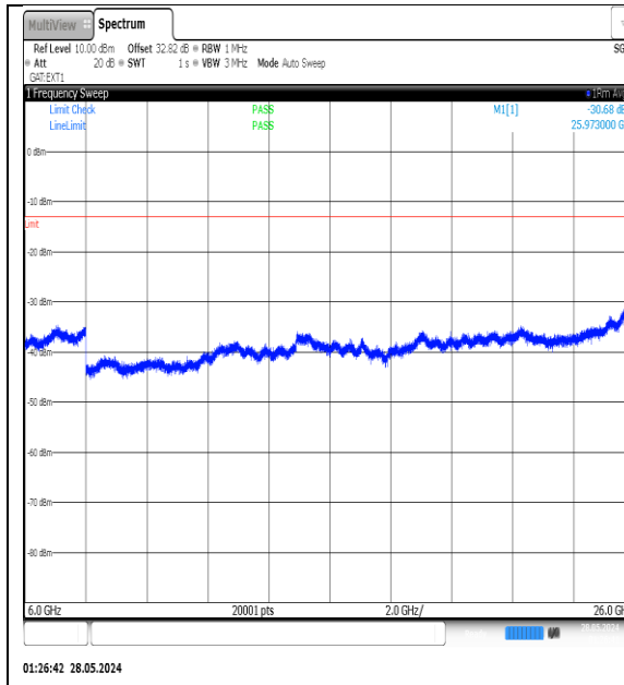
NTNV-N77-3450-3550-PC3-30-15-L-DFT-QPSK-Edge_1RB_Left-6000-26000-Ant1-PASS
