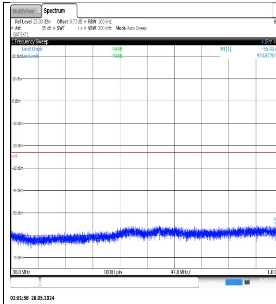
NTNV-N77-3450-3550-PC3-30-40-M-DFT-QPSK-Edge_1RB_Left-30-1000-Ant1-PASS
