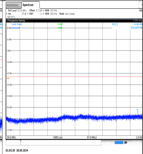
N77-3450-3550-PC3-30-30-M-DFT-QPSK- Edge_1RB_Left-30-1000-Ant1-PASS
