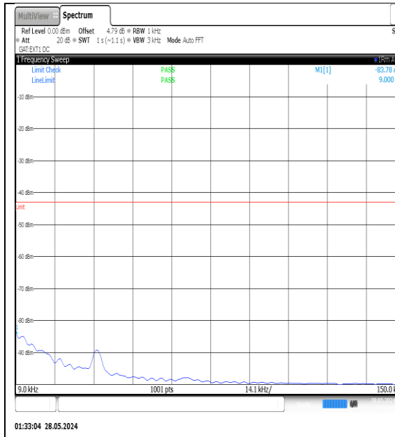
NTNV-N77-3450-3550-PC3-30-20-L-DFT-QPSK- Edge_1RB_Left-0.009-0.15-Ant1-PASS
