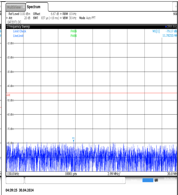
NTVN-N41-PC3-30-80-H-DFT-QPSK- Edge_1RB_Left-0.15-30-Ant1-PASS
