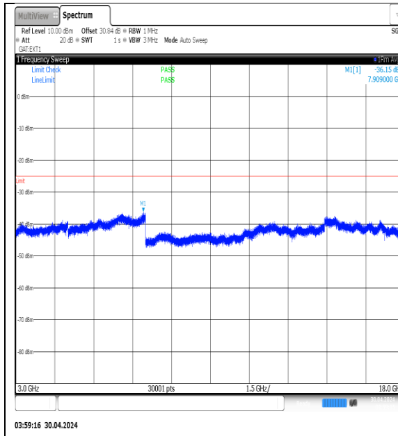
NTVN-N41-PC3-30-60-H-DFT-QPSK-Edge_1RB_Left-3000-18000-Ant1-PASS
