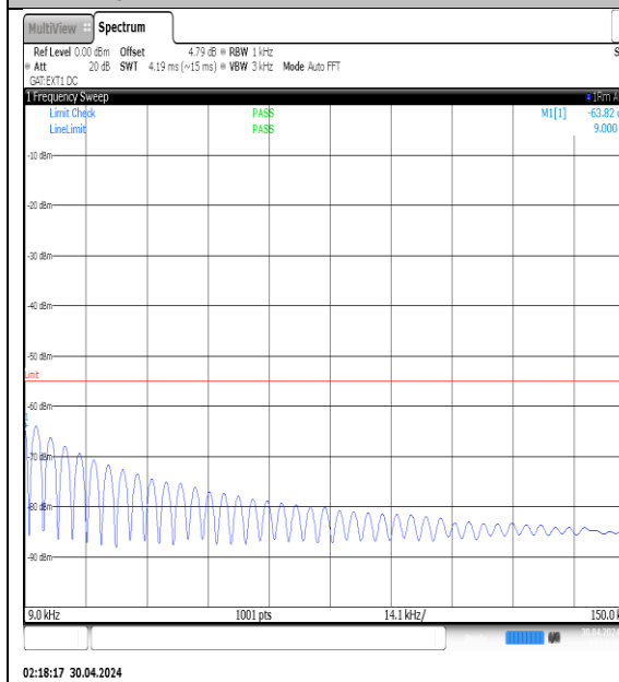
NTVN-N41-PC3-30-20-M-DFT-QPSK- Edge_1RB_Left-0.009-0.15-Ant1-PASS
