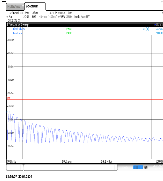
NTVN-N41-PC3-30-30-M-DFT-QPSK-Edge_1RB_Left-0.009-0.15-Ant1-PASS
