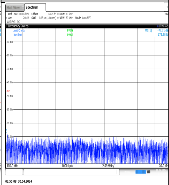
NTVN-N41-PC3-30-30-H-DFT-QPSK- Edge_1RB_Left-0.15-30-Ant1-PASS
