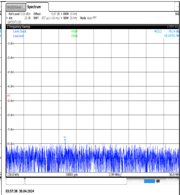
NTVN-N41-PC3-30-60-H-DFT-QPSK- Edge_1RB_Left-0.15-30-Ant1-PASS
