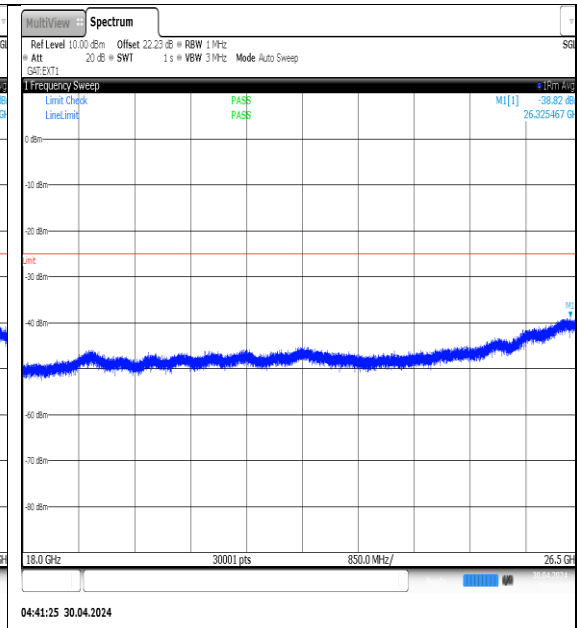
NTVN-N41-PC3-30-80-H-DFT-QPSK-Edge_1RB_Left-18000-26500-Ant1-PASS
