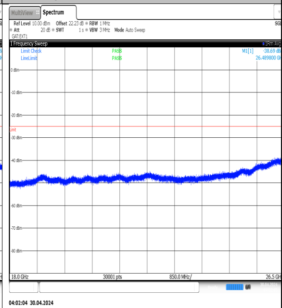
NTNV-N41-PC3-30-70-L-DFT-QPSK- Edge_1RB_Left-18000-26500-Ant1-PASS
