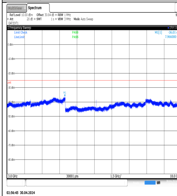
NTNV-N41-PC3-30-30-H-DFT-QPSK- Edge_1RB_Left-3000-18000-Ant1-PASS
