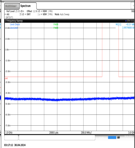
NTVN-N41-PC3-30-40-H-DFT-QPSK-Edge_1RB_Left-1000-3000-Ant1-PASS
