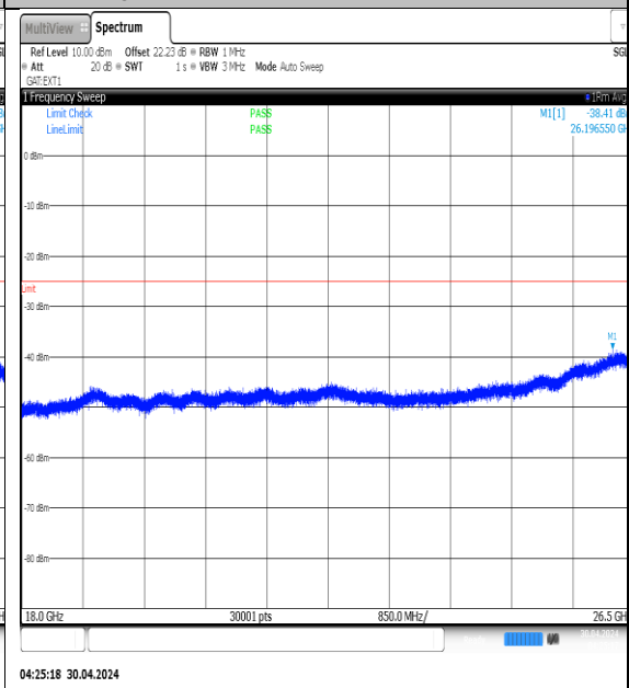
NTNV-N41-PC3-30-80-M-DFT-QPSK- Edge_1RB_Left-18000-26500-Ant1-PASS
