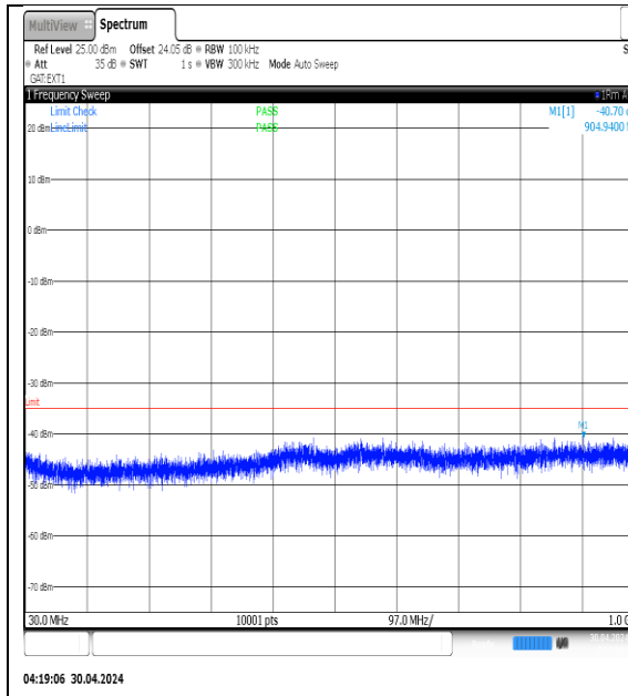
NTNV-N41-PC3-30-70-H-DFT-QPSK- Edge_1RB_Left-30-1000-Ant1-PASS
