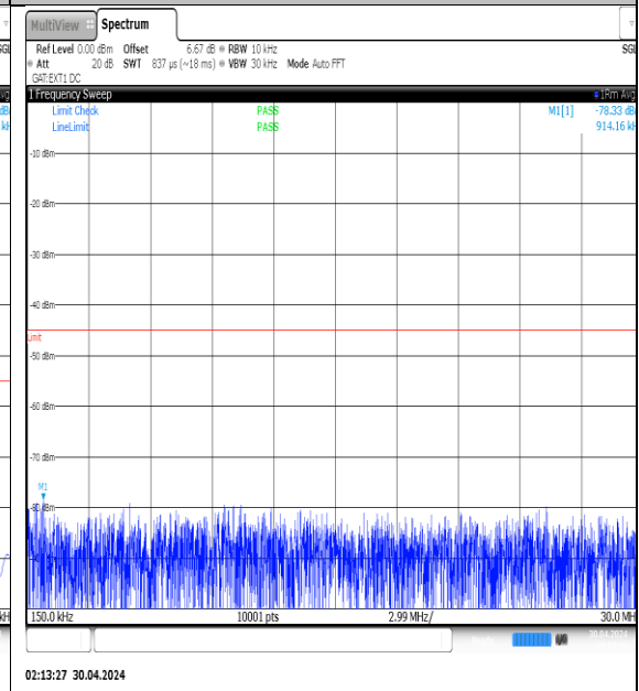
NTVN-N41-PC3-30-15-H-DFT-QPSK-Edge_1RB_Left-0.15-30-Ant1-PASS
