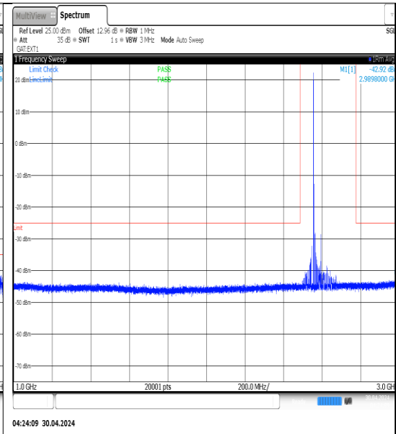
NTNV-N41-PC3-30-80-M-DFT-QPSK- Edge_1RB_Left-1000-3000-Ant1-PASS
