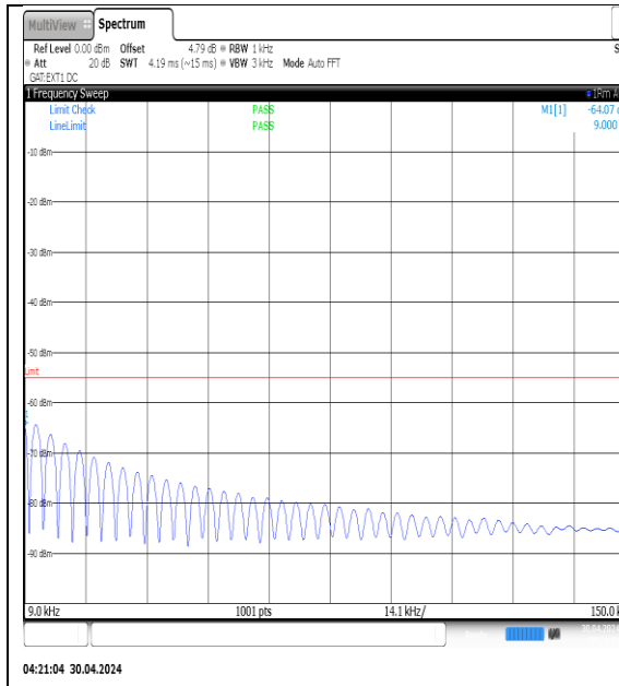
NTVN-N41-PC3-30-80-L-DFT-QPSK- Edge_1RB_Left-0.009-0.15-Ant1-PASS
