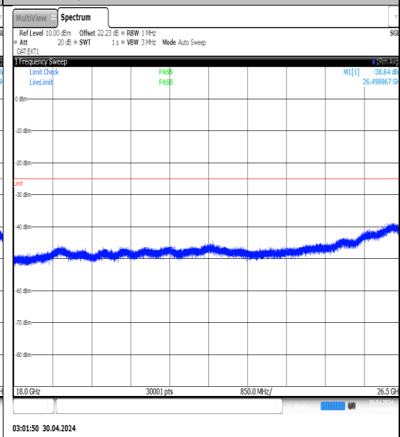
NTNV-N41-PC3-30-40-M-DFT-QPSK- Edge_1RB_Left-18000-26500-Ant1-PASS
