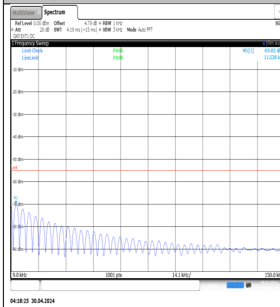
NTVN-N41-PC3-30-70-H-DFT-QPSK-Edge_1RB_Left-0.009-0.15-Ant1-PASS
