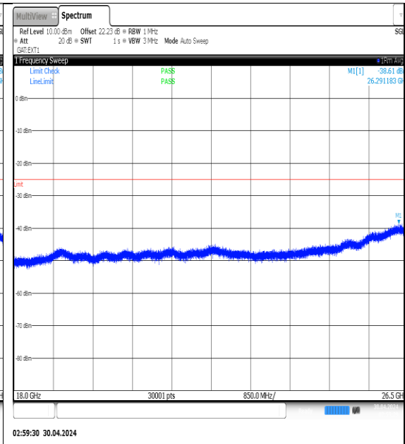
NTVN-N41-PC3-30-40-L-DFT-QPSK- Edge_1RB_Left-18000-26500-Ant1-PASS
