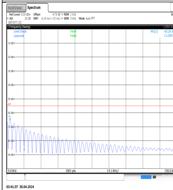
NTVN-N41-PC3-30-60-M-DFT-QPSK-Edge_1RB_Left-0.009-0.15-Ant1-PASS
