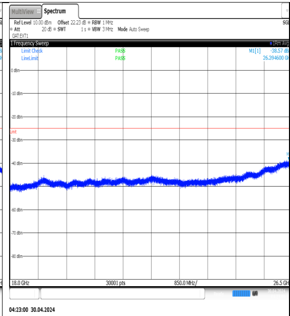
NTVN-N41-PC3-30-80-L-DFT-QPSK- Edge_1RB_Left-18000-26500-Ant1-PASS
