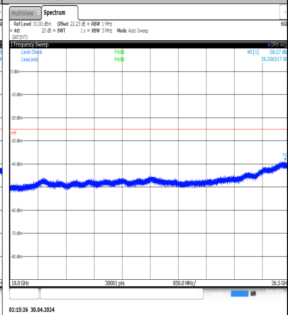
NTNV-N41-PC3-30-15-H-DFT-QPSK- Edge_1RB_Left-18000-26500-Ant1-PASS
