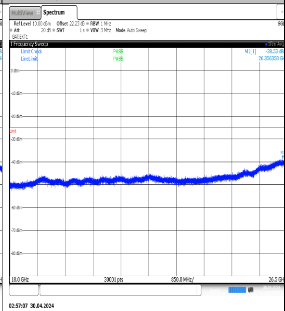
NTNV-N41-PC3-30-30-H-DFT-QPSK- Edge_1RB_Left-18000-26500-Ant1-PASS
