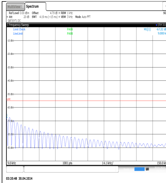
NTVN-N41-PC3-30-50-M-DFT-QPSK- Edge_1RB_Left-0.009-0.15-Ant1-PASS
