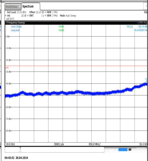
NTVN-N41-PC3-30-90-L-DFT-QPSK-Edge_1RB_Left-18000-26500-Ant1-PASS
