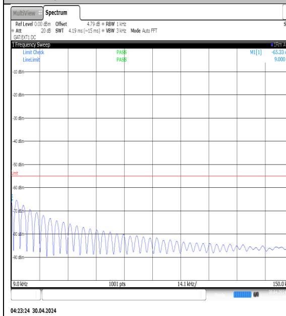
NTVN-N41-PC3-30-80-M-DFT-QPSK- Edge_1RB_Left-0.009-0.15-Ant1-PASS
