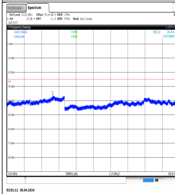
NTNV-N41-PC3-30-40-M-DFT-QPSK- Edge_1RB_Left-3000-18000-Ant1-PASS
