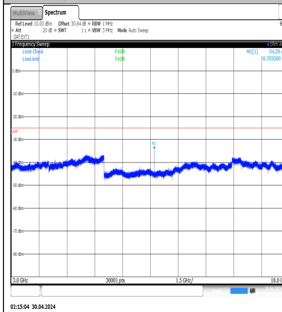
NTNV-N41-PC3-30-15-H-DFT-QPSK- Edge_1RB_Left-3000-18000-Ant1-PASS
