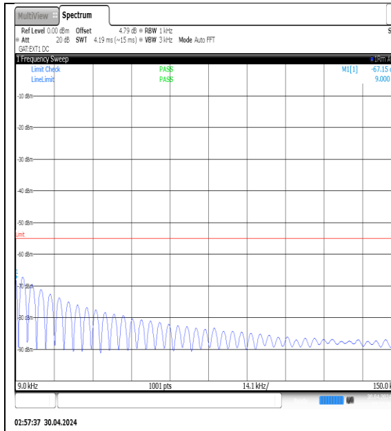
NTVN-N41-PC3-30-40-L-DFT-QPSK-Edge_1RB_Left-0.009-0.15-Ant1-PASS
