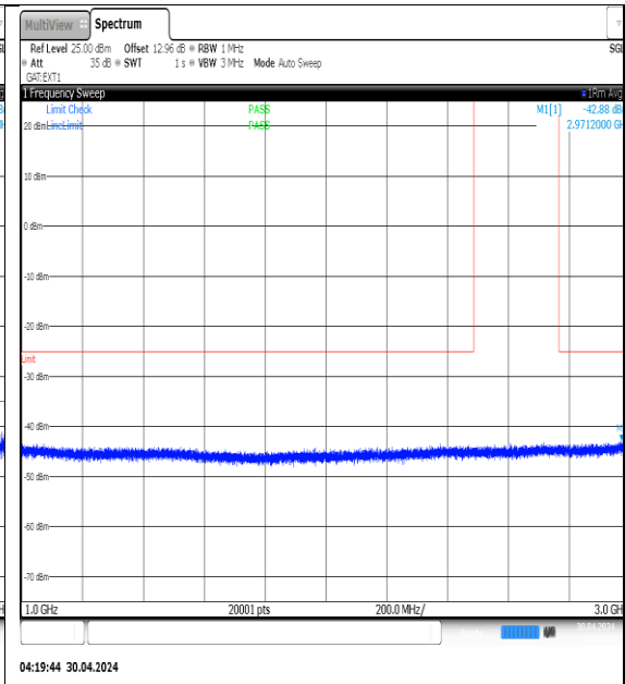
NTNV-N41-PC3-30-70-H-DFT-QPSK- Edge_1RB_Left-1000-3000-Ant1-PASS
