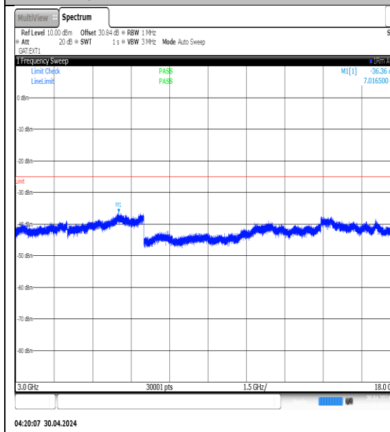
NTNV-N41-PC3-30-70-H-DFT-QPSK- Edge_1RB_Left-3000-18000-Ant1-PASS
