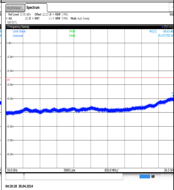
NTNV-N41-PC3-30-70-H-DFT-QPSK- Edge_1RB_Left-18000-26500-Ant1-PASS
