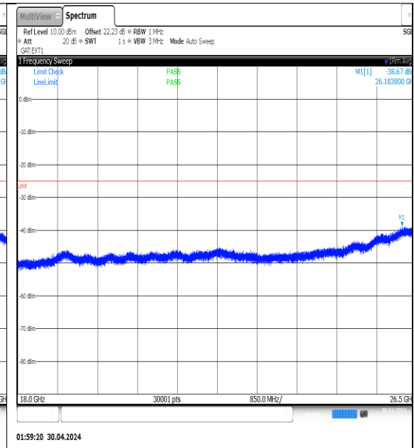
NTVN-N41-PC3-30-15-M-DFT-QPSK-Edge_1RB_Left-18000-26500-Ant1-PASS
