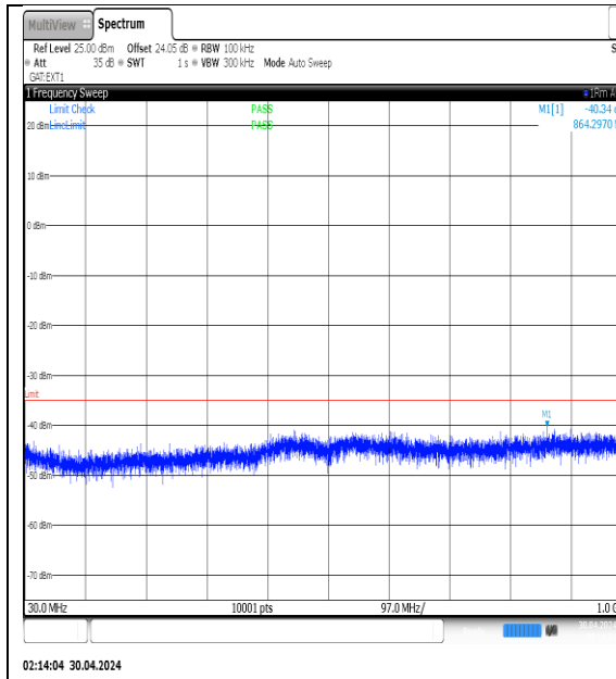
NTNV-N41-PC3-30-15-H-DFT-QPSK- Edge_1RB_Left-30-1000-Ant1-PASS
