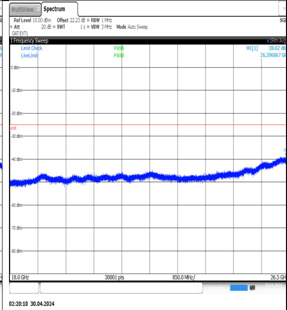
NTNV-N41-PC3-30-20-M-DFT-QPSK- Edge_1RB_Left-18000-26500-Ant1-PASS
