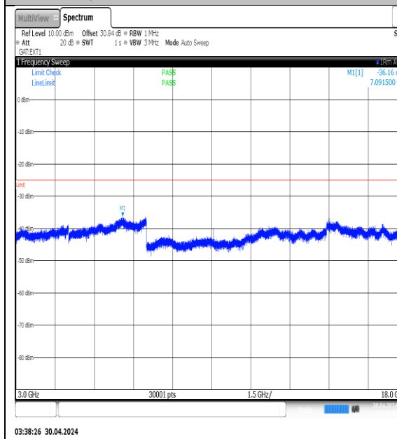
NTNV-N41-PC3-30-50-H-DFT-QPSK- Edge_1RB_Left-3000-18000-Ant1-PASS
