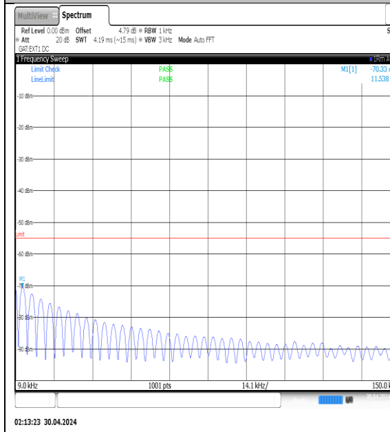
NTVN-N41-PC3-30-15-H-DFT-QPSK-Edge_1RB_Left-0.009-0.15-Ant1-PASS
