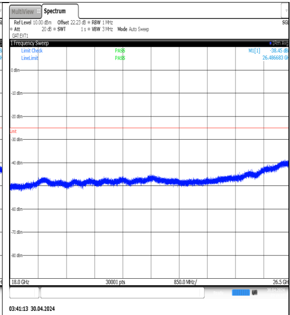
NTVN-N41-PC3-30-60-L-DFT-QPSK-Edge_1RB_Left-18000-26500-Ant1-PASS
