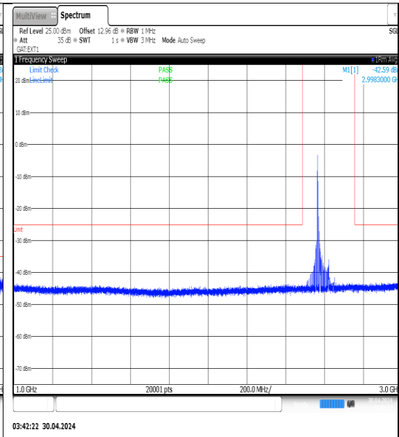
NTNV-N41-PC3-30-60-M-DFT-QPSK- Edge_1RB_Left-1000-3000-Ant1-PASS
