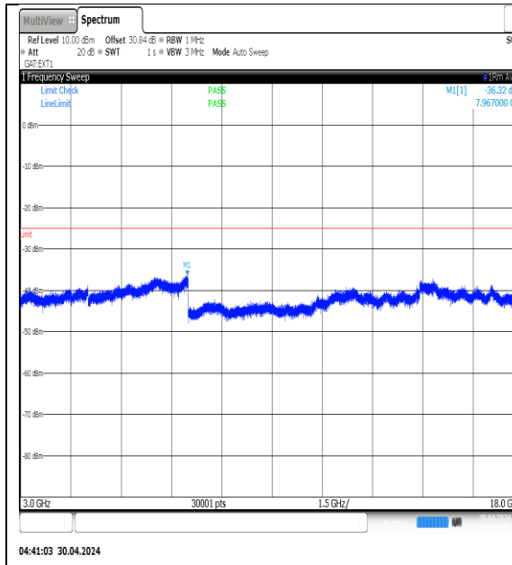
NTVN-N41-PC3-30-80-H-DFT-QPSK-Edge_1RB_Left-3000-18000-Ant1-PASS
