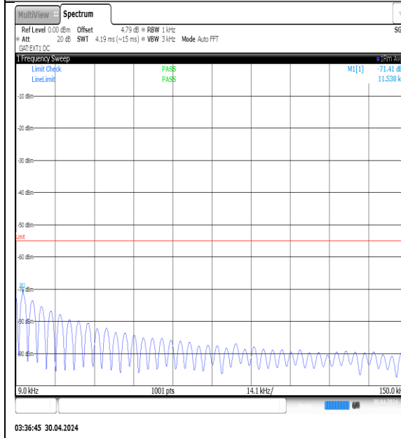
NTVN-N41-PC3-30-50-H-DFT-QPSK-Edge_1RB_Left-0.009-0.15-Ant1-PASS
