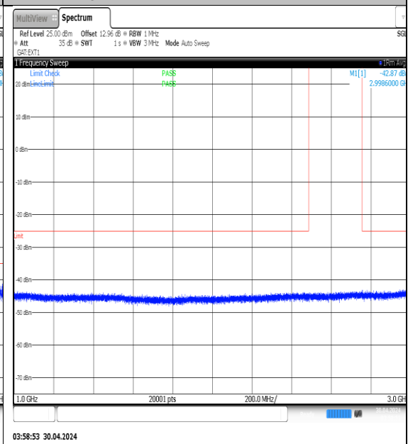
NTVN-N41-PC3-30-60-H-DFT-QPSK- Edge_1RB_Left-1000-3000-Ant1-PASS
