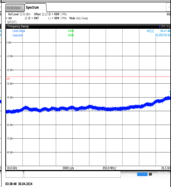
NTNV-N41-PC3-30-50-H-DFT-QPSK- Edge_1RB_Left-18000-26500-Ant1-PASS
