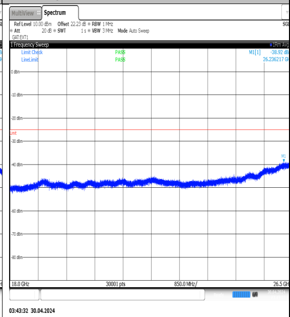
NTNV-N41-PC3-30-60-M-DFT-QPSK- Edge_1RB_Left-18000-26500-Ant1-PASS
