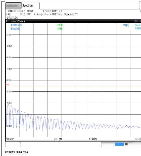
NTVN-N41-PC3-30-20-H-DFT-QPSK- Edge_1RB_Left-0.009-0.15-Ant1-PASS
