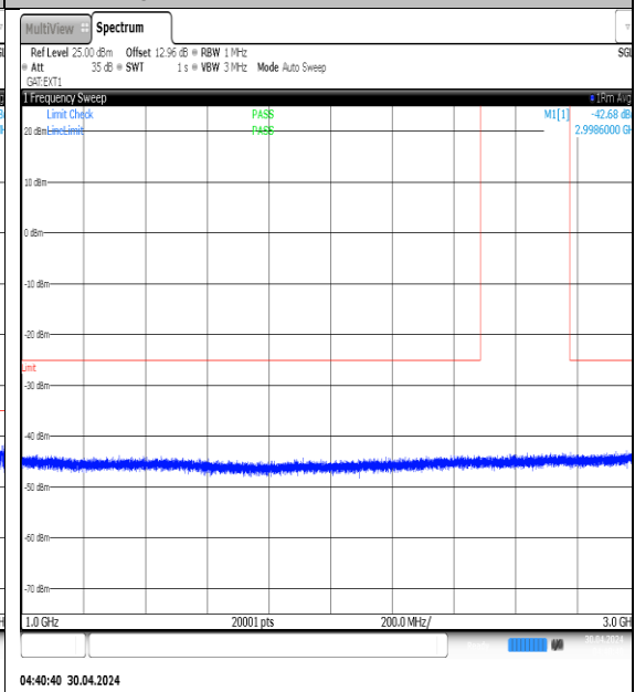
NTVN-N41-PC3-30-80-H-DFT-QPSK- Edge_1RB_Left-1000-3000-Ant1-PASS
