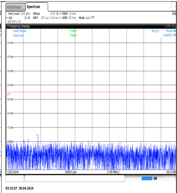
NTVN-N41-PC3-30-40-H-DFT-QPSK-Edge_1RB_Left-0.15-30-Ant1-PASS
