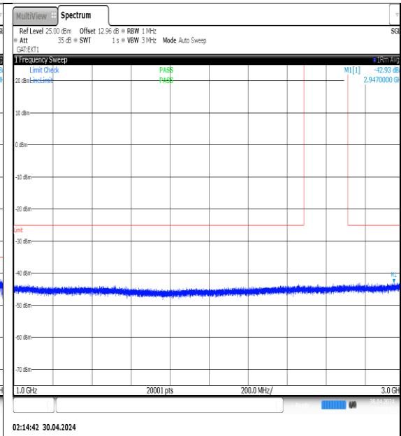
NTNV-N41-PC3-30-15-H-DFT-QPSK- Edge_1RB_Left-1000-3000-Ant1-PASS
