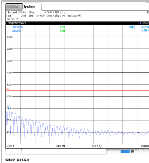
NTVN-N41-PC3-30-30-H-DFT-QPSK- Edge_1RB_Left-0.009-0.15-Ant1-PASS
