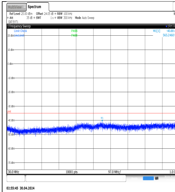
NTNV-N41-PC3-30-30-H-DFT-QPSK- Edge_1RB_Left-30-1000-Ant1-PASS
