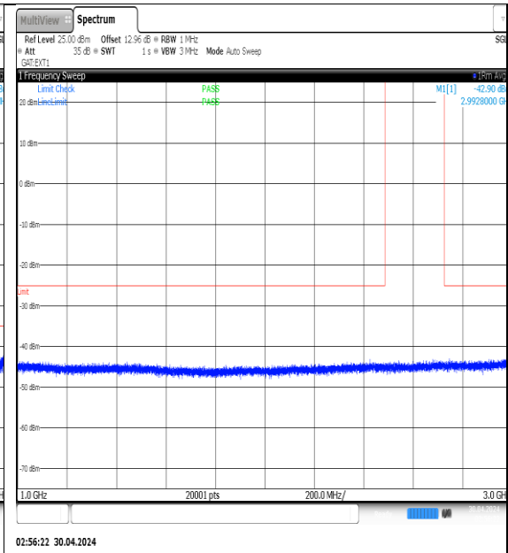
NTNV-N41-PC3-30-30-H-DFT-QPSK- Edge_1RB_Left-1000-3000-Ant1-PASS
