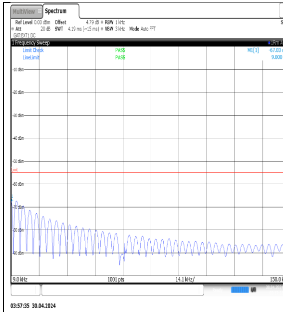
NTVN-N41-PC3-30-60-H-DFT-QPSK- Edge_1RB_Left-0.009-0.15-Ant1-PASS
