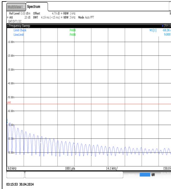
NTVN-N41-PC3-30-40-H-DFT-QPSK-Edge_1RB_Left-0.009-0.15-Ant1-PASS
