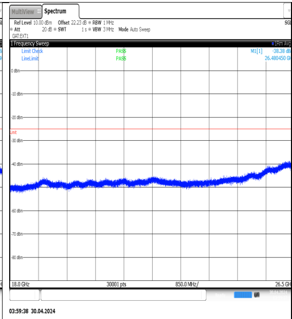
NTVN-N41-PC3-30-60-H-DFT-QPSK-Edge_1RB_Left-18000-26500-Ant1-PASS
