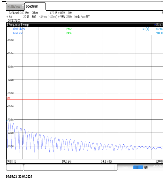
NTVN-N41-PC3-30-80-H-DFT-QPSK- Edge_1RB_Left-0.009-0.15-Ant1-PASS
