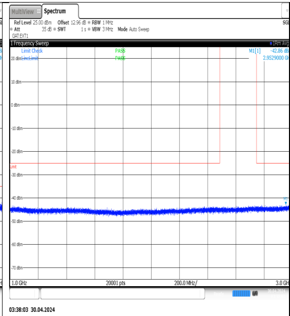
NTNV-N41-PC3-30-50-H-DFT-QPSK- Edge_1RB_Left-1000-3000-Ant1-PASS
