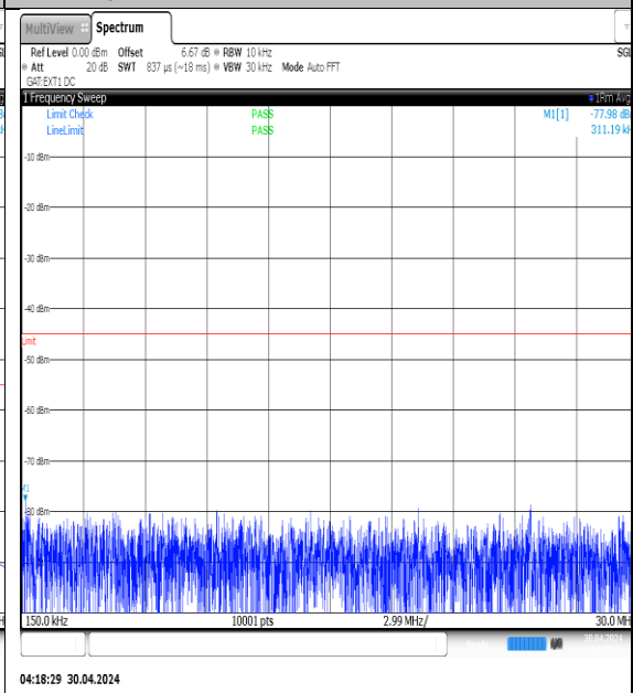
NTVN-N41-PC3-30-70-H-DFT-QPSK-Edge_1RB_Left-0.15-30-Ant1-PASS
