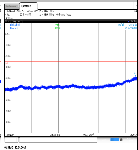
NTNV-N41-PC3-30-30-L-DFT-QPSK- Edge_1RB_Left-18000-26500-Ant1-PASS
