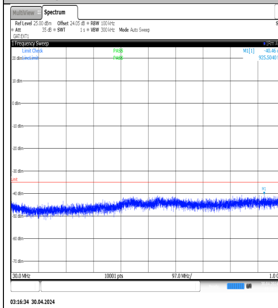
NTVN-N41-PC3-30-40-H-DFT-QPSK-Edge_1RB_Left-30-1000-Ant1-PASS
