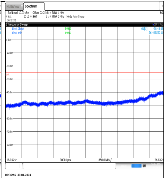
NTVN-N41-PC3-30-20-H-DFT-QPSK-Edge_1RB_Left-18000-26500-Ant1-PASS
