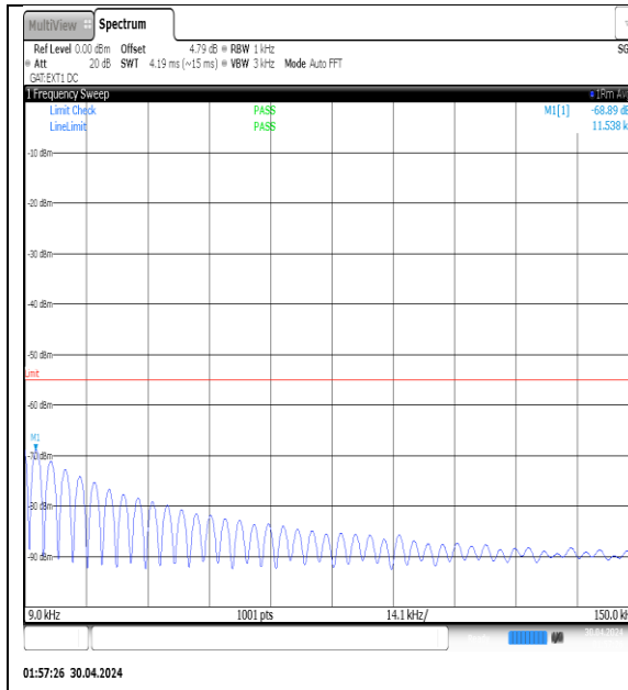
NTVN-N41-PC3-30-15-M-DFT-QPSK-Edge_1RB_Left-0.009-0.15-Ant1-PASS
