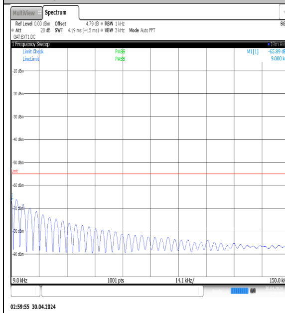
NTVN-N41-PC3-30-40-M-DFT-QPSK- Edge_1RB_Left-0.009-0.15-Ant1-PASS
