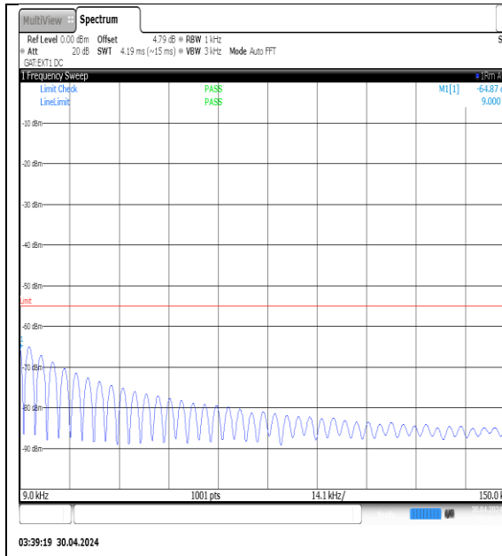
NTVN-N41-PC3-30-60-L-DFT-QPSK-Edge_1RB_Left-0.009-0.15-Ant1-PASS
