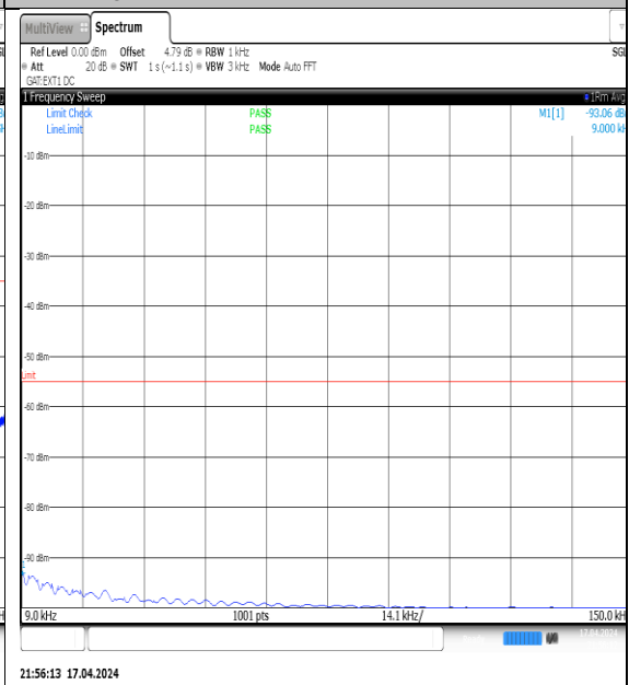
NTVN-N38-PC3-30-15-H-DFT-QPSK- Edge_1RB_Left-0.009-0.15-Ant1-PASS
