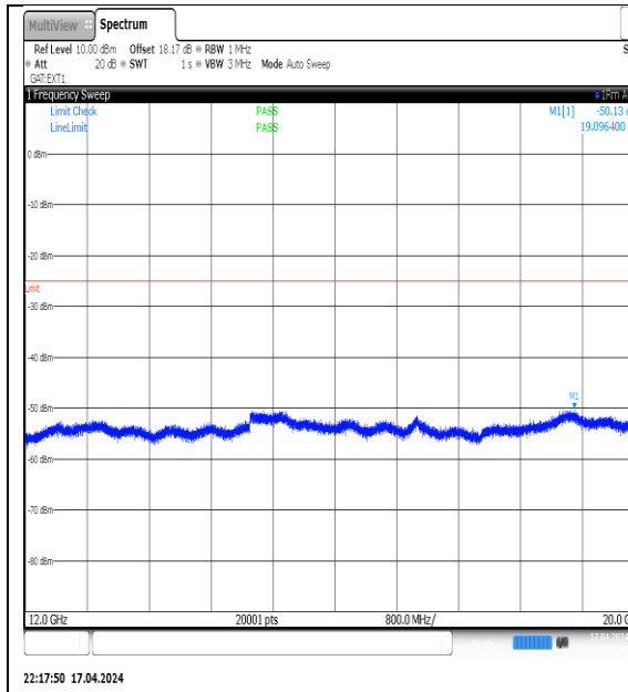
NTVN-N38-PC3-30-30-M-DFT-QPSK- Edge_1RB_Left-12000-20000-Ant1-PASS
