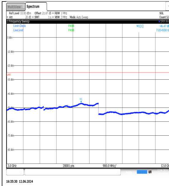
NTN-N7-PC3-15-30-H-DFT-QPSK-Edge_1RB_Left-3000-12000-Ant1-PASS
