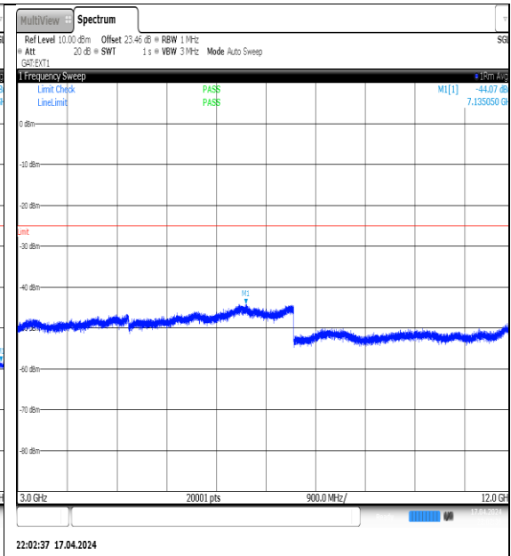
NTVN-N38-PC3-30-20-L-DFT-QPSK-Edge_1RB_Left-3000-12000-Ant1-PASS
