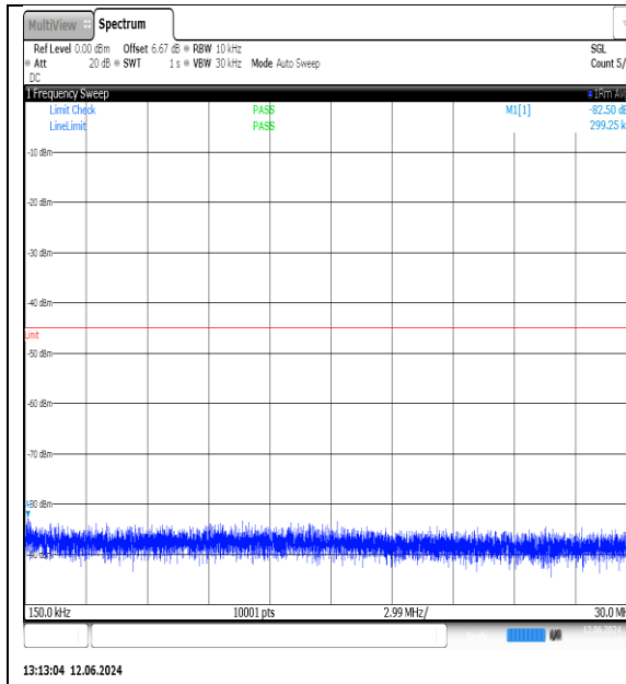
NTNV-N7-PC3-15-30-L-DFT-QPSK- Edge_1RB_Left-0.15-30-Ant1-PASS
