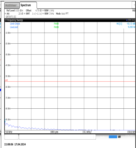
NTVN-N38-PC3-30-20-H-DFT-QPSK-Edge_1RB_Left-0.009-0.15-Ant1-PASS
