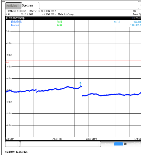
NTNV-N7-PC3-15-40-M-DFT-QPSK-Edge_1RB_Left-3000-12000-Ant1-PASS
