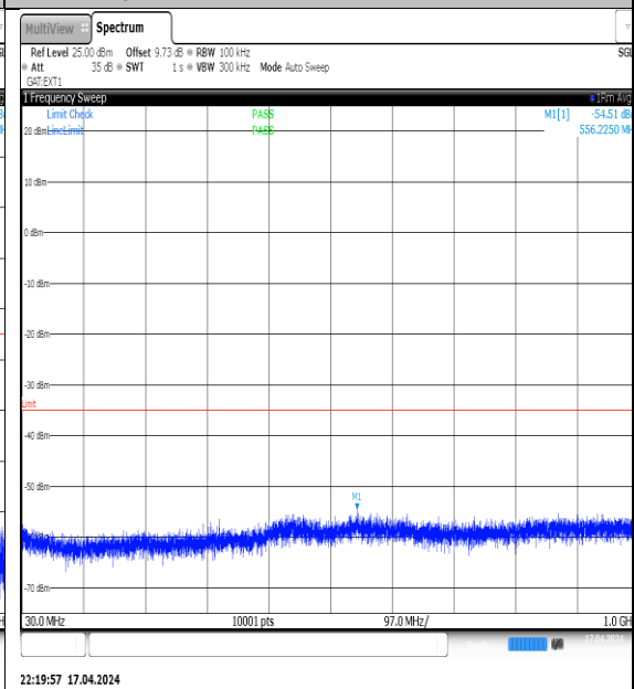
NTVN-N38-PC3-30-30-H-DFT-QPSK- Edge_1RB_Left-30-1000-Ant1-PASS
