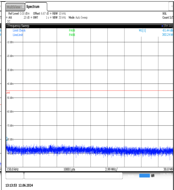
NTNV-N7-PC3-15-30-M-DFT-QPSK-Edge_1RB_Left-0.15-30-Ant1-PASS
