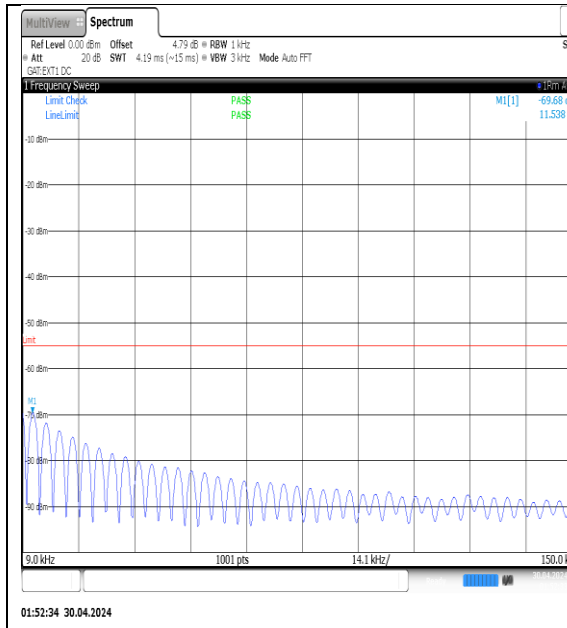
NTVN-N41-PC3-30-10-H-DFT-QPSK- Edge_1RB_Left-0.009-0.15-Ant1-PASS
