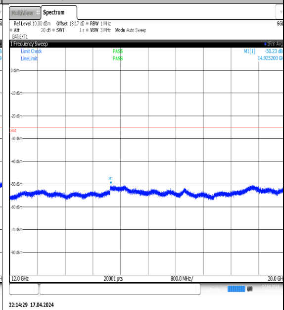
NTVN-N38-PC3-30-30-L-DFT-QPSK- Edge_1RB_Left-12000-20000-Ant1-PASS
