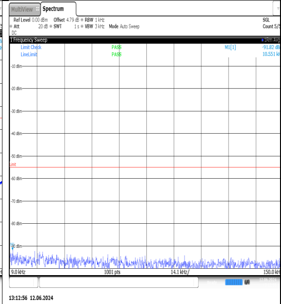
NTNV-N7-PC3-15-30-L-DFT-QPSK-Edge_1RB_Left-0.009-0.15-Ant1-PASS
