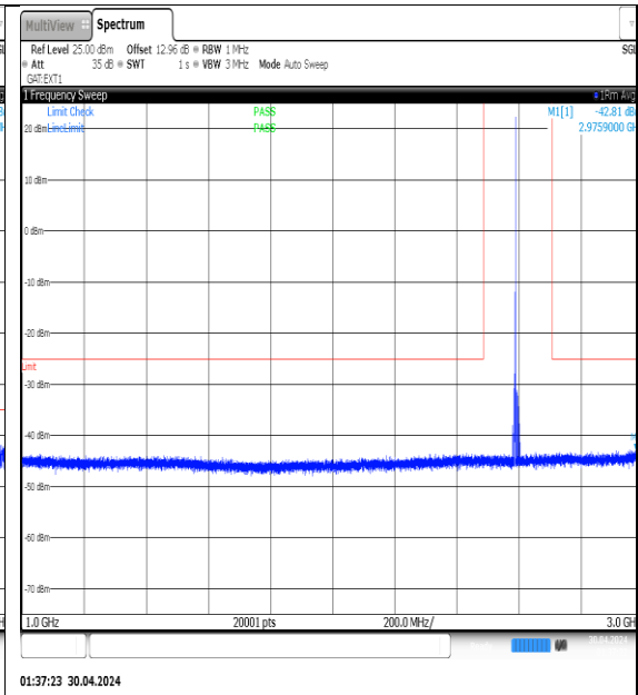
NTNV-N41-PC3-30-10-M-DFT-QPSK- Edge_1RB_Left-1000-3000-Ant1-PASS
