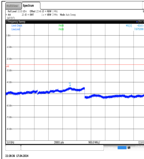
NTVN-N38-PC3-30-40-M-DFT-QPSK- Edge_1RB_Left-3000-12000-Ant1-PASS
