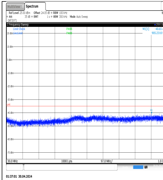
NTNV-N41-PC3-30-10-M-DFT-QPSK- Edge_1RB_Left-30-1000-Ant1-PASS
