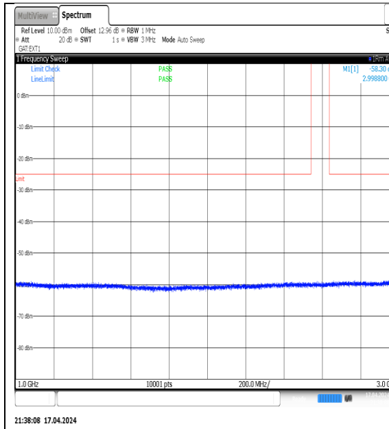
NTVN-N38-PC3-30-10-L-DFT-QPSK-Edge_1RB_Left-1000-3000-Ant1-PASS
