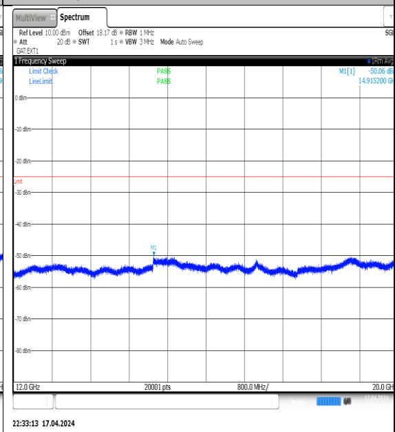
NTNV-N38-PC3-30-40-H-DFT-QPSK- Edge_1RB_Left-12000-20000-Ant1-PASS
