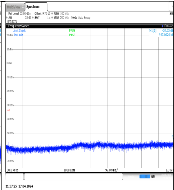
NTVN-N38-PC3-30-15-H-DFT-QPSK- Edge_1RB_Left-30-1000-Ant1-PASS
