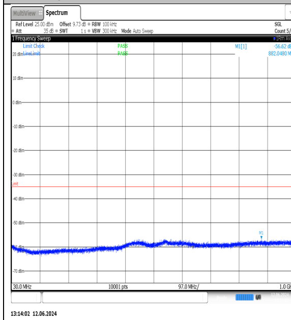
NTNV-N7-PC3-15-30-M-DFT-QPSK-Edge_1RB_Left-30-1000-Ant1-PASS
