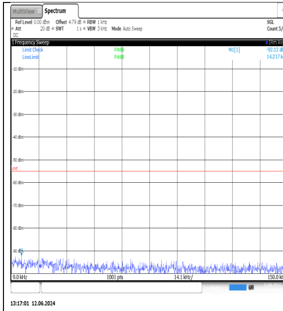
NTNV-N7-PC3-15-40-H-DFT-QPSK-Edge_1RB_Left-0.009-0.15-Ant1-PASS
