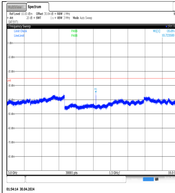
NTVN-N41-PC3-30-10-H-DFT-QPSK-Edge_1RB_Left-3000-18000-Ant1-PASS
