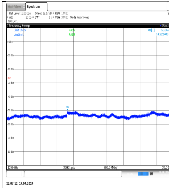
NTVN-N38-PC3-30-20-M-DFT-QPSK-Edge_1RB_Left-12000-20000-Ant1-PASS
