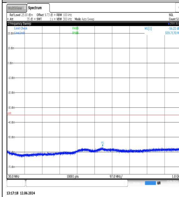
NTNV-N7-PC3-15-40-H-DFT-QPSK-Edge_1RB_Left-30-1000-Ant1-PASS
