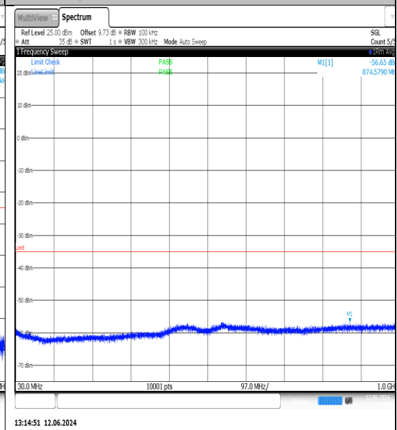
NTN-N7-PC3-15-30-H-DFT-QPSK-Edge_1RB_Left-30-1000-Ant1-PASS
