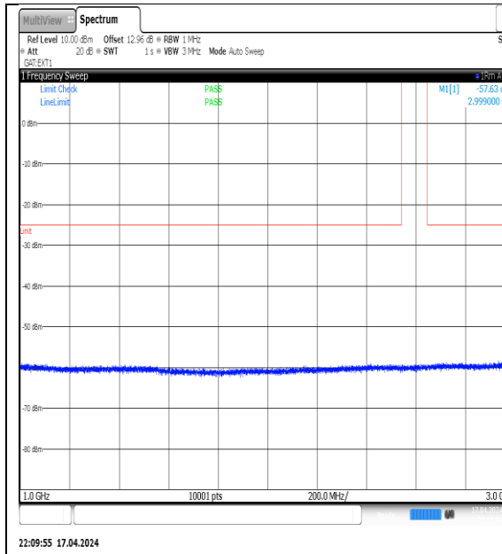
NTVN-N38-PC3-30-20-H-DFT-QPSK-Edge_1RB_Left-1000-3000-Ant1-PASS
