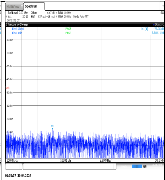
NTVN-N41-PC3-30-10-H-DFT-QPSK- Edge_1RB_Left-0.15-30-Ant1-PASS
