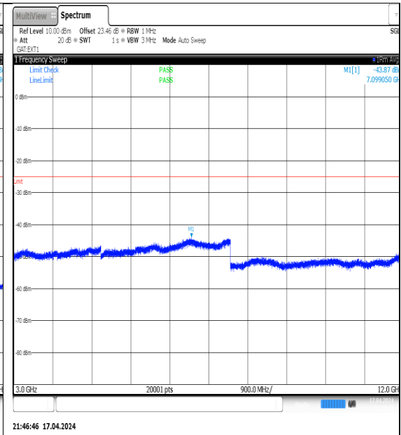
NTVN-N38-PC3-30-10-H-DFT-QPSK-Edge_1RB_Left-3000-12000-Ant1-PASS
