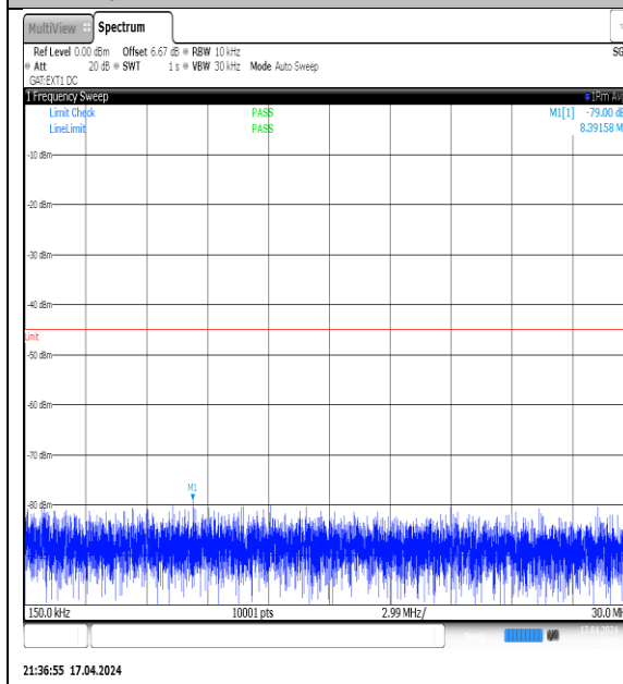
NTN-N38-PC3-30-10-L-DFT-QPSK-Edge_1RB_Left-0.15-30-Ant1-PASS
