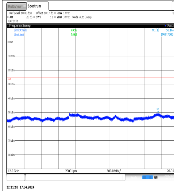
NTVN-N38-PC3-30-20-H-DFT-QPSK-Edge_1RB_Left-12000-20000-Ant1-PASS
