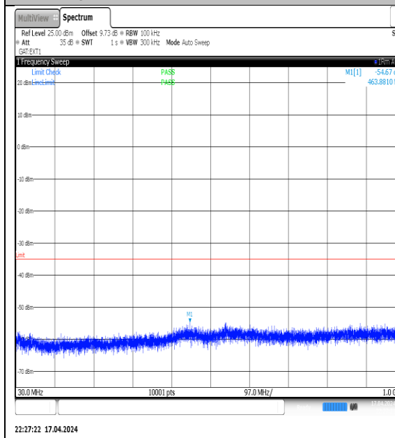
NTVN-N38-PC3-30-40-M-DFT-QPSK-Edge_1RB_Left-30-1000-Ant1-PASS
