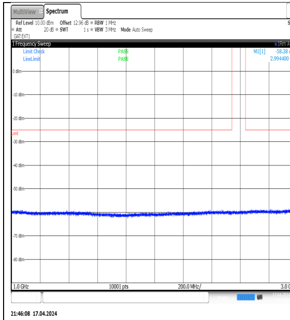
NTVN-N38-PC3-30-10-H-DFT-QPSK-Edge_1RB_Left-1000-3000-Ant1-PASS
