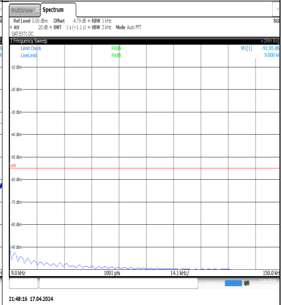
NTVN-N38-PC3-30-15-L-DFT-QPSK-Edge_1RB_Left-0.009-0.15-Ant1-PASS
