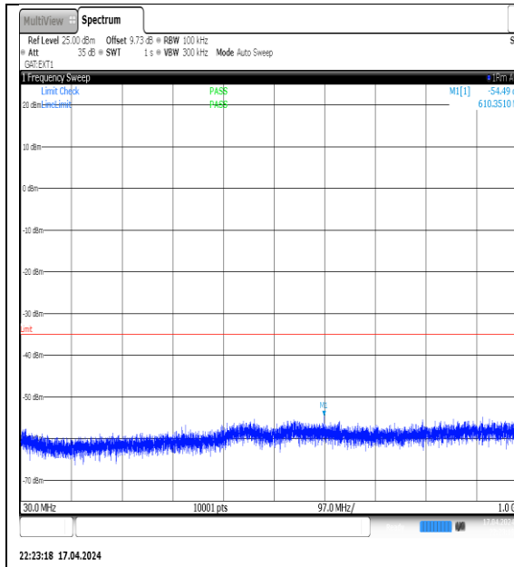
NTNV-N38-PC3-30-40-L-DFT-QPSK- Edge_1RB_Left-30-1000-Ant1-PASS
