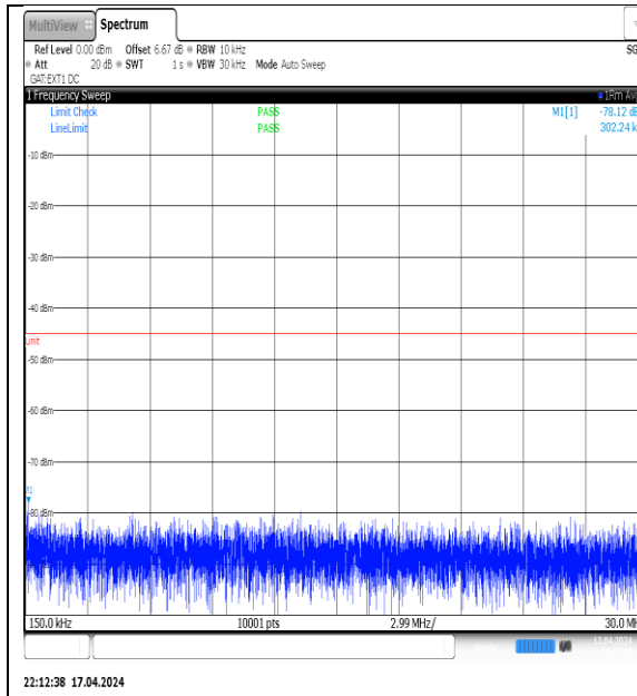
NTVN-N38-PC3-30-30-L-DFT-QPSK- Edge_1RB_Left-0.15-30-Ant1-PASS
