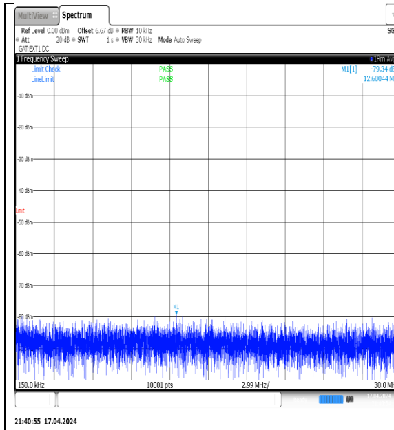
NTVN-N38-PC3-30-10-M-DFT-QPSK- Edge_1RB_Left-0.15-30-Ant1-PASS
