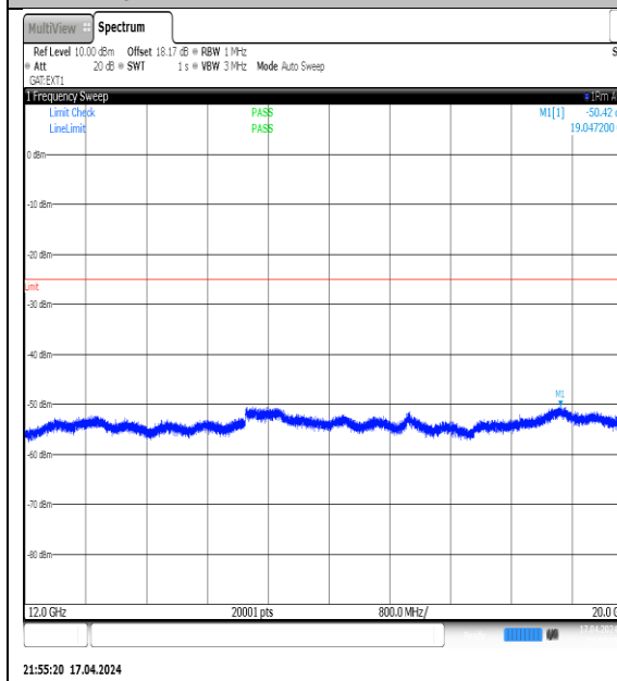
NTVN-N38-PC3-30-15-M-DFT-QPSK- Edge_1RB_Left-12000-20000-Ant1-PASS
