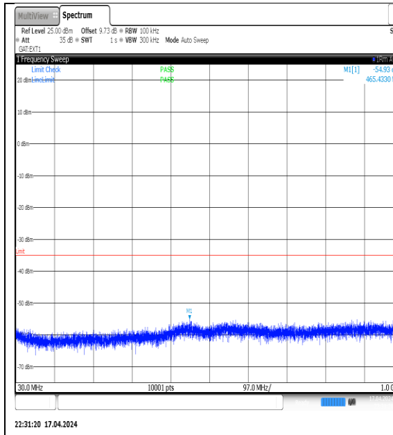
NTNV-N38-PC3-30-40-H-DFT-QPSK- Edge_1RB_Left-30-1000-Ant1-PASS
