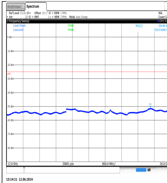
NTN-N7-PC3-15-30-M-DFT-QPSK-Edge_1RB_Left-12000-20000-Ant1-PASS
