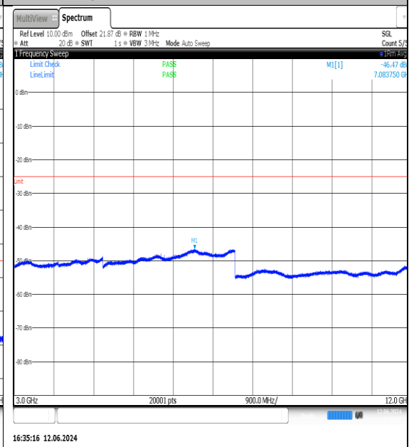
NTNV-N7-PC3-15-30-M-DFT-QPSK-Edge_1RB_Left-3000-12000-Ant1-PASS
