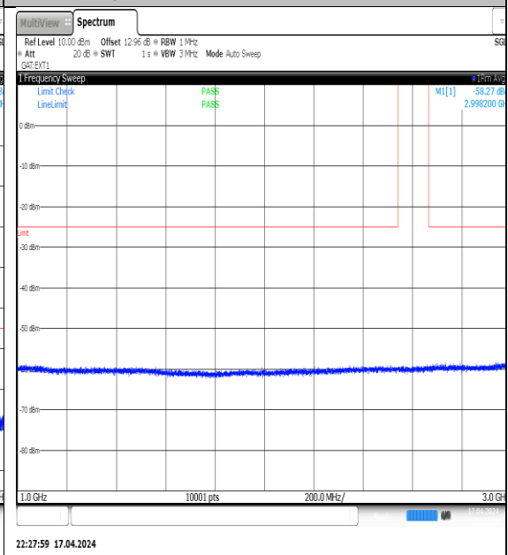
NTVN-N38-PC3-30-40-M-DFT-QPSK-Edge_1RB_Left-1000-3000-Ant1-PASS
