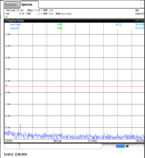
NTNV-N7-PC3-15-40-M-DFT-QPSK-Edge_1RB_Left-0.009-0.15-Ant1-PASS
