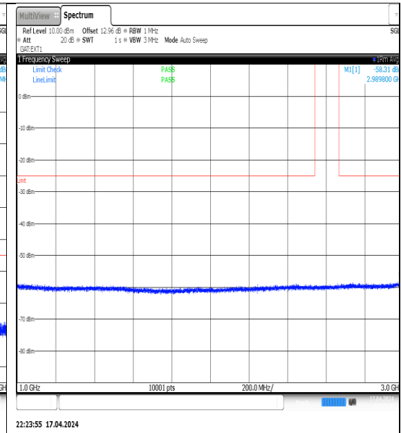
NTNV-N38-PC3-30-40-L-DFT-QPSK- Edge_1RB_Left-1000-3000-Ant1-PASS
