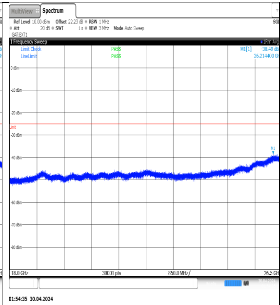
NTVN-N41-PC3-30-10-H-DFT-QPSK-Edge_1RB_Left-18000-26500-Ant1-PASS
