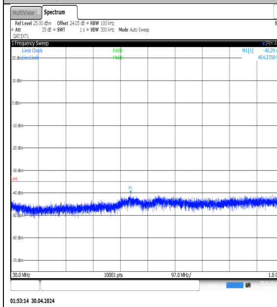
NTVN-N41-PC3-30-10-H-DFT-QPSK- Edge_1RB_Left-30-1000-Ant1-PASS
