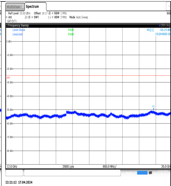
NTVN-N38-PC3-30-30-H-DFT-QPSK-Edge_1RB_Left-12000-20000-Ant1-PASS
