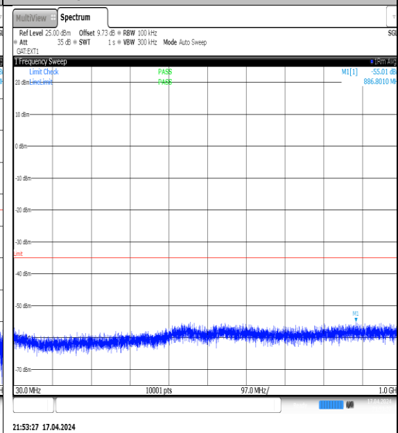
NTVN-N38-PC3-30-15-M-DFT-QPSK-Edge_1RB_Left-30-1000-Ant1-PASS
