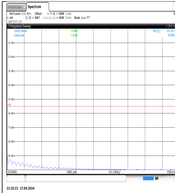
NTVN-N38-PC3-30-30-M-DFT-QPSK- Edge_1RB_Left-0.009-0.15-Ant1-PASS
