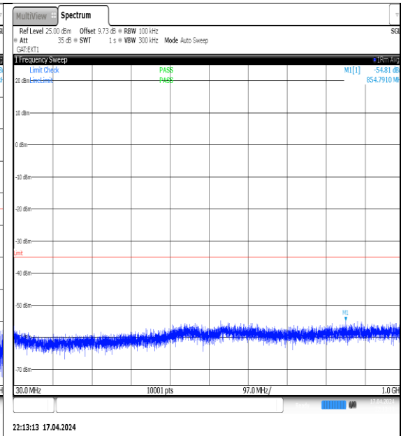
NTVN-N38-PC3-30-30-L-DFT-QPSK- Edge_1RB_Left-30-1000-Ant1-PASS
