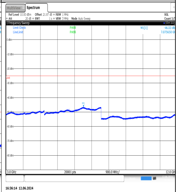
NTNV-N7-PC3-15-40-H-DFT-QPSK-Edge_1RB_Left-3000-12000-Ant1-PASS
