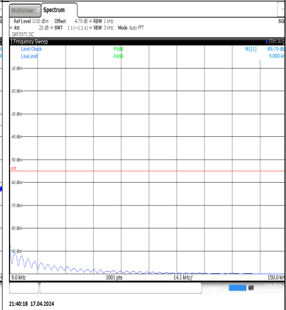
NTVN-N38-PC3-30-10-M-DFT-QPSK-Edge_1RB_Left-0.009-0.15-Ant1-PASS
