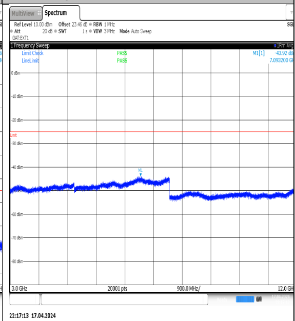
NTVN-N38-PC3-30-30-M-DFT-QPSK- Edge_1RB_Left-3000-12000-Ant1-PASS
