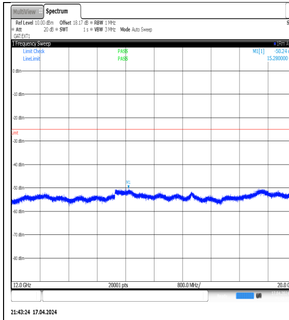
NTVN-N38-PC3-30-10-M-DFT-QPSK- Edge_1RB_Left-12000-20000-Ant1-PASS
