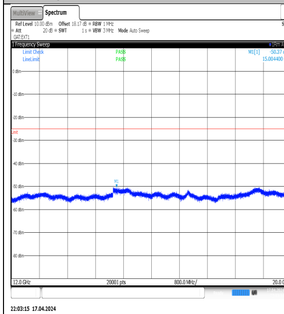
NTVN-N38-PC3-30-20-L-DFT-QPSK-Edge_1RB_Left-12000-20000-Ant1-PASS
