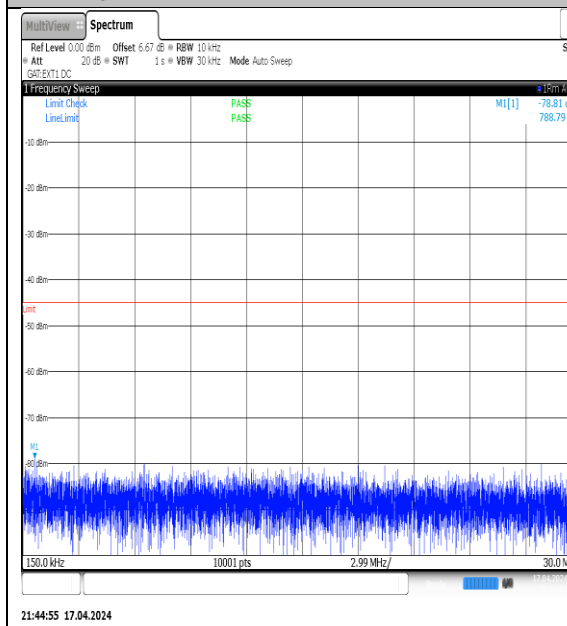
NTVN-N38-PC3-30-10-H-DFT-QPSK- Edge_1RB_Left-0.15-30-Ant1-PASS
