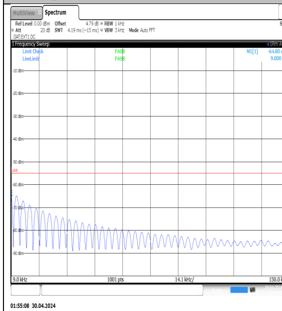
NTVN-N41-PC3-30-15-L-DFT-QPSK-Edge_1RB_Left-0.009-0.15-Ant1-PASS
