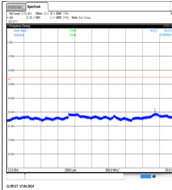
NTVN-N38-PC3-30-15-H-DFT-QPSK-Edge_1RB_Left-12000-20000-Ant1-PASS
