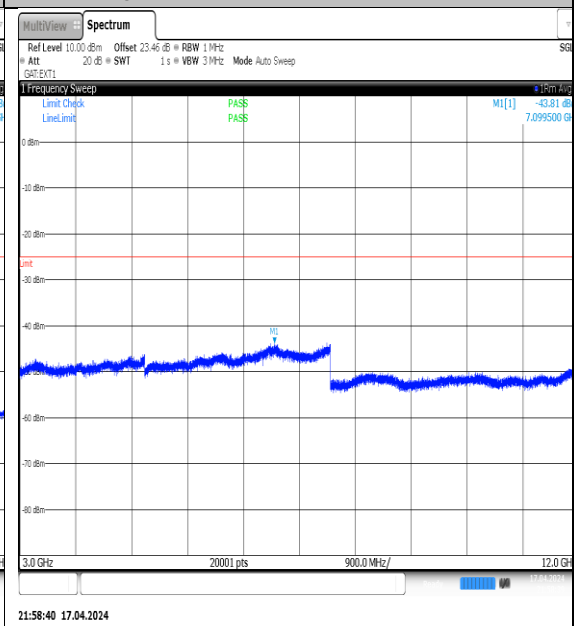
NTVN-N38-PC3-30-15-H-DFT-QPSK- Edge_1RB_Left-3000-12000-Ant1-PASS
