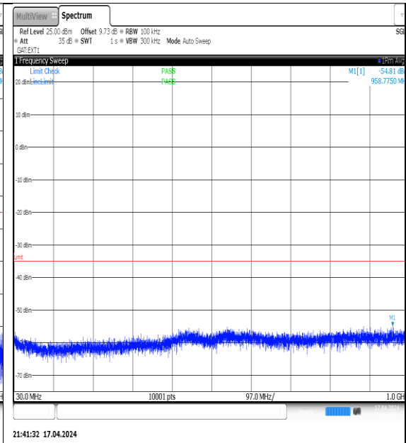
NTVN-N38-PC3-30-10-M-DFT-QPSK- Edge_1RB_Left-30-1000-Ant1-PASS
