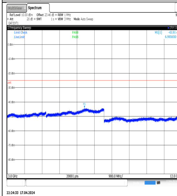
NTNV-N38-PC3-30-40-L-DFT-QPSK- Edge_1RB_Left-3000-12000-Ant1-PASS
