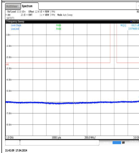
NTVN-N38-PC3-30-10-M-DFT-QPSK- Edge_1RB_Left-1000-3000-Ant1-PASS
