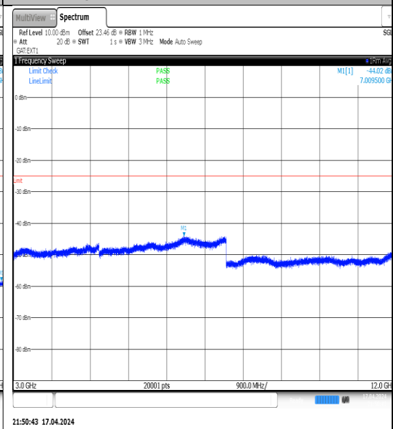
NTNV-N38-PC3-30-15-L-DFT-QPSK- Edge_1RB_Left-3000-12000-Ant1-PASS
