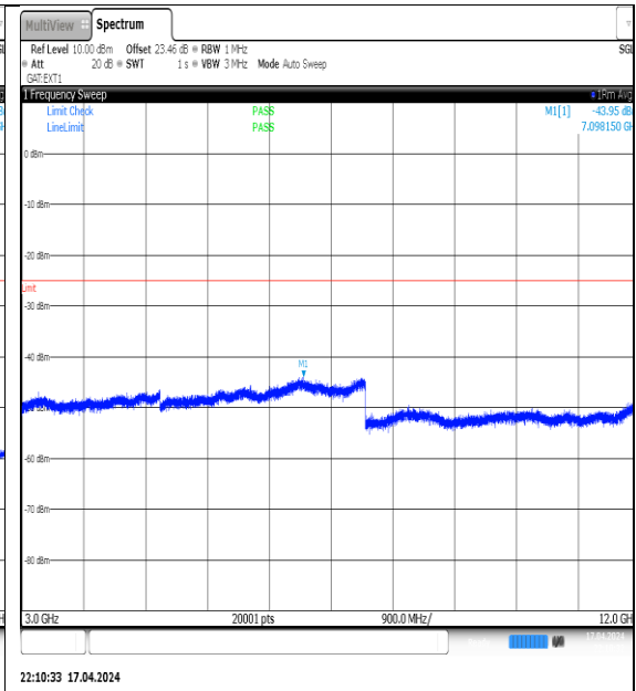
NTVN-N38-PC3-30-20-H-DFT-QPSK-Edge_1RB_Left-3000-12000-Ant1-PASS
