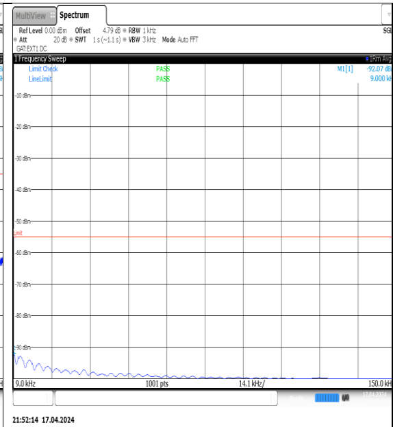
NTVN-N38-PC3-30-15-M-DFT-QPSK-Edge_1RB_Left-0.009-0.15-Ant1-PASS
