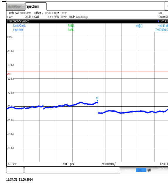
NTNV-N7-PC3-15-25-M-DFT-QPSK-Edge_1RB_Left-3000-12000-Ant1-PASS
