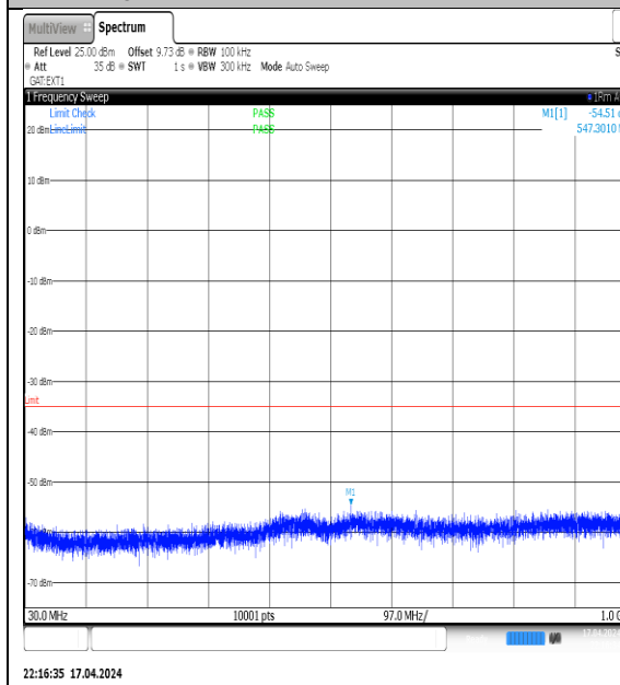
NTVN-N38-PC3-30-30-M-DFT-QPSK- Edge_1RB_Left-30-1000-Ant1-PASS
