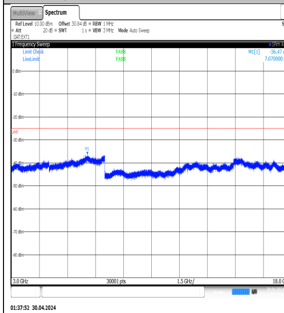
NTNV-N41-PC3-30-10-M-DFT-QPSK- Edge_1RB_Left-3000-18000-Ant1-PASS
