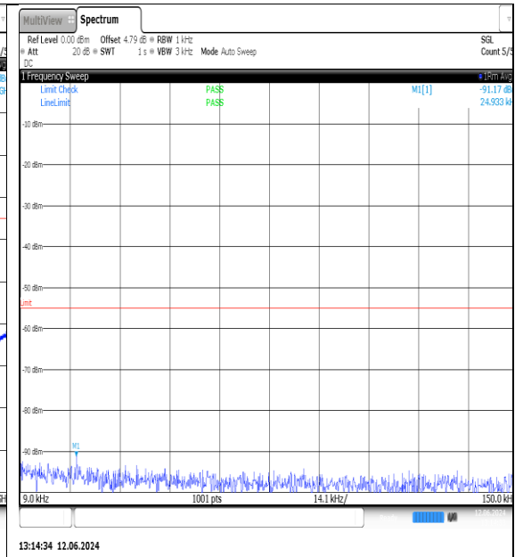
NTN-N7-PC3-15-30-H-DFT-QPSK-Edge_1RB_Left-0.009-0.15-Ant1-PASS
