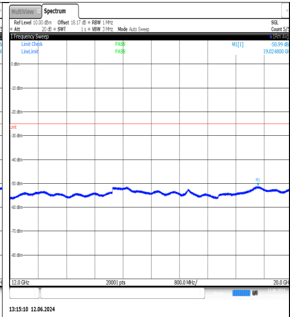
NTN-N7-PC3-15-30-H-DFT-QPSK-Edge_1RB_Left-12000-20000-Ant1-PASS
