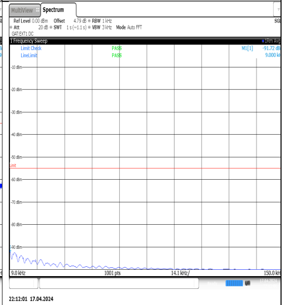
NTVN-N38-PC3-30-30-L-DFT-QPSK-Edge_1RB_Left-0.009-0.15-Ant1-PASS
