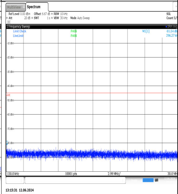
NTN-N7-PC3-15-40-L-DFT-QPSK-Edge_1RB_Left-0.15-30-Ant1-PASS
