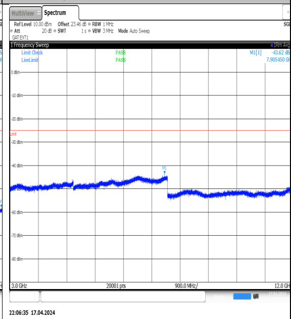
NTVN-N38-PC3-30-20-M-DFT-QPSK- Edge_1RB_Left-3000-12000-Ant1-PASS
