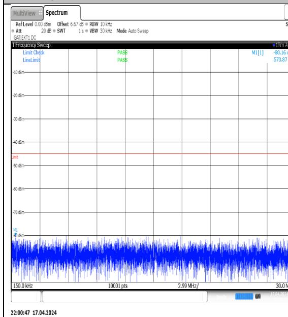
NTVN-N38-PC3-30-20-L-DFT-QPSK-Edge_1RB_Left-0.15-30-Ant1-PASS
