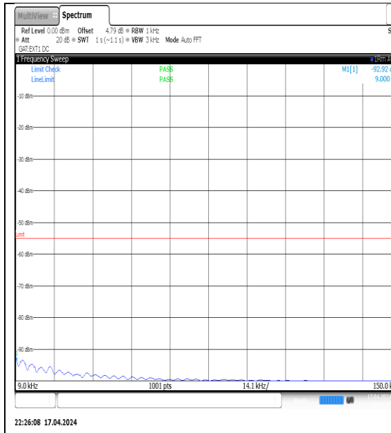
NTVN-N38-PC3-30-40-M-DFT-QPSK-Edge_1RB_Left-0.009-0.15-Ant1-PASS
