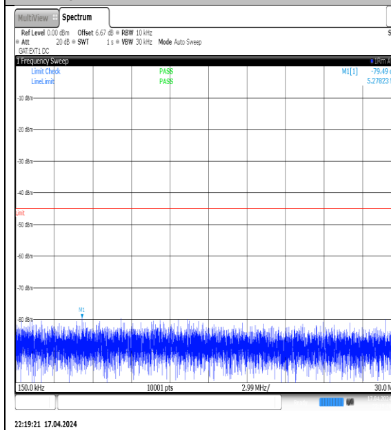
NTVN-N38-PC3-30-30-H-DFT-QPSK- Edge_1RB_Left-0.15-30-Ant1-PASS
