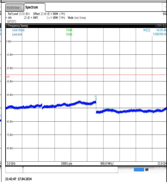
NTVN-N38-PC3-30-10-M-DFT-QPSK- Edge_1RB_Left-3000-12000-Ant1-PASS
