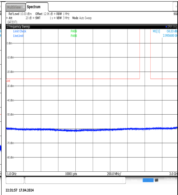
NTNV-N38-PC3-30-40-H-DFT-QPSK- Edge_1RB_Left-1000-3000-Ant1-PASS
