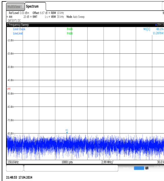
NTNV-N38-PC3-30-15-L-DFT-QPSK- Edge_1RB_Left-0.15-30-Ant1-PASS
