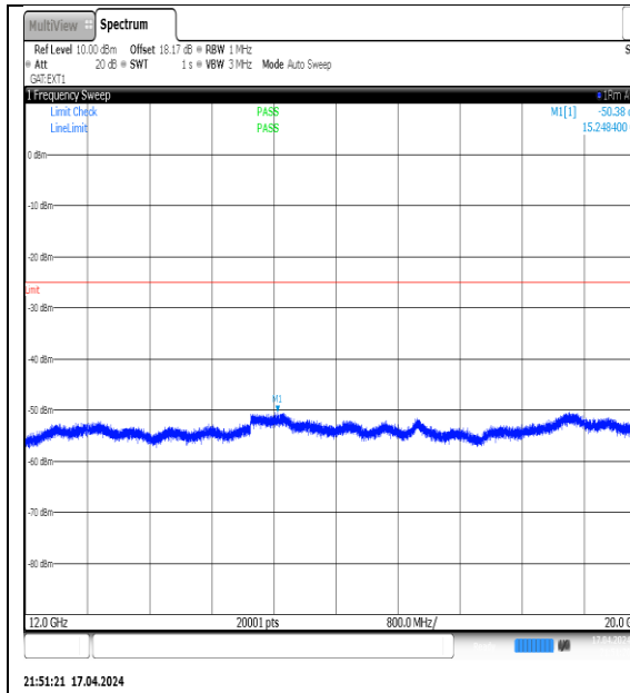
NTVN-N38-PC3-30-15-L-DFT-QPSK-Edge_1RB_Left-12000-20000-Ant1-PASS
