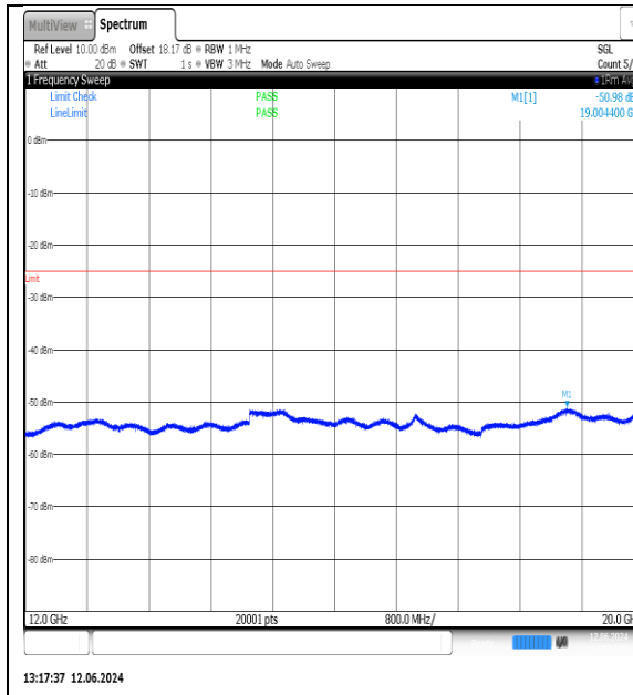
NTN-N7-PC3-15-40-H-DFT-QPSK-Edge_1RB_Left-12000-20000-Ant1-PASS
