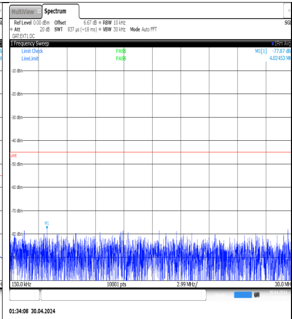
NTVN-N41-PC3-30-10-L-DFT-QPSK-Edge_1RB_Left-0.15-30-Ant1-PASS
