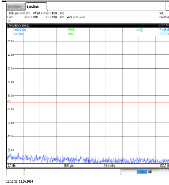
NTN-N7-PC3-15-40-L-DFT-QPSK-Edge_1RB_Left-0.009-0.15-Ant1-PASS
