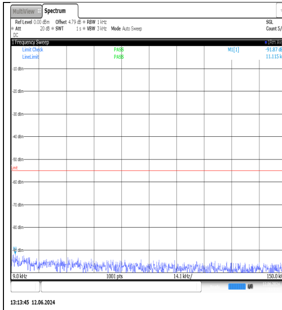
NTNV-N7-PC3-15-30-M-DFT-QPSK-Edge_1RB_Left-0.009-0.15-Ant1-PASS
