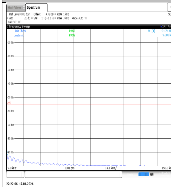
NTVN-N38-PC3-30-40-L-DFT-QPSK-Edge_1RB_Left-0.009-0.15-Ant1-PASS
