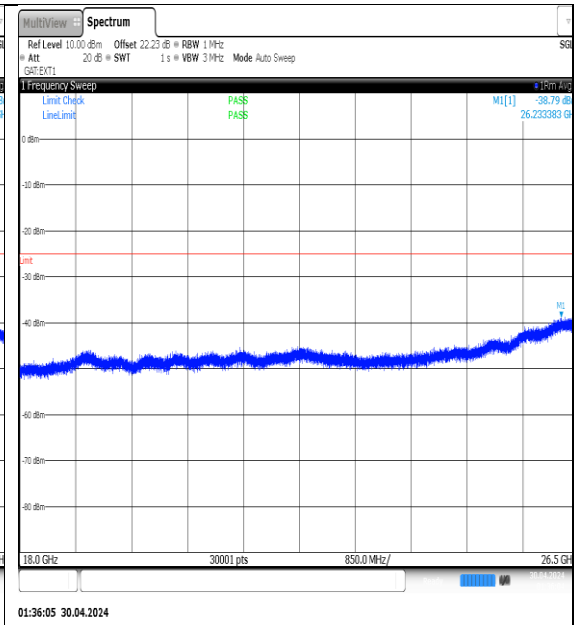
NTVN-N41-PC3-30-10-L-DFT-QPSK-Edge_1RB_Left-18000-26500-Ant1-PASS
