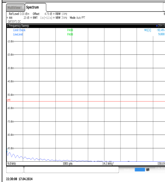
NTVN-N38-PC3-30-40-H-DFT-QPSK- Edge_1RB_Left-0.009-0.15-Ant1-PASS
