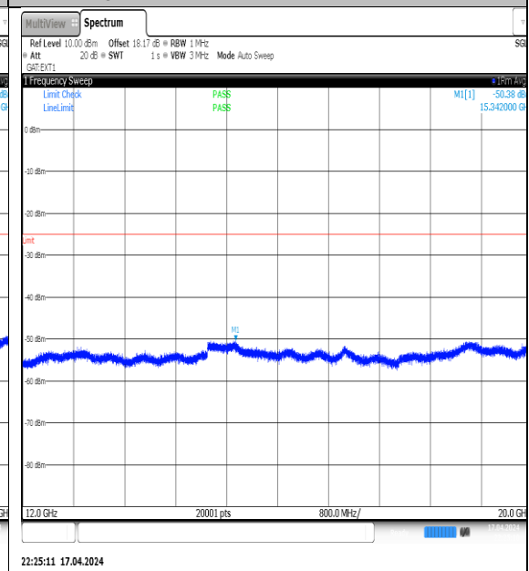
NTNV-N38-PC3-30-40-L-DFT-QPSK- Edge_1RB_Left-12000-20000-Ant1-PASS
