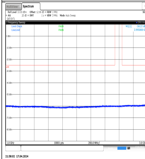
NTVN-N38-PC3-30-15-H-DFT-QPSK- Edge_1RB_Left-1000-3000-Ant1-PASS
