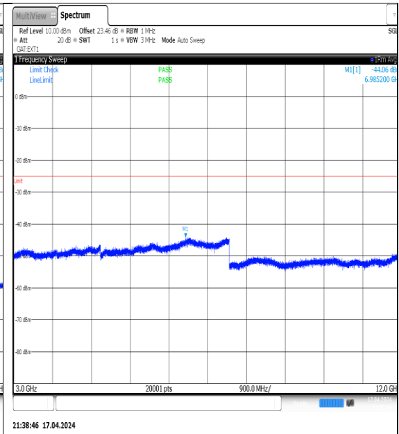
NTVN-N38-PC3-30-10-L-DFT-QPSK-Edge_1RB_Left-3000-12000-Ant1-PASS
