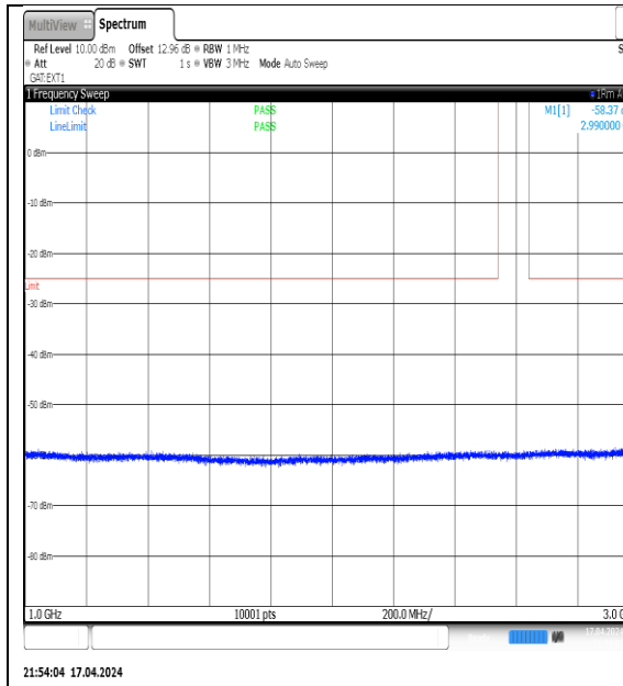
NTVN-N38-PC3-30-15-M-DFT-QPSK- Edge_1RB_Left-1000-3000-Ant1-PASS
