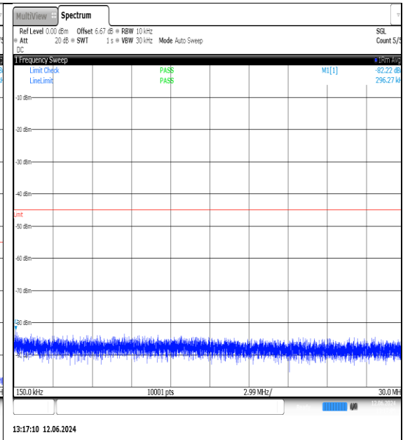
NTNV-N7-PC3-15-40-H-DFT-QPSK-Edge_1RB_Left-0.15-30-Ant1-PASS
