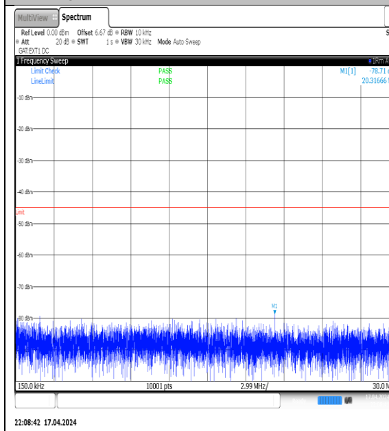
NTVN-N38-PC3-30-20-H-DFT-QPSK-Edge_1RB_Left-0.15-30-Ant1-PASS
