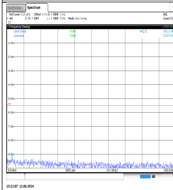
NTNV-N7-PC3-15-25-H-DFT-QPSK-Edge_1RB_Left-0.009-0.15-Ant1-PASS
