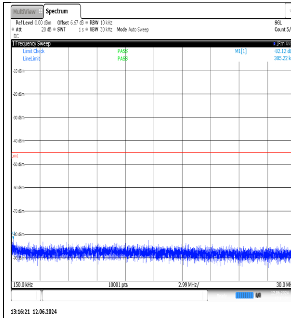
NTNV-N7-PC3-15-40-M-DFT-QPSK-Edge_1RB_Left-0.15-30-Ant1-PASS
