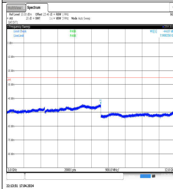
NTVN-N38-PC3-30-30-L-DFT-QPSK- Edge_1RB_Left-3000-12000-Ant1-PASS
