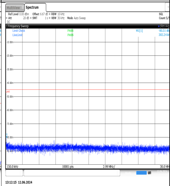
NTNV-N7-PC3-15-25-H-DFT-QPSK-Edge_1RB_Left-0.15-30-Ant1-PASS
