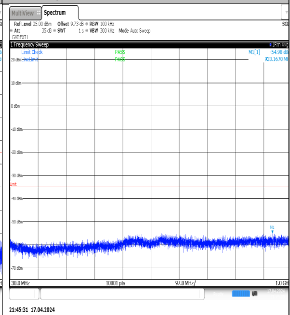
NTVN-N38-PC3-30-10-H-DFT-QPSK- Edge_1RB_Left-30-1000-Ant1-PASS
