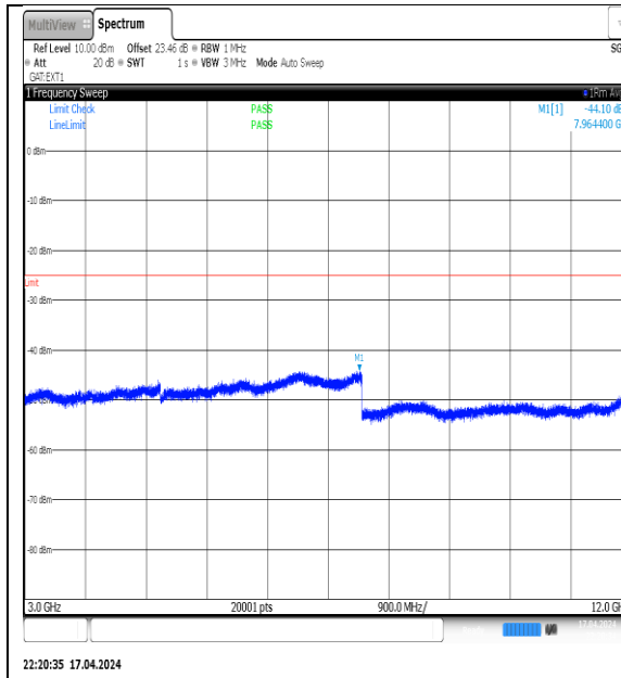
NTVN-N38-PC3-30-30-H-DFT-QPSK-Edge_1RB_Left-3000-12000-Ant1-PASS
