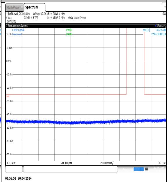
NTVN-N41-PC3-30-10-H-DFT-QPSK- Edge_1RB_Left-1000-3000-Ant1-PASS
