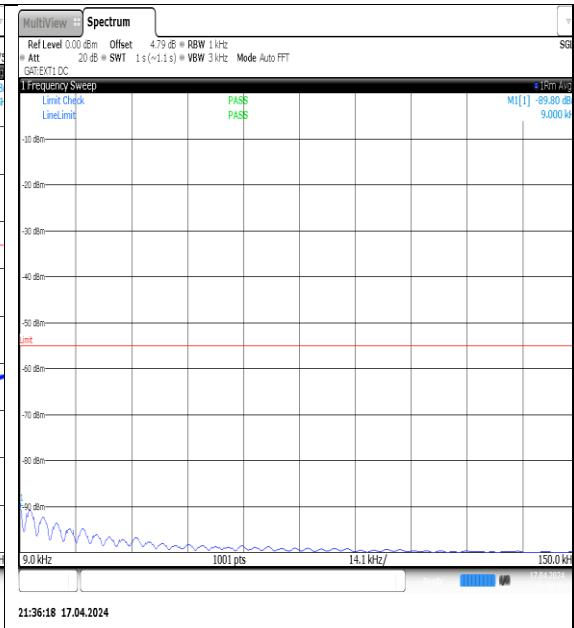
NTN-N38-PC3-30-10-L-DFT-QPSK-Edge_1RB_Left-0.009-0.15-Ant1-PASS
