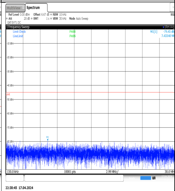
NTVN-N38-PC3-30-40-H-DFT-QPSK- Edge_1RB_Left-0.15-30-Ant1-PASS
