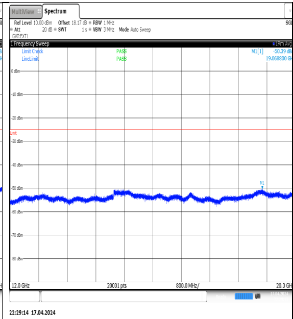
NTVN-N38-PC3-30-40-M-DFT-QPSK- Edge_1RB_Left-12000-20000-Ant1-PASS
