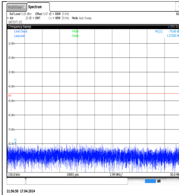
NTVN-N38-PC3-30-15-H-DFT-QPSK- Edge_1RB_Left-0.15-30-Ant1-PASS
