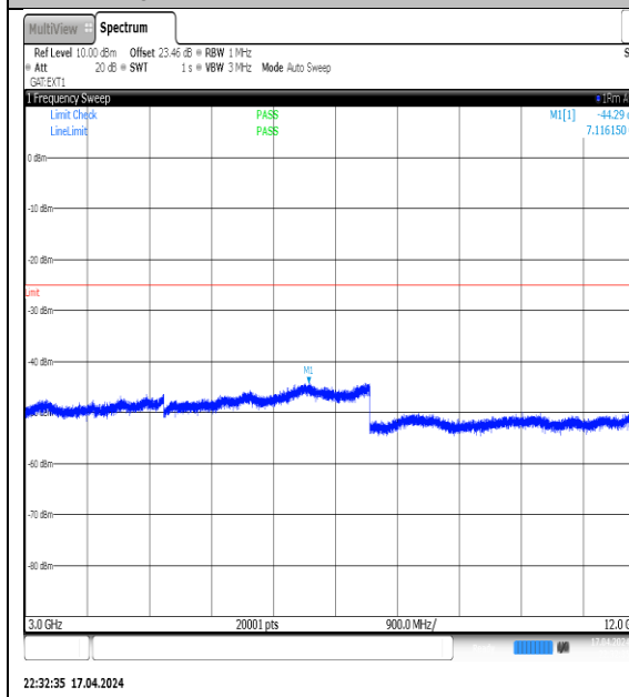
NTNV-N38-PC3-30-40-H-DFT-QPSK- Edge_1RB_Left-3000-12000-Ant1-PASS
