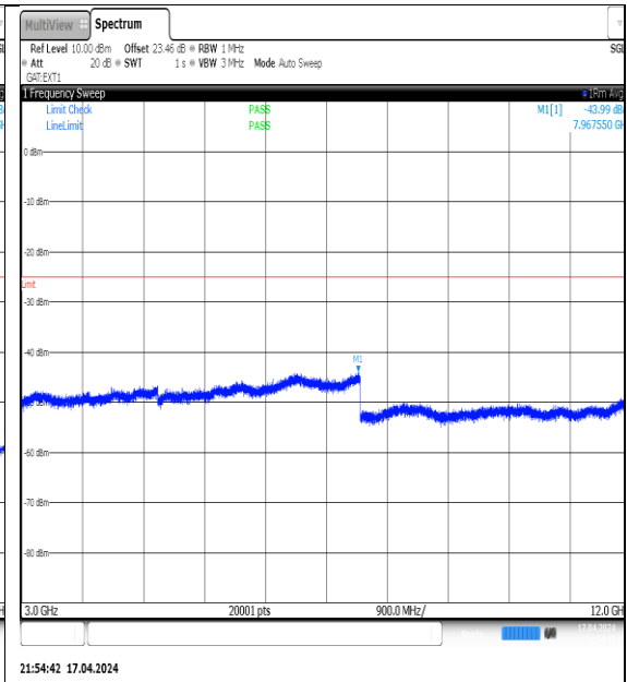
NTVN-N38-PC3-30-15-M-DFT-QPSK- Edge_1RB_Left-3000-12000-Ant1-PASS
