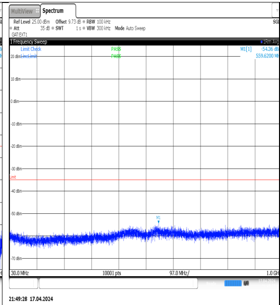
NTNV-N38-PC3-30-15-L-DFT-QPSK- Edge_1RB_Left-30-1000-Ant1-PASS
