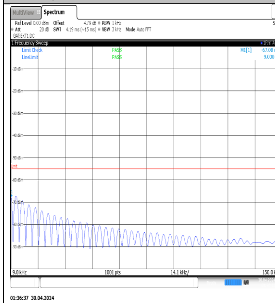
NTVN-N41-PC3-30-10-M-DFT-QPSK-Edge_1RB_Left-0.009-0.15-Ant1-PASS
