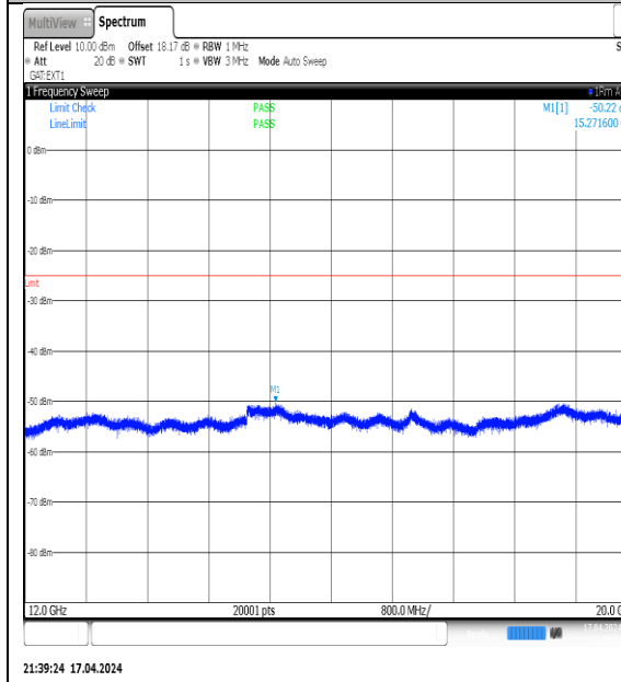
NTVN-N38-PC3-30-10-L-DFT-QPSK-Edge_1RB_Left-12000-20000-Ant1-PASS
