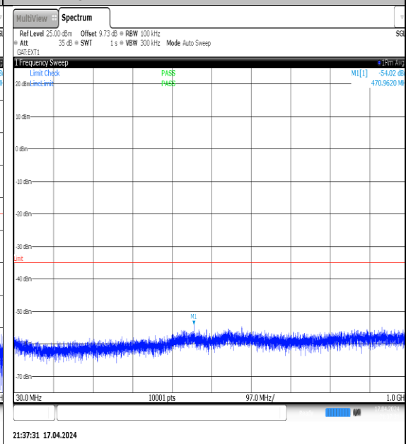
NTN-N38-PC3-30-10-L-DFT-QPSK-Edge_1RB_Left-30-1000-Ant1-PASS
