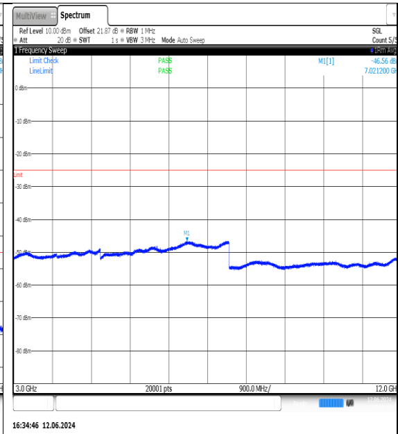
NTNV-N7-PC3-15-25-H-DFT-QPSK-Edge_1RB_Left-3000-12000-Ant1-PASS
