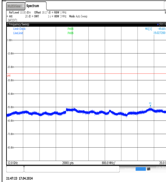
NTVN-N38-PC3-30-10-H-DFT-QPSK-Edge_1RB_Left-12000-20000-Ant1-PASS
