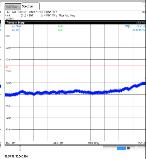
NTNV-N41-PC3-30-10-M-DFT-QPSK- Edge_1RB_Left-18000-26500-Ant1-PASS
