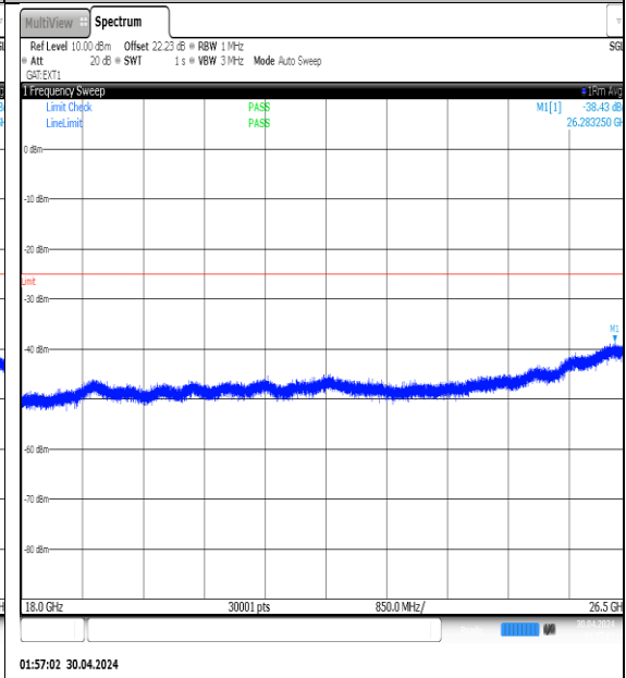
NTVN-N41-PC3-30-15-L-DFT-QPSK-Edge_1RB_Left-18000-26500-Ant1-PASS
