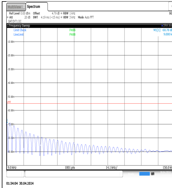
NTVN-N41-PC3-30-10-L-DFT-QPSK-Edge_1RB_Left-0.009-0.15-Ant1-PASS
