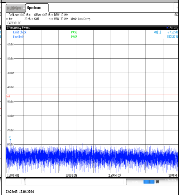
NTVN-N38-PC3-30-40-L-DFT-QPSK-Edge_1RB_Left-0.15-30-Ant1-PASS
