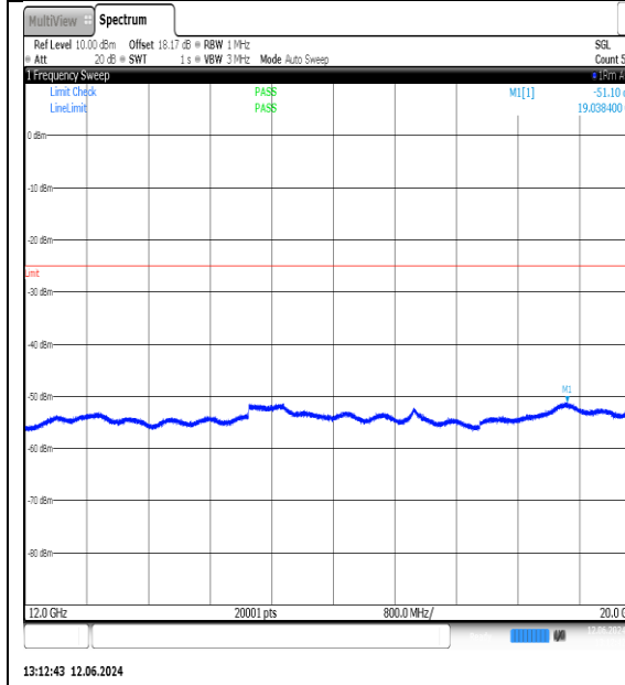
NTNV-N7-PC3-15-25-H-DFT-QPSK-Edge_1RB_Left-12000-20000-Ant1-PASS
