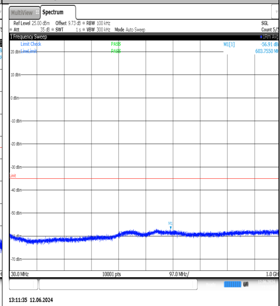
NTN-N7-PC3-15-25-M-DFT-QPSK- Edge_1RB_Left-30-1000-Ant1-PASS
