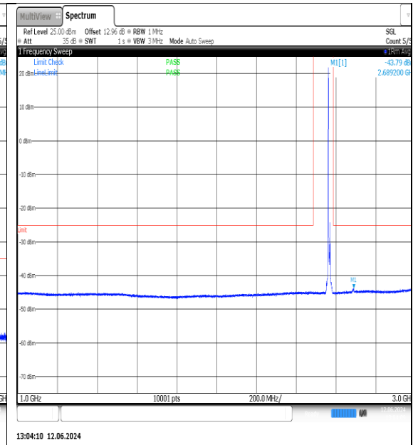
NTNV-N7-PC3-15-10-H-DFT-QPSK-Edge_1RB_Left-1000-3000-Ant1-PASS
