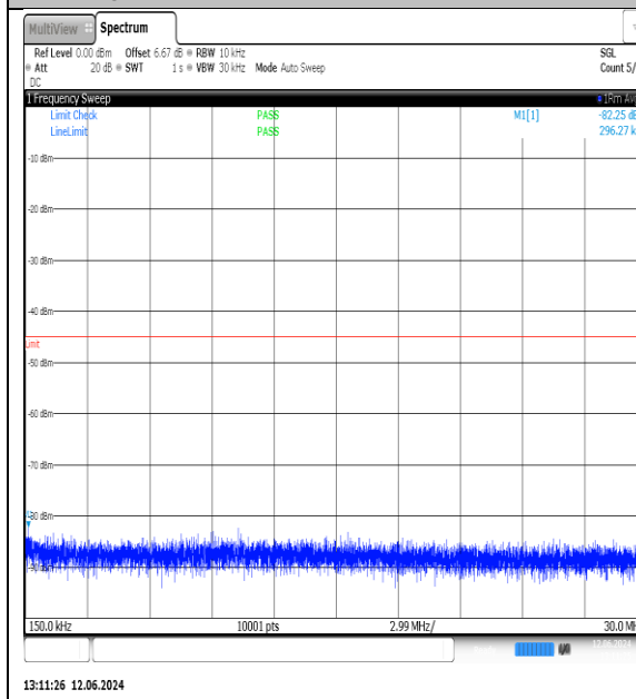
NTN-N7-PC3-15-25-M-DFT-QPSK- Edge_1RB_Left-0.15-30-Ant1-PASS
