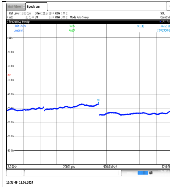
NTNV-N7-PC3-15-20-M-DFT-QPSK-Edge_1RB_Left-3000-12000-Ant1-PASS
