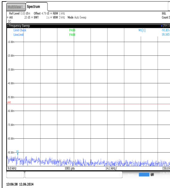
NTN-N7-PC3-15-15-H-DFT-QPSK-Edge_1RB_Left-0.009-0.15-Ant1-PASS
