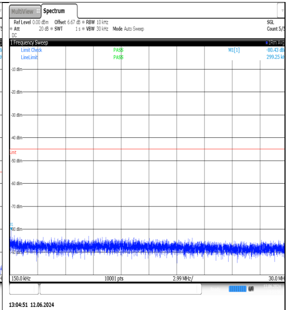
NTNV-N7-PC3-15-15-L-DFT-QPSK-Edge_1RB_Left-0.15-30-Ant1-PASS
