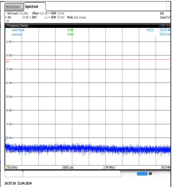
NTNV-N5-PC3-15-10-M-DFT-QPSK- Edge_1RB_Left-0.15-30-Ant1-PASS
