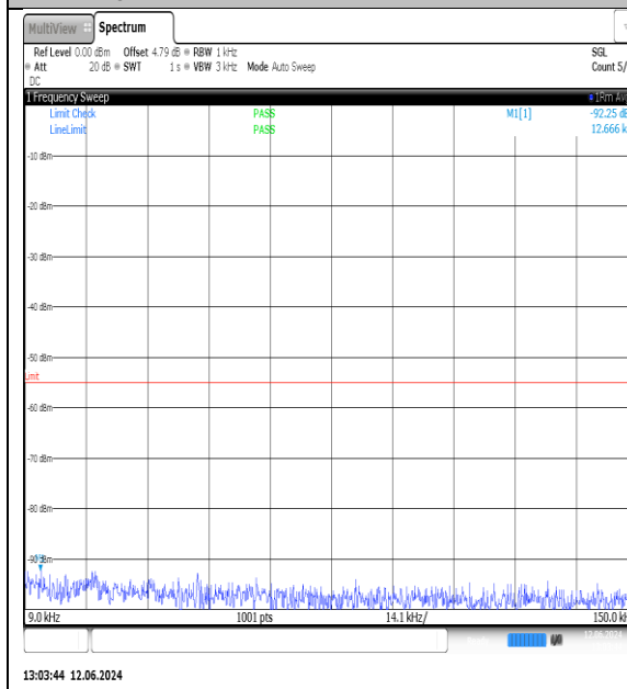
NTVN-N7-PC3-15-10-H-DFT-QPSK-Edge_1RB_Left-0.009-0.15-Ant1-PASS
