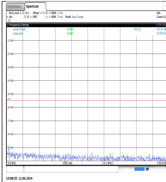
NTVN-N7-PC3-15-20-M-DFT-QPSK-Edge_1RB_Left-0.009-0.15-Ant1-PASS
