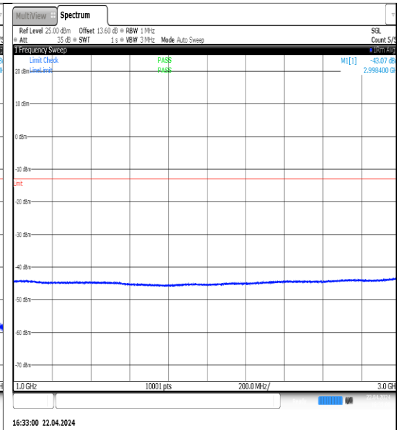
NTNV-N5-PC3-15-5-M-DFT-QPSK- Edge_1RB_Left-1000-3000-Ant1-PASS
