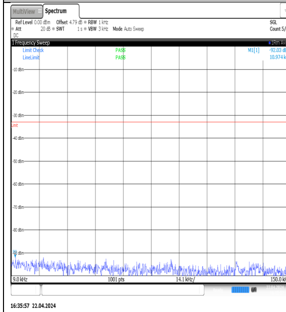
NTN-N5-PC3-15-10-L-DFT-QPSK- Edge_1RB_Left-0.009-0.15-Ant1-PASS
