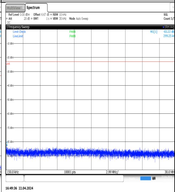
NTNV-N5-PC3-15-20-H-DFT-QPSK-Edge_1RB_Left-0.15-30-Ant1-PASS
