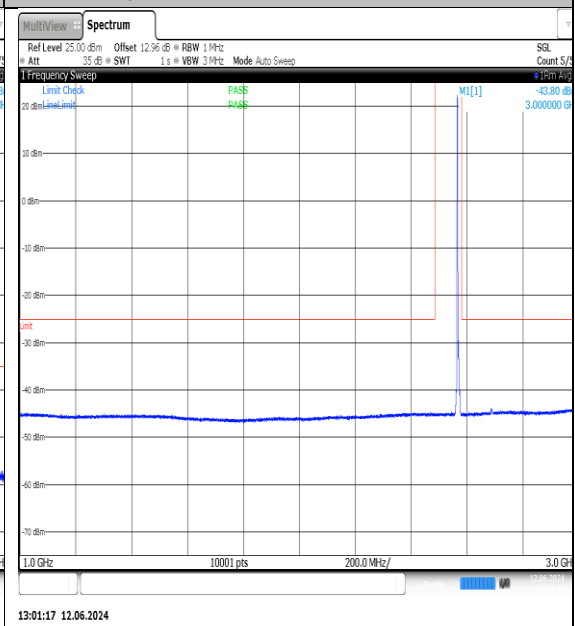
NTNV-N7-PC3-15-5-H-DFT-QPSK- Edge_1RB_Left-1000-3000-Ant1-PASS
