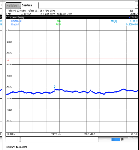
NTNV-N7-PC3-15-10-H-DFT-QPSK-Edge_1RB_Left-12000-20000-Ant1-PASS
