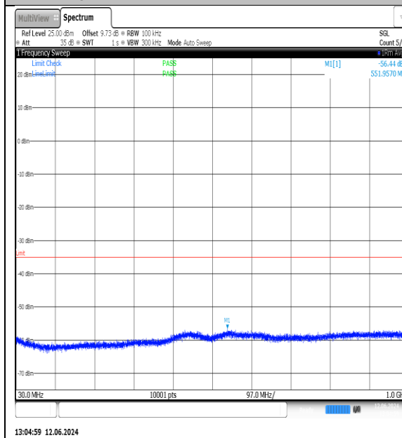
NTNV-N7-PC3-15-15-L-DFT-QPSK-Edge_1RB_Left-30-1000-Ant1-PASS
