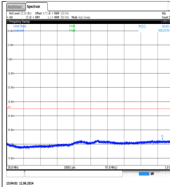
NTNV-N7-PC3-15-10-H-DFT-QPSK-Edge_1RB_Left-30-1000-Ant1-PASS
