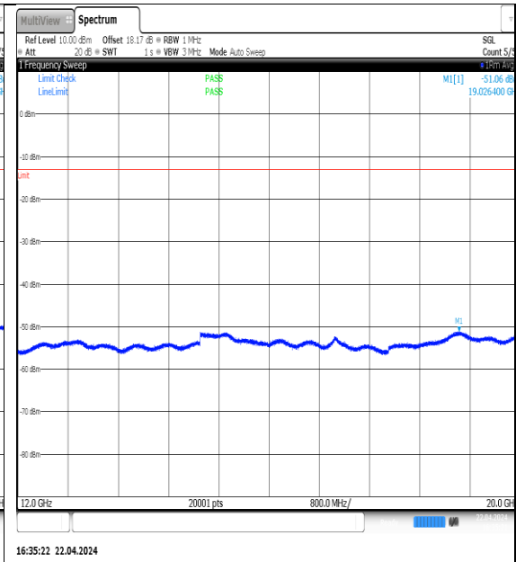
NTN-N5-PC3-15-5-H-DFT-QPSK- Edge_1RB_Left-12000-20000-Ant1-PASS
