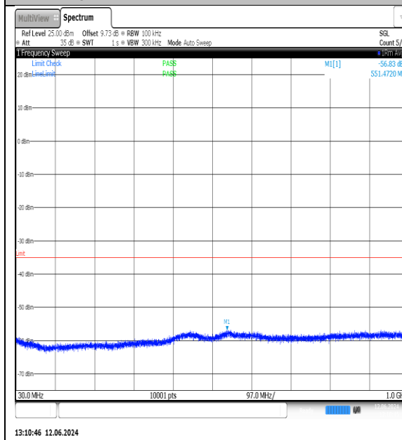
NTNV-N7-PC3-15-25-L-DFT-QPSK- Edge_1RB_Left-30-1000-Ant1-PASS
