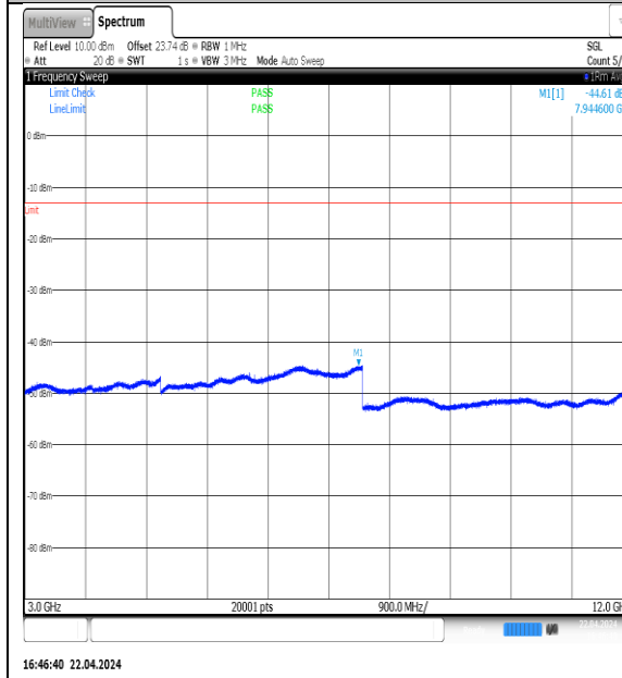
NTNV-N5-PC3-15-20-L-DFT-QPSK-Edge_1RB_Left-3000-12000-Ant1-PASS
