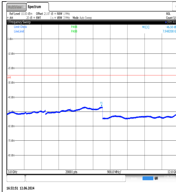
NTNV-N7-PC3-15-15-L-DFT-QPSK-Edge_1RB_Left-3000-12000-Ant1-PASS
