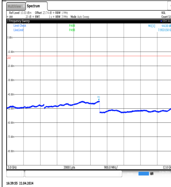
NTNV-N5-PC3-15-10-H-DFT-QPSK-Edge_1RB_Left-3000-12000-Ant1-PASS
