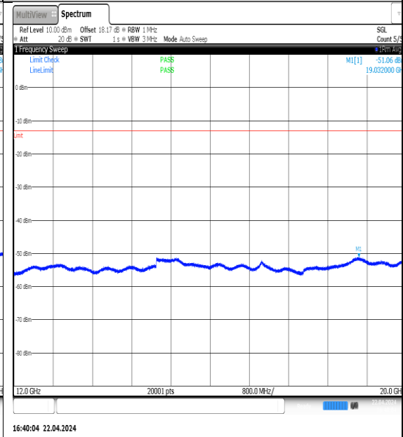
NTNV-N5-PC3-15-10-H-DFT-QPSK-Edge_1RB_Left-12000-20000-Ant1-PASS
