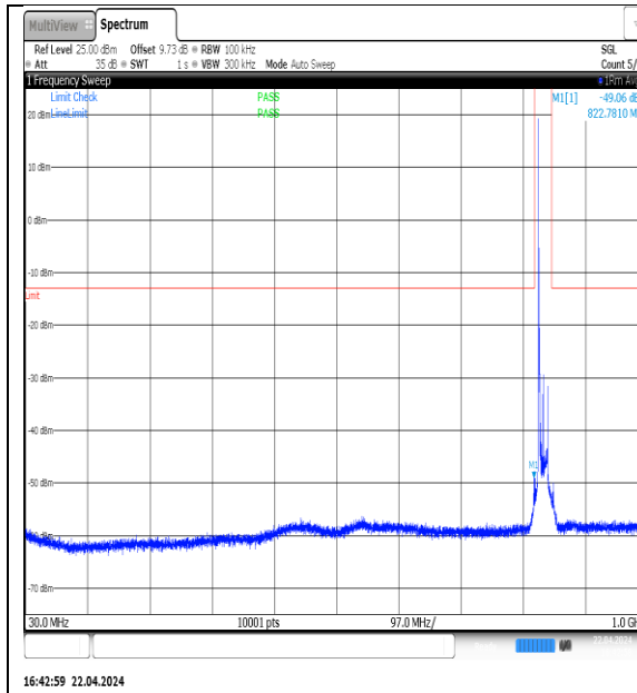
NTNV-N5-PC3-15-15-M-DFT-QPSK-Edge_1RB_Left-30-1000-Ant1-PASS
