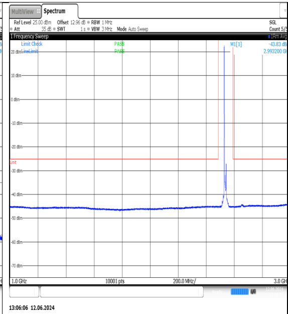
NTNV-N7-PC3-15-15-M-DFT-QPSK-Edge_1RB_Left-1000-3000-Ant1-PASS
