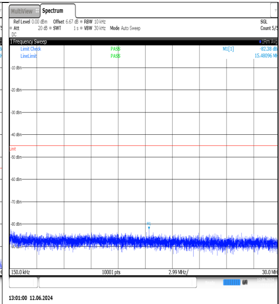
NTNV-N7-PC3-15-5-H-DFT-QPSK- Edge_1RB_Left-0.15-30-Ant1-PASS
