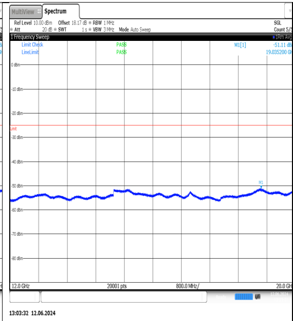
NTVN-N7-PC3-15-10-M-DFT-QPSK-Edge_1RB_Left-12000-20000-Ant1-PASS
