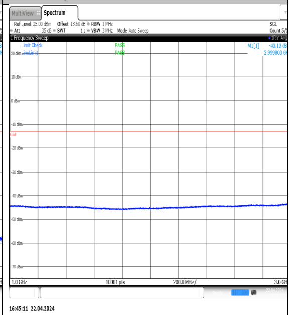
NTNV-N5-PC3-15-15-H-DFT-QPSK- Edge_1RB_Left-1000-3000-Ant1-PASS
