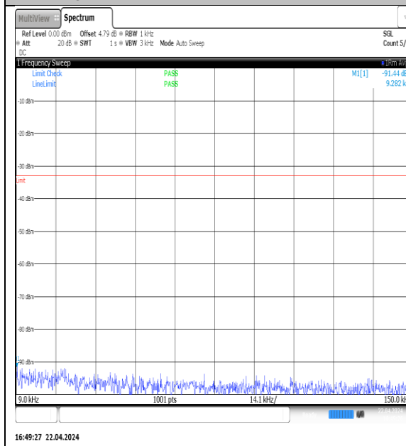
NTNV-N5-PC3-15-20-H-DFT-QPSK-Edge_1RB_Left-0.009-0.15-Ant1-PASS
