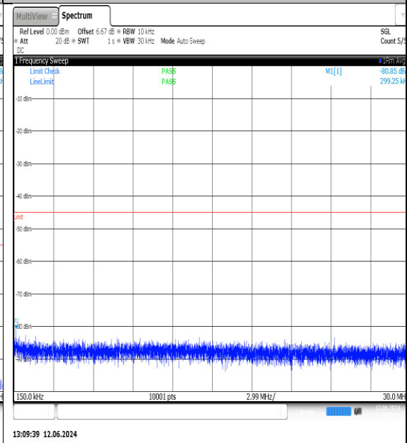
NTNV-N7-PC3-15-20-H-DFT-QPSK-Edge_1RB_Left-0.15-30-Ant1-PASS
