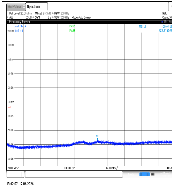
NTNV-N7-PC3-15-10-L-DFT-QPSK-Edge_1RB_Left-30-1000-Ant1-PASS
