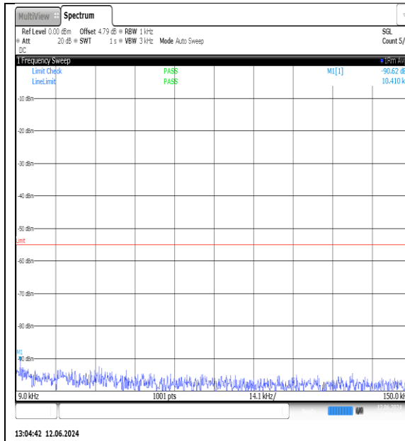
NTNV-N7-PC3-15-15-L-DFT-QPSK-Edge_1RB_Left-0.009-0.15-Ant1-PASS
