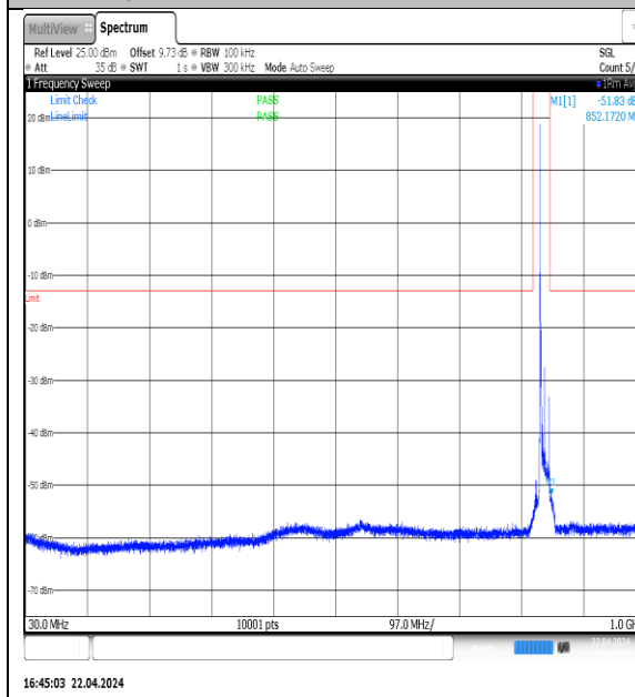
NTNV-N5-PC3-15-15-H-DFT-QPSK- Edge_1RB_Left-30-1000-Ant1-PASS
