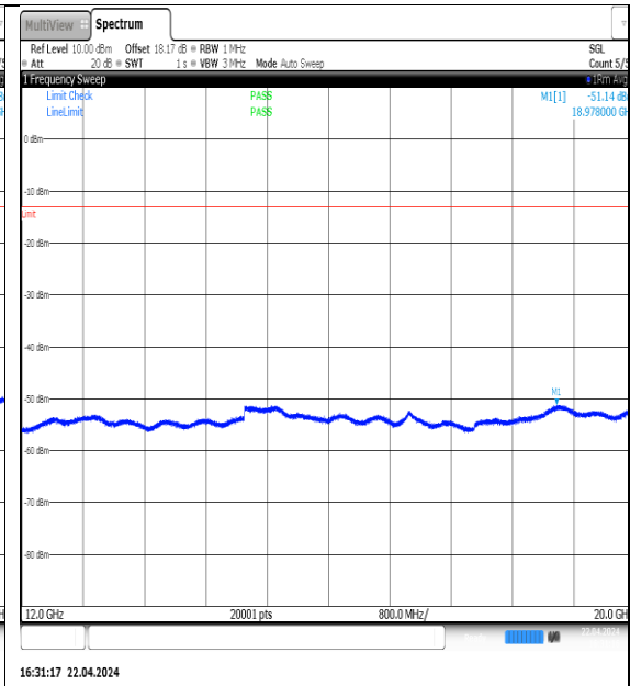
NTNV-N5-PC3-15-5-L-DFT-QPSK-Edge_1RB_Left-12000-20000-Ant1-PASS
