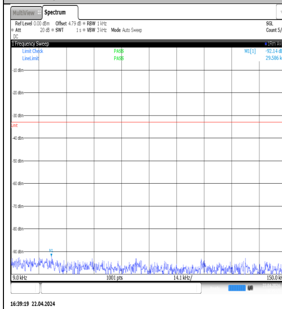
NTNV-N5-PC3-15-10-H-DFT-QPSK- Edge_1RB_Left-0.009-0.15-Ant1-PASS
