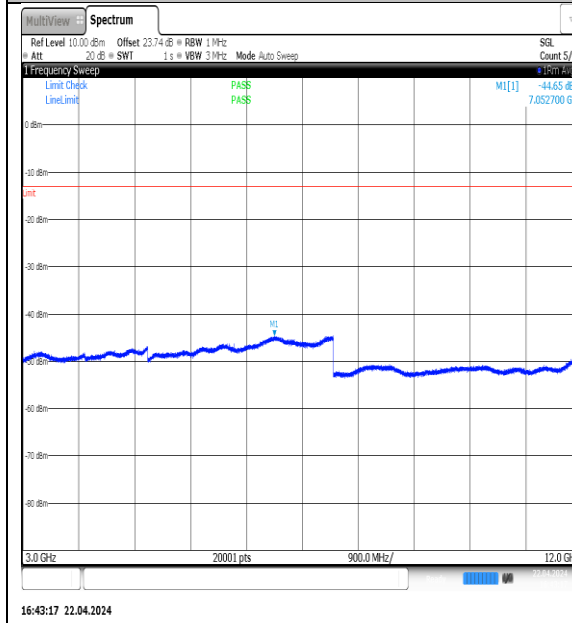
NTNV-N5-PC3-15-15-M-DFT-QPSK-Edge_1RB_Left-3000-12000-Ant1-PASS
