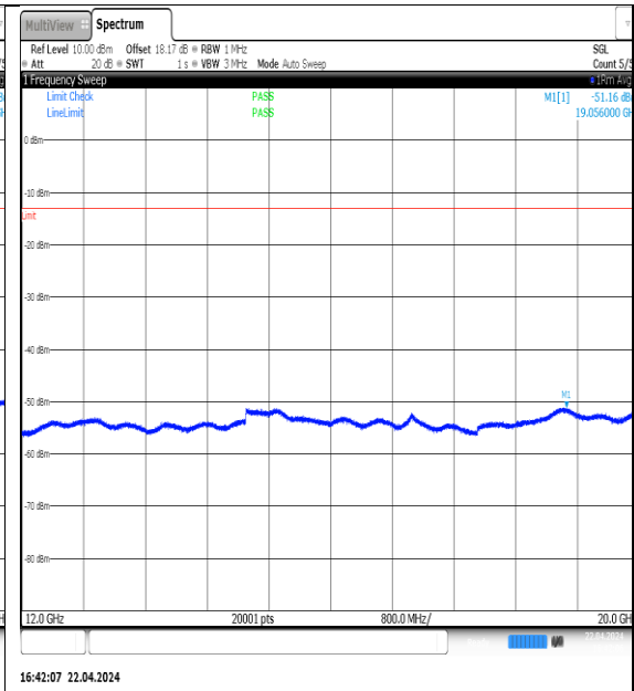
NTN-N5-PC3-15-15-L-DFT-QPSK-Edge_1RB_Left-12000-20000-Ant1-PASS
