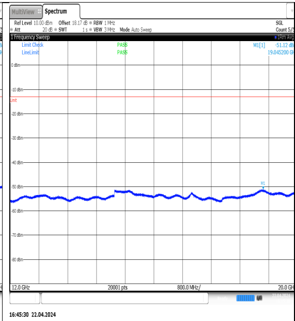
NTNV-N5-PC3-15-15-H-DFT-QPSK-Edge_1RB_Left-12000-20000-Ant1-PASS
