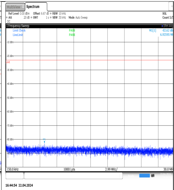
NTNV-N5-PC3-15-15-H-DFT-QPSK- Edge_1RB_Left-0.15-30-Ant1-PASS
