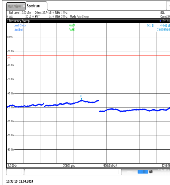
NTNV-N5-PC3-15-5-M-DFT-QPSK- Edge_1RB_Left-3000-12000-Ant1-PASS
