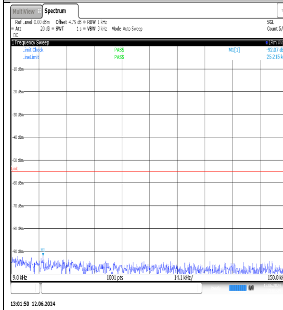
NTNV-N7-PC3-15-10-L-DFT-QPSK-Edge_1RB_Left-0.009-0.15-Ant1-PASS
