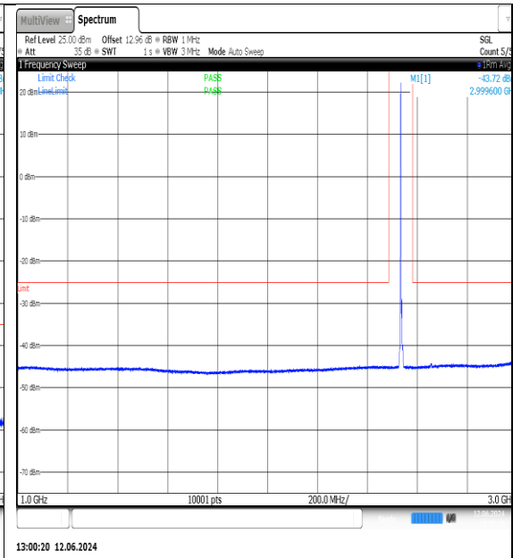
NTNV-N7-PC3-15-5-M-DFT-QPSK-Edge_1RB_Left-1000-3000-Ant1-PASS
