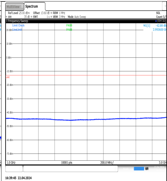
NTNV-N5-PC3-15-10-H-DFT-QPSK-Edge_1RB_Left-1000-3000-Ant1-PASS
