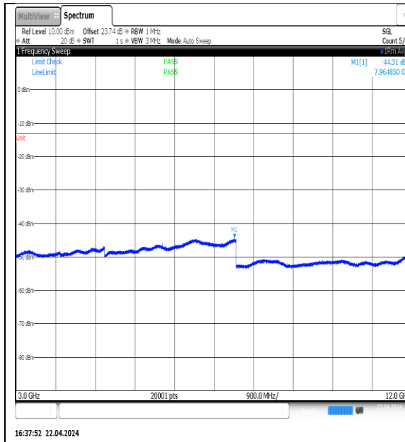
NTNV-N5-PC3-15-10-M-DFT-QPSK- Edge_1RB_Left-3000-12000-Ant1-PASS
