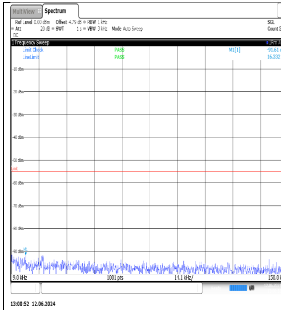
NTNV-N7-PC3-15-5-H-DFT-QPSK- Edge_1RB_Left-0.009-0.15-Ant1-PASS
