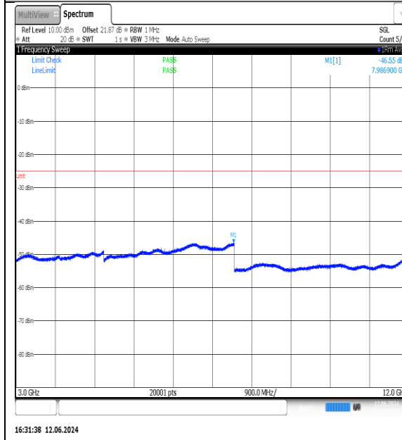
NTNV-N7-PC3-15-5-M-DFT-QPSK-Edge_1RB_Left-3000-12000-Ant1-PASS
