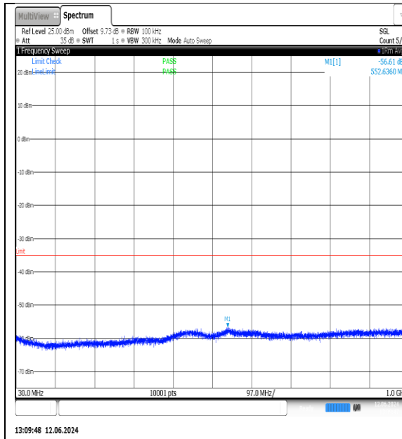
NTNV-N7-PC3-15-20-H-DFT-QPSK-Edge_1RB_Left-30-1000-Ant1-PASS
