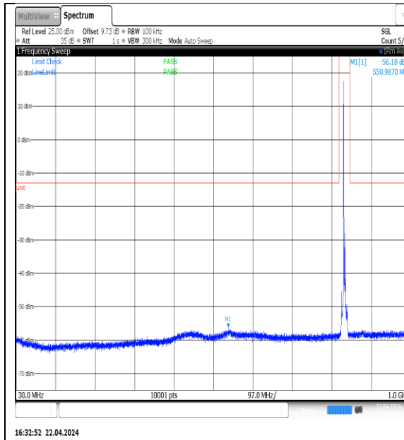
NTNV-N5-PC3-15-5-M-DFT-QPSK- Edge_1RB_Left-30-1000-Ant1-PASS
