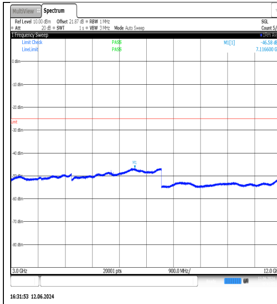
NTNV-N7-PC3-15-5-H-DFT-QPSK-Edge_1RB_Left-3000-12000-Ant1-PASS
