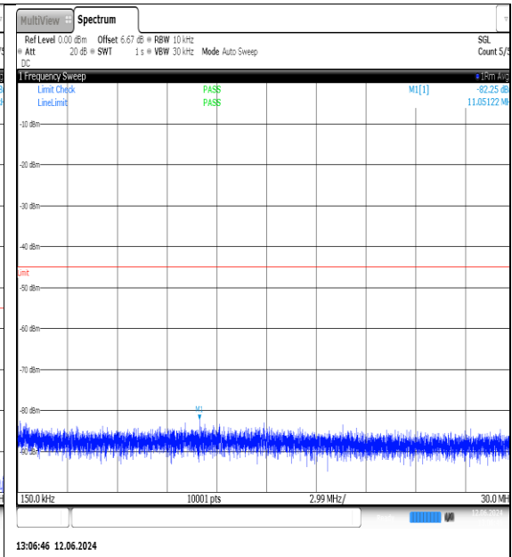
NTN-N7-PC3-15-15-H-DFT-QPSK-Edge_1RB_Left-0.15-30-Ant1-PASS
