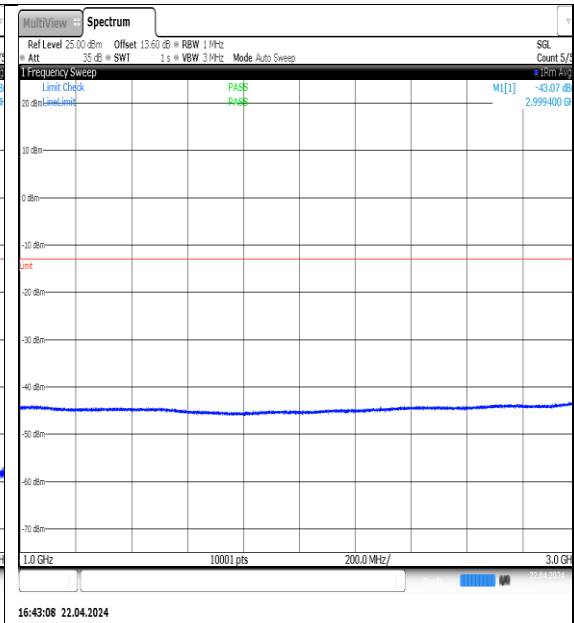
NTNV-N5-PC3-15-15-M-DFT-QPSK-Edge_1RB_Left-1000-3000-Ant1-PASS
