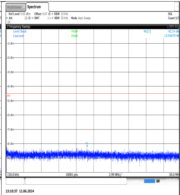
NTNV-N7-PC3-15-25-L-DFT-QPSK- Edge_1RB_Left-0.15-30-Ant1-PASS
