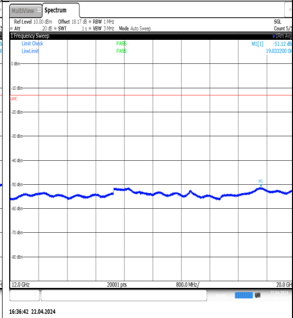
NTNV-N5-PC3-15-10-L-DFT-QPSK-Edge_1RB_Left-12000-20000-Ant1-PASS
