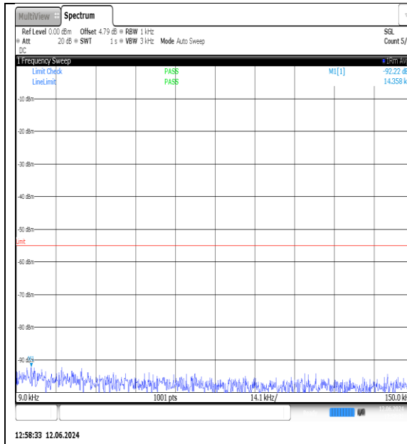
NTNV-N7-PC3-15-5-L-DFT-QPSK- Edge_1RB_Left-0.009-0.15-Ant1-PASS
