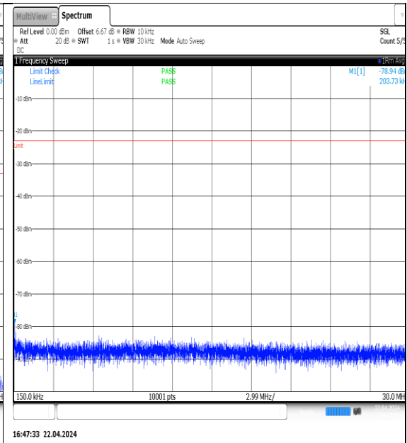
NTNV-N5-PC3-15-20-M-DFT-QPSK- Edge_1RB_Left-0.15-30-Ant1-PASS
