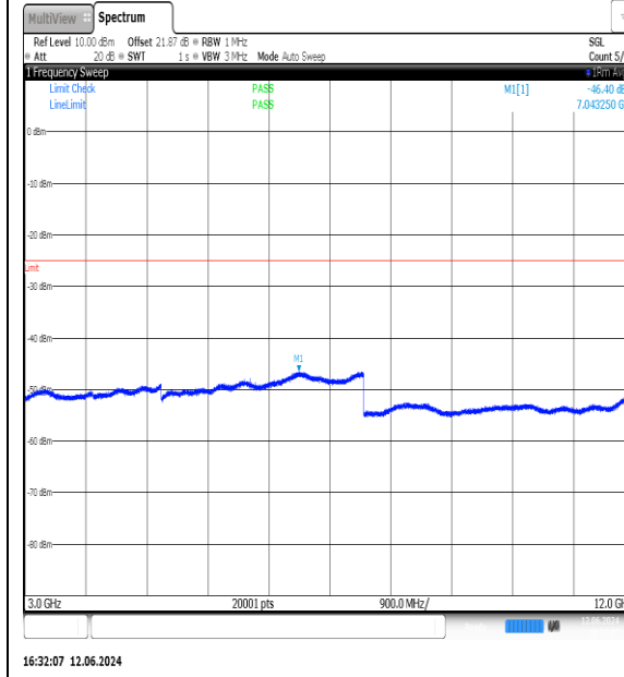
NTNV-N7-PC3-15-10-L-DFT-QPSK-Edge_1RB_Left-3000-12000-Ant1-PASS
