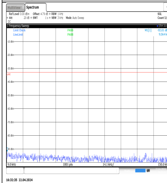
NTNV-N5-PC3-15-5-M-DFT-QPSK-Edge_1RB_Left-0.009-0.15-Ant1-PASS
