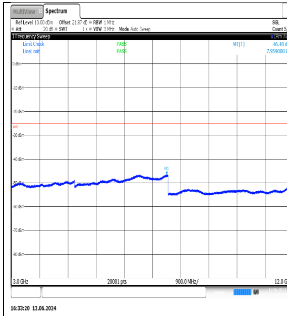
NTN-N7-PC3-15-15-H-DFT-QPSK-Edge_1RB_Left-3000-12000-Ant1-PASS
