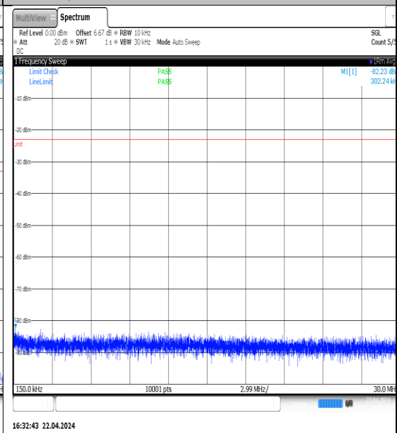
NTNV-N5-PC3-15-5-M-DFT-QPSK-Edge_1RB_Left-0.15-30-Ant1-PASS
