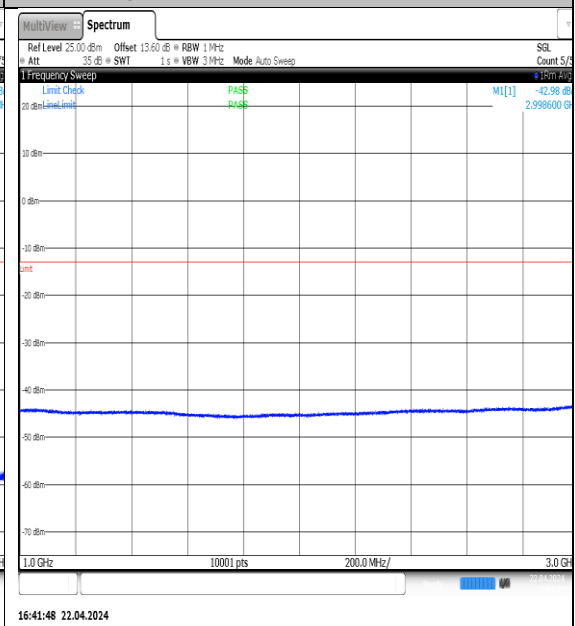
NTNV-N5-PC3-15-15-L-DFT-QPSK- Edge_1RB_Left-1000-3000-Ant1-PASS
