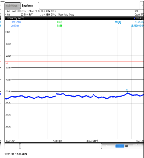
NTNV-N7-PC3-15-5-H-DFT-QPSK-Edge_1RB_Left-12000-20000-Ant1-PASS
