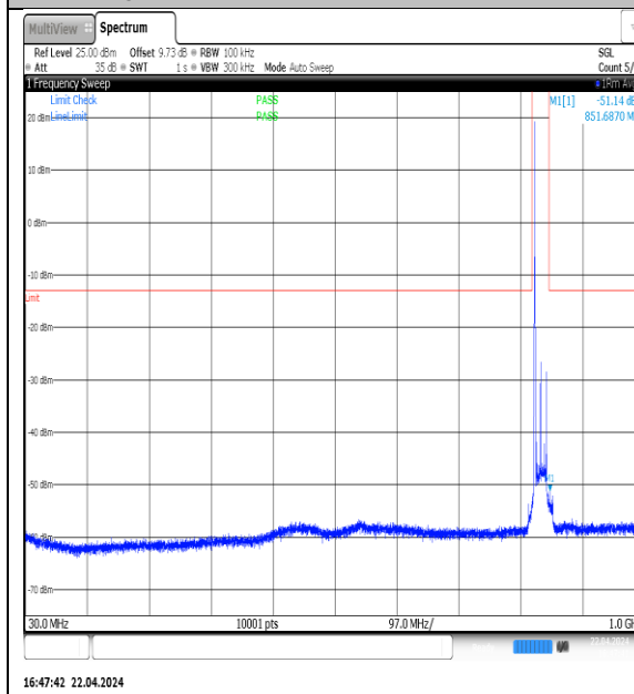
NTNV-N5-PC3-15-20-M-DFT-QPSK- Edge_1RB_Left-30-1000-Ant1-PASS
