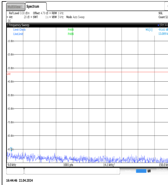
NTNV-N5-PC3-15-15-H-DFT-QPSK- Edge_1RB_Left-0.009-0.15-Ant1-PASS
