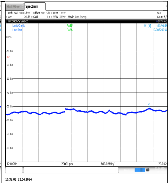
NTNV-N5-PC3-15-10-M-DFT-QPSK- Edge_1RB_Left-12000-20000-Ant1-PASS
