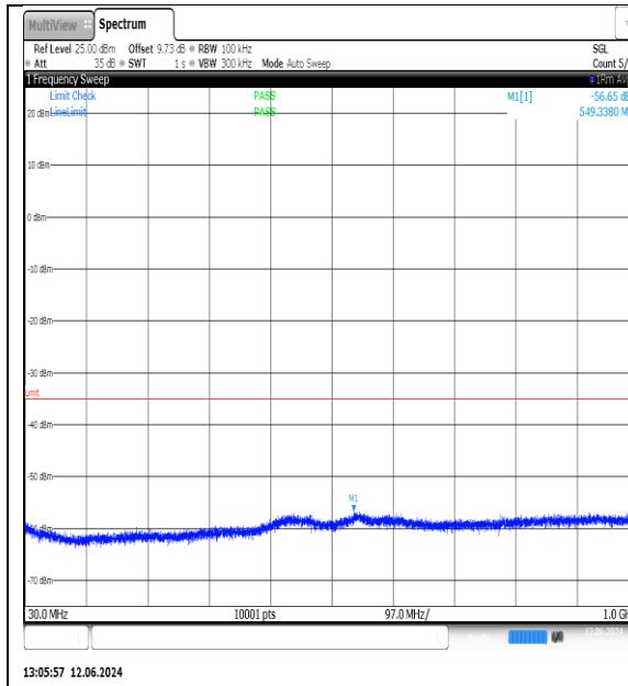
NTNV-N7-PC3-15-15-M-DFT-QPSK-Edge_1RB_Left-30-1000-Ant1-PASS
