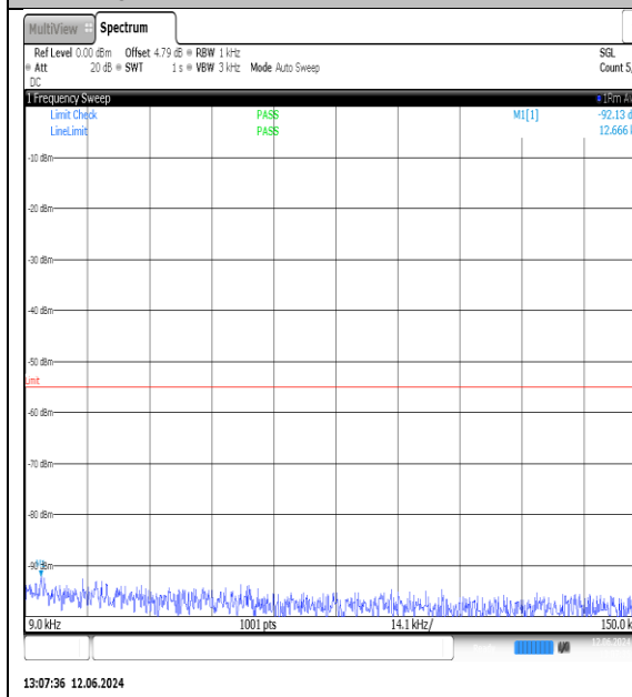
NTN-N7-PC3-15-20-L-DFT-QPSK-Edge_1RB_Left-0.009-0.15-Ant1-PASS
