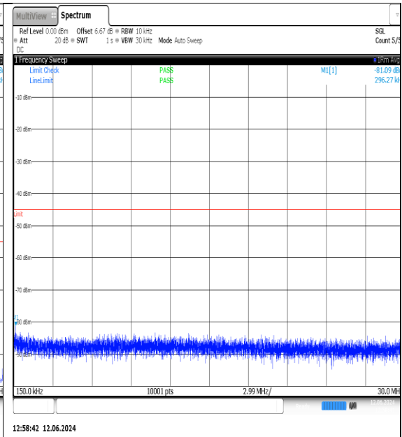
NTNV-N7-PC3-15-5-L-DFT-QPSK- Edge_1RB_Left-0.15-30-Ant1-PASS
