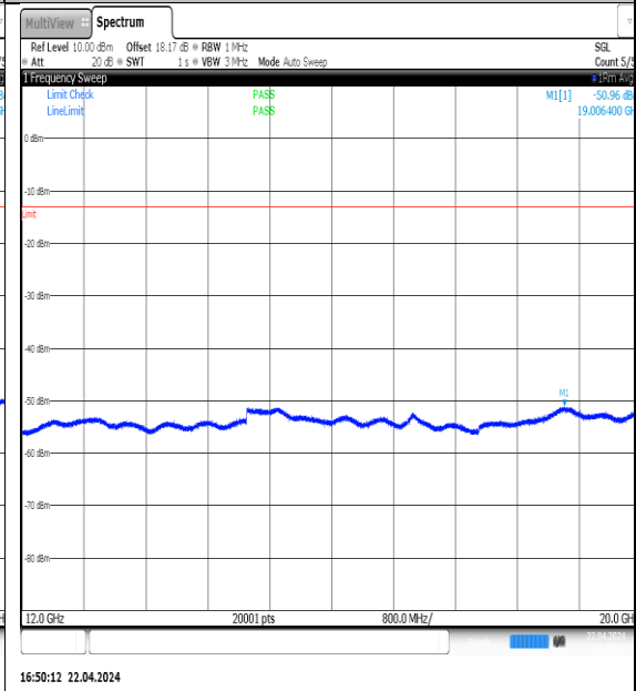
NTNV-N5-PC3-15-20-H-DFT-QPSK-Edge_1RB_Left-12000-20000-Ant1-PASS
