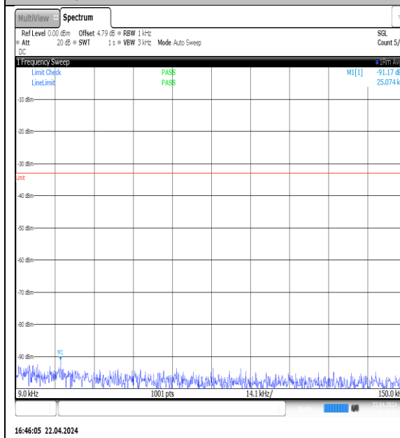
NTNV-N5-PC3-15-20-L-DFT-QPSK-Edge_1RB_Left-0.009-0.15-Ant1-PASS
