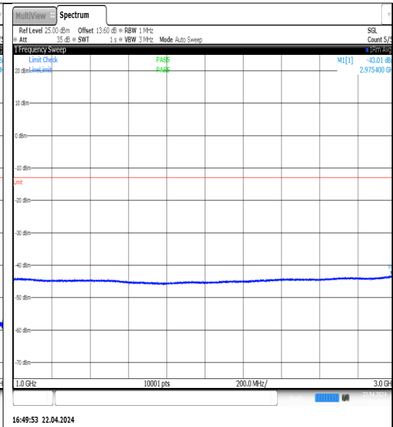
NTNV-N5-PC3-15-20-H-DFT-QPSK-Edge_1RB_Left-1000-3000-Ant1-PASS
