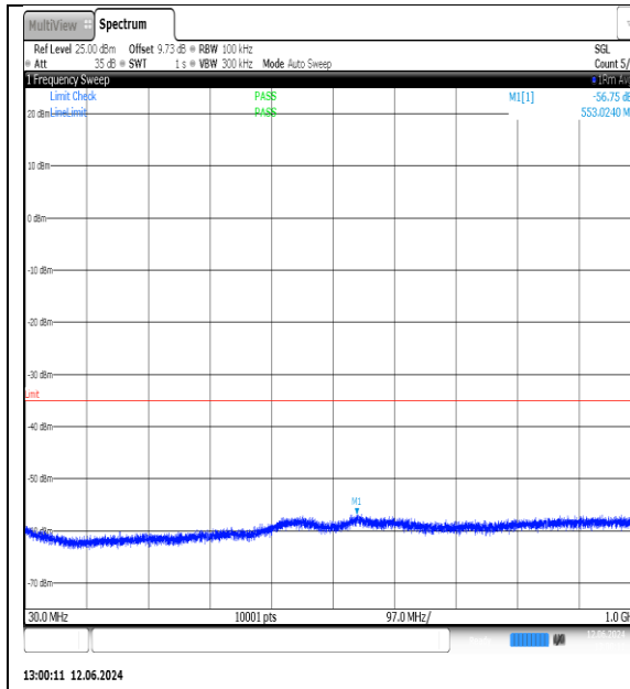
NTNV-N7-PC3-15-5-M-DFT-QPSK-Edge_1RB_Left-30-1000-Ant1-PASS
