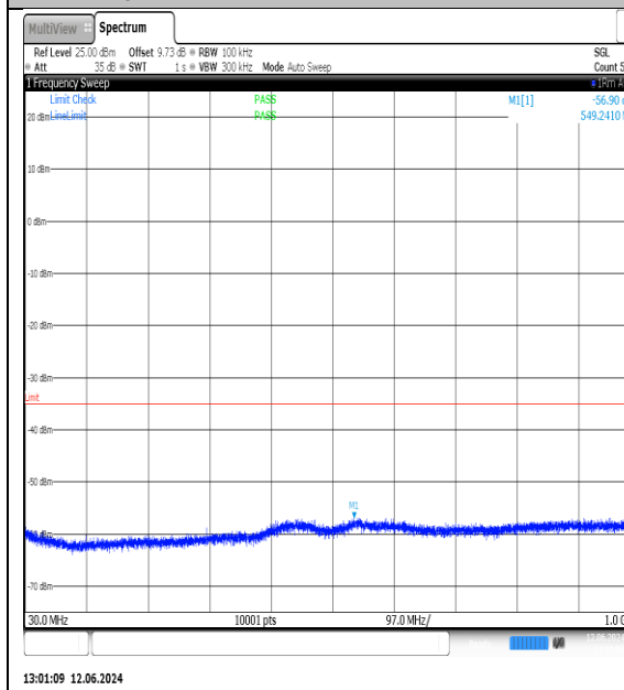
NTNV-N7-PC3-15-5-H-DFT-QPSK- Edge_1RB_Left-30-1000-Ant1-PASS
