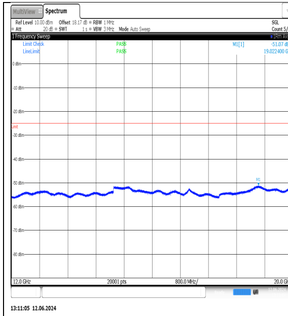
NTN-N7-PC3-15-25-L-DFT-QPSK- Edge_1RB_Left-12000-20000-Ant1-PASS
