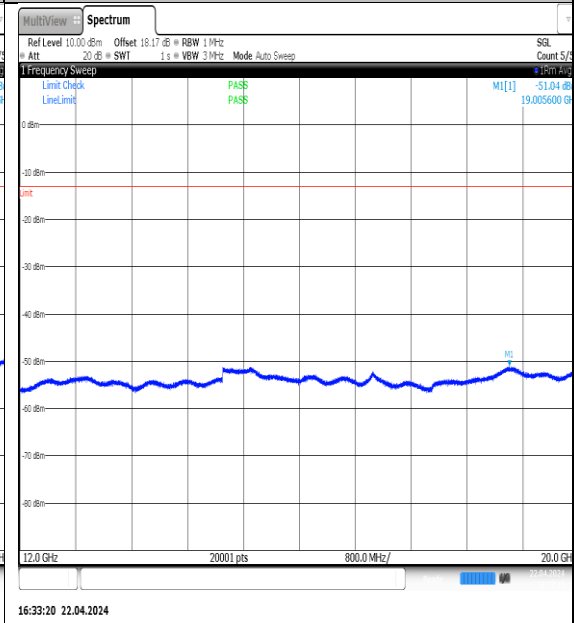
NTNV-N5-PC3-15-5-M-DFT-QPSK- Edge_1RB_Left-12000-20000-Ant1-PASS
