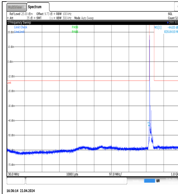
NTNV-N5-PC3-15-10-L-DFT-QPSK-Edge_1RB_Left-30-1000-Ant1-PASS
