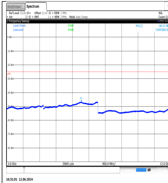
NTN-N7-PC3-15-5-L-DFT-QPSK-Edge_1RB_Left-3000-12000-Ant1-PASS
