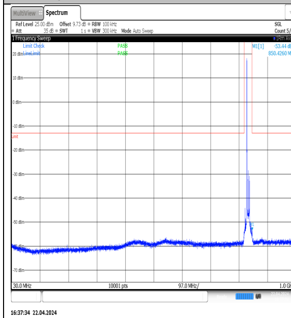
NTNV-N5-PC3-15-10-M-DFT-QPSK- Edge_1RB_Left-30-1000-Ant1-PASS
