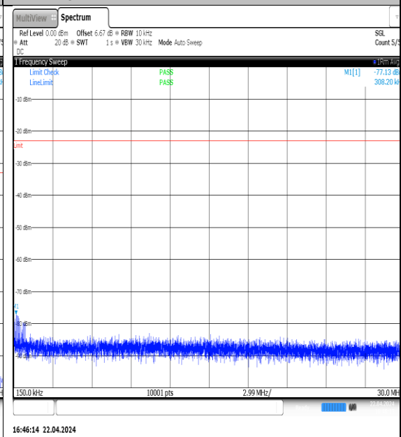
NTNV-N5-PC3-15-20-L-DFT-QPSK-Edge_1RB_Left-0.15-30-Ant1-PASS
