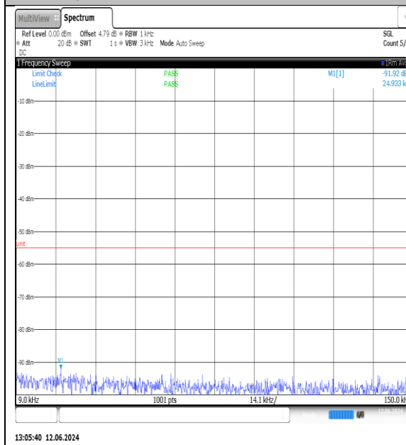
NTNV-N7-PC3-15-15-M-DFT-QPSK-Edge_1RB_Left-0.009-0.15-Ant1-PASS
