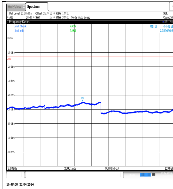
NTNV-N5-PC3-15-20-M-DFT-QPSK-Edge_1RB_Left-3000-12000-Ant1-PASS
