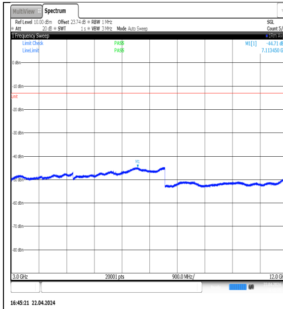
NTNV-N5-PC3-15-15-H-DFT-QPSK-Edge_1RB_Left-3000-12000-Ant1-PASS
