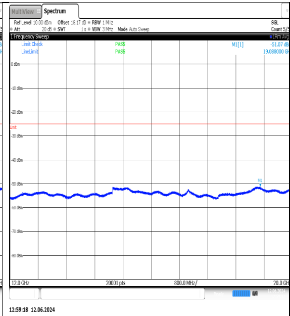
NTN-N7-PC3-15-5-L-DFT-QPSK-Edge_1RB_Left-12000-20000-Ant1-PASS
