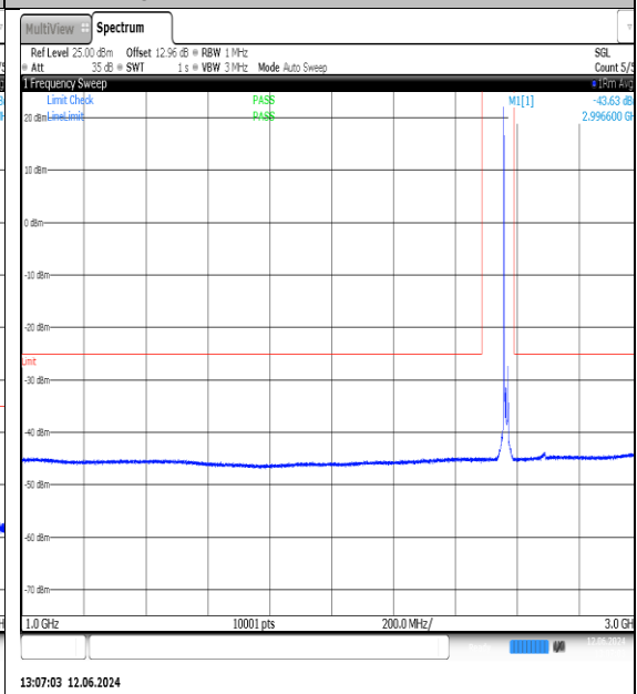
NTN-N7-PC3-15-15-H-DFT-QPSK-Edge_1RB_Left-1000-3000-Ant1-PASS
