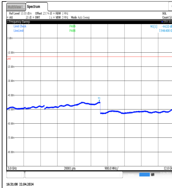
NTNV-N5-PC3-15-5-L-DFT-QPSK-Edge_1RB_Left-3000-12000-Ant1-PASS
