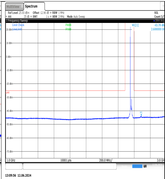
NTNV-N7-PC3-15-20-H-DFT-QPSK-Edge_1RB_Left-1000-3000-Ant1-PASS
