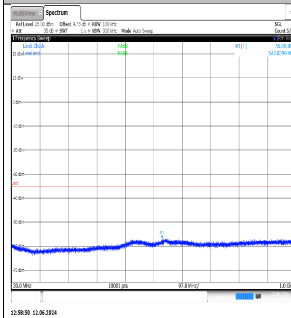
NTNV-N7-PC3-15-5-L-DFT-QPSK- Edge_1RB_Left-30-1000-Ant1-PASS
