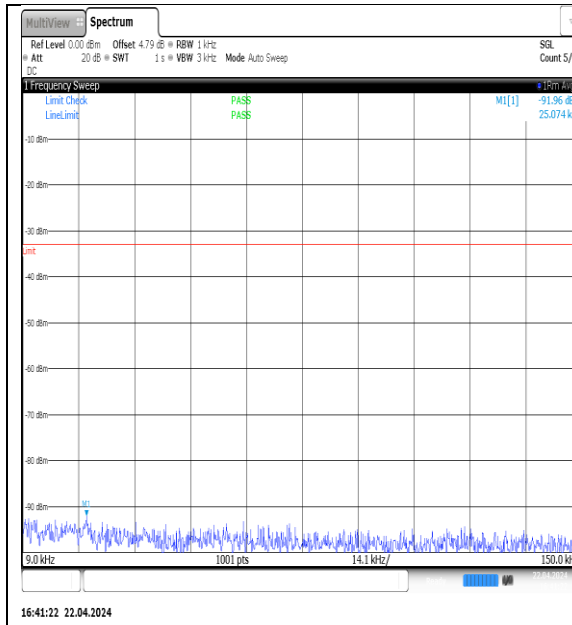
NTNV-N5-PC3-15-15-L-DFT-QPSK- Edge_1RB_Left-0.009-0.15-Ant1-PASS
