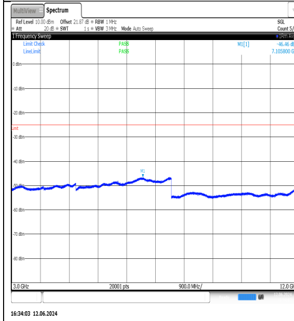
NTNV-N7-PC3-15-20-H-DFT-QPSK-Edge_1RB_Left-3000-12000-Ant1-PASS
