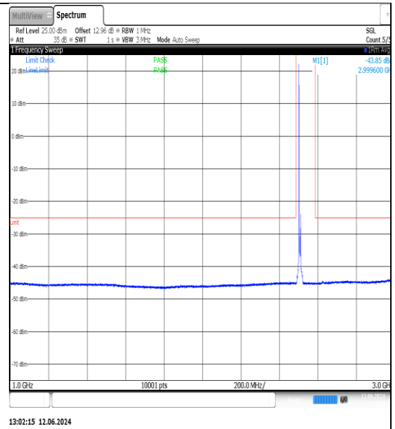
NTNV-N7-PC3-15-10-L-DFT-QPSK-Edge_1RB_Left-1000-3000-Ant1-PASS
