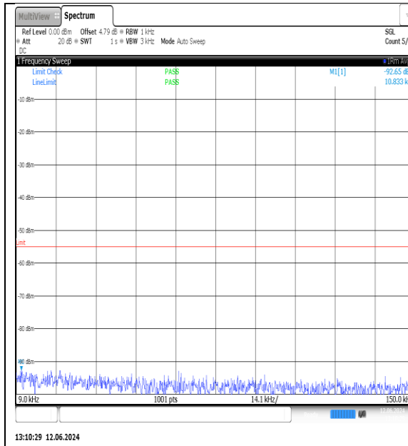
NTNV-N7-PC3-15-25-L-DFT-QPSK- Edge_1RB_Left-0.009-0.15-Ant1-PASS
