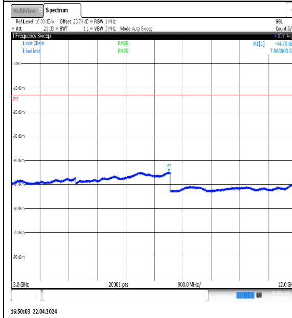
NTNV-N5-PC3-15-20-H-DFT-QPSK-Edge_1RB_Left-3000-12000-Ant1-PASS
