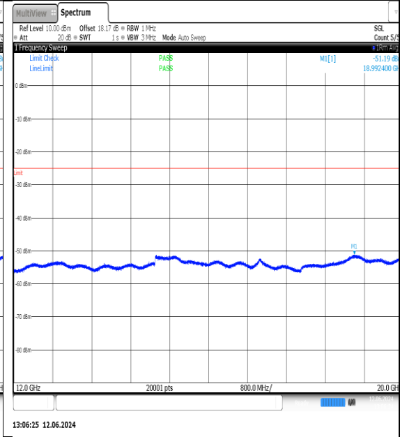
NTNV-N7-PC3-15-15-M-DFT-QPSK-Edge_1RB_Left-12000-20000-Ant1-PASS
