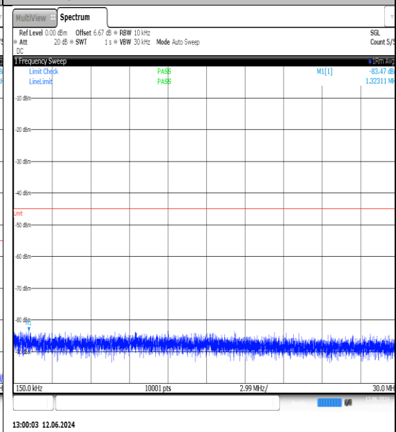
NTN-N7-PC3-15-5-M-DFT-QPSK-Edge_1RB_Left-0.15-30-Ant1-PASS
