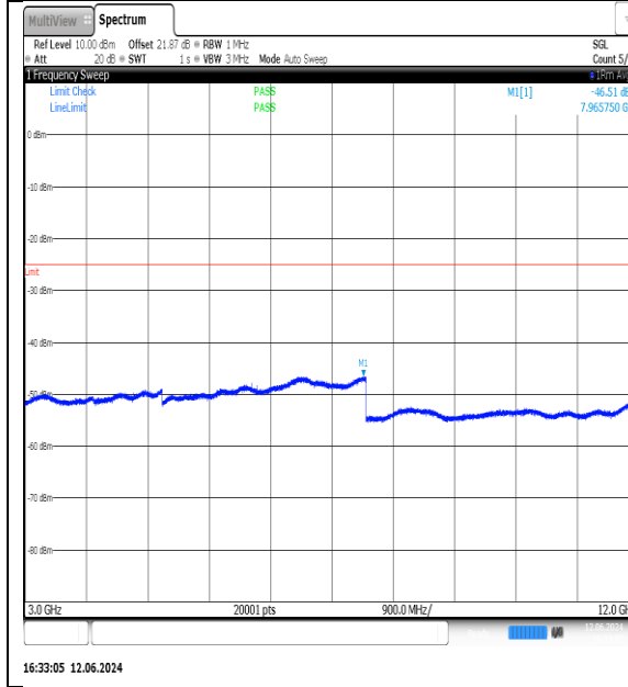
NTNV-N7-PC3-15-15-M-DFT-QPSK-Edge_1RB_Left-3000-12000-Ant1-PASS
