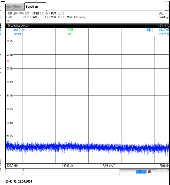
NTNV-N5-PC3-15-15-L-DFT-QPSK- Edge_1RB_Left-0.15-30-Ant1-PASS
