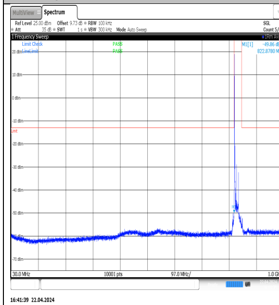
NTNV-N5-PC3-15-15-L-DFT-QPSK- Edge_1RB_Left-30-1000-Ant1-PASS
