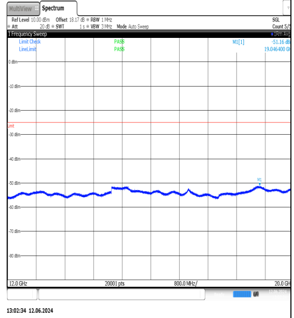
NTNV-N7-PC3-15-10-L-DFT-QPSK-Edge_1RB_Left-12000-20000-Ant1-PASS
