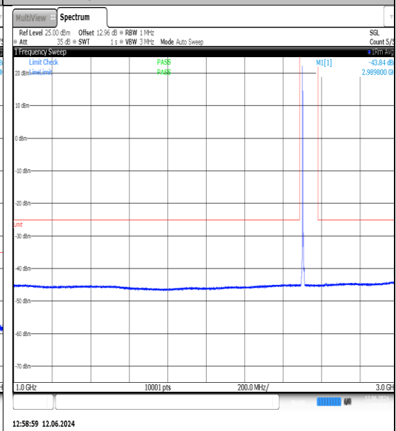
NTNV-N7-PC3-15-5-L-DFT-QPSK- Edge_1RB_Left-1000-3000-Ant1-PASS
