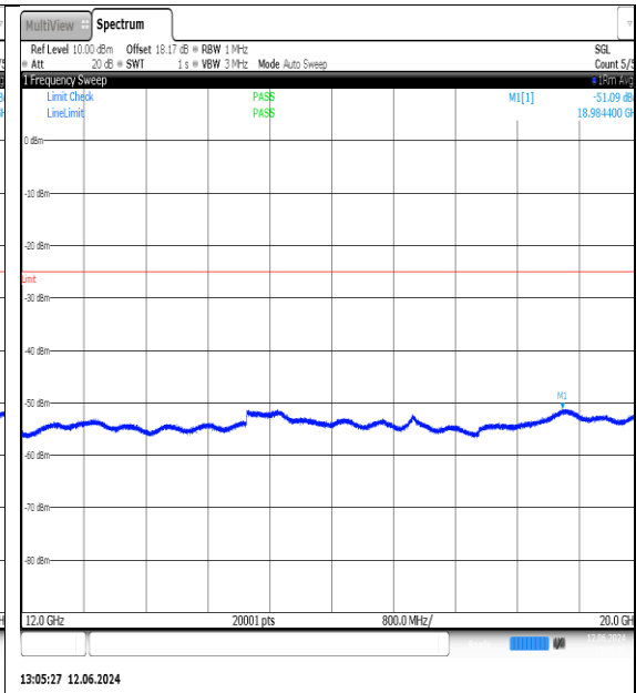
NTNV-N7-PC3-15-15-L-DFT-QPSK-Edge_1RB_Left-12000-20000-Ant1-PASS
