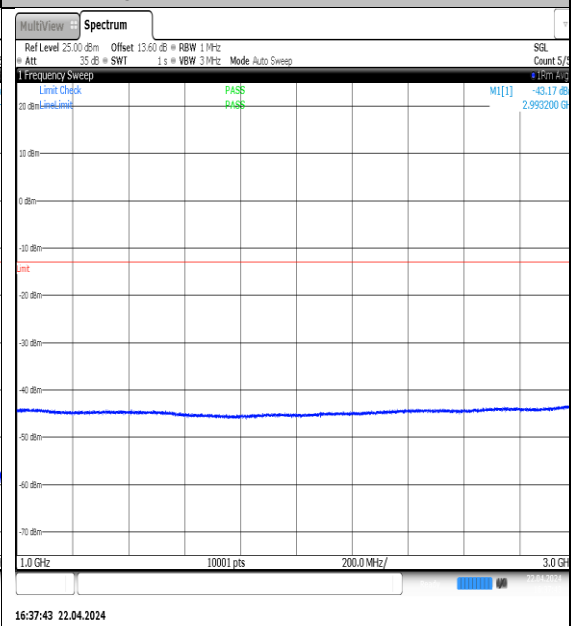
NTNV-N5-PC3-15-10-M-DFT-QPSK- Edge_1RB_Left-1000-3000-Ant1-PASS
