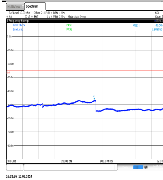
NTNV-N7-PC3-15-10-H-DFT-QPSK-Edge_1RB_Left-3000-12000-Ant1-PASS
