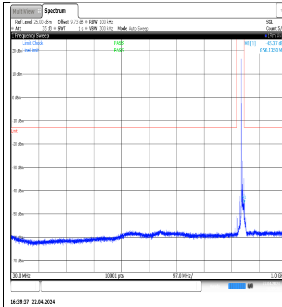
NTNV-N5-PC3-15-10-H-DFT-QPSK-Edge_1RB_Left-30-1000-Ant1-PASS
