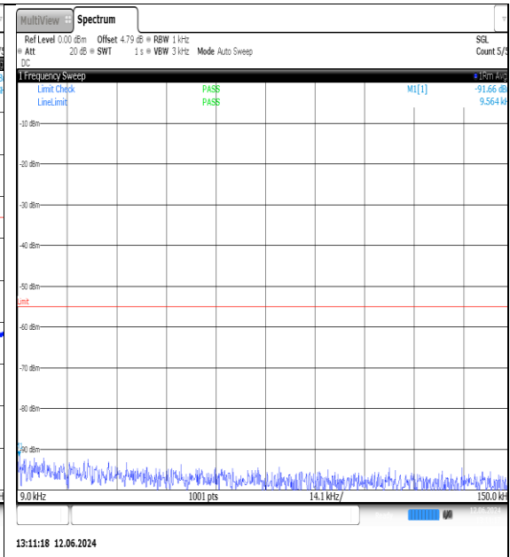
NTN-N7-PC3-15-25-M-DFT-QPSK- Edge_1RB_Left-0.009-0.15-Ant1-PASS
