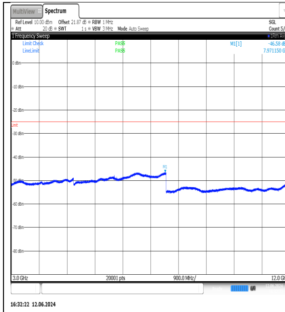
NTVN-N7-PC3-15-10-M-DFT-QPSK-Edge_1RB_Left-3000-12000-Ant1-PASS
