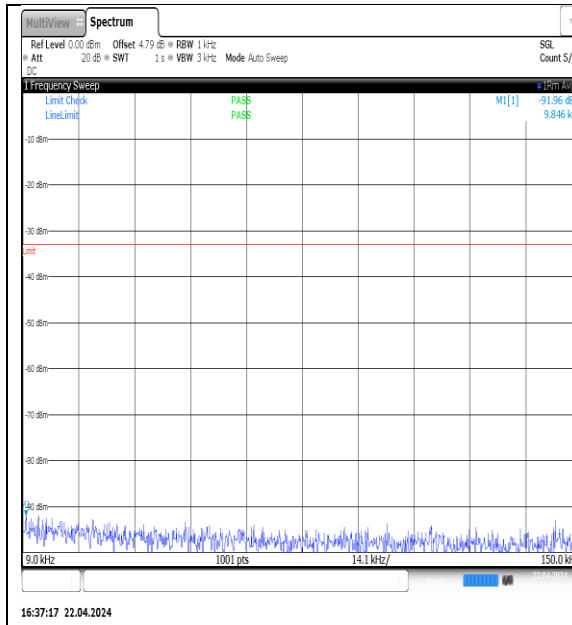
NTNV-N5-PC3-15-10-M-DFT-QPSK- Edge_1RB_Left-0.009-0.15-Ant1-PASS
