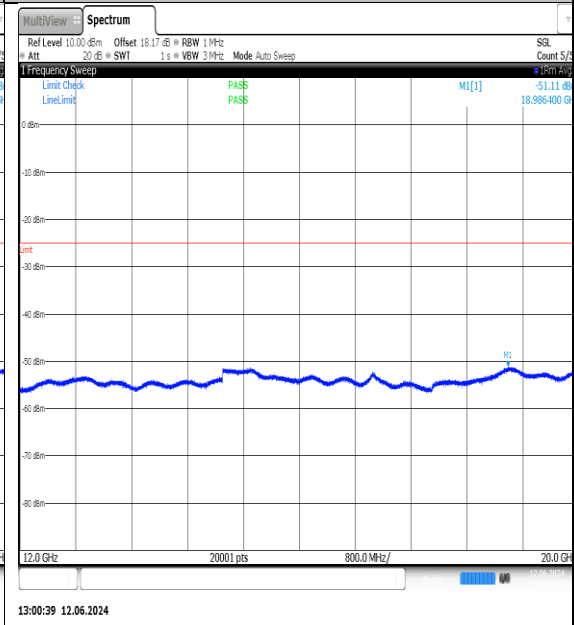
NTNV-N7-PC3-15-5-M-DFT-QPSK-Edge_1RB_Left-12000-20000-Ant1-PASS
