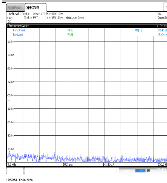
NTN-N7-PC3-15-5-M-DFT-QPSK-Edge_1RB_Left-0.009-0.15-Ant1-PASS
