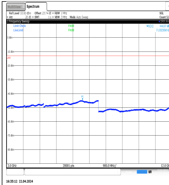
NTN-N5-PC3-15-5-H-DFT-QPSK- Edge_1RB_Left-3000-12000-Ant1-PASS
