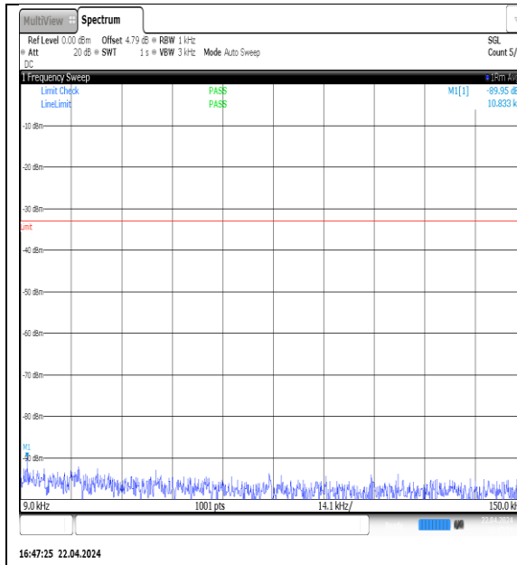
NTNV-N5-PC3-15-20-M-DFT-QPSK- Edge_1RB_Left-0.009-0.15-Ant1-PASS
