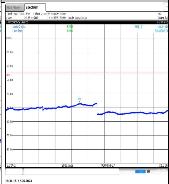
NTNV-N7-PC3-15-25-L-DFT-QPSK- Edge_1RB_Left-3000-12000-Ant1-PASS
