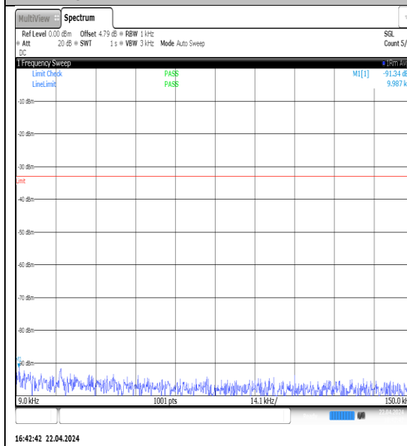
NTN-N5-PC3-15-15-M-DFT-QPSK-Edge_1RB_Left-0.009-0.15-Ant1-PASS
