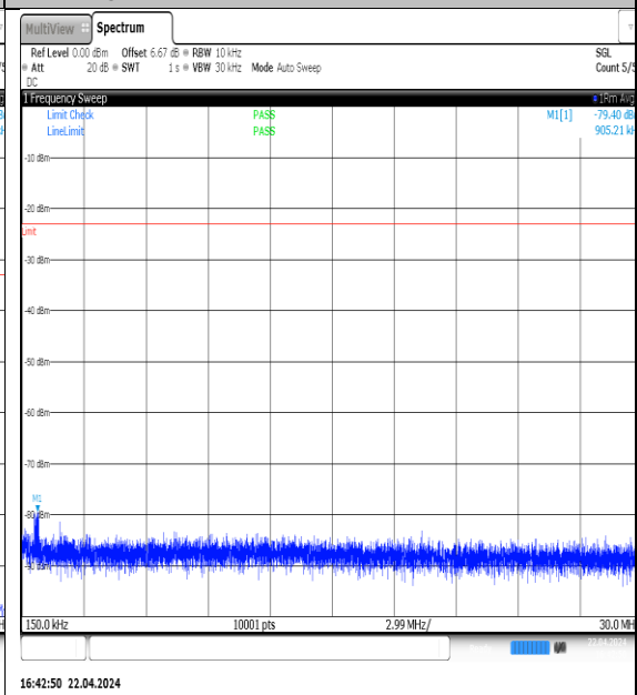
NTN-N5-PC3-15-15-M-DFT-QPSK-Edge_1RB_Left-0.15-30-Ant1-PASS
