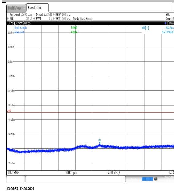
NTN-N7-PC3-15-15-H-DFT-QPSK-Edge_1RB_Left-30-1000-Ant1-PASS
