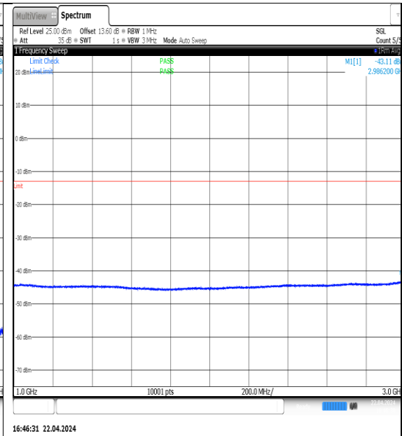
NTNV-N5-PC3-15-20-L-DFT-QPSK-Edge_1RB_Left-1000-3000-Ant1-PASS
