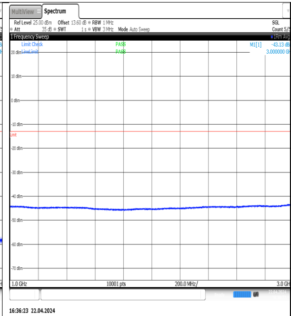
NTNV-N5-PC3-15-10-L-DFT-QPSK-Edge_1RB_Left-1000-3000-Ant1-PASS
