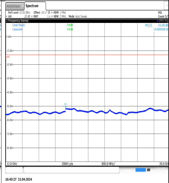
NTNV-N5-PC3-15-15-M-DFT-QPSK-Edge_1RB_Left-12000-20000-Ant1-PASS
