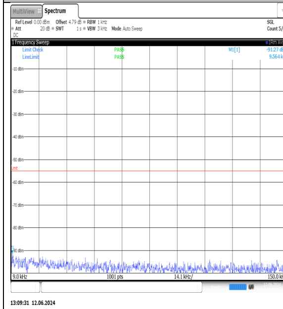
NTNV-N7-PC3-15-20-H-DFT-QPSK-Edge_1RB_Left-0.009-0.15-Ant1-PASS
