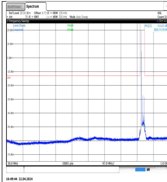
NTNV-N5-PC3-15-20-H-DFT-QPSK-Edge_1RB_Left-30-1000-Ant1-PASS
