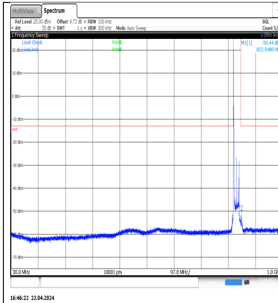
NTNV-N5-PC3-15-20-L-DFT-QPSK-Edge_1RB_Left-30-1000-Ant1-PASS
