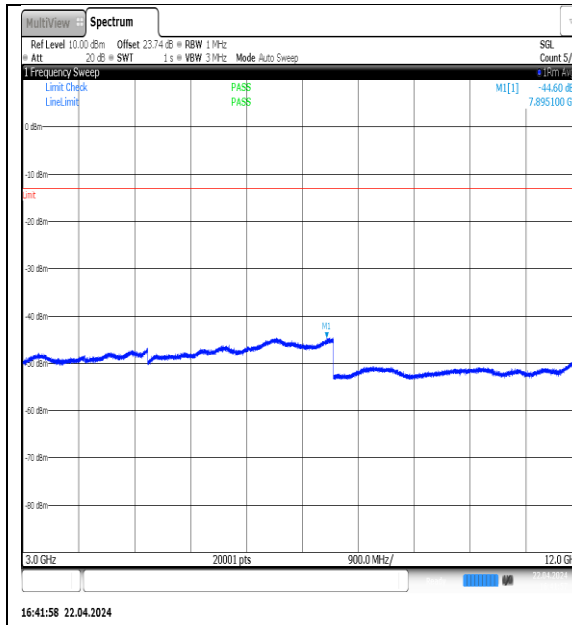
NTN-N5-PC3-15-15-L-DFT-QPSK-Edge_1RB_Left-3000-12000-Ant1-PASS
