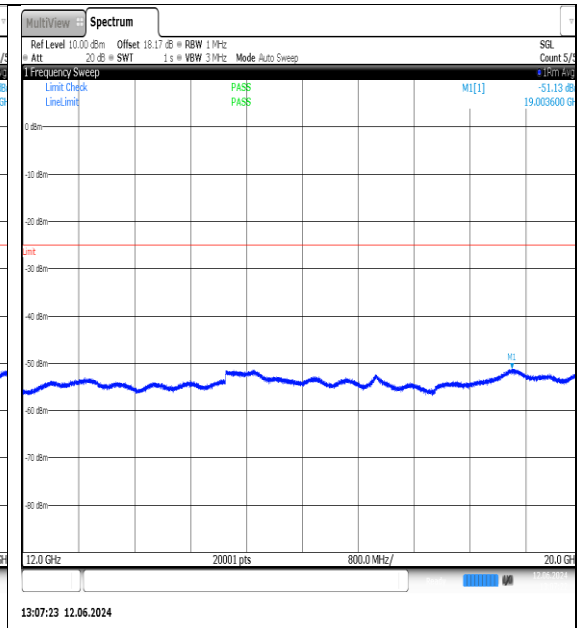
NTN-N7-PC3-15-15-H-DFT-QPSK-Edge_1RB_Left-12000-20000-Ant1-PASS
