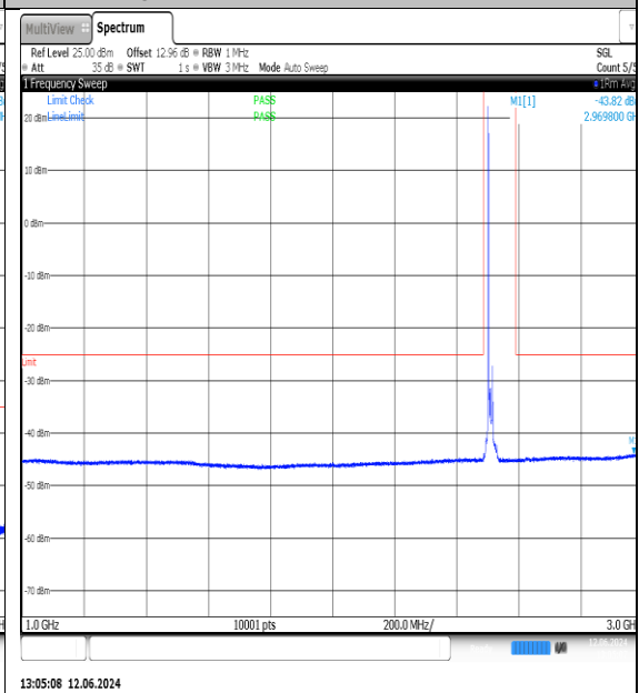
NTNV-N7-PC3-15-15-L-DFT-QPSK-Edge_1RB_Left-1000-3000-Ant1-PASS
