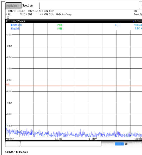
NTVN-N7-PC3-15-10-M-DFT-QPSK-Edge_1RB_Left-0.009-0.15-Ant1-PASS
