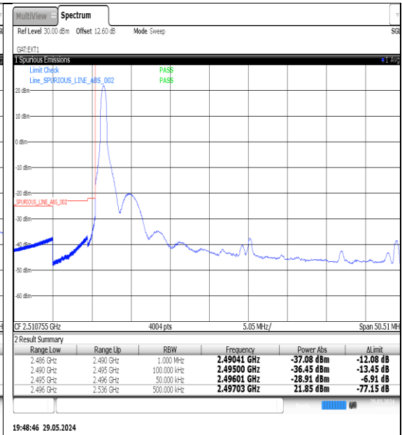
NTNV-N41-PC3-30-40-L-DFT-QPSK-Edge_1RB_Left-Ant1-PASS
