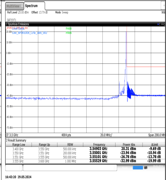
NTNV-N77-3450-3550-PC3-30-10-H-DFT-QPSK-Edge_1RB_Right-Ant1-PASS
