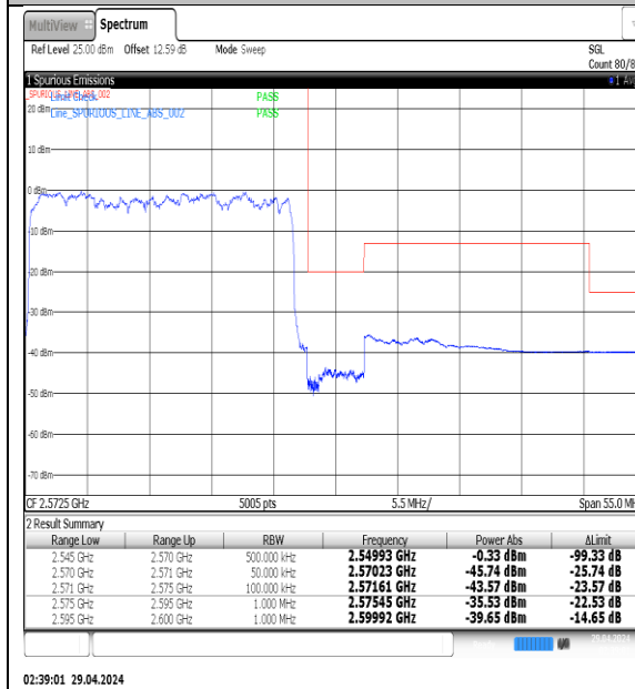
NTNV-N7-PC3-15-25-H-DFT-QPSK-Outter_Full-Ant1-PASS
