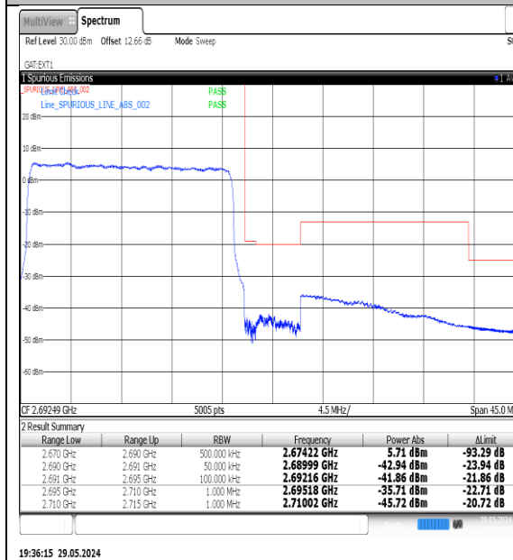
NTNV-N41-PC3-30-20-H-DFT-QPSK-Outter_Full-Ant1-PASS
