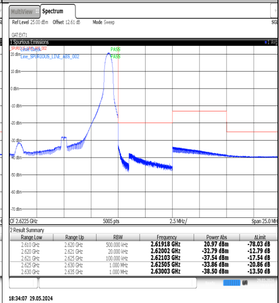
NTNV-N38-PC3-30-10-H-DFT-QPSK-Edge_1RB_Right-Ant1-PASS
