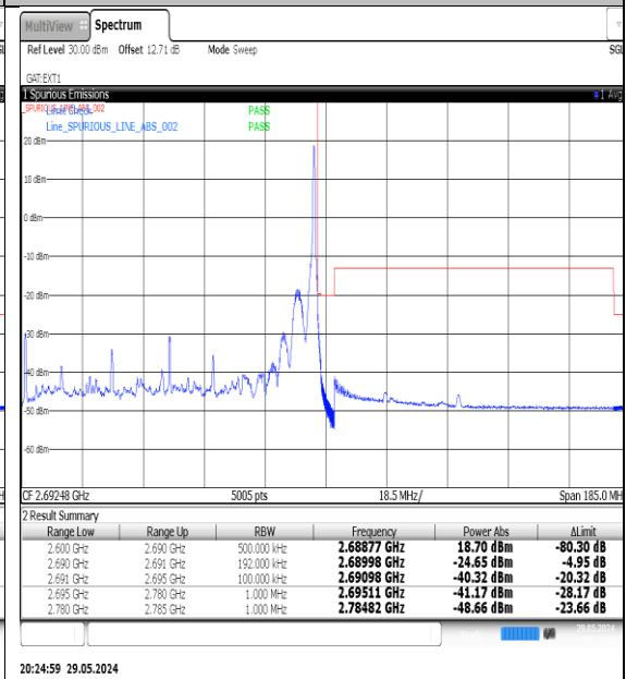
NTNV-N41-PC3-30-90-H-DFT-QPSK-Edge_1RB_Right-Ant1-PASS
