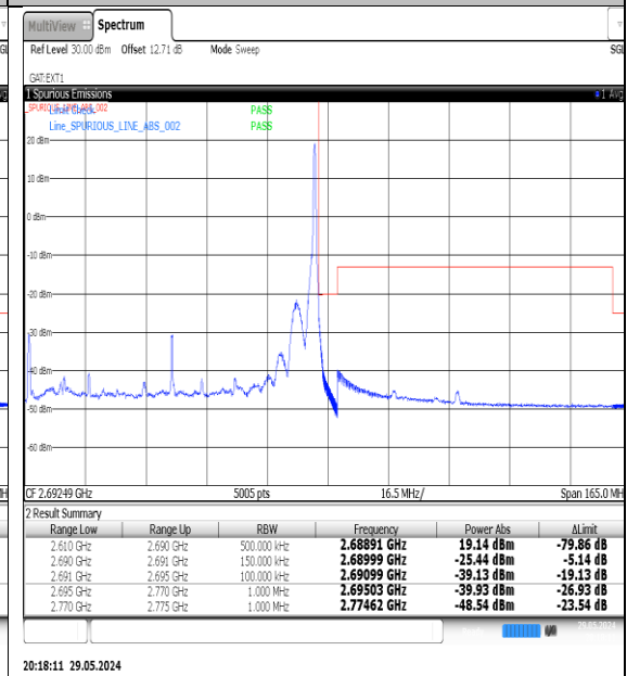
NTNV-N41-PC3-30-80-H-DFT-QPSK-Edge_1RB_Right-Ant1-PASS
