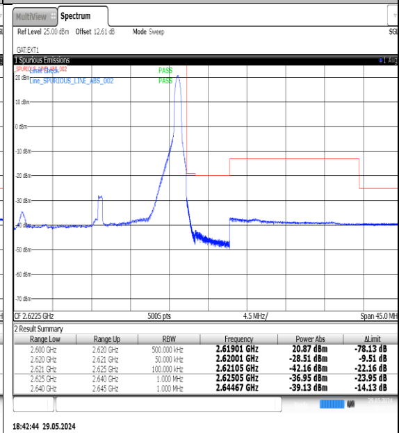
18:42:44 29.05.2024 NTNV-N38-PC3-30-20-H-DFT-QPSK-Edge_1RB_Right-Ant1-PASS
