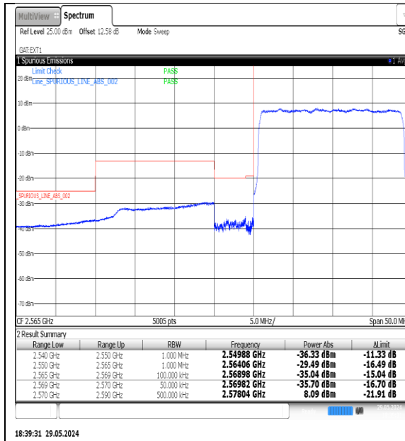
18:39:31 29.05.2024 NTNV-N38-PC3-30-20-L-DFT-QPSK-Outter_Full-Ant1-PASS
