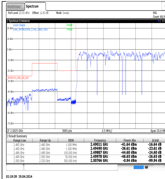
NTNV-N7-PC3-15-25-L-DFT-QPSK-Outter_Full-Ant1-PASS
