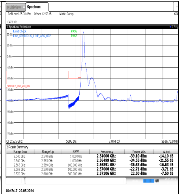
NTNV-N38-PC3-30-40-L-DFT-QPSK-Edge_1RB_Left-Ant1-PASS
