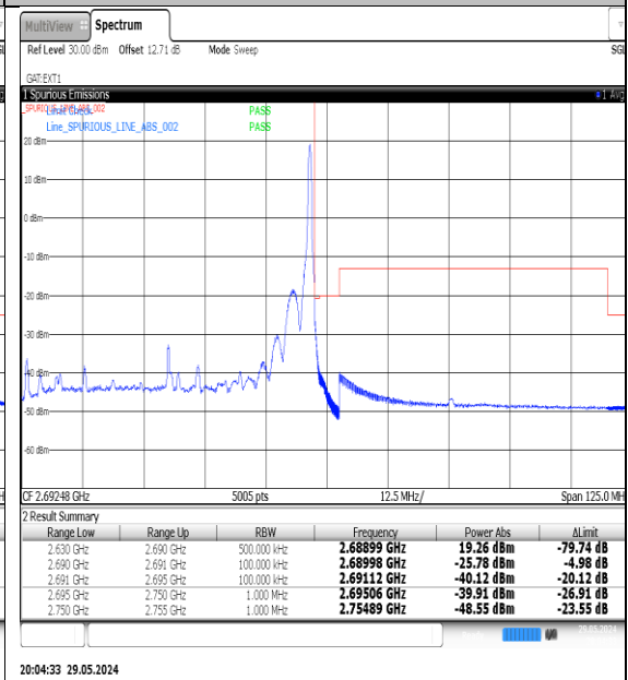
NTNV-N41-PC3-30-60-H-DFT-QPSK-Edge_1RB_Right-Ant1-PASS
