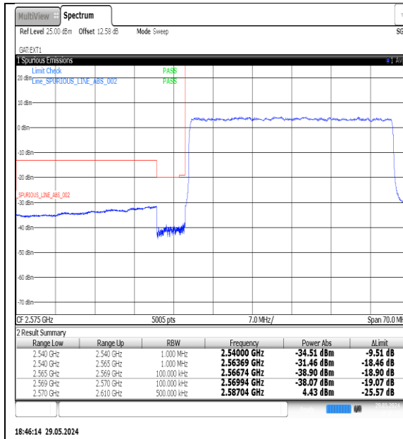
NTNV-N38-PC3-30-40-L-DFT-QPSK-Outter_Full-Ant1-PASS
