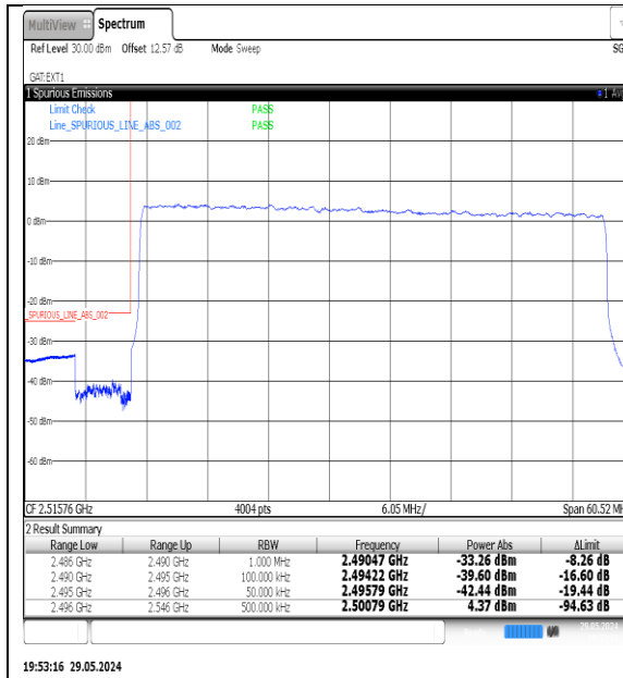
NTNV-N41-PC3-30-50-L-DFT-QPSK-Outter_Full-Ant1-PASS
