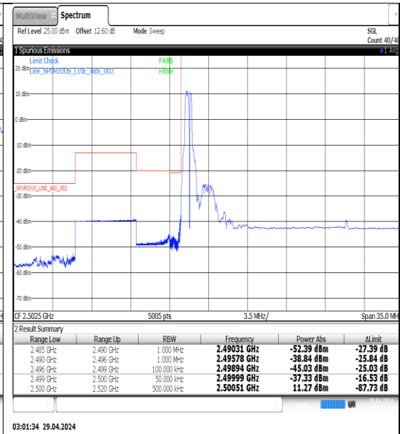
NTNV-N7-PC3-15-30-L-DFT-QPSK-Edge_1RB_Left-Ant1-PASS
