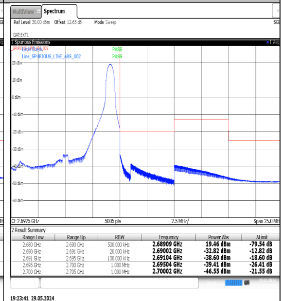
NTNV-N41-PC3-30-10-H-DFT-QPSK-Edge_1RB_Right-Ant1-PASS
