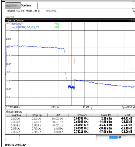
NTNV-N41-PC3-30-50-H-DFT-QPSK-Outter_Full-Ant1-PASS
