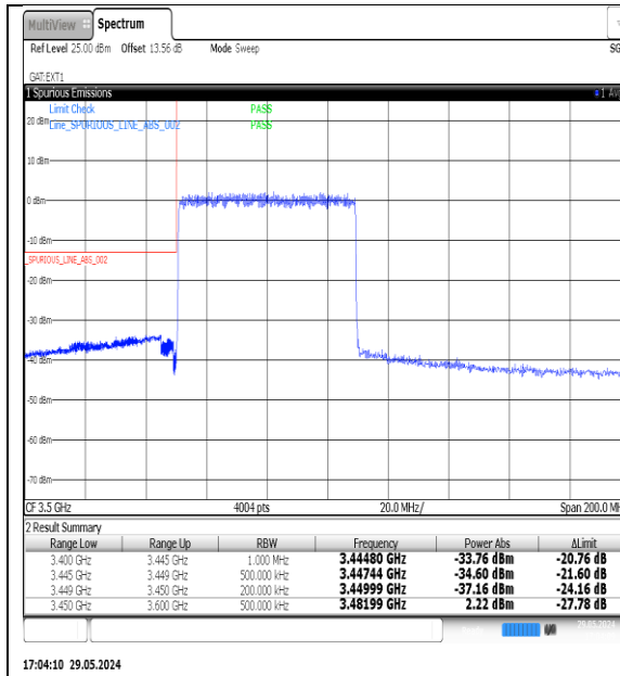
NTNV-N77-3450-3550-PC3-30-60-L-DFT-QPSK-Outer_Full-Ant1-PASS
