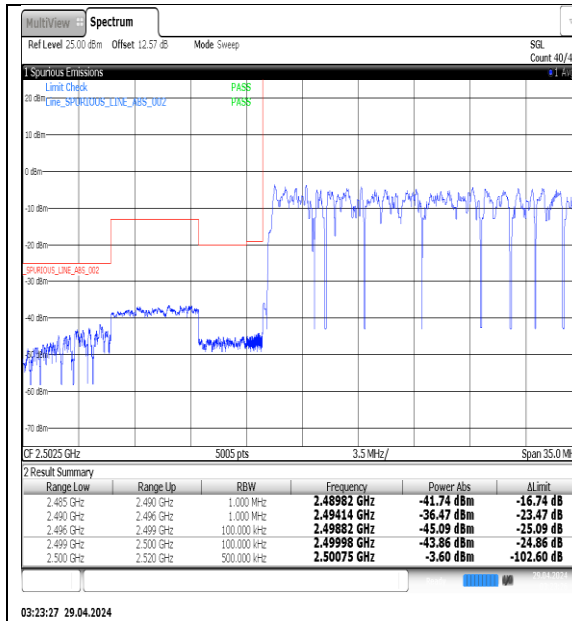
NTNV-N7-PC3-15-40-L-DFT-QPSK-Outter_Full-Ant1-PASS
