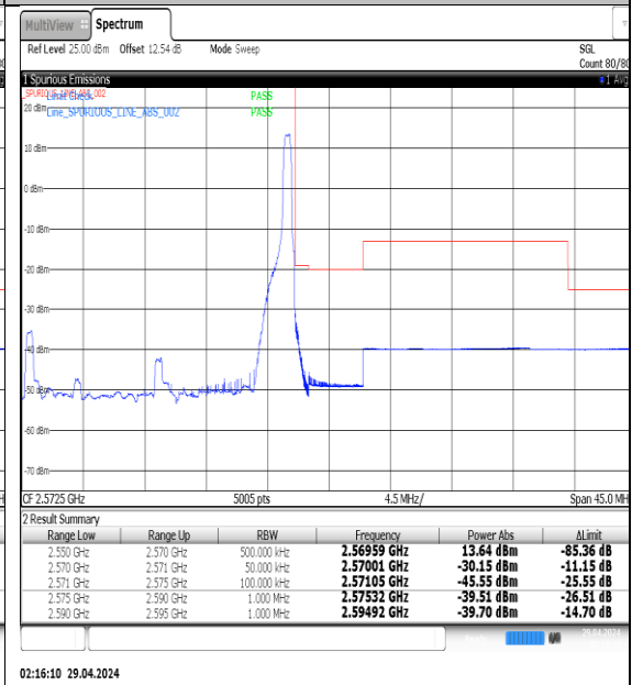
NTNV-N7-PC3-15-20-H-DFT-QPSK-Edge_1RB_Right-Ant1-PASS
