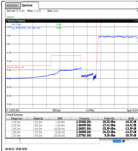
NTNV-N38-PC3-30-15-L-DFT-QPSK-Outer_Full-Ant1-PASS
