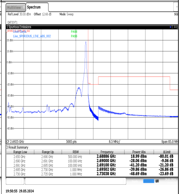
NTNV-N41-PC3-30-40-H-DFT-QPSK-Edge_1RB_Right-Ant1-PASS
