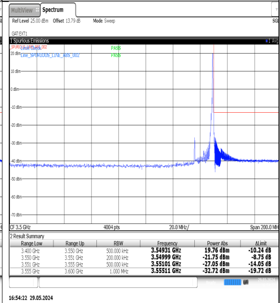
NTNV-N77-3450-3550-PC3-30-15-H-DFT-QPSK-Edge_1RB_Right-Ant1-PASS
