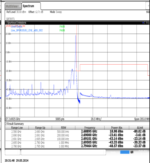
NTVN-N41-PC3-30-100-H-DFT-QPSK-Edge_1RB_Right-Ant1-PASS
