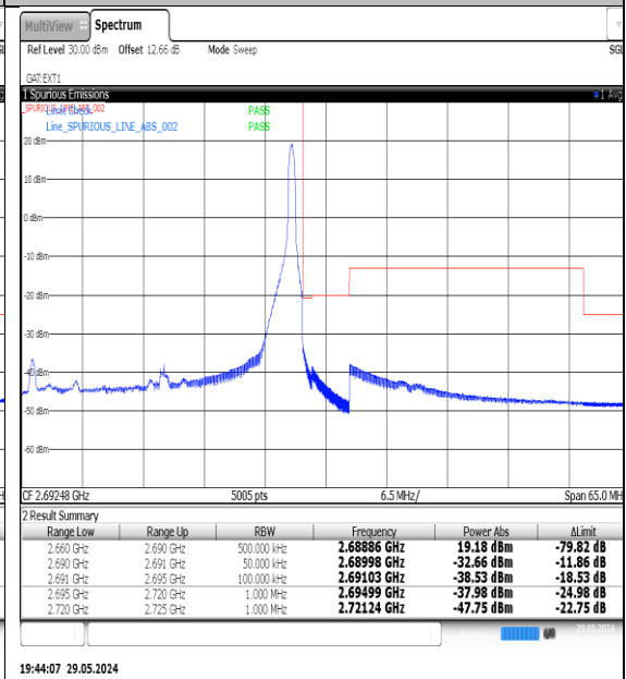
NTNV-N41-PC3-30-30-H-DFT-QPSK-Edge_1RB_Right-Ant1-PASS
