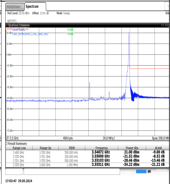
NTNV-N77-3450-3550-PC3-30-50-H-DFT-QPSK-Edge_1RB_Right-Ant1-PASS
