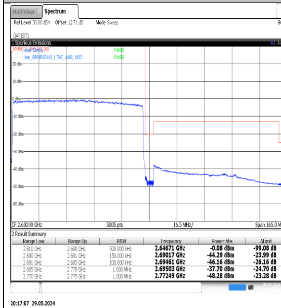
NTNV-N41-PC3-30-80-H-DFT-QPSK-Outter_Full-Ant1-PASS
