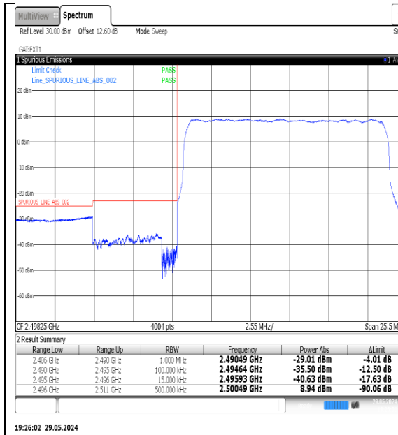
NTNV-N41-PC3-30-15-L-DFT-QPSK-Outter_Full-Ant1-PASS
