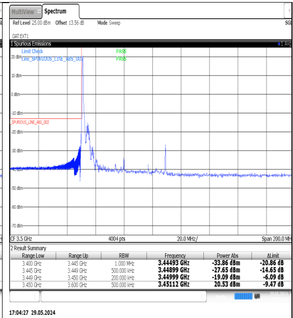
NTNV-N77-3450-3550-PC3-30-60-L-DFT-QPSK-Edge_1RB_Left-Ant1-PASS
