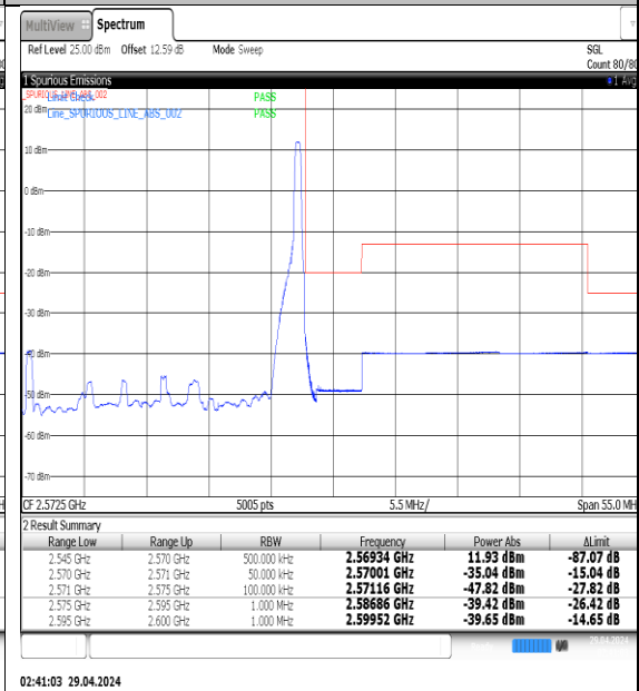
NTNV-N7-PC3-15-25-H-DFT-QPSK-Edge_1RB_Right-Ant1-PASS
