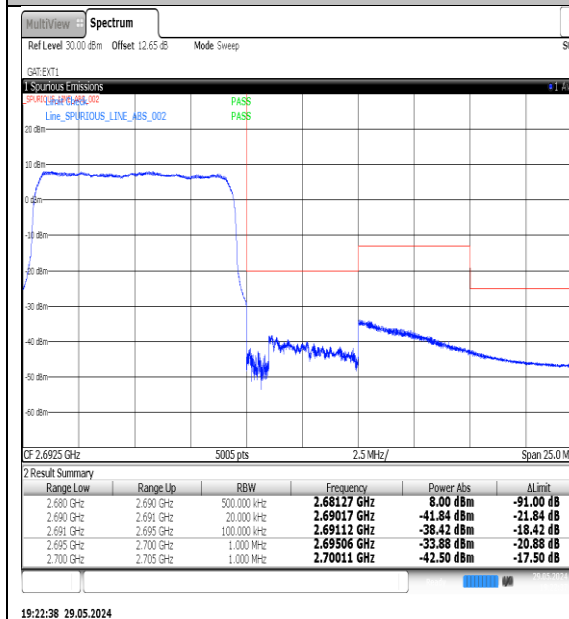
NTNV-N41-PC3-30-10-H-DFT-QPSK-Outter_Full-Ant1-PASS
