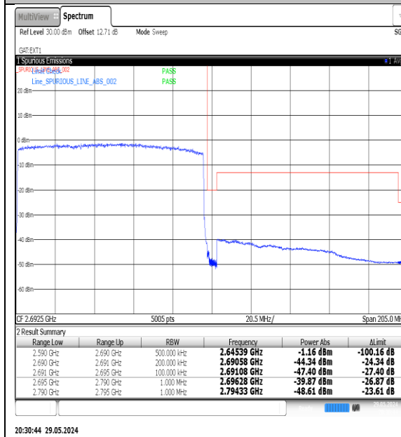
NTVN-N41-PC3-30-100-H-DFT-QPSK-Outter_Full-Ant1-PASS
