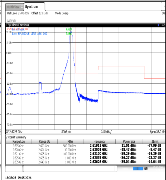
NTNV-N38-PC3-30-15-H-DFT-QPSK-Edge_1RB_Right-Ant1-PASS
