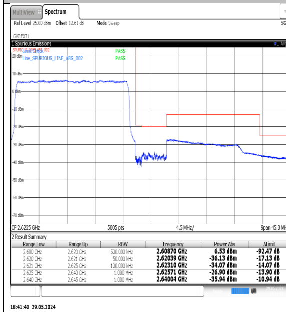
18:41:40 29.05.2024 NTNV-N38-PC3-30-20-H-DFT-QPSK-Outter_Full-Ant1-PASS
