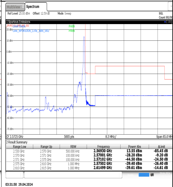
NTNV-N7-PC3-15-40-H-DFT-QPSK-Edge_1RB_Right-Ant1-PASS
