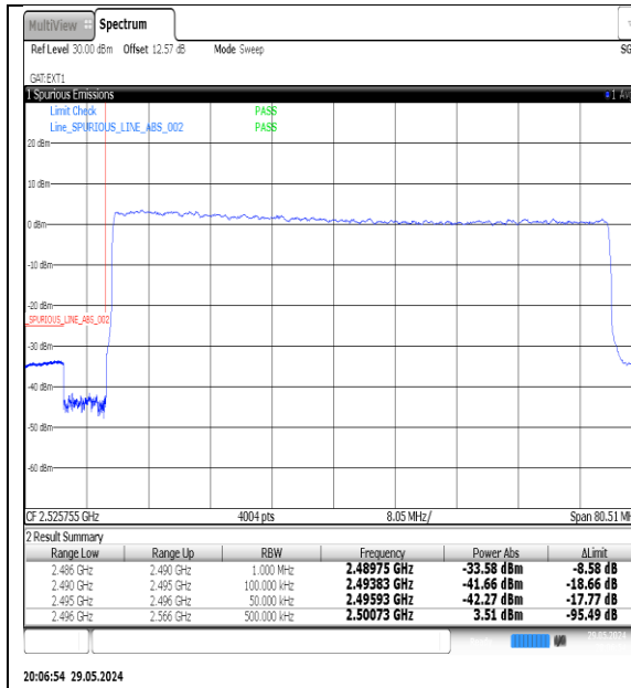
NTNV-N41-PC3-30-70-L-DFT-QPSK-Outter_Full-Ant1-PASS
