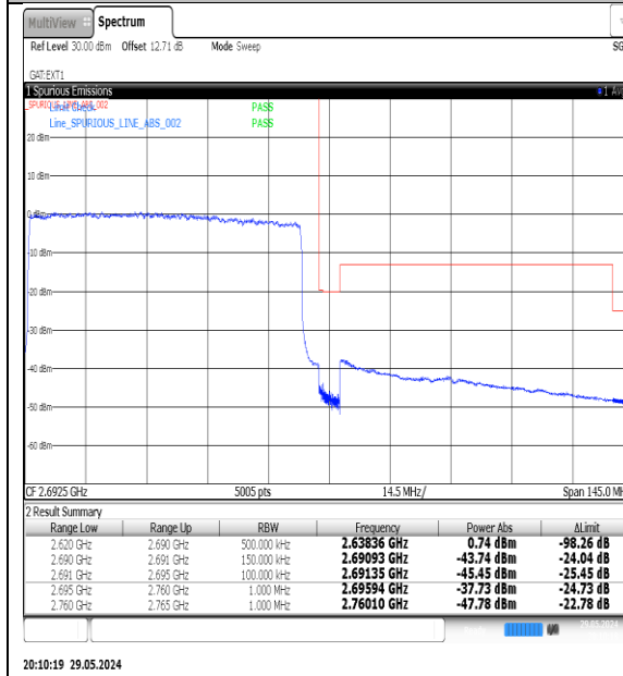
NTNV-N41-PC3-30-70-H-DFT-QPSK-Outter_Full-Ant1-PASS
