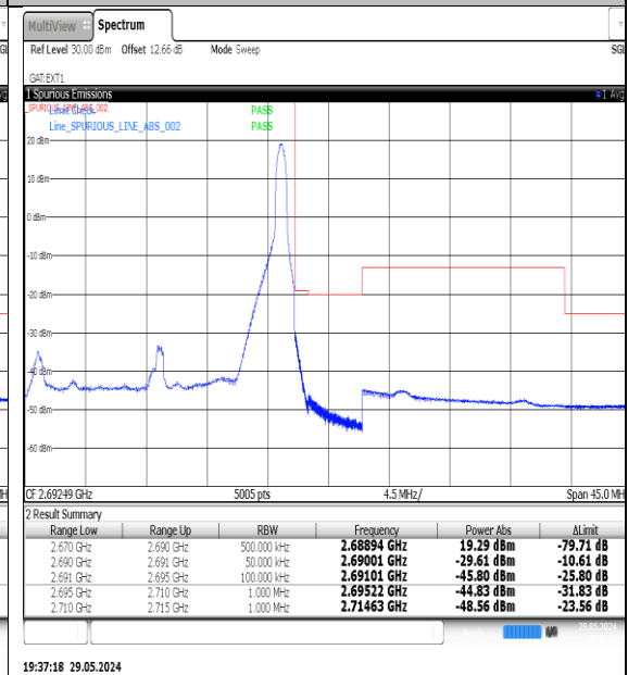
NTNV-N41-PC3-30-20-H-DFT-QPSK-Edge_1RB_Right-Ant1-PASS
