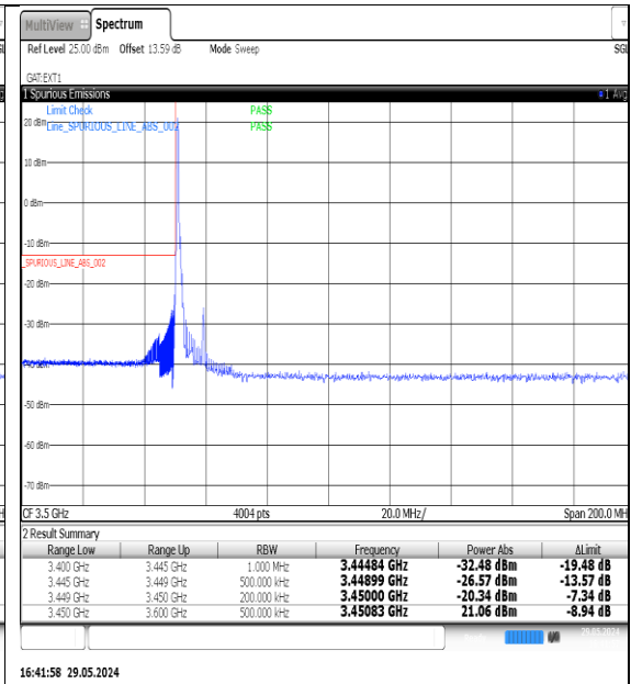
NTNV-N77-3450-3550-PC3-30-10-L-DFT-QPSK-Edge_1RB_Left-Ant1-PASS
