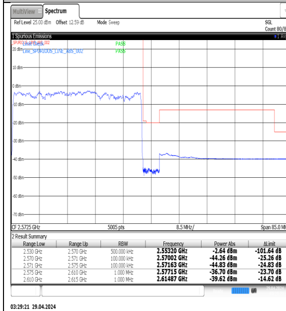
NTNV-N7-PC3-15-40-H-DFT-QPSK-Outter_Full-Ant1-PASS
