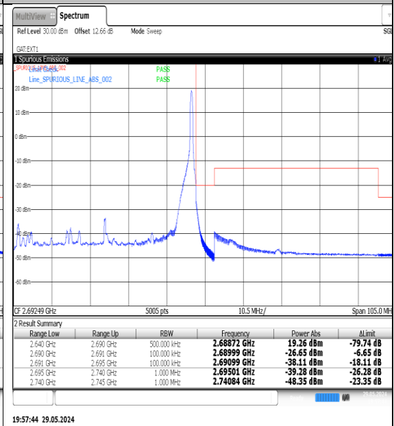
NTNV-N41-PC3-30-50-H-DFT-QPSK-Edge_1RB_Right-Ant1-PASS
