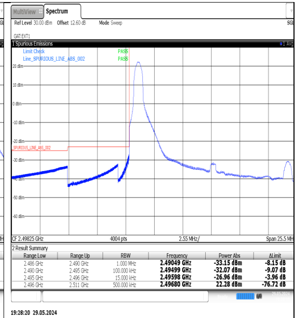
NTNV-N41-PC3-30-15-L-DFT-QPSK-Edge_1RB_Left-Ant1-PASS
