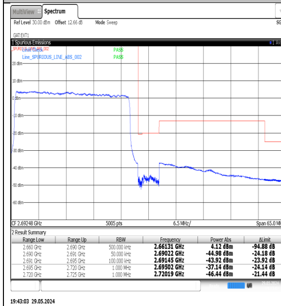
NTNV-N41-PC3-30-30-H-DFT-QPSK-Outter_Full-Ant1-PASS
