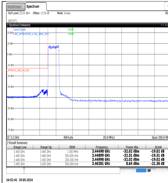
NTNV-N77-3450-3550-PC3-30-15-L-DFT-QPSK-Outer_Full-Ant1-PASS
