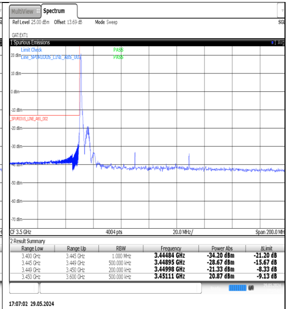
NTNV-N77-3450-3550-PC3-30-80-L-DFT-QPSK-Edge_1RB_Left-Ant1-PASS
