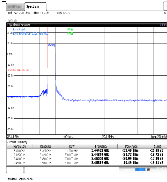
NTNV-N77-3450-3550-PC3-30-10-L-DFT-QPSK-Outer_Full-Ant1-PASS
