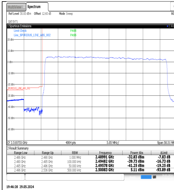
NTNV-N41-PC3-30-40-L-DFT-QPSK-Outter_Full-Ant1-PASS
