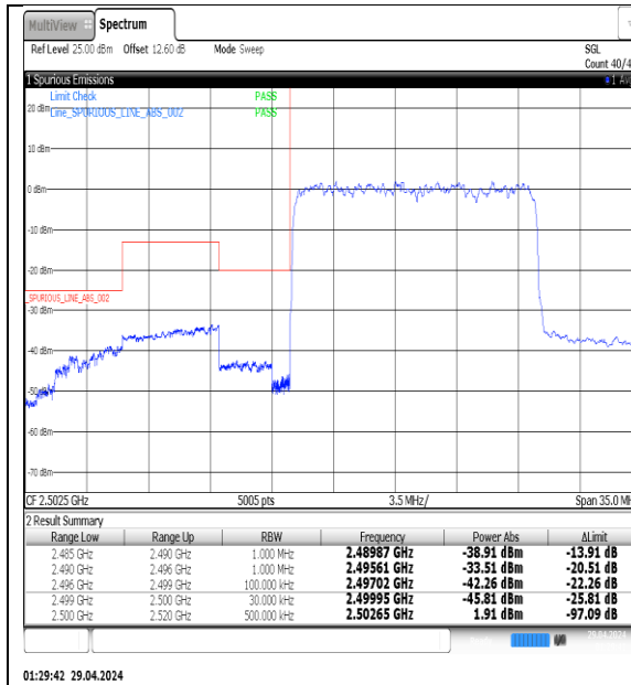
NTNV-N7-PC3-15-15-L-DFT-QPSK-Outter_Full-Ant1-PASS
