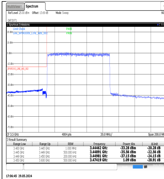
NTNV-N77-3450-3550-PC3-30-80-L-DFT-QPSK-Outer_Full-Ant1-PASS
