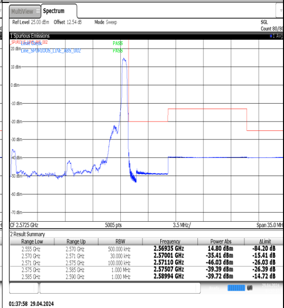
NTNV-N7-PC3-15-15-H-DFT-QPSK-Edge_1RB_Right-Ant1-PASS
