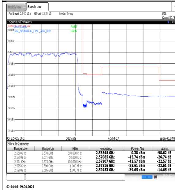
NTNV-N7-PC3-15-20-H-DFT-QPSK-Outter_Full-Ant1-PASS
