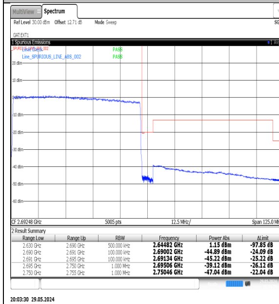
NTNV-N41-PC3-30-60-H-DFT-QPSK-Outter_Full-Ant1-PASS
