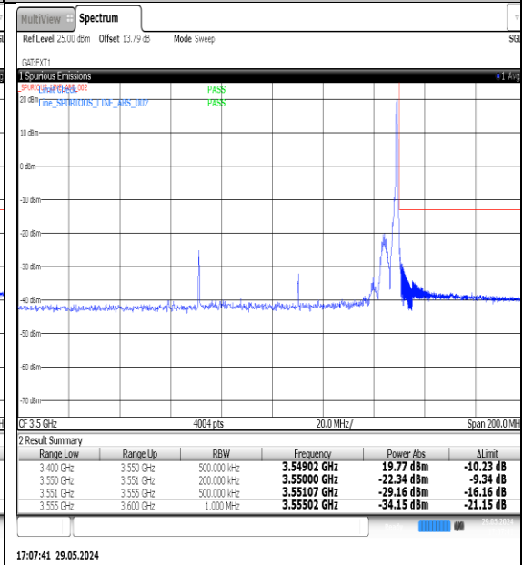
NTNV-N77-3450-3550-PC3-30-80-H-DFT-QPSK-Edge_1RB_Right-Ant1-PASS
