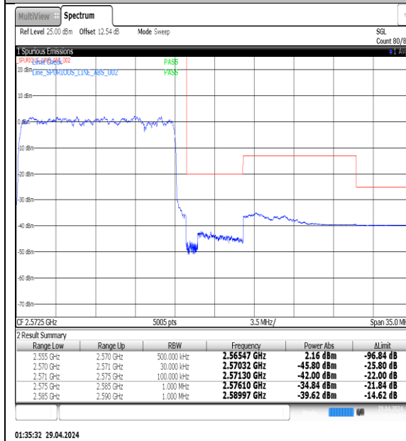
NTNV-N7-PC3-15-15-H-DFT-QPSK-Outter_Full-Ant1-PASS
