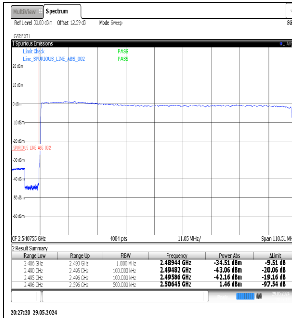
NTVN-N41-PC3-30-100-L-DFT-QPSK-Outter_Full-Ant1-PASS
