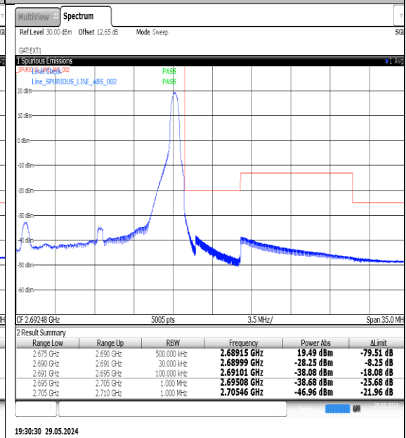
NTNV-N41-PC3-30-15-H-DFT-QPSK-Edge_1RB_Right-Ant1-PASS
