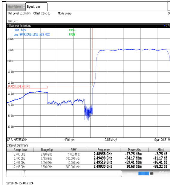
NTNV-N41-PC3-30-10-L-DFT-QPSK-Outter_Full-Ant1-PASS
