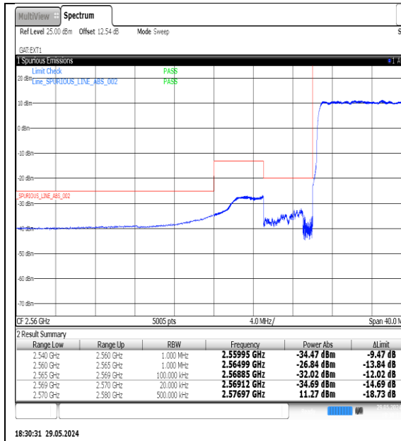
NTNV-N38-PC3-30-10-L-DFT-QPSK-Outter_Full-Ant1-PASS
