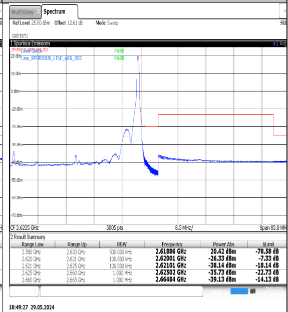
NTNV-N38-PC3-30-40-H-DFT-QPSK-Edge_1RB_Right-Ant1-PASS
