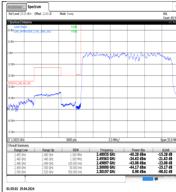
NTNV-N7-PC3-15-20-L-DFT-QPSK-Outter_Full-Ant1-PASS
