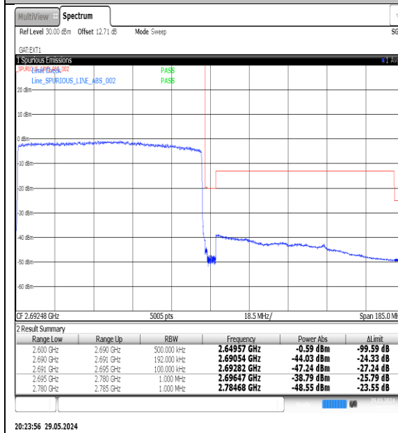
NTNV-N41-PC3-30-90-H-DFT-QPSK-Outer_Full-Ant1-PASS
