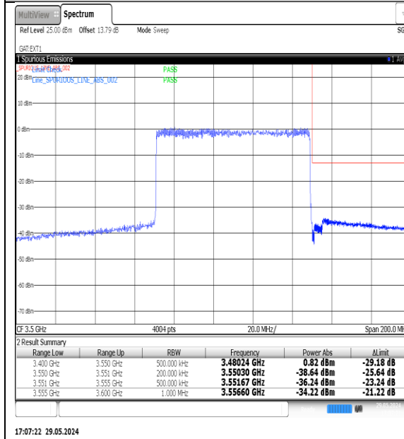
NTNV-N77-3450-3550-PC3-30-80-H-DFT-QPSK-Outer_Full-Ant1-PASS
