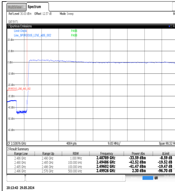
NTNV-N41-PC3-30-80-L-DFT-QPSK-Outter_Full-Ant1-PASS
