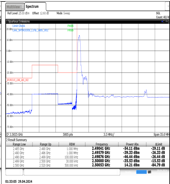
NTNV-N7-PC3-15-15-L-DFT-QPSK-Edge_1RB_Left-Ant1-PASS
