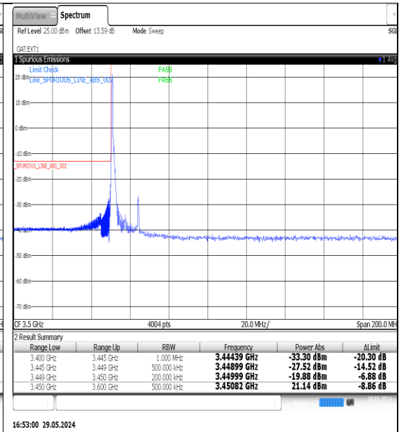
NTNV-N77-3450-3550-PC3-30-15-L-DFT-QPSK-Edge_1RB_Left-Ant1-PASS
