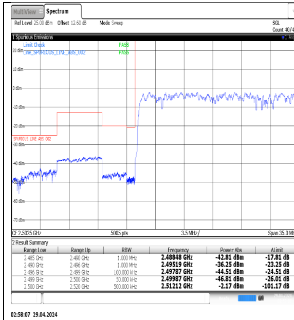
NTNV-N7-PC3-15-30-L-DFT-QPSK-Outer_Full-Ant1-PASS
