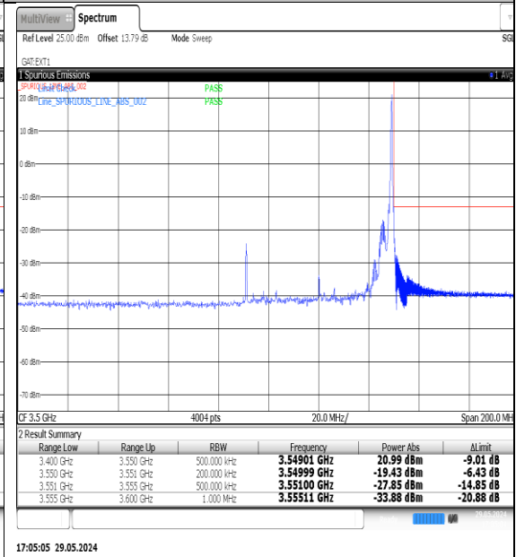
NTNV-N77-3450-3550-PC3-30-60-H-DFT-QPSK-Edge_1RB_Right-Ant1-PASS
