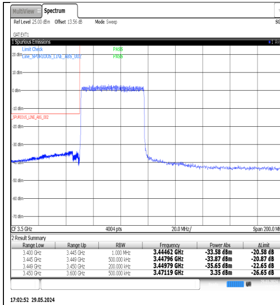
NTNV-N77-3450-3550-PC3-30-50-L-DFT-QPSK-Outer_Full-Ant1-PASS
