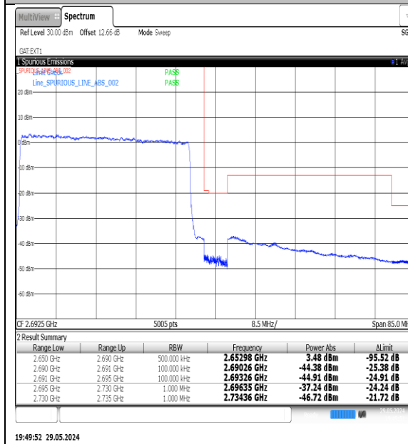
NTNV-N41-PC3-30-40-H-DFT-QPSK-Outter_Full-Ant1-PASS
