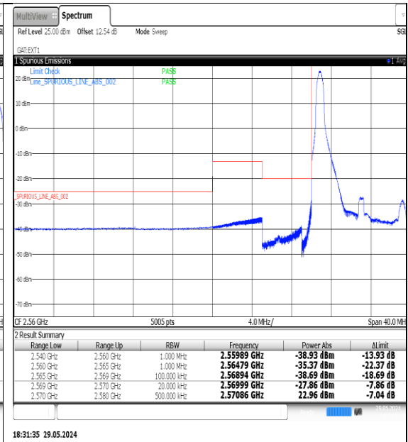
NTNV-N38-PC3-30-10-L-DFT-QPSK-Edge_1RB_Left-Ant1-PASS
