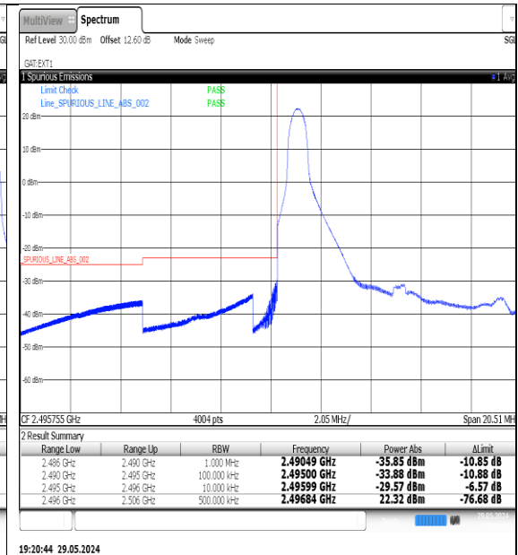
NTNV-N41-PC3-30-10-L-DFT-QPSK-Edge_1RB_Left-Ant1-PASS
