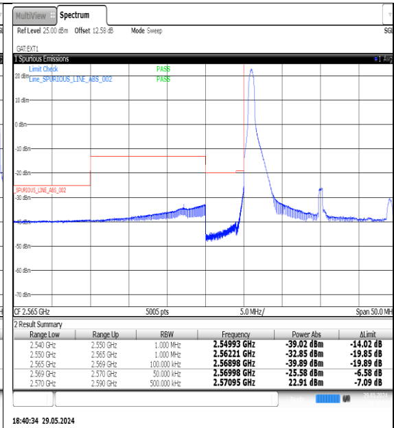
18:40:34 29.05.2024 NTNV-N38-PC3-30-20-L-DFT-QPSK-Edge_1RB_Left-Ant1-PASS
