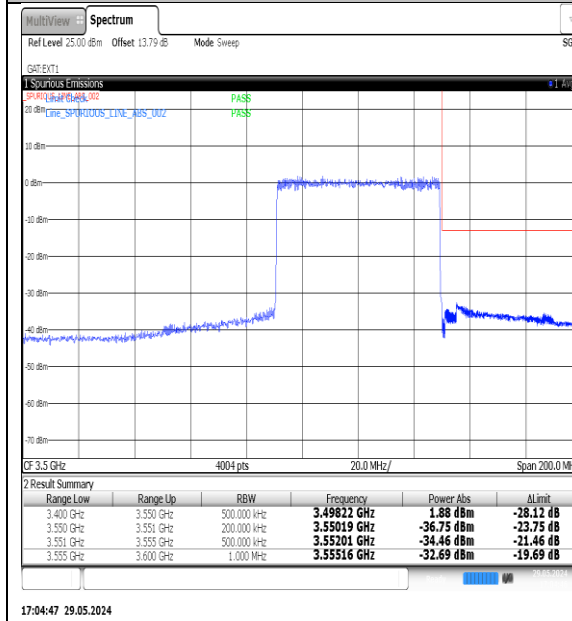
NTNV-N77-3450-3550-PC3-30-60-H-DFT-QPSK-Outer_Full-Ant1-PASS
