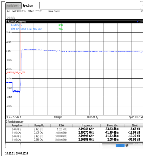
NTNV-N41-PC3-30-90-L-DFT-QPSK-Outer_Full-Ant1-PASS
