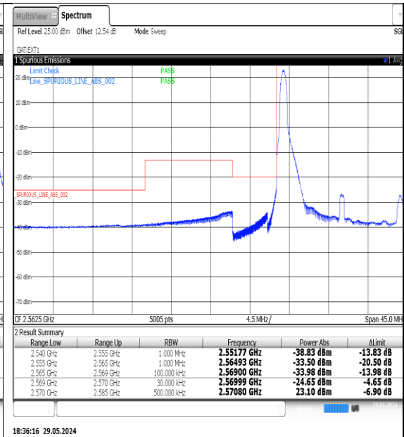
NTNV-N38-PC3-30-15-L-DFT-QPSK-Edge_1RB_Left-Ant1-PASS
