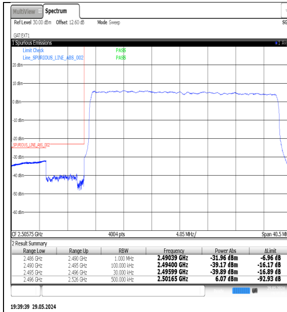
NTNV-N41-PC3-30-30-L-DFT-QPSK-Outter_Full-Ant1-PASS
