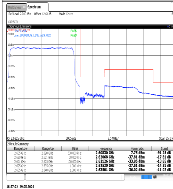
NTNV-N38-PC3-30-15-H-DFT-QPSK-Outer_Full-Ant1-PASS
