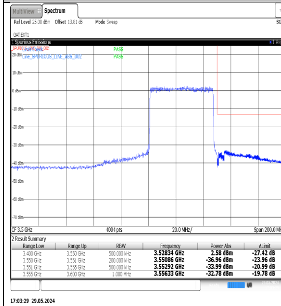
NTNV-N77-3450-3550-PC3-30-50-H-DFT-QPSK-Outer_Full-Ant1-PASS
