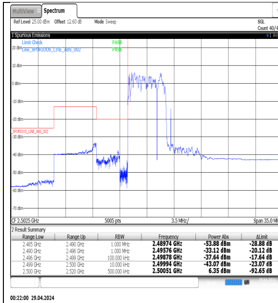
NTNV-N7-PC3-15-5-L-DFT-QPSK-Outer_Full-Ant1-PASS
