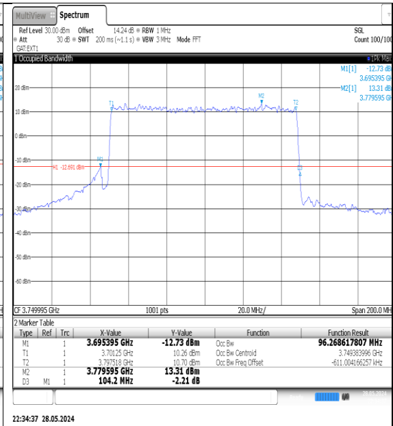
NTNV-N78-3700-3800-PC3-30-100-M-DFT- 16QAM-Outer_Full-Ant1-PASS
