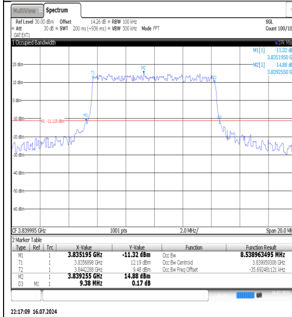
NTNV-N77-3700-3980-PC3-30-10-M-DFT- PI2BPSK-Outer_Full-Ant1-PASS
