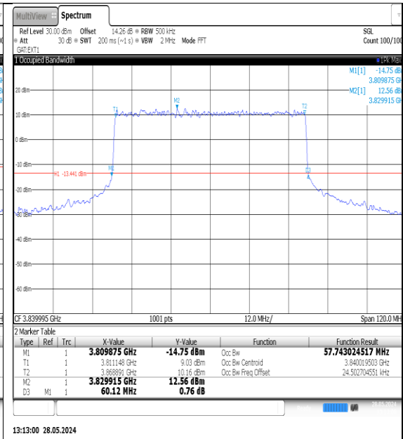
NTNV-N77-3700-3980-PC3-30-60-M-DFT-16QAM-Outer_Full-Ant1-PASS
