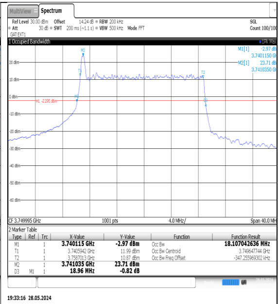
NTNV-N78-3700-3800-PC3-30-20-M-DFT-QPSK- Outer_Full-Ant1-PASS
