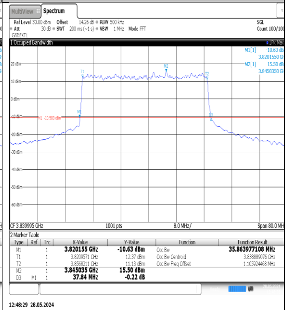
NTNV-N77-3700-3980-PC3-30-40-M-DFT-16QAM-Outer_Full-Ant1-PASS
