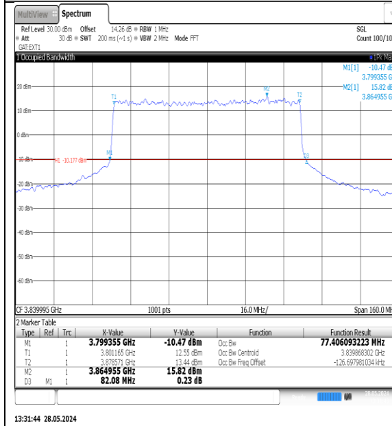
NTNV-N77-3700-3980-PC3-30-80-M-DFT-QPSK-Outter_Full-Ant1-PASS
