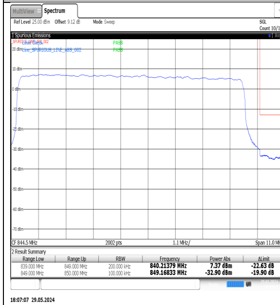
NTNV-N5-PC3-15-10-H-DFT-QPSK-Outter_Full-Ant1-PASS
