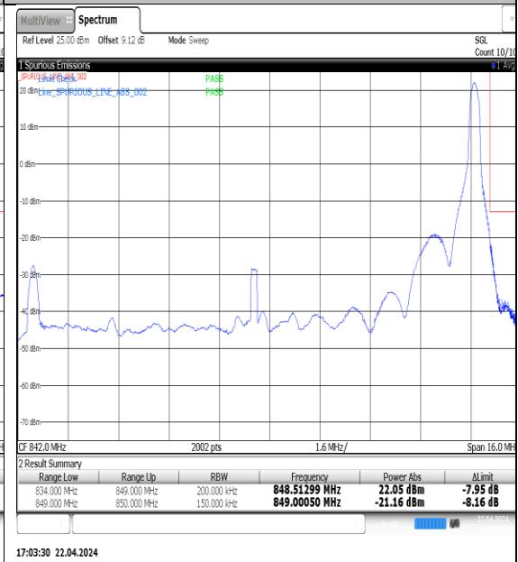
NTNV-N5-PC3-15-15-H-DFT-QPSK-Edge_1RB_Right-Ant1-PASS
