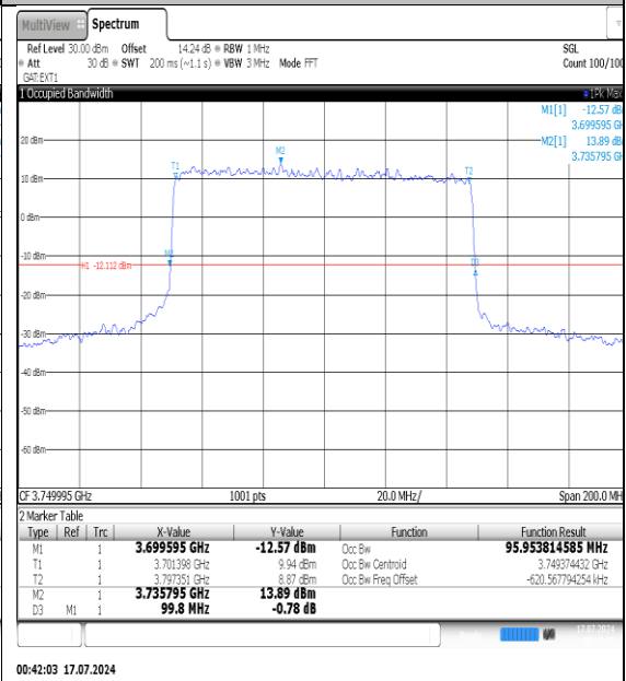
NTNV-N78-3700-3800-PC3-30-100-M-DFT-Pi2BPSK-Outer_Full-Ant1-PASS
