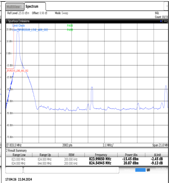
NTNV-N5-PC3-15-20-L-DFT-QPSK-Edge_1RB_Left-Ant1-PASS
