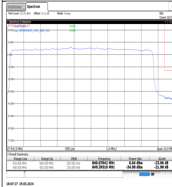
NTNV-N5-PC3-15-15-H-DFT-QPSK-Outer_Full-Ant1-PASS
