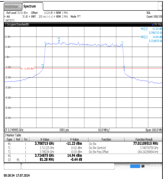
NTNV-N78-3700-3800-PC3-30-80-M-DFT-PI2BPSK-Outer_Full-Ant1-PASS
