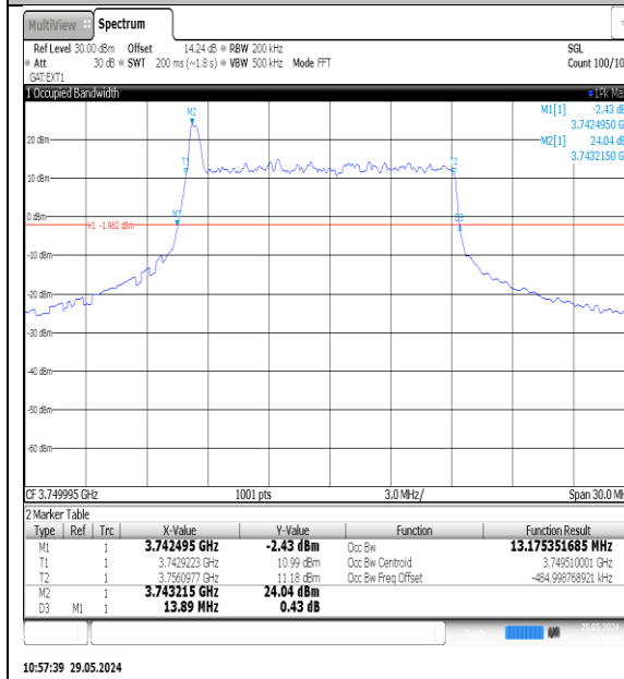
NTNV-N78-3700-3800-PC3-30-15-M-DFT-QPSK-Outer_Full-Ant1-PASS
