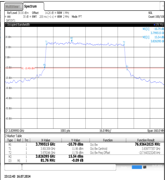
NTNV-N77-3700-3980-PC3-30-80-M-DFT-PI2BPSK-Outter_Full-Ant1-PASS
