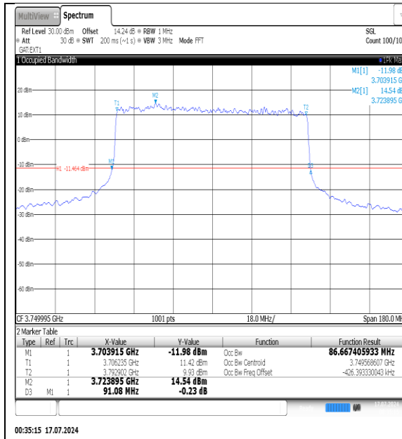
NTNV-N78-3700-3800-PC3-30-90-M-DFT-Pi2BPSK-Outer_Full-Ant1-PASS
