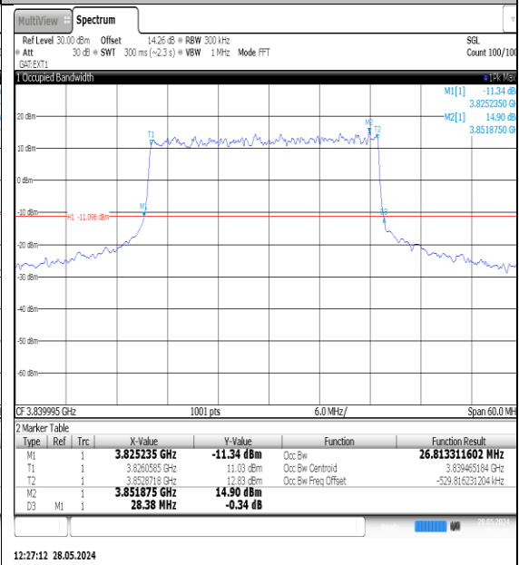
NTVN-N77-3700-3980-PC3-30-30-M-DFT-QPSK-Outer_Full-Ant1-PASS
