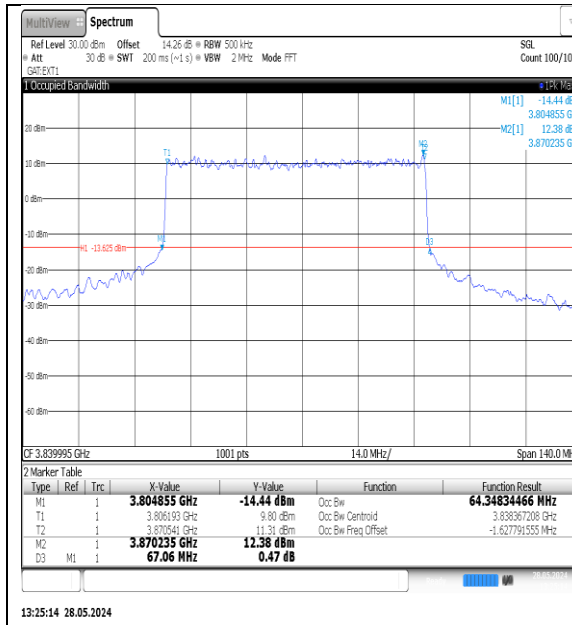
NTNV-N77-3700-3980-PC3-30-70-M-DFT-16QAM-Outter_Full-Ant1-PASS
