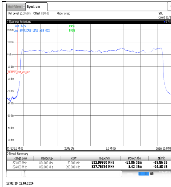
NTNV-N5-PC3-15-15-L-DFT-QPSK-Outer_Full-Ant1-PASS
