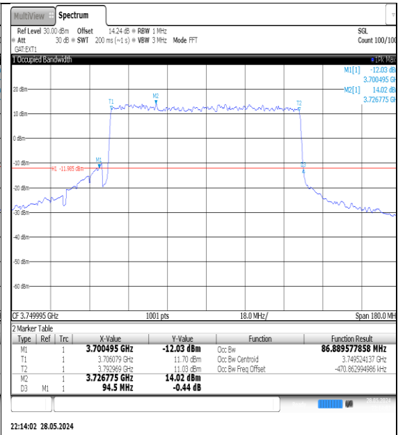
NTNV-N78-3700-3800-PC3-30-90-M-DFT-QPSK-Outer_Full-Ant1-PASS
