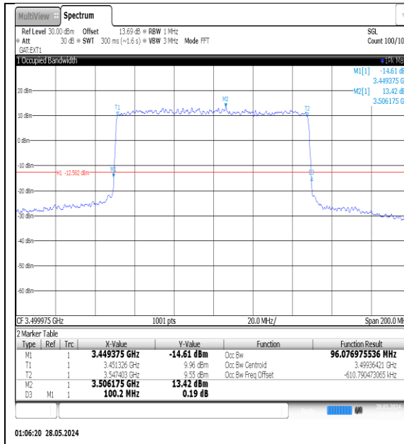
NTNV-N77-3450-3550-PC3-30-100-M-DFT- QPSK-Outer_Full-Ant1-PASS
