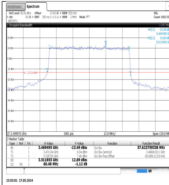
NTNV-N77-3450-3550-PC3-30-60-M-DFT-QPSK-Outer_Full-Ant1-PASS
