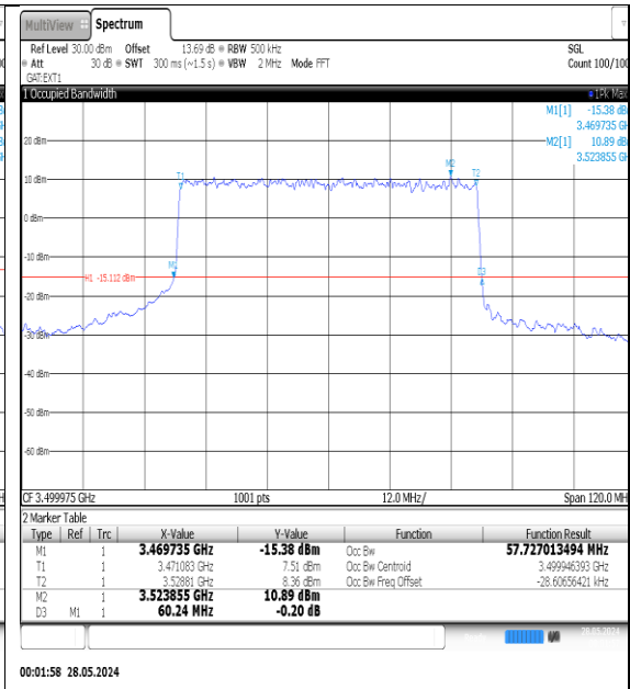
NTNV-N77-3450-3550-PC3-30-60-M-DFT-16QAM-Outer_Full-Ant1-PASS
