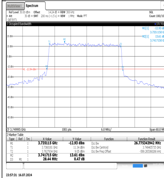
NTNV-N78-3700-3800-PC3-30-30-M-DFT-PI2BPSK-Outer_Full-Ant1-PASS
