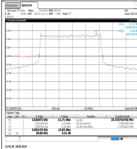
NTNV-N77-3700-3980-PC3-30-40-M-DFT-QPSK-Outer_Full-Ant1-PASS
