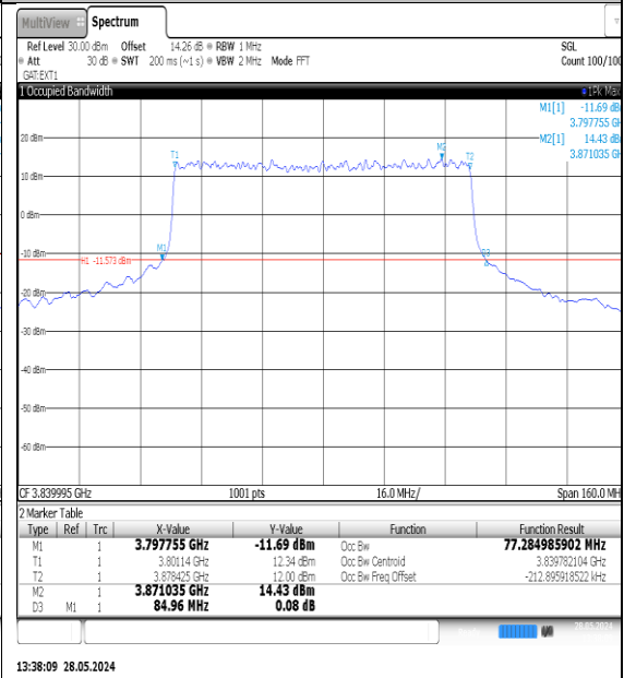
NTNV-N77-3700-3980-PC3-30-80-M-DFT-16QAM-Outter_Full-Ant1-PASS
