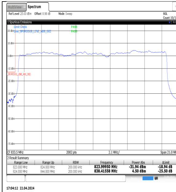
NTNV-N5-PC3-15-20-L-DFT-QPSK-Outter_Full-Ant1-PASS
