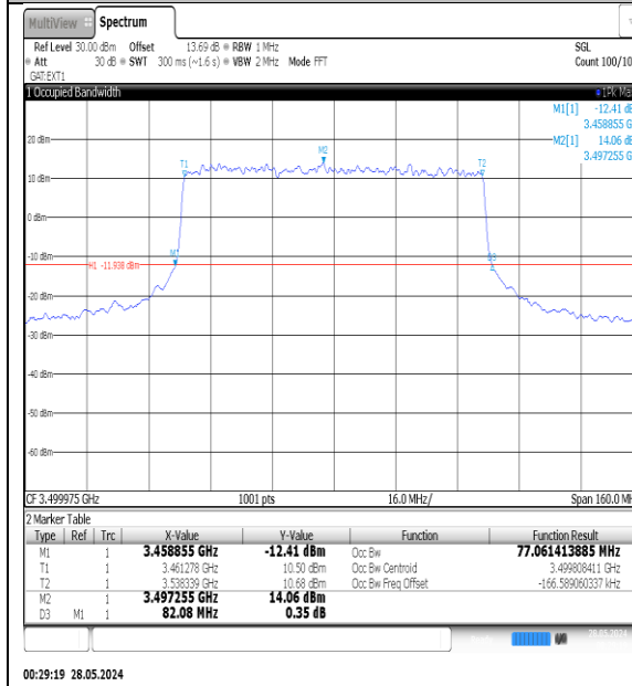
NTNV-N77-3450-3550-PC3-30-80-M-DFT-QPSK-Outter_Full-Ant1-PASS
