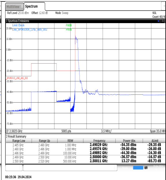
NTNV-N7-PC3-15-5-L-DFT-QPSK-Edge_1RB_Left-Ant1-PASS
