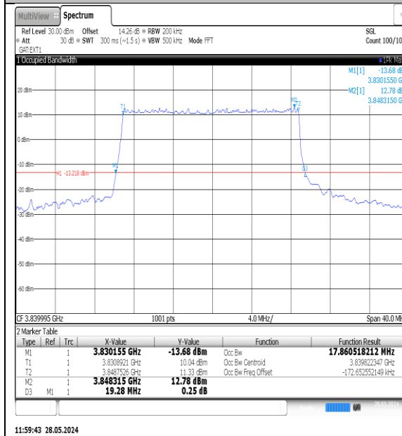
NTNV-N77-3700-3980-PC3-30-20-M-DFT- 16QAM-Outer_Full-Ant1-PASS
