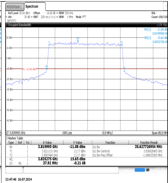
NTNV-N77-3700-3980-PC3-30-40-M-DFT-PI2BPSK-Outer_Full-Ant1-PASS
