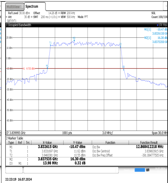
NTNV-N77-3700-3980-PC3-30-15-M-DFT-PI2BPSK-Outer_Full-Ant1-PASS
