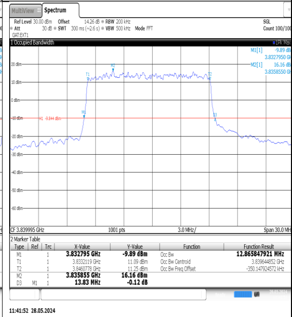
NTNV-N77-3700-3980-PC3-30-15-M-DFT-16QAM-Outer_Full-Ant1-PASS
