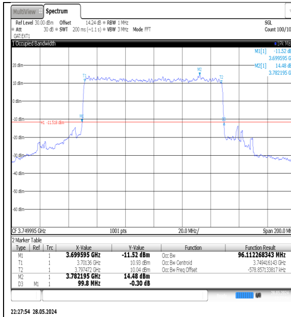
NTNV-N78-3700-3800-PC3-30-100-M-DFT- QPSK-Outer_Full-Ant1-PASS
