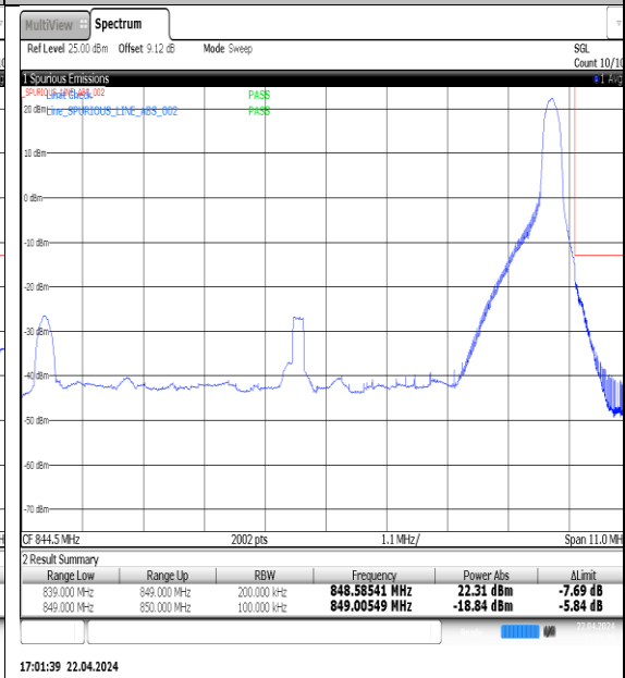
NTNV-N5-PC3-15-10-H-DFT-QPSK-Edge_1RB_Right-Ant1-PASS
