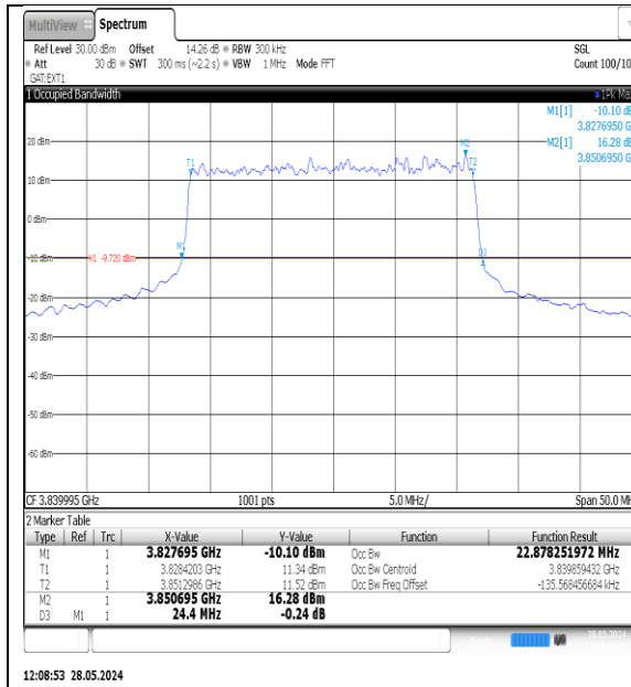
NTVN-N77-3700-3980-PC3-30-25-M-DFT-QPSK-Outer_Full-Ant1-PASS
