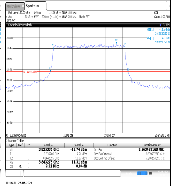
NTNV-N77-3700-3980-PC3-30-10-M-DFT-QPSK- Outer_Full-Ant1-PASS
