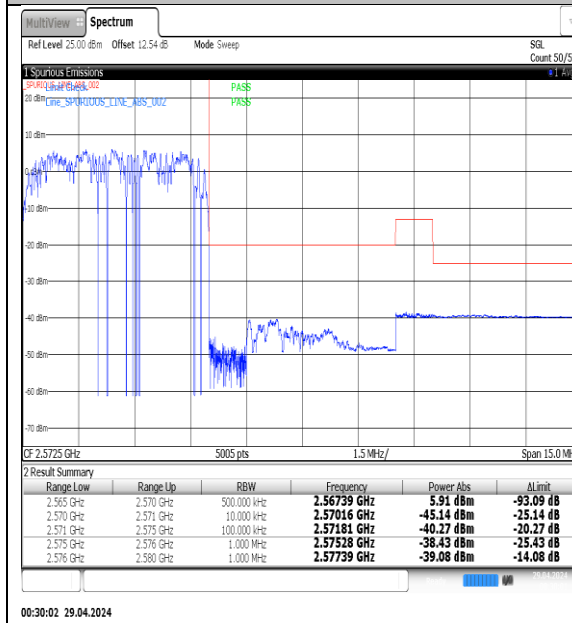
NTNV-N7-PC3-15-5-H-DFT-QPSK-Outer_Full-Ant1-PASS
