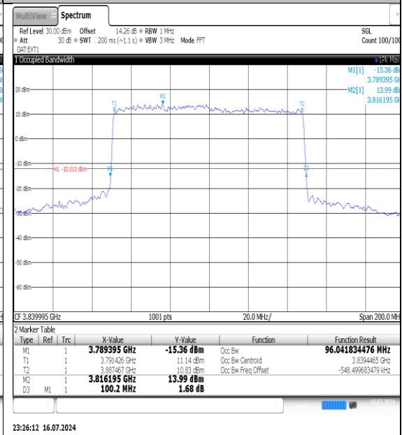
NTNV-N77-3700-3980-PC3-30-100-M-DFT-Pi2BPSK-Outer_Full-Ant1-PASS
