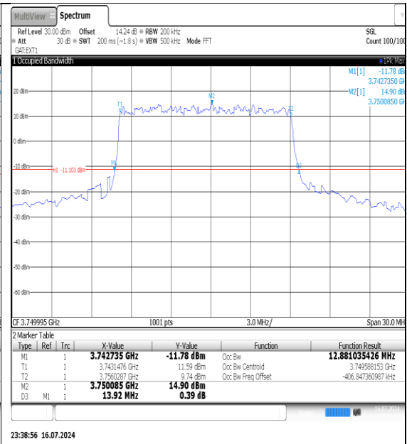
NTNV-N78-3700-3800-PC3-30-15-M-DFT-PI2BPSK-Outer_Full-Ant1-PASS
