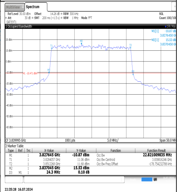
NTNV-N77-3700-3980-PC3-30-25-M-DFT- P12BPSK-Outer_Full-Ant1-PASS
