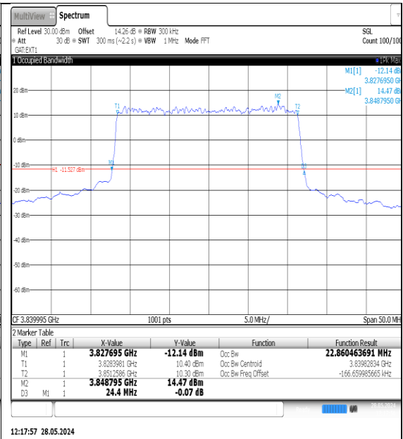
NTVN-N77-3700-3980-PC3-30-25-M-DFT-16QAM-Outer_Full-Ant1-PASS
