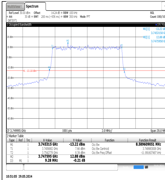
NTNV-N78-3700-3800-PC3-30-10-M-DFT-16QAM-Outer_Full-Ant1-PASS
