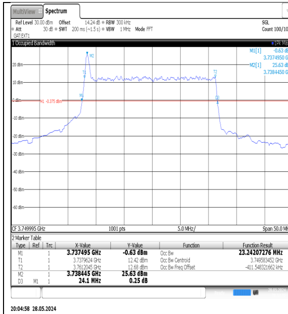
NTNV-N78-3700-3800-PC3-30-25-M-DFT-QPSK-Outer_Full-Ant1-PASS
