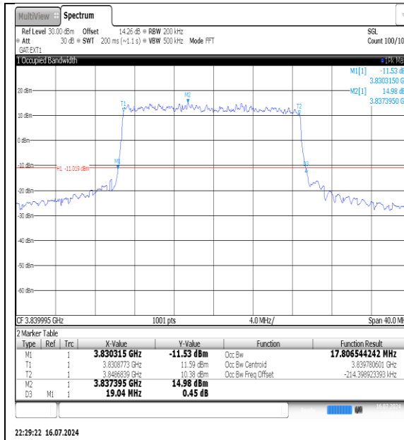
NTNV-N77-3700-3980-PC3-30-20-M-DFT- P12BPSK-Outer_Full-Ant1-PASS
