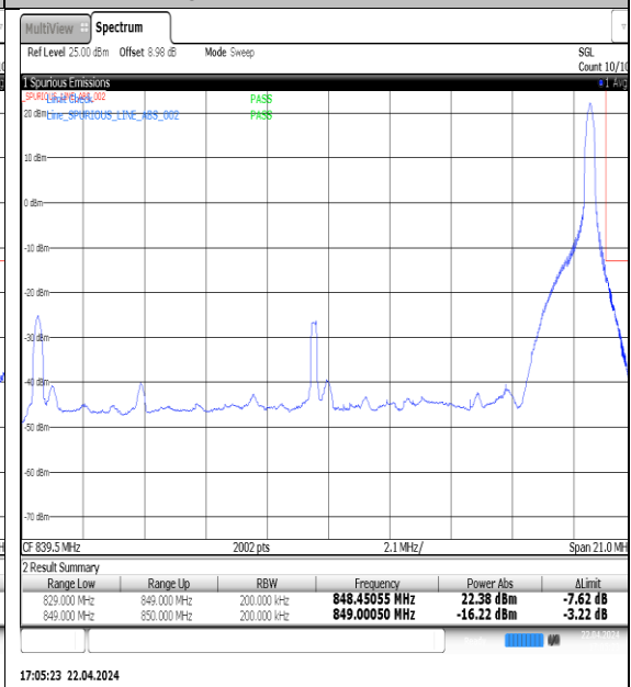
NTNV-N5-PC3-15-20-H-DFT-QPSK-Edge_1RB_Right-Ant1-PASS
