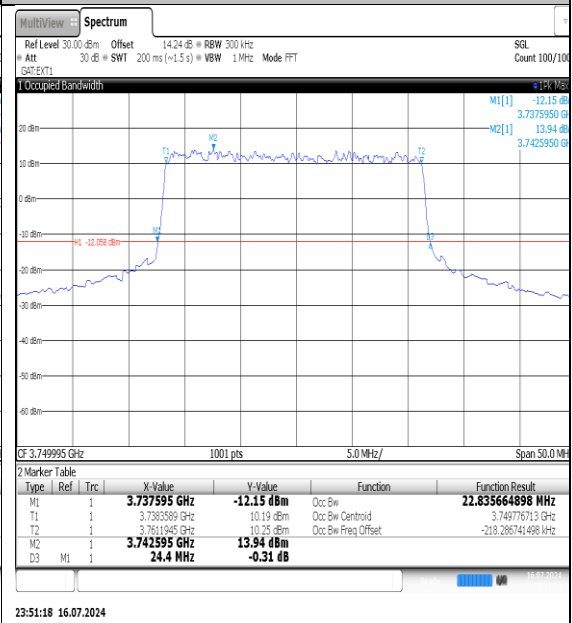
NTNV-N78-3700-3800-PC3-30-25-M-DFT- Pi2BPSK-Outer_Full-Ant1-PASS
