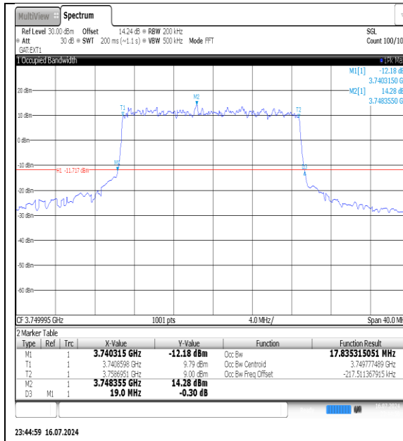
NTNV-N78-3700-3800-PC3-30-20-M-DFT- Pi2BPSK-Outer_Full-Ant1-PASS
