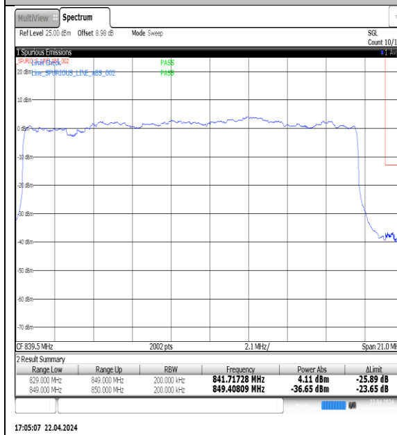
NTNV-N5-PC3-15-20-H-DFT-QPSK-Outter_Full-Ant1-PASS
