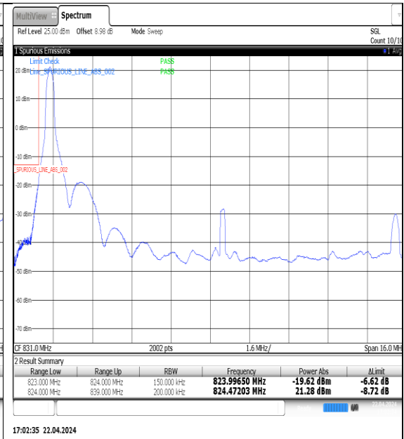
NTNV-N5-PC3-15-15-L-DFT-QPSK-Edge_1RB_Left-Ant1-PASS
