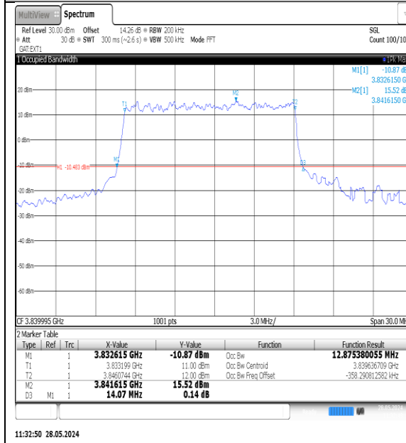
NTNV-N77-3700-3980-PC3-30-15-M-DFT-QPSK-Outer_Full-Ant1-PASS
