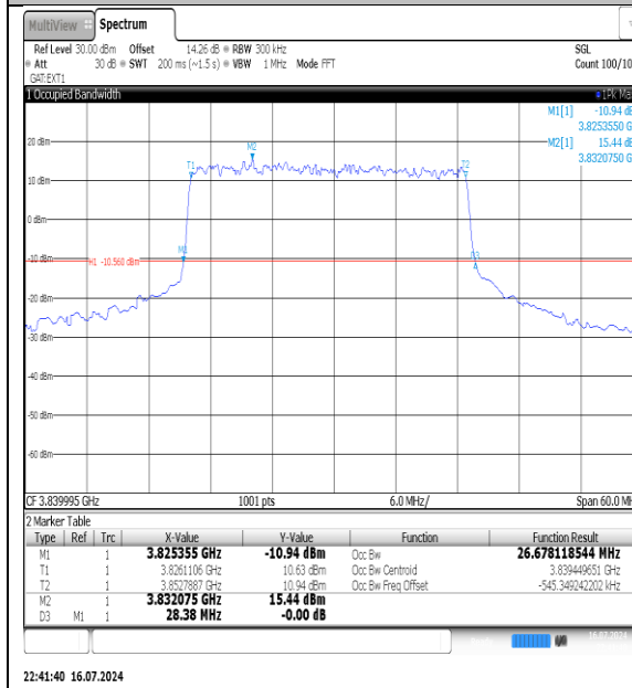
NTVN-N77-3700-3980-PC3-30-30-M-DFT-PI2BPSK-Outer_Full-Ant1-PASS
