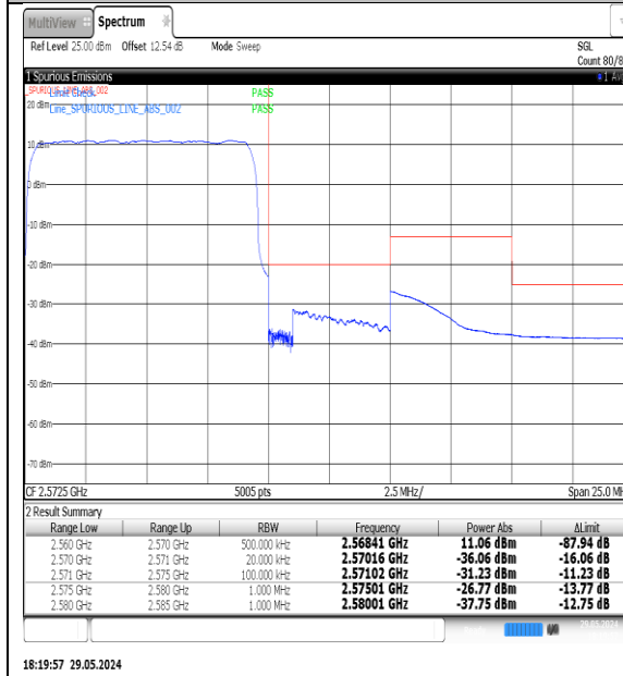
NTNV-N7-PC3-15-10-H-DFT-QPSK-Outter_Full-Ant1-PASS
