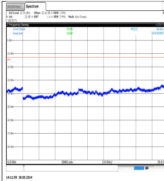
NTNV-N77-3700-3980-PC3-30-10-H-DFT-QPSK-Edge_1RB_Left-6000-26000-Ant1-PASS
