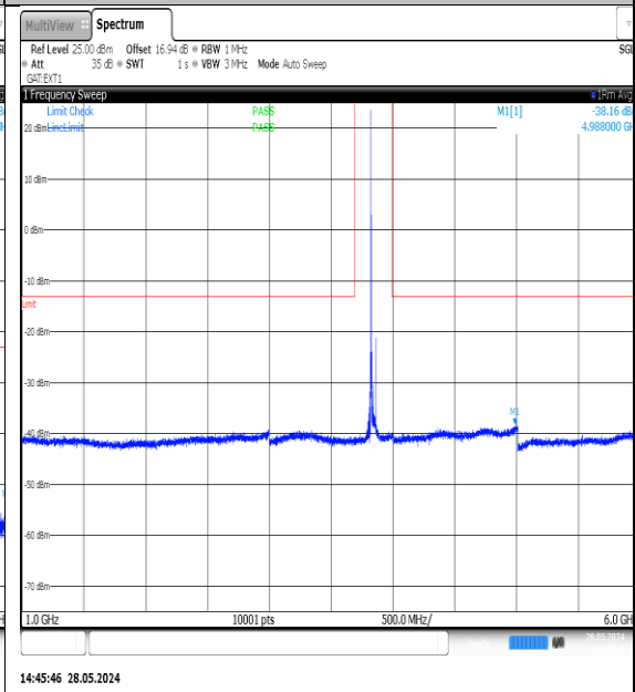
NTVN-N77-3700-3980-PC3-30-40-M-DFT-QPSK-Edge_1RB_Left-1000-6000-Ant1-PASS
