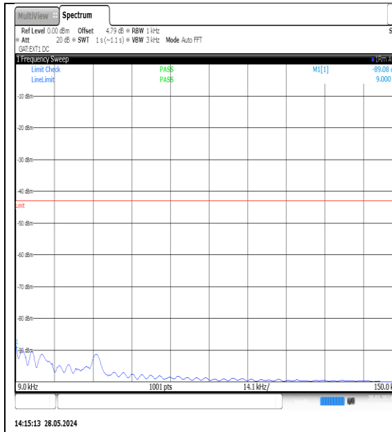
NTNV-N77-3700-3980-PC3-30-15-M-DFT-QPSK- Edge_1RB_Left-0.009-0.15-Ant1-PASS
