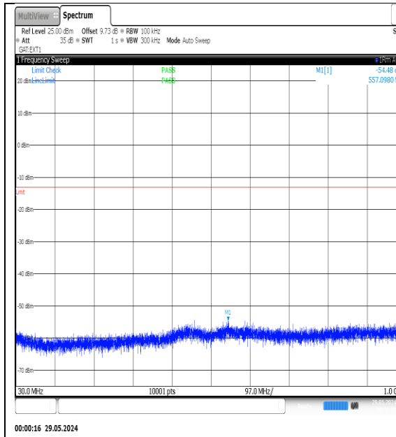
NTNV-N78-3700-3800-PC3-30-100-H-DFT-QPSK-Edge_1RB_Left-30-100-Ant1-PASS
