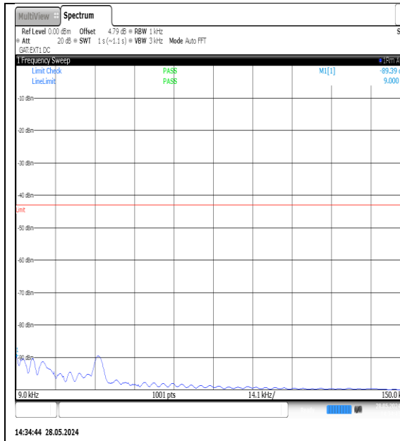
NTNV-N77-3700-3980-PC3-30-30-L-DFT-QPSK-Edge_1RB_Left-0.009-0.15-Ant1-PASS
