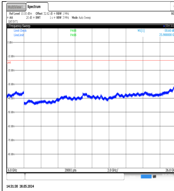
NTNV-N77-3700-3980-PC3-30-25-M-DFT-QPSK- Edge_1RB_Left-6000-26000-Ant1-PASS
