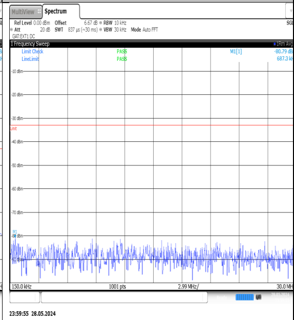
N78-3700-3800-PC3-30-100-H-DFT-QPSK-Edge_1RB_Left-0.15-30-Ant1-PASS
