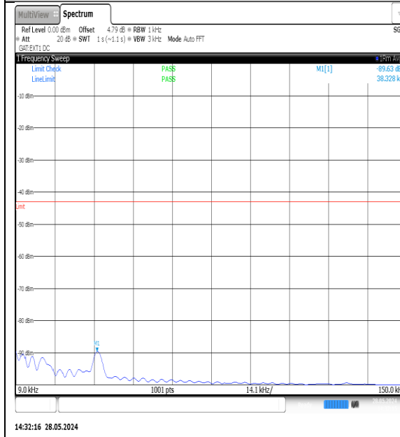
NTNV-N77-3700-3980-PC3-30-25-H-DFT-QPSK- Edge_1RB_Left-0.009-0.15-Ant1-PASS
