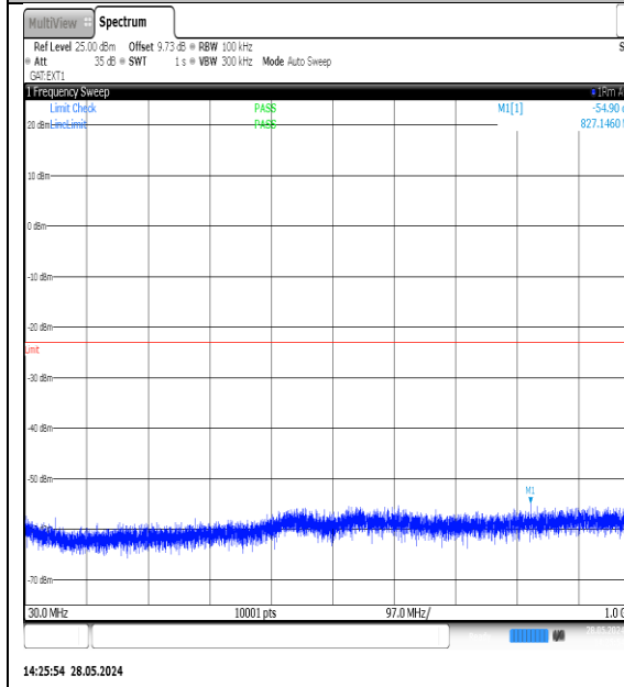
NTNV-N77-3700-3980-PC3-30-20-H-DFT-QPSK-Edge_1RB_Left-30-1000-Ant1-PASS
