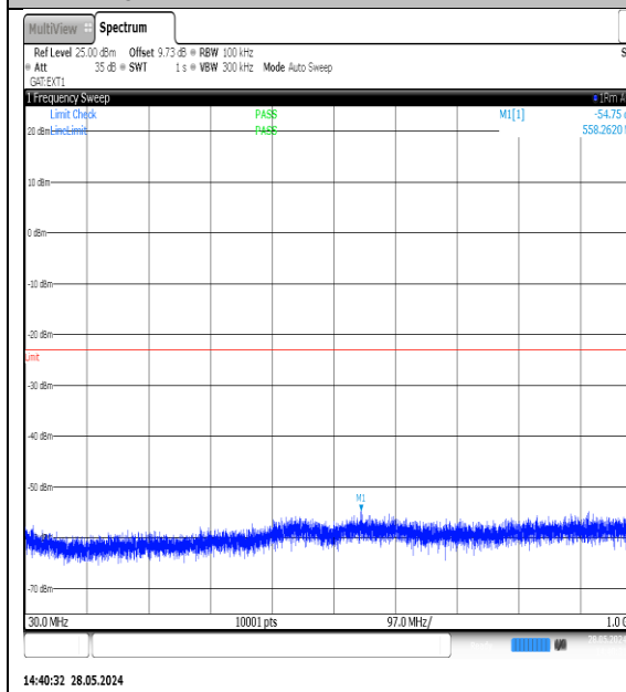
NTNV-N77-3700-3980-PC3-30-30-H-DFT-QPSK- Edge_1RB_Left-30-1000-Ant1-PASS
