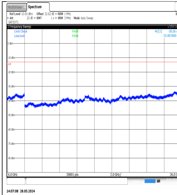
NTNV-N77-3700-3980-PC3-30-10-L-DFT-QPSK-Edge_1RB_Left-6000-26000-Ant1-PASS
