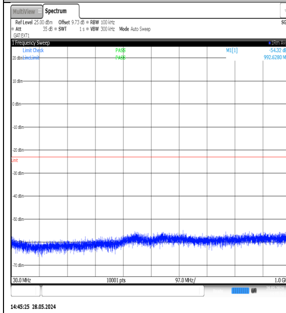
NTVN-N77-3700-3980-PC3-30-40-M-DFT-QPSK-Edge_1RB_Left-30-1000-Ant1-PASS
