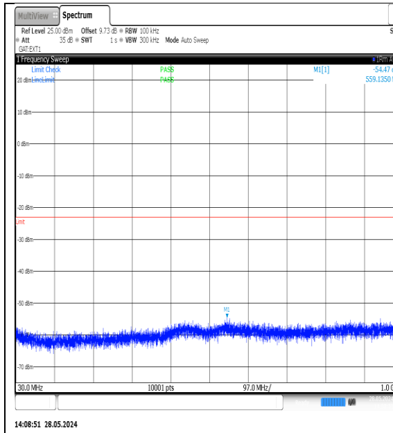
NTNV-N77-3700-3980-PC3-30-10-M-DFT-QPSK- Edge_1RB_Left-30-1000-Ant1-PASS
