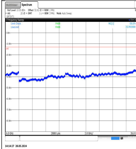
NTNV-N77-3700-3980-PC3-30-15-L-DFT-QPSK-Edge_1RB_Left-6000-26000-Ant1-PASS
