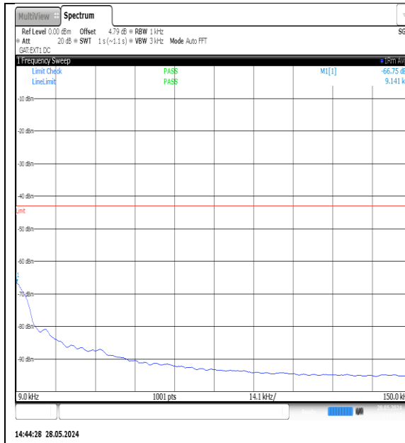
NTVN-N77-3700-3980-PC3-30-40-M-DFT-QPSK-Edge_1RB_Left-0.009-0.15-Ant1-PASS
