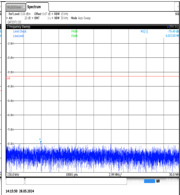
NTNV-N77-3700-3980-PC3-30-15-M-DFT-QPSK- Edge_1RB_Left-0.15-30-Ant1-PASS
