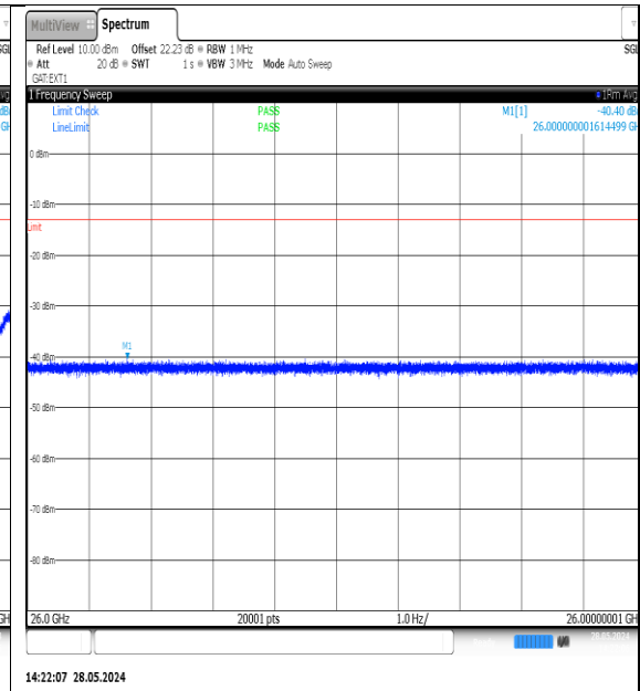
NTNV-N77-3700-3980-PC3-30-20-L-DFT-QPSK-Edge_1RB_Left-26000-40000-Ant1-PASS
