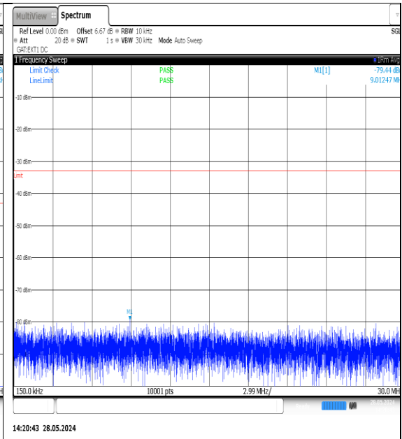
NTNV-N77-3700-3980-PC3-30-20-L-DFT-QPSK- Edge_1RB_Left-0.15-30-Ant1-PASS
