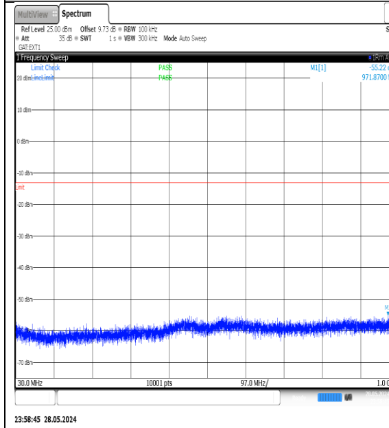
N78-3700-3800-PC3-30-100-M-DFT- QPSK-Edge_1RB_Left-30-1000-Ant1-PASS
