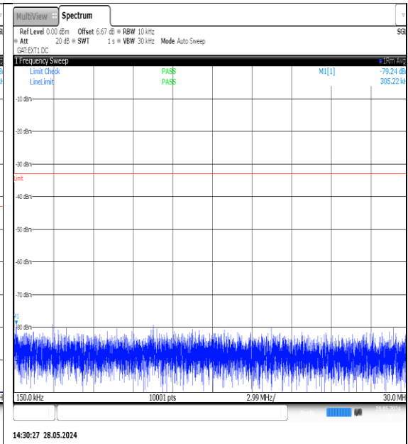
NTVN-N77-3700-3980-PC3-30-25-M-DFT-QPSK-Edge_1RB_Left-0.15-30-Ant1-PASS
