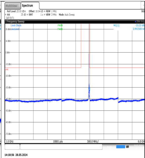
NTNV-N77-3700-3980-PC3-30-15-H-DFT-QPSK- Edge_1RB_Left-1000-6000-Ant1-PASS
