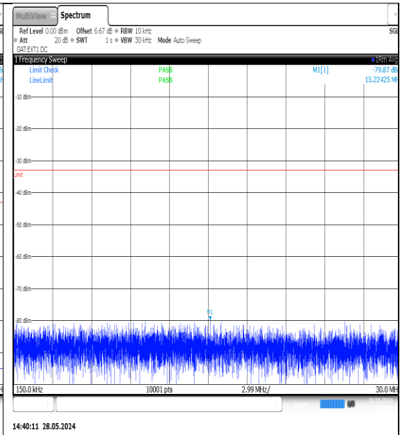
NTNV-N77-3700-3980-PC3-30-30-H-DFT-QPSK- Edge_1RB_Left-0.15-30-Ant1-PASS
