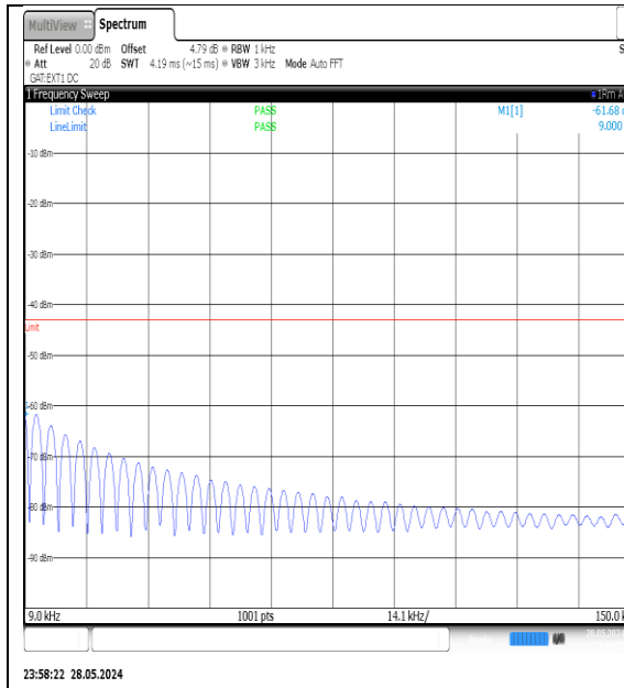
N78-3700-3800-PC3-30-100-M-DFT- QPSK-Edge_1RB_Left-0.009-0.15-Ant1-PASS
