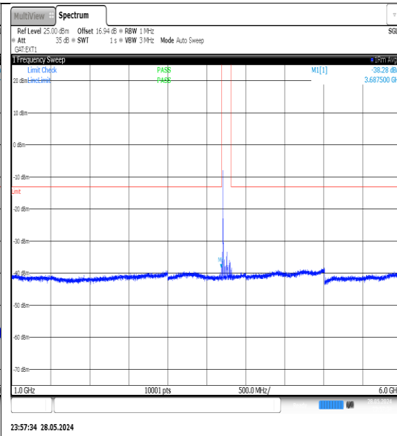
NTNV-N78-3700-3800-PC3-30-100-L-DFT-QPSK-Edge_1RB_Left-1000-6000-Ant1-PASS
