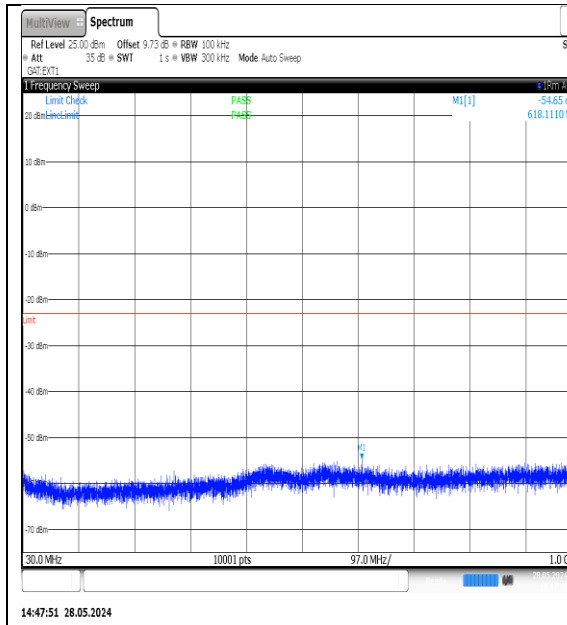
NTNV-N77-3700-3980-PC3-30-40-H-DFT-QPSK- Edge_1RB_Left-30-1000-Ant1-PASS
