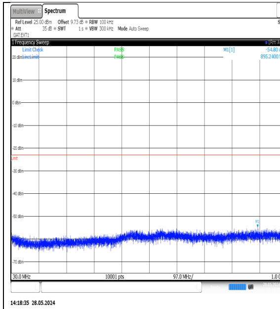
NTNV-N77-3700-3980-PC3-30-15-H-DFT-QPSK- Edge_1RB_Left-30-1000-Ant1-PASS
