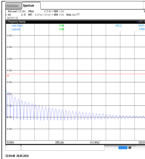
NTNV-N78-3700-3800-PC3-30-90-H-DFT-QPSK-Edge_1RB_Left-0.009-0.15-Ant1-PASS
