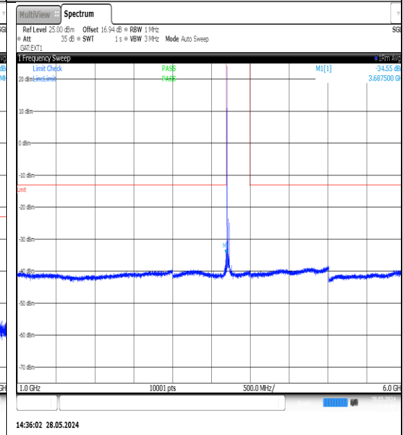
NTNV-N77-3700-3980-PC3-30-30-L-DFT-QPSK-Edge_1RB_Left-1000-6000-Ant1-PASS
