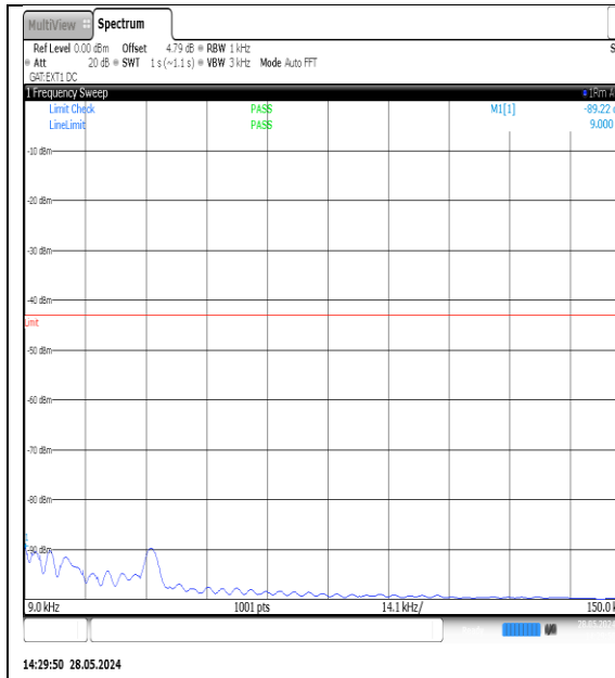
NTVN-N77-3700-3980-PC3-30-25-M-DFT-QPSK-Edge_1RB_Left-0.009-0.15-Ant1-PASS
