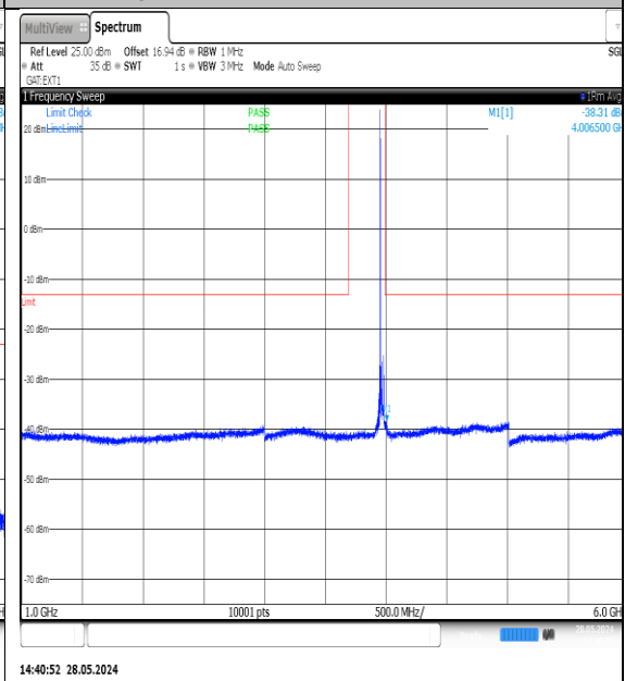
NTNV-N77-3700-3980-PC3-30-30-H-DFT-QPSK- Edge_1RB_Left-1000-6000-Ant1-PASS
