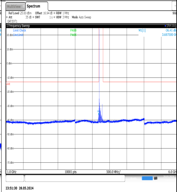
NTNV-N78-3700-3800-PC3-30-90-L-DFT-QPSK-Edge_1RB_Left-1000-6000-Ant1-PASS
