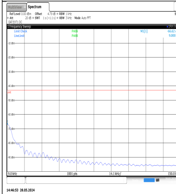
NTVN-N77-3700-3980-PC3-30-40-H-DFT-QPSK-Edge_1RB_Left-0.009-0.15-Ant1-PASS
