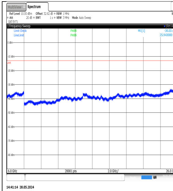
NTNV-N77-3700-3980-PC3-30-30-H-DFT-QPSK-Edge_1RB_Left-6000-26000-Ant1-PASS
