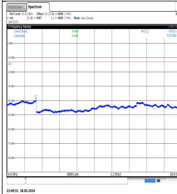
NTNV-N78-3700-3800-PC3-30-80-H-DFT-QPSK- Edge_1RB_Left-6000-18000-Ant1-PASS
