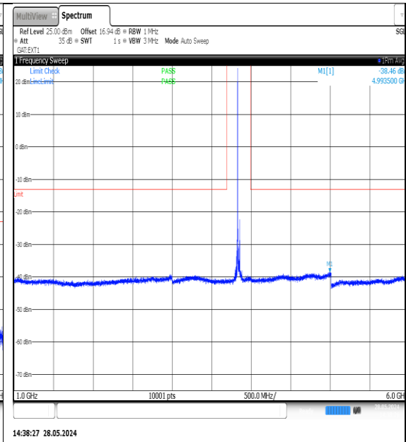
NTVN-N77-3700-3980-PC3-30-30-M-DFT-QPSK-Edge_1RB_Left-1000-6000-Ant1-PASS
