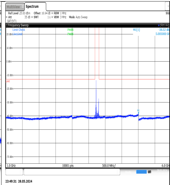
NTNV-N78-3700-3800-PC3-30-80-H-DFT-QPSK- Edge_1RB_Left-1000-6000-Ant1-PASS
