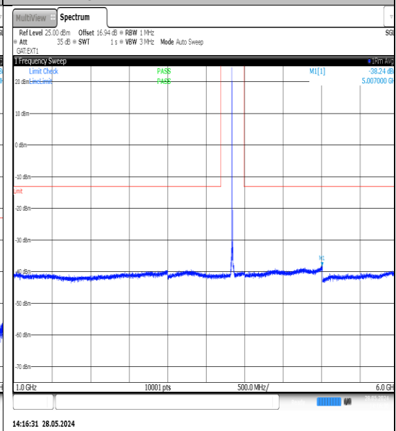
NTNV-N77-3700-3980-PC3-30-15-M-DFT-QPSK- Edge_1RB_Left-1000-6000-Ant1-PASS
