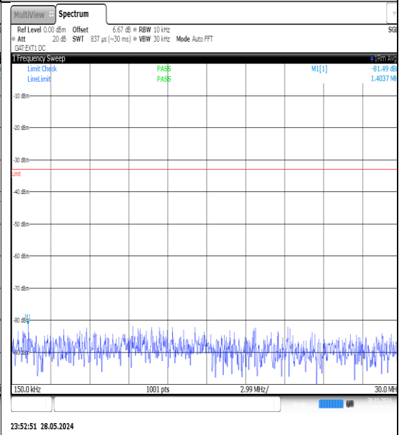
NTNV-N78-3700-3800-PC3-30-90-M-DFT-QPSK-Edge_1RB_Left-0.15-30-Ant1-PASS
