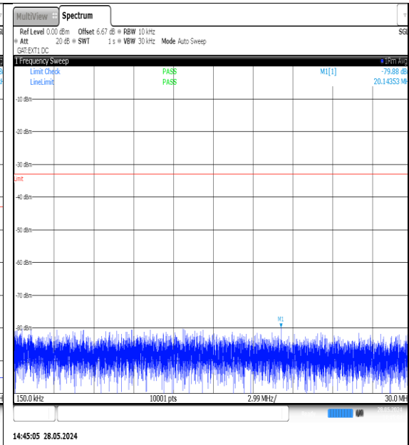
NTVN-N77-3700-3980-PC3-30-40-M-DFT-QPSK-Edge_1RB_Left-0.15-30-Ant1-PASS
