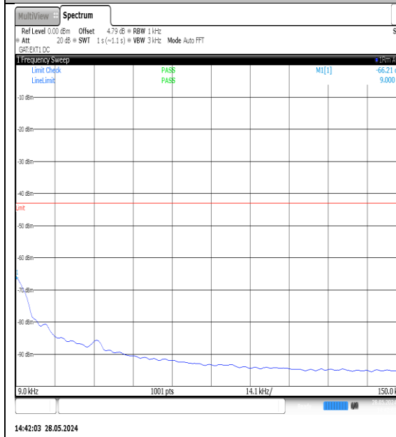
NTNV-N77-3700-3980-PC3-30-40-L-DFT-QPSK-Edge_1RB_Left-0.009-0.15-Ant1-PASS
