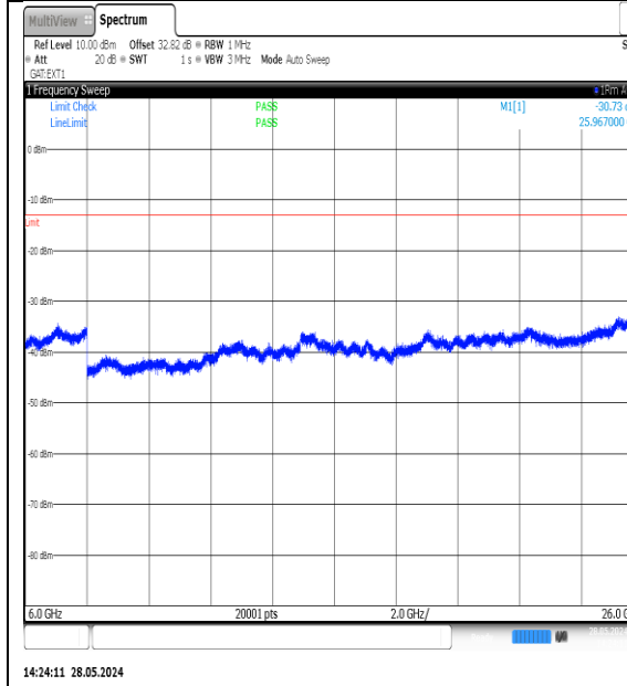
NTNV-N77-3700-3980-PC3-30-20-M-DFT-QPSK- Edge_1RB_Left-6000-26000-Ant1-PASS
