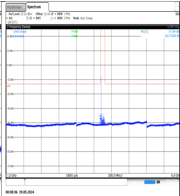
NTNV-N78-3700-3800-PC3-30-100-H-DFT-QPSK-Edge_1RB_Left-1000-6000-Ant1-PASS
