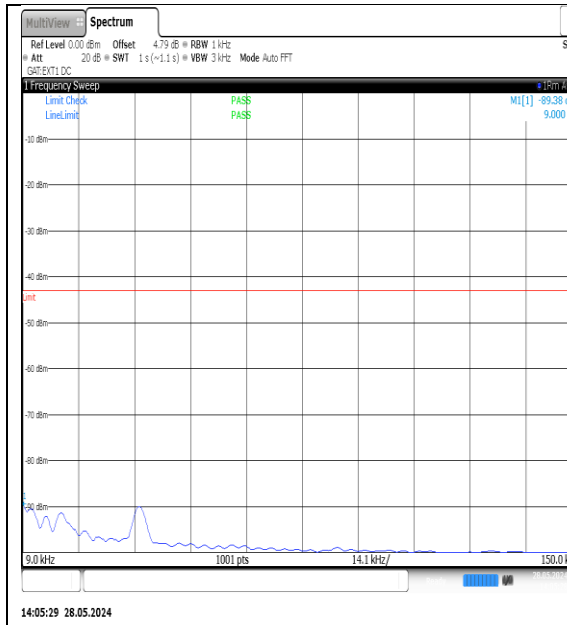
NTNV-N77-3700-3980-PC3-30-10-L-DFT-QPSK- Edge_1RB_Left-0.009-0.15-Ant1-PASS
