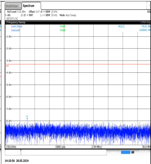
NTNV-N77-3700-3980-PC3-30-10-H-DFT-QPSK- Edge_1RB_Left-0.15-30-Ant1-PASS
