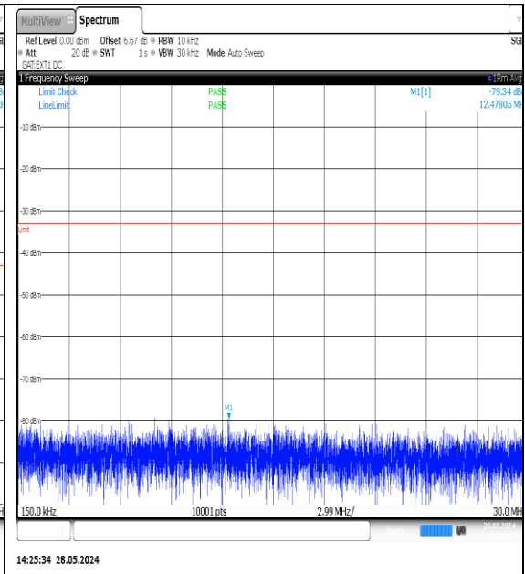
NTNV-N77-3700-3980-PC3-30-20-H-DFT-QPSK-Edge_1RB_Left-0.15-30-Ant1-PASS
