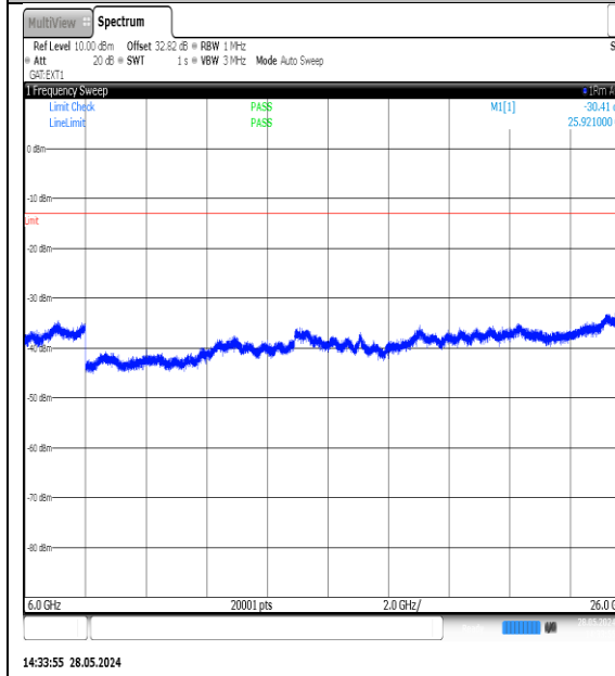
NTNV-N77-3700-3980-PC3-30-25-H-DFT-QPSK- Edge_1RB_Left-6000-26000-Ant1-PASS
