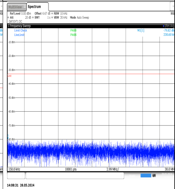
NTNV-N77-3700-3980-PC3-30-10-M-DFT-QPSK-Edge_1RB_Left-0.15-30-Ant1-PASS
