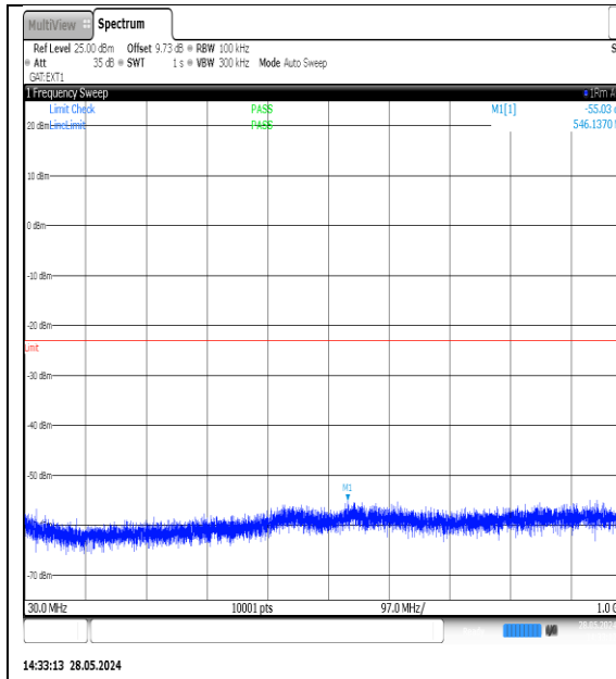
NTNV-N77-3700-3980-PC3-30-25-H-DFT-QPSK- Edge_1RB_Left-30-1000-Ant1-PASS
