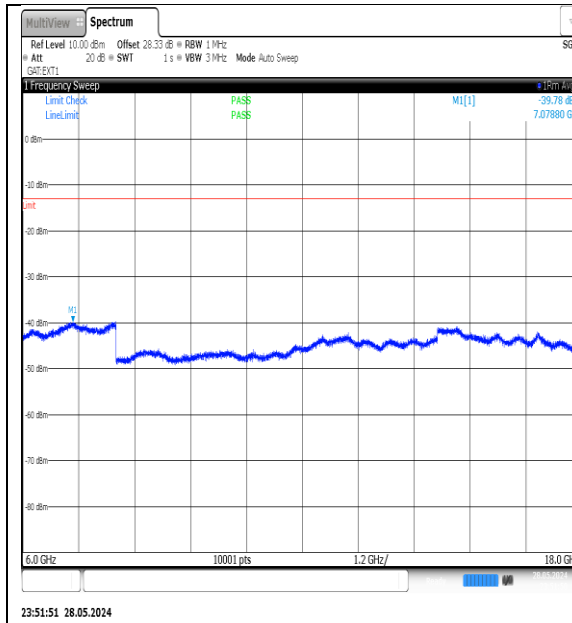
NTNV-N78-3700-3800-PC3-30-90-L-DFT-QPSK-Edge_1RB_Left-6000-18000-Ant1-PASS
