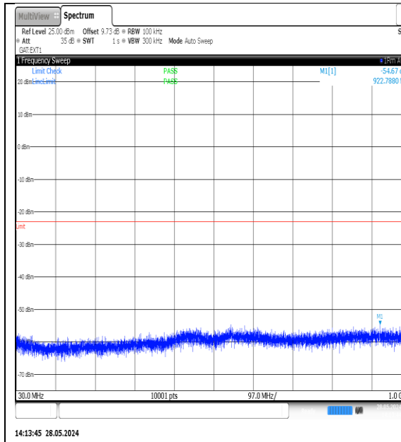
NTNV-N77-3700-3980-PC3-30-15-L-DFT-QPSK-Edge_1RB_Left-30-1000-Ant1-PASS
