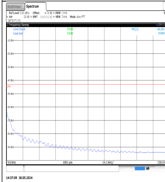
NTNV-N77-3700-3980-PC3-30-30-M-DFT-QPSK- Edge_1RB_Left-0.009-0.15-Ant1-PASS
