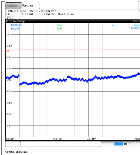
NTNV-N77-3700-3980-PC3-30-20-H-DFT-QPSK-Edge_1RB_Left-6000-26000-Ant1-PASS
