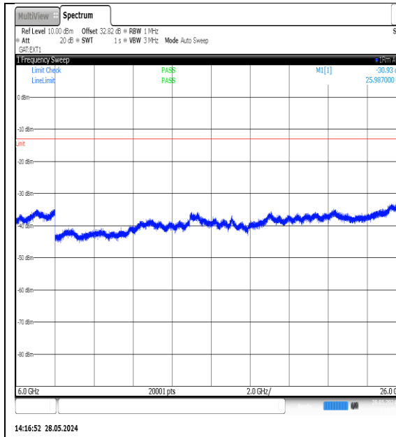
N77-3700-3980-PC3-30-15-M-DFT-QPSK- Edge_1RB_Left-6000-26000-Ant1-PASS
