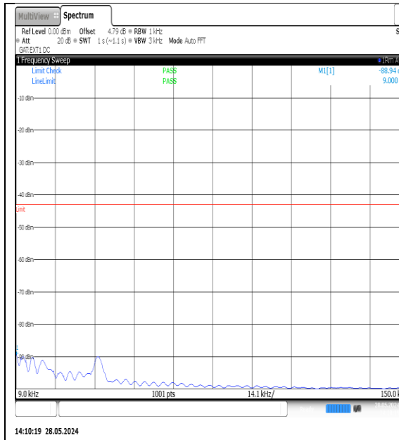
NTNV-N77-3700-3980-PC3-30-10-H-DFT-QPSK- Edge_1RB_Left-0.009-0.15-Ant1-PASS
