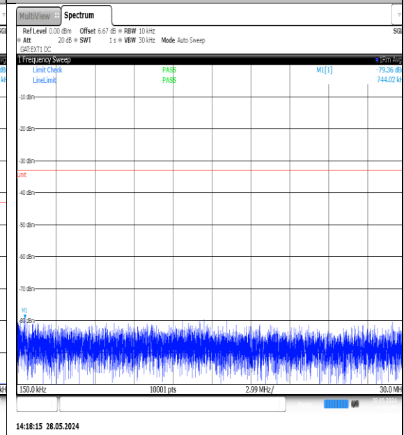
N77-3700-3980-PC3-30-15-H-DFT-QPSK- Edge_1RB_Left-0.15-30-Ant1-PASS
