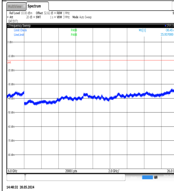
NTNV-N77-3700-3980-PC3-30-40-H-DFT-QPSK- Edge_1RB_Left-6000-26000-Ant1-PASS
