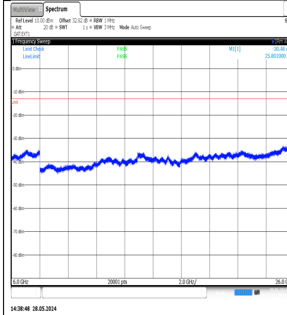
NTVN-N77-3700-3980-PC3-30-30-M-DFT-QPSK-Edge_1RB_Left-6000-26000-Ant1-PASS
