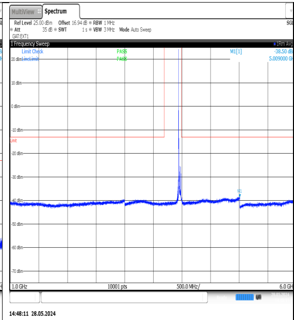
NTNV-N77-3700-3980-PC3-30-40-H-DFT-QPSK- Edge_1RB_Left-1000-6000-Ant1-PASS
