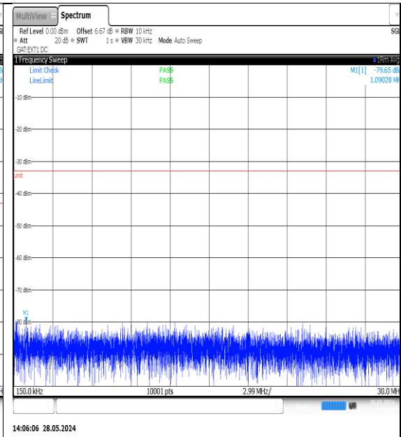
NTNV-N77-3700-3980-PC3-30-10-L-DFT-QPSK- Edge_1RB_Left-0.15-30-Ant1-PASS
