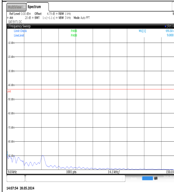
NTNV-N77-3700-3980-PC3-30-10-M-DFT-QPSK-Edge_1RB_Left-0.009-0.15-Ant1-PASS
