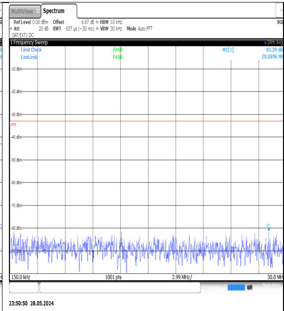
NTNV-N78-3700-3800-PC3-30-90-L-DFT-QPSK-Edge_1RB_Left-0.15-30-Ant1-PASS
