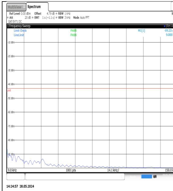
NTNV-N77-3700-3980-PC3-30-20-H-DFT-QPSK-Edge_1RB_Left-0.009-0.15-Ant1-PASS
