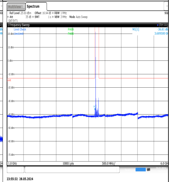
NTNV-N78-3700-3800-PC3-30-90-H-DFT-QPSK-Edge_1RB_Left-1000-6000-Ant1-PASS
