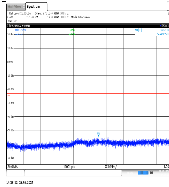
NTNV-N77-3700-3980-PC3-30-25-L-DFT-QPSK- Edge_1RB_Left-30-1000-Ant1-PASS
