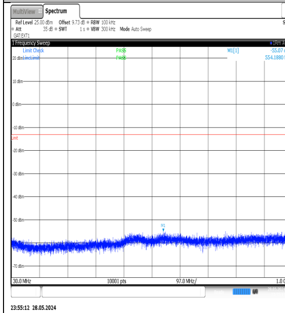
NTNV-N78-3700-3800-PC3-30-90-H-DFT-QPSK-Edge_1RB_Left-30-1000-Ant1-PASS
