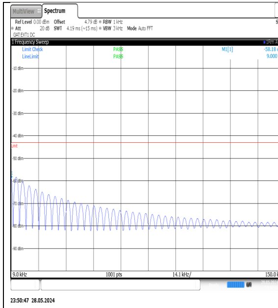
NTNV-N78-3700-3800-PC3-30-90-L-DFT-QPSK-Edge_1RB_Left-0.009-0.15-Ant1-PASS
