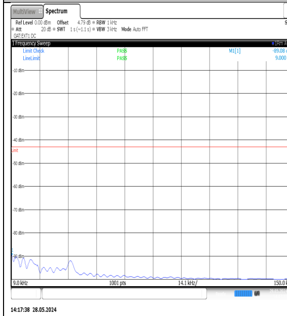
N77-3700-3980-PC3-30-15-H-DFT-QPSK- Edge_1RB_Left-0.009-0.15-Ant1-PASS
