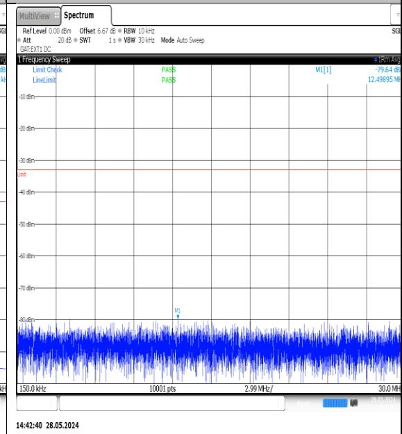
NTNV-N77-3700-3980-PC3-30-40-L-DFT-QPSK-Edge_1RB_Left-0.15-30-Ant1-PASS
