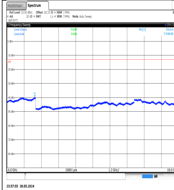
NTNV-N78-3700-3800-PC3-30-100-L-DFT-QPSK-Edge_1RB_Left-6000-18000-Ant1-PASS
