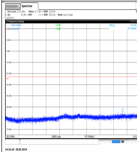
NTNV-N77-3700-3980-PC3-30-15-M-DFT-QPSK- Edge_1RB_Left-30-1000-Ant1-PASS
