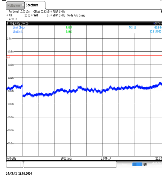
NTNV-N77-3700-3980-PC3-30-40-L-DFT-QPSK-Edge_1RB_Left-6000-26000-Ant1-PASS
