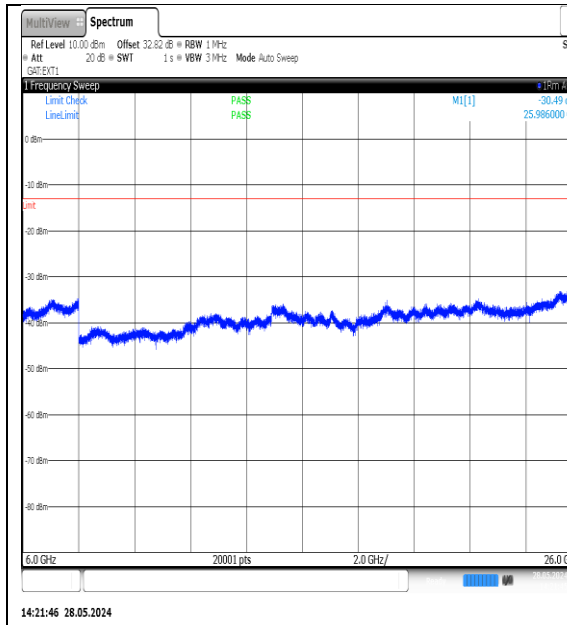
NTNV-N77-3700-3980-PC3-30-20-L-DFT-QPSK-Edge_1RB_Left-6000-26000-Ant1-PASS
