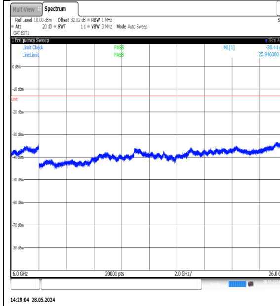
NTNV-N77-3700-3980-PC3-30-25-L-DFT-QPSK- Edge_1RB_Left-6000-26000-Ant1-PASS
