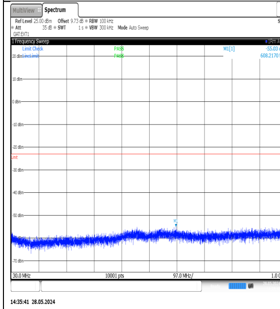
NTNV-N77-3700-3980-PC3-30-30-L-DFT-QPSK-Edge_1RB_Left-30-1000-Ant1-PASS
