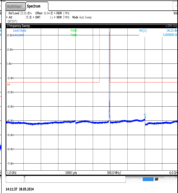
NTNV-N77-3700-3980-PC3-30-10-H-DFT-QPSK- Edge_1RB_Left-1000-6000-Ant1-PASS
