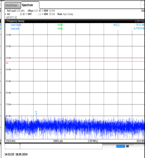
NTNV-N77-3700-3980-PC3-30-25-H-DFT-QPSK- Edge_1RB_Left-0.15-30-Ant1-PASS
