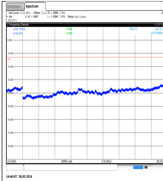
NTVN-N77-3700-3980-PC3-30-40-M-DFT-QPSK-Edge_1RB_Left-6000-26000-Ant1-PASS
