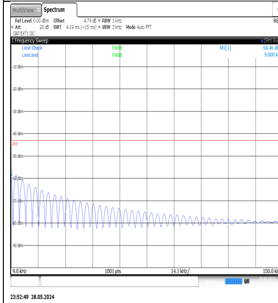
NTNV-N78-3700-3800-PC3-30-90-M-DFT-QPSK-Edge_1RB_Left-0.009-0.15-Ant1-PASS
