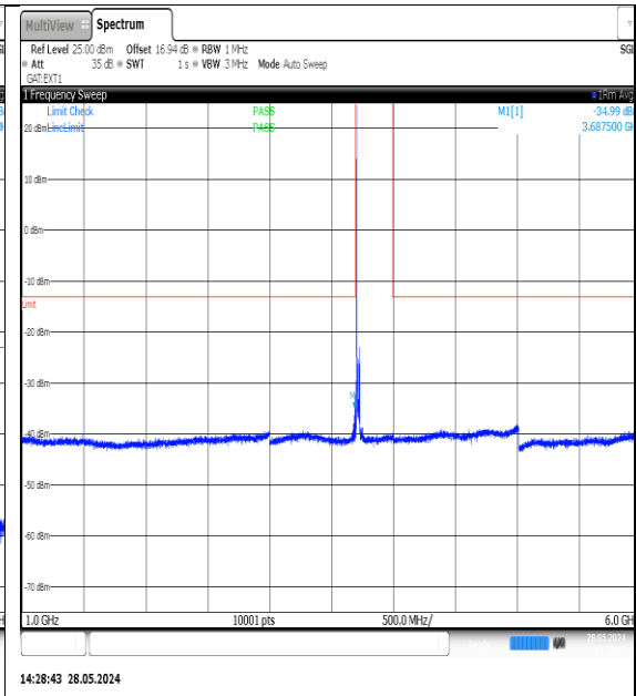
NTNV-N77-3700-3980-PC3-30-25-L-DFT-QPSK- Edge_1RB_Left-1000-6000-Ant1-PASS
