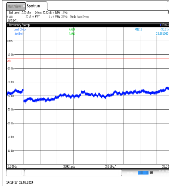
NTNV-N77-3700-3980-PC3-30-15-H-DFT-QPSK- Edge_1RB_Left-6000-26000-Ant1-PASS
