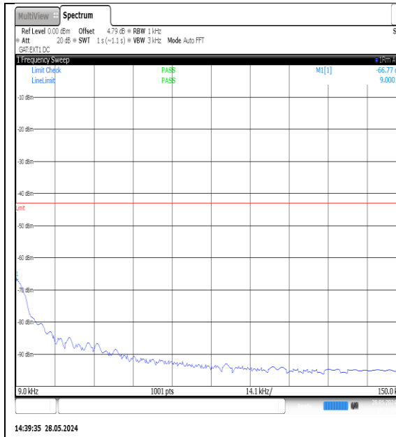
NTNV-N77-3700-3980-PC3-30-30-H-DFT-QPSK- Edge_1RB_Left-0.009-0.15-Ant1-PASS
