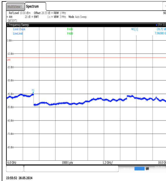
NTVN-N78-3700-3800-PC3-30-90-H-DFT-QPSK-Edge_1RB_Left-6000-18000-Ant1-PASS
