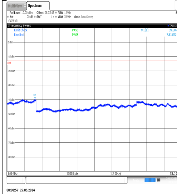
NTNV-N78-3700-3800-PC3-30-100-H-DFT-QPSK-Edge_1RB_Left-6000-18000-Ant1-PASS
