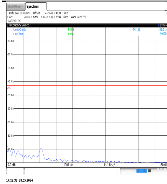
NTNV-N77-3700-3980-PC3-30-20-M-DFT-QPSK-Edge_1RB_Left-0.009-0.15-Ant1-PASS
