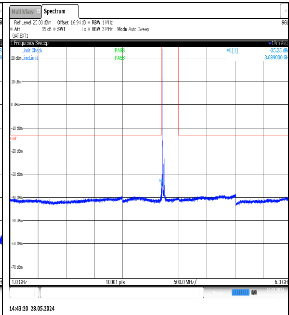
NTNV-N77-3700-3980-PC3-30-40-L-DFT-QPSK-Edge_1RB_Left-1000-6000-Ant1-PASS
