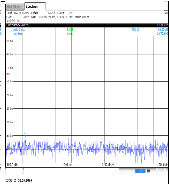
N78-3700-3800-PC3-30-100-M-DFT- QPSK-Edge_1RB_Left-0.15-30-Ant1-PASS
