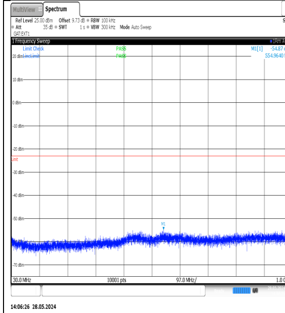
NTNV-N77-3700-3980-PC3-30-10-L-DFT-QPSK- Edge_1RB_Left-30-1000-Ant1-PASS
