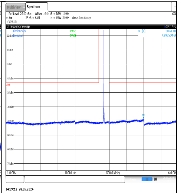
NTNV-N77-3700-3980-PC3-30-10-M-DFT-QPSK- Edge_1RB_Left-1000-6000-Ant1-PASS
