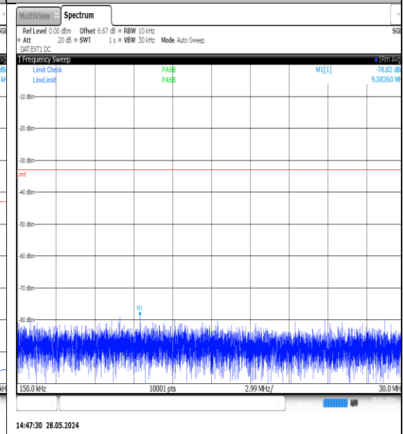
NTVN-N77-3700-3980-PC3-30-40-H-DFT-QPSK-Edge_1RB_Left-0.15-30-Ant1-PASS
