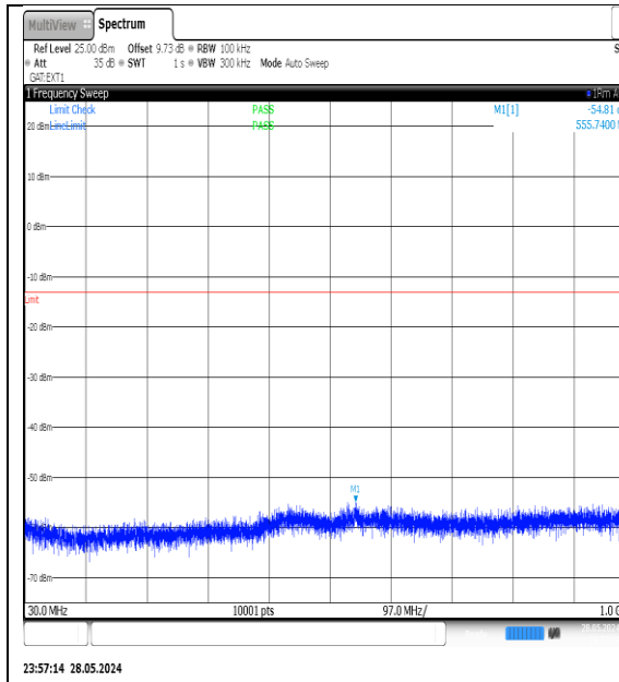
NTNV-N78-3700-3800-PC3-30-100-L-DFT-QPSK-Edge_1RB_Left-30-100-Ant1-PASS
