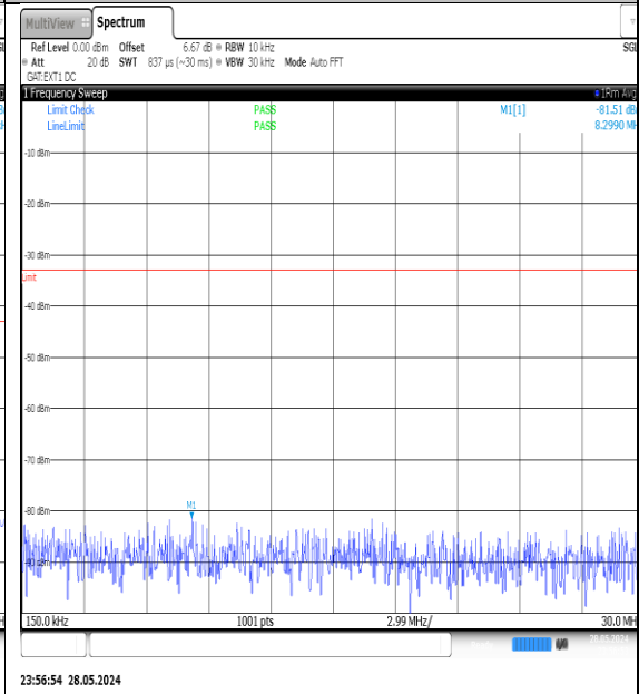
NTVN-N78-3700-3800-PC3-30-100-L-DFT-QPSK-Edge_1RB_Left-0.15-30-Ant1-PASS
