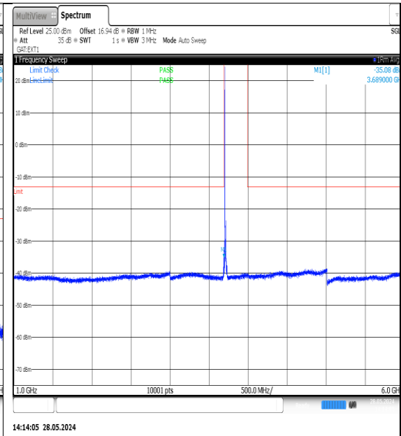
NTNV-N77-3700-3980-PC3-30-15-L-DFT-QPSK-Edge_1RB_Left-1000-6000-Ant1-PASS
