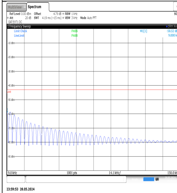
N78-3700-3800-PC3-30-100-H-DFT-QPSK-Edge_1RB_Left-0.009-0.15-Ant1-PASS
