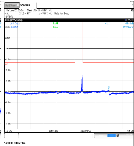
NTNV-N77-3700-3980-PC3-30-25-H-DFT-QPSK- Edge_1RB_Left-1000-6000-Ant1-PASS
