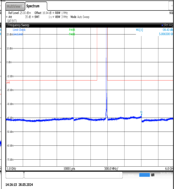
NTNV-N77-3700-3980-PC3-30-20-H-DFT-QPSK-Edge_1RB_Left-1000-6000-Ant1-PASS
