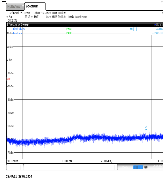
NTNV-N78-3700-3800-PC3-30-80-H-DFT-QPSK- Edge_1RB_Left-30-1000-Ant1-PASS
