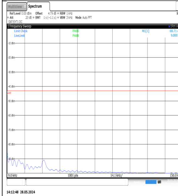
NTNV-N77-3700-3980-PC3-30-15-L-DFT-QPSK-Edge_1RB_Left-0.009-0.15-Ant1-PASS
