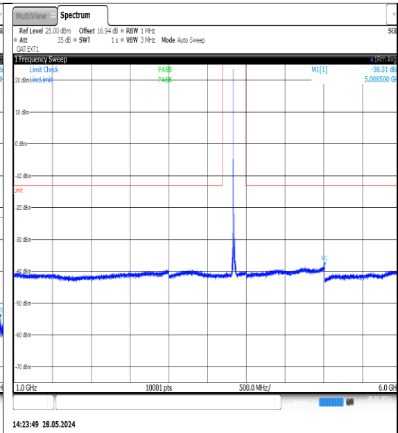
NTNV-N77-3700-3980-PC3-30-20-M-DFT-QPSK- Edge_1RB_Left-1000-6000-Ant1-PASS
