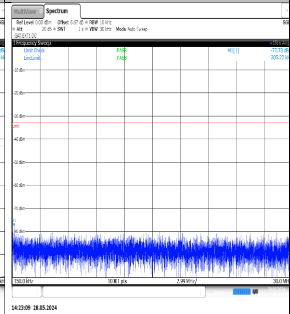
NTNV-N77-3700-3980-PC3-30-20-M-DFT-QPSK-Edge_1RB_Left-0.15-30-Ant1-PASS
