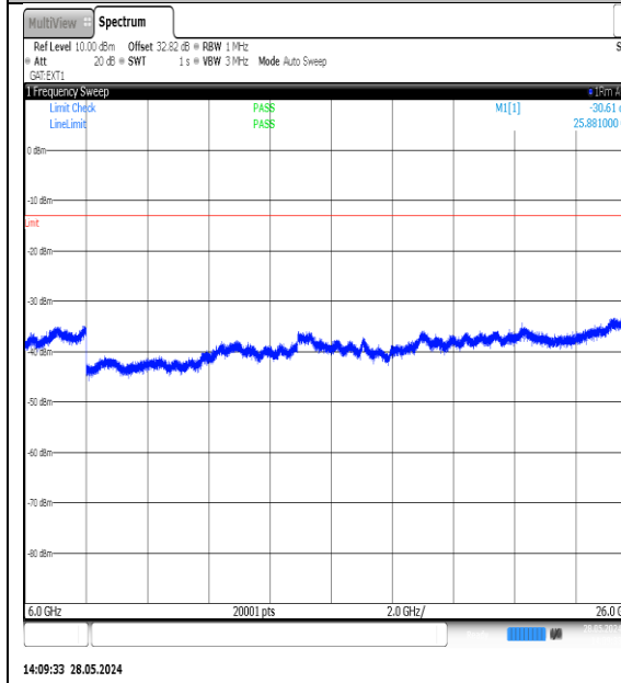
NTNV-N77-3700-3980-PC3-30-10-M-DFT-QPSK- Edge_1RB_Left-6000-26000-Ant1-PASS
