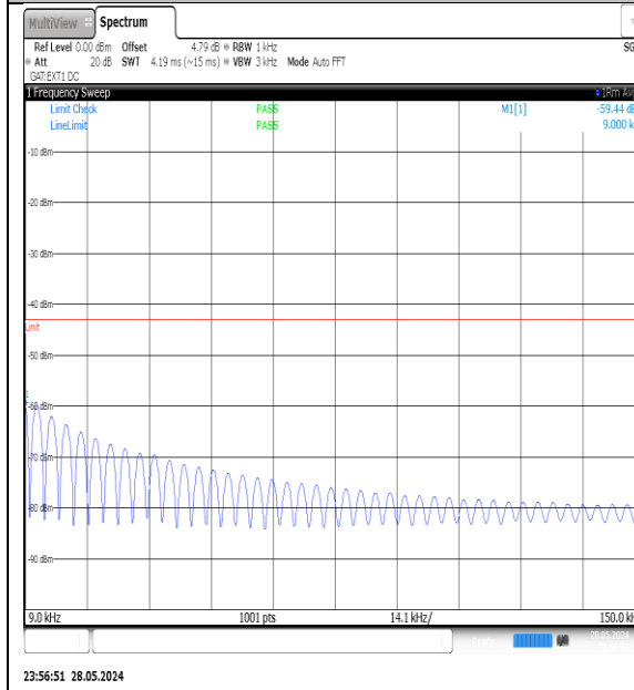
NTVN-N78-3700-3800-PC3-30-100-L-DFT-QPSK-Edge_1RB_Left-0.009-0.15-Ant1-PASS
