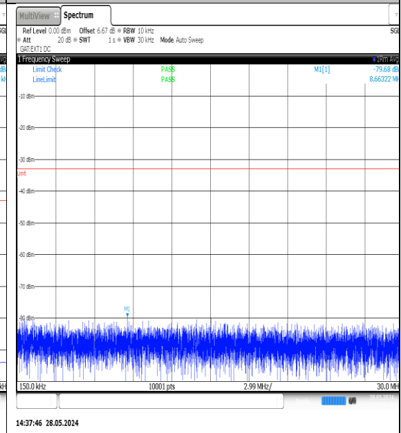
NTNV-N77-3700-3980-PC3-30-30-M-DFT-QPSK- Edge_1RB_Left-0.15-30-Ant1-PASS
