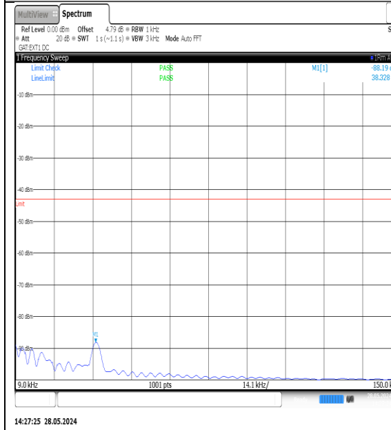
NTNV-N77-3700-3980-PC3-30-25-L-DFT-QPSK-Edge_1RB_Left-0.009-0.15-Ant1-PASS
