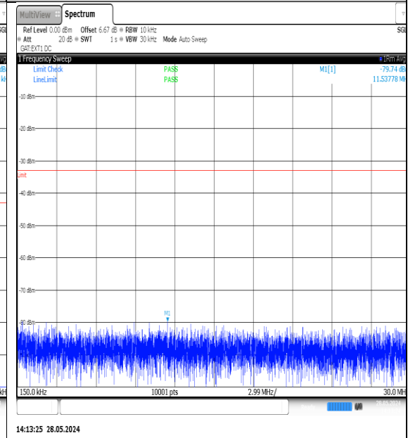
NTNV-N77-3700-3980-PC3-30-15-L-DFT-QPSK-Edge_1RB_Left-0.15-30-Ant1-PASS
