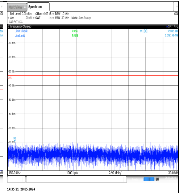
NTNV-N77-3700-3980-PC3-30-30-L-DFT-QPSK-Edge_1RB_Left-0.15-30-Ant1-PASS
