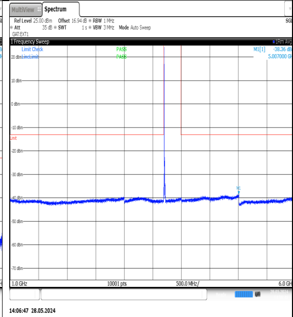
NTNV-N77-3700-3980-PC3-30-10-L-DFT-QPSK- Edge_1RB_Left-1000-6000-Ant1-PASS
