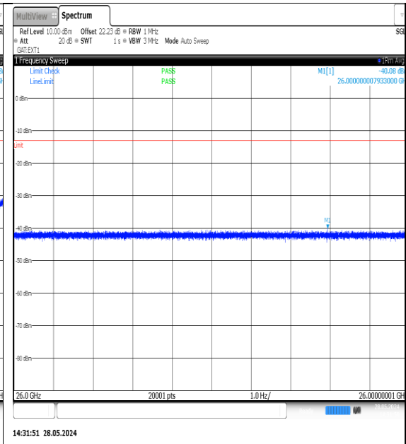
NTNV-N77-3700-3980-PC3-30-25-M-DFT-QPSK- Edge_1RB_Left-26000-40000-Ant1-PASS
