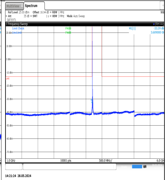
NTNV-N77-3700-3980-PC3-30-20-L-DFT-QPSK- Edge_1RB_Left-1000-6000-Ant1-PASS
