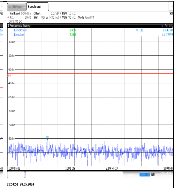
NTNV-N78-3700-3800-PC3-30-90-H-DFT-QPSK-Edge_1RB_Left-0.15-30-Ant1-PASS
