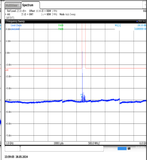
N78-3700-3800-PC3-30-100-M-DFT- QPSK-Edge_1RB_Left-1000-6000-Ant1-PASS
