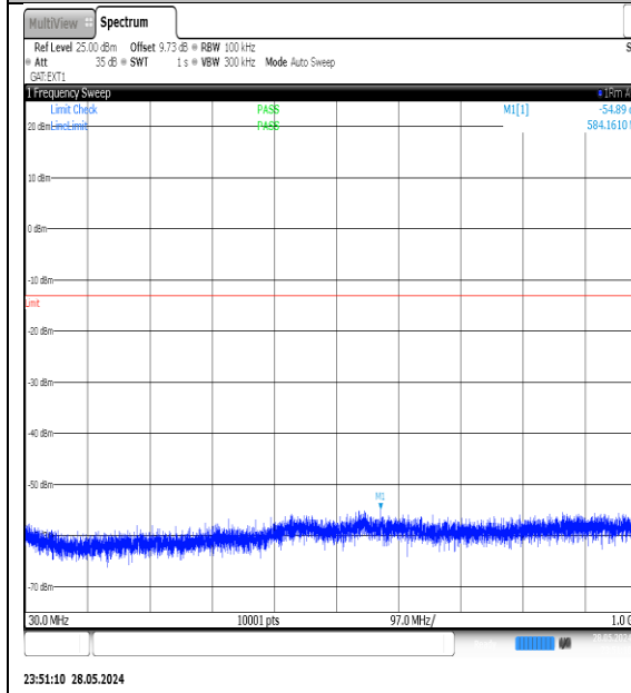
NTNV-N78-3700-3800-PC3-30-90-L-DFT-QPSK-Edge_1RB_Left-30-1000-Ant1-PASS
