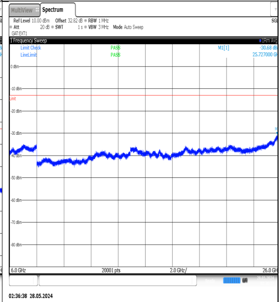
NTNV-N77-3450-3550-PC3-30-80-M-DFT-QPSK- Edge_1RB_Left-6000-26000-Ant1-PASS
