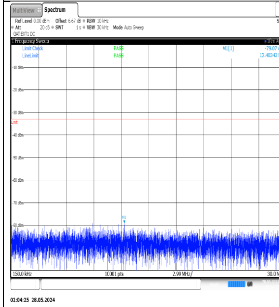
NTVN-N77-3450-3550-PC3-30-40-H-DFT-QPSK-Edge_1RB_Left-0.15-30-Ant1-PASS
