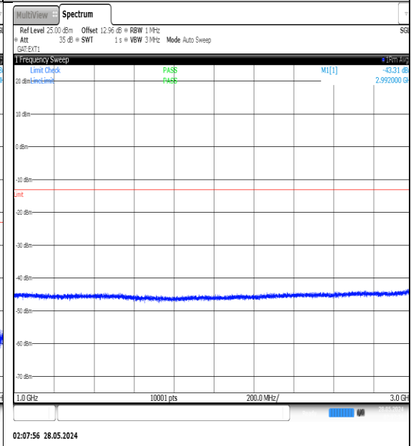
NTNV-N77-3450-3550-PC3-30-50-L-DFT-QPSK-Edge_1RB_Left-1000-3000-Ant1-PASS
