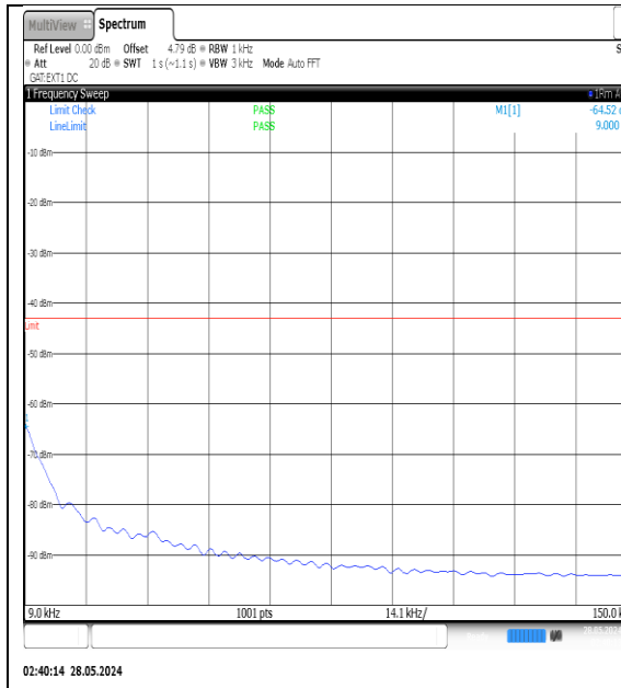
NTNV-N77-3450-3550-PC3-30-90-L-DFT-QPSK-Edge_1RB_Left-0.009-0.15-Ant1-PASS
