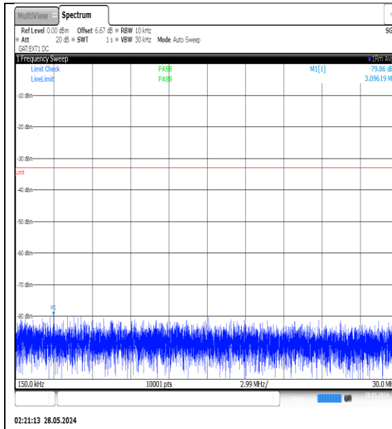
NTNV-N77-3450-3550-PC3-30-60-H-DFT-QPSK- Edge_1RB_Left-0.15-30-Ant1-PASS
