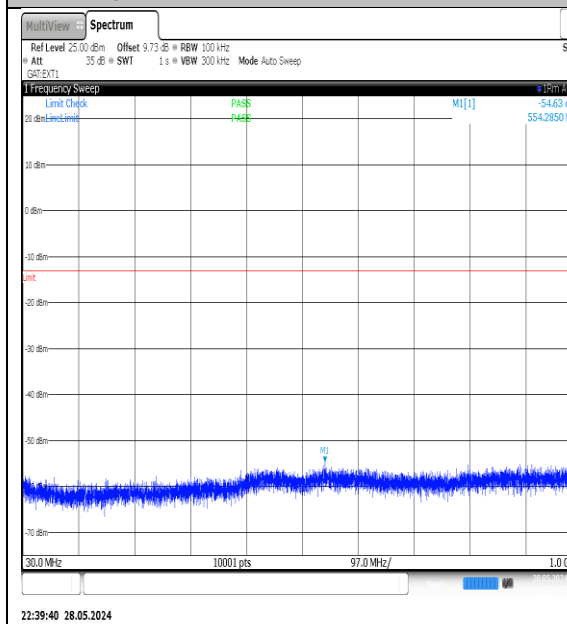
NTNV-N78-3700-3800-PC3-30-10-H-DFT-QPSK- Edge_1RB_Left-30-1000-Ant1-PASS
