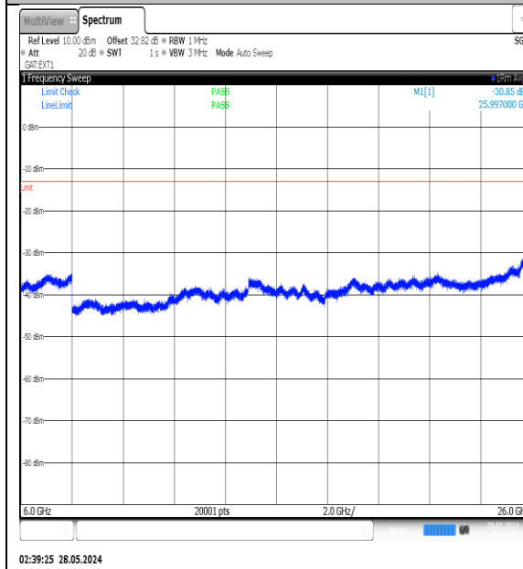
NTNV-N77-3450-3550-PC3-30-80-H-DFT-QPSK-Edge_1RB_Left-6000-26000-Ant1-PASS
