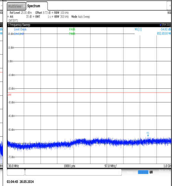
NTVN-N77-3450-3550-PC3-30-40-H-DFT-QPSK-Edge_1RB_Left-30-1000-Ant1-PASS
