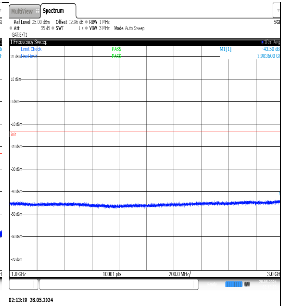
NTNV-N77-3450-3550-PC3-30-50-H-DFT-QPSK- Edge_1RB_Left-1000-3000-Ant1-PASS
