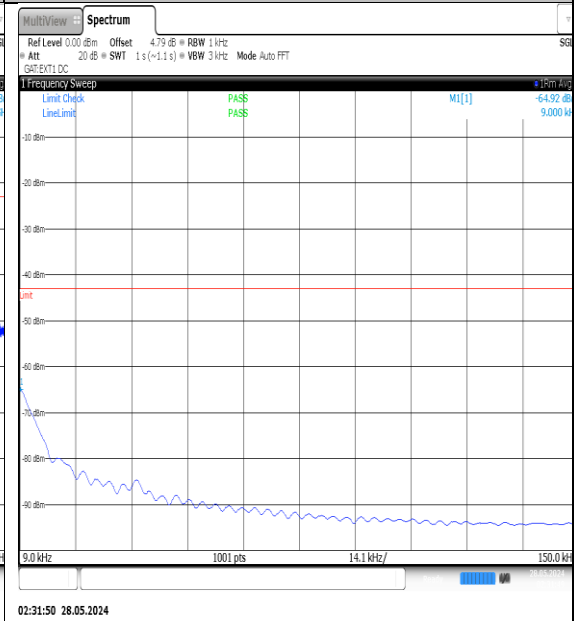
NTNV-N77-3450-3550-PC3-30-80-L-DFT-QPSK- Edge_1RB_Left-0.009-0.15-Ant1-PASS
