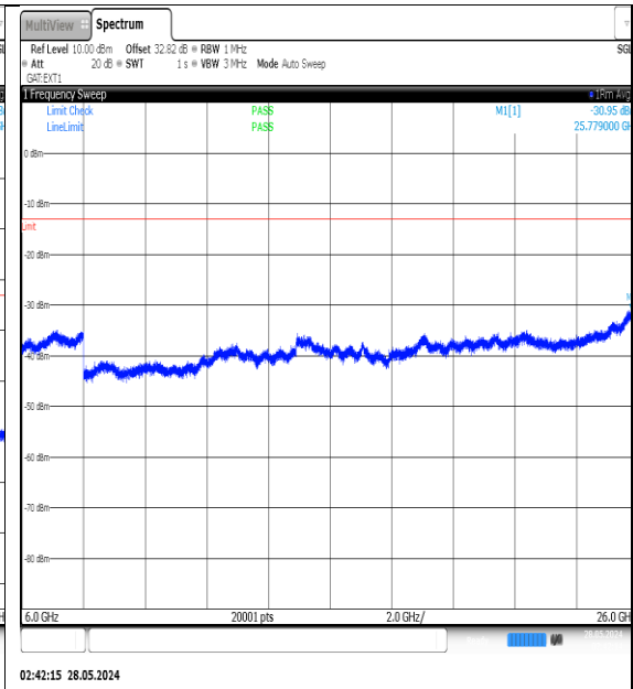
NTNV-N77-3450-3550-PC3-30-90-L-DFT-QPSK- Edge_1RB_Left-6000-26000-Ant1-PASS
