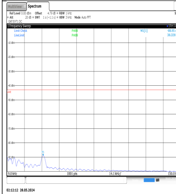
NTVN-N77-3450-3550-PC3-30-50-H-DFT-QPSK-Edge_1RB_Left-0.009-0.15-Ant1-PASS
