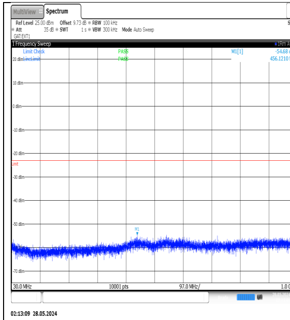
NTNV-N77-3450-3550-PC3-30-50-H-DFT-QPSK- Edge_1RB_Left-30-1000-Ant1-PASS
