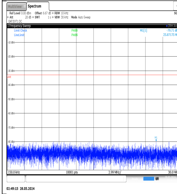
NTNV-N77-3450-3550-PC3-30-100-M-DFT-QPSK-Edge_1RB_Left-0.15-30-Ant1-PASS
