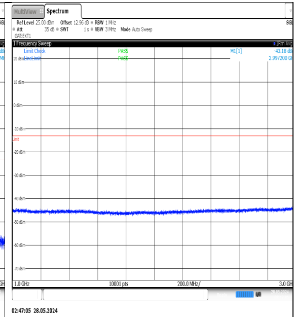
NTNV-N77-3450-3550-PC3-30-90-H-DFT-QPSK- Edge_1RB_Left-1000-3000-Ant1-PASS
