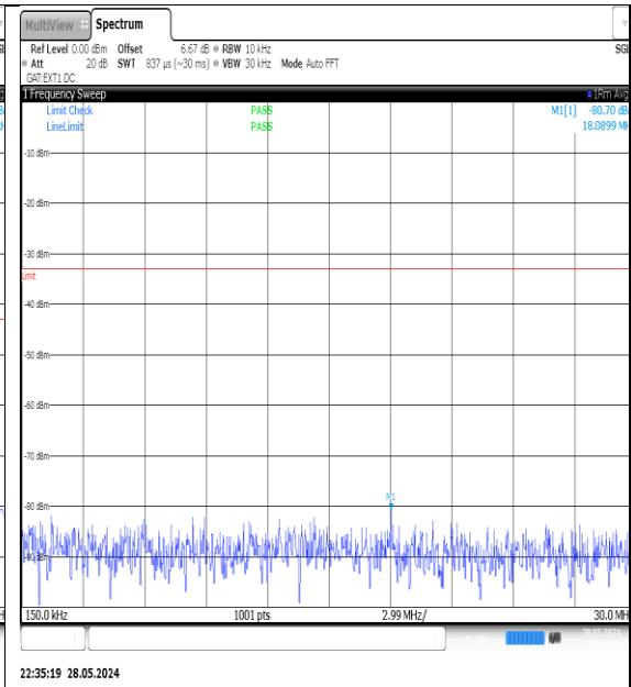
NTNV-N78-3700-3800-PC3-30-10-L-DFT-QPSK- Edge_1RB_Left-0.15-30-Ant1-PASS
