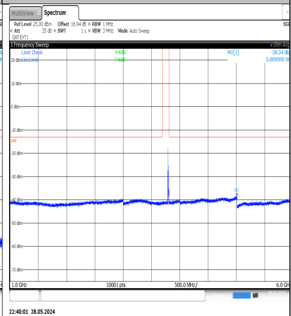
NTNV-N78-3700-3800-PC3-30-10-H-DFT-QPSK- Edge_1RB_Left-1000-6000-Ant1-PASS
