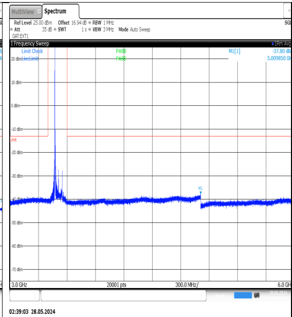
NTNV-N77-3450-3550-PC3-30-80-H-DFT-QPSK-Edge_1RB_Left-3000-6000-Ant1-PASS
