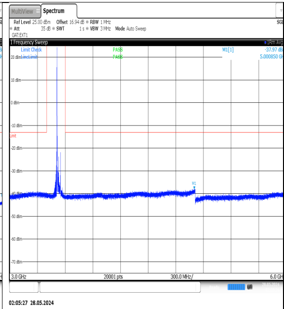
NTNV-N77-3450-3550-PC3-30-40-H-DFT-QPSK-Edge_1RB_Left-3000-6000-Ant1-PASS
