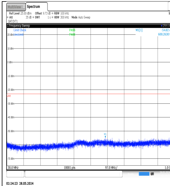
NTNV-N77-3450-3550-PC3-30-70-L-DFT-QPSK- Edge_1RB_Left-30-1000-Ant1-PASS
