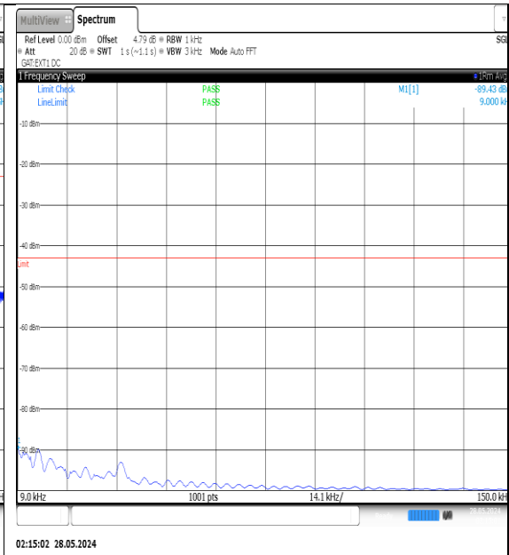
NTNV-N77-3450-3550-PC3-30-60-L-DFT-QPSK-Edge_1RB_Left-0.009-0.15-Ant1-PASS
