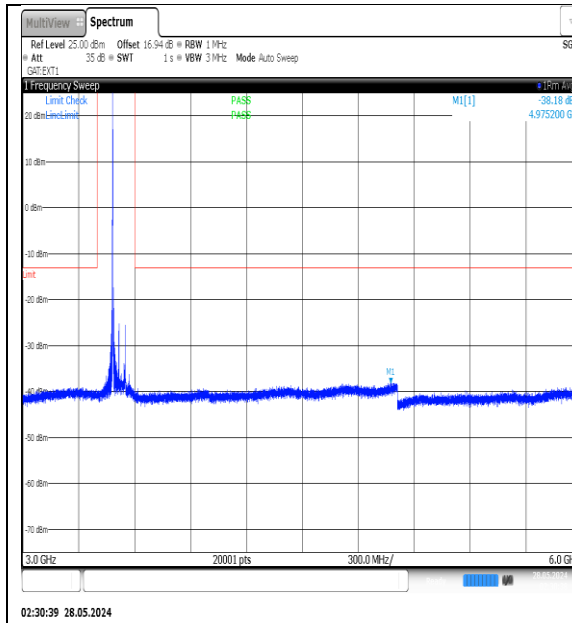
NTNV-N77-3450-3550-PC3-30-70-H-DFT-QPSK- Edge_1RB_Left-3000-6000-Ant1-PASS
