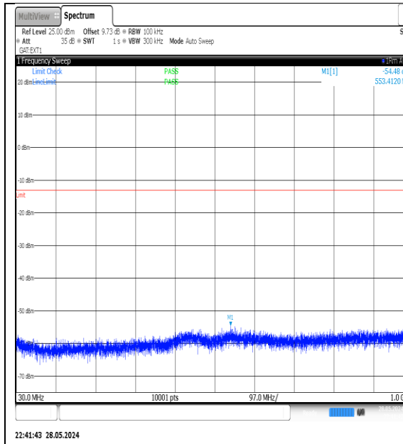
NTNV-N78-3700-3800-PC3-30-15-L-DFT-QPSK- Edge_1RB_Left-30-1000-Ant1-PASS
