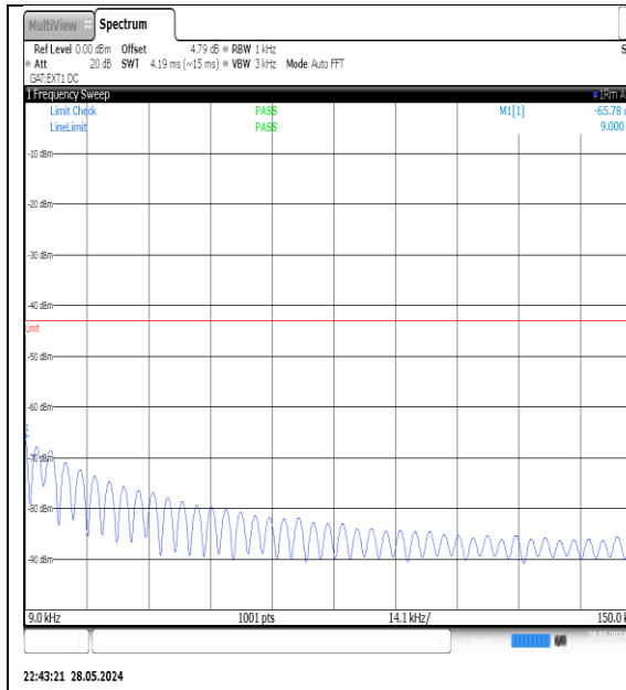
NTVN-N78-3700-3800-PC3-30-15-M-DFT-QPSK-Edge_1RB_Left-0.009-0.15-Ant1-PASS
