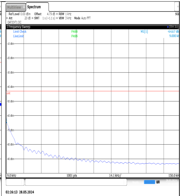
NTNV-N77-3450-3550-PC3-30-70-M-DFT-QPSK-Edge_1RB_Left-0.009-0.15-Ant1-PASS
