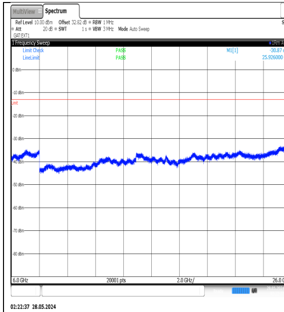
NTNV-N77-3450-3550-PC3-30-60-H-DFT-QPSK-Edge_1RB_Left-6000-26000-Ant1-PASS
