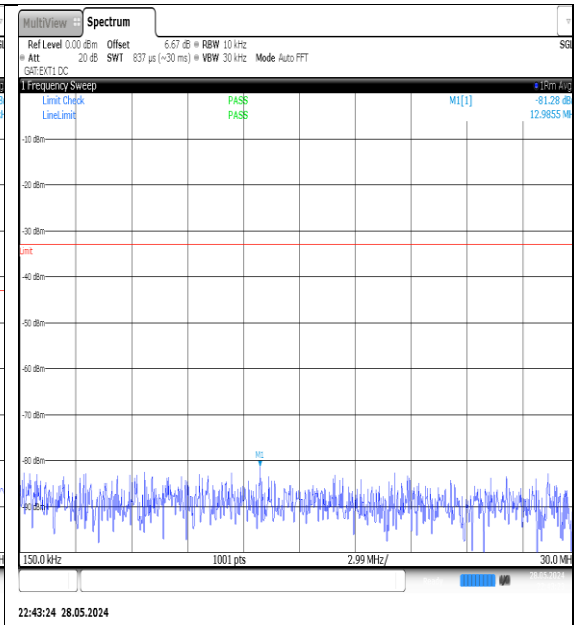
NTVN-N78-3700-3800-PC3-30-15-M-DFT-QPSK-Edge_1RB_Left-0.15-30-Ant1-PASS
