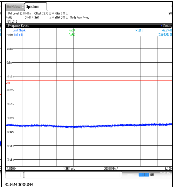
NTNV-N77-3450-3550-PC3-30-70-L-DFT-QPSK- Edge_1RB_Left-1000-3000-Ant1-PASS
