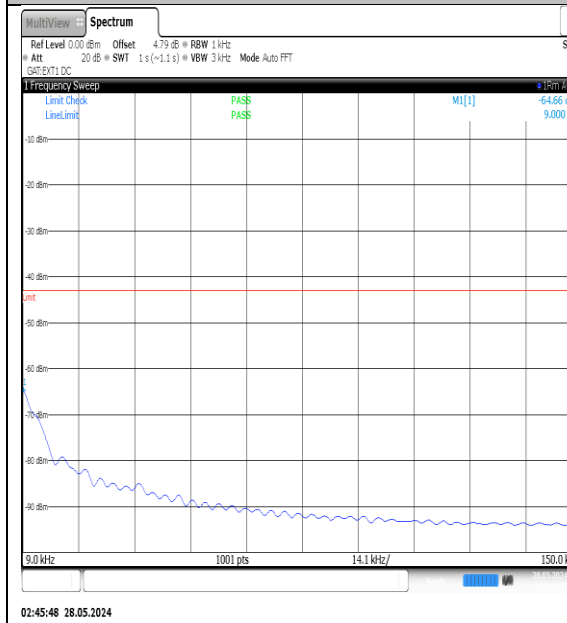
NTVN-N77-3450-3550-PC3-30-90-H-DFT-QPSK-Edge_1RB_Left-0.009-0.15-Ant1-PASS
