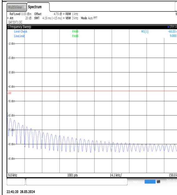
NTVN-N78-3700-3800-PC3-30-15-L-DFT-QPSK-Edge_1RB_Left-0.009-0.15-Ant1-PASS
