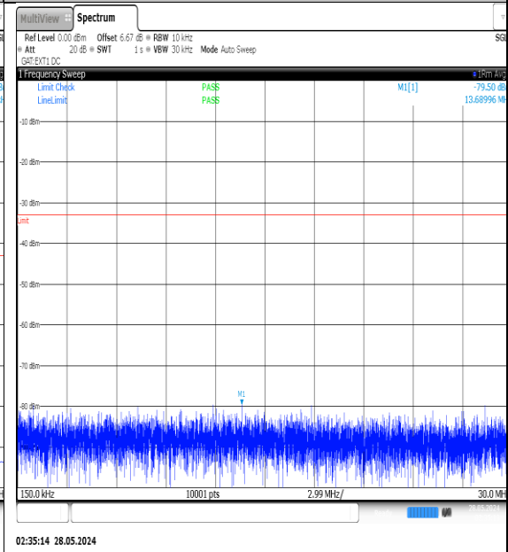
NTNV-N77-3450-3550-PC3-30-80-M-DFT-QPSK- Edge_1RB_Left-0.15-30-Ant1-PASS
