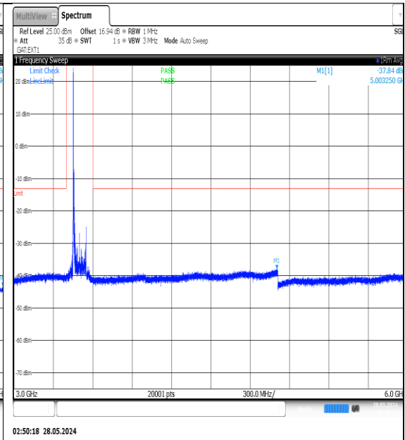
N77-3450-3550-PC3-30-100-M-DFT- QPSK-Edge_1RB_Left-3000-6000-Ant1-PASS
