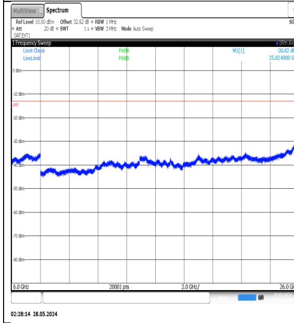
NTNV-N77-3450-3550-PC3-30-70-M-DFT-QPSK-Edge_1RB_Left-6000-26000-Ant1-PASS
