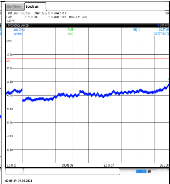
NTNV-N77-3450-3550-PC3-30-50-L-DFT-QPSK- Edge_1RB_Left-6000-26000-Ant1-PASS
