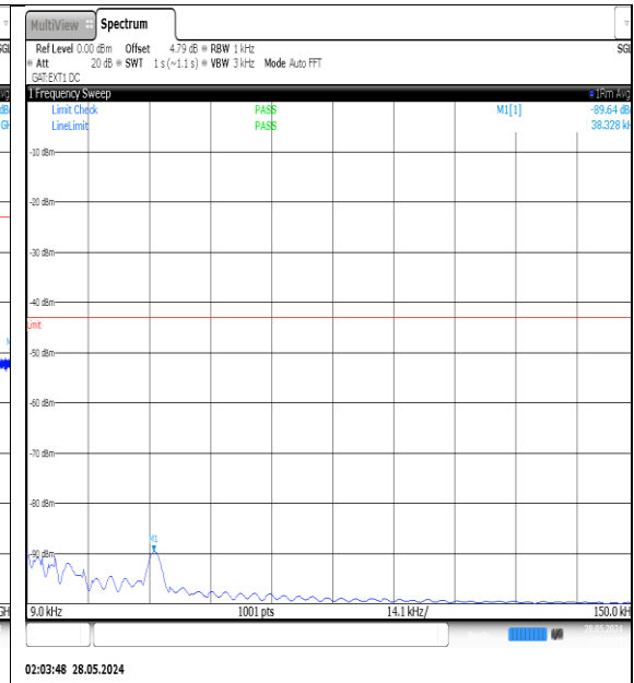
NTVN-N77-3450-3550-PC3-30-40-H-DFT-QPSK-Edge_1RB_Left-0.009-0.15-Ant1-PASS
