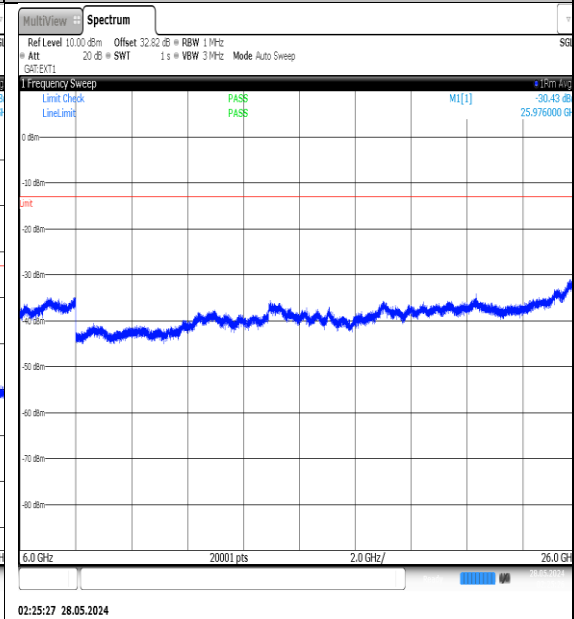
NTNV-N77-3450-3550-PC3-30-70-L-DFT-QPSK- Edge_1RB_Left-6000-26000-Ant1-PASS
