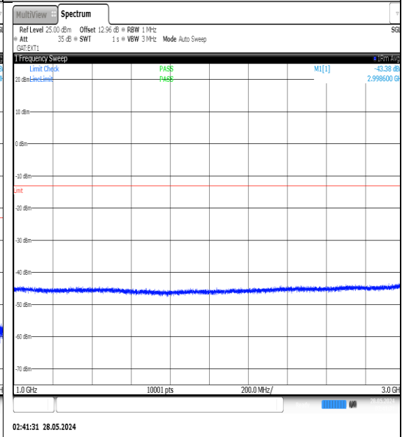
NTNV-N77-3450-3550-PC3-30-90-L-DFT-QPSK-Edge_1RB_Left-1000-3000-Ant1-PASS
