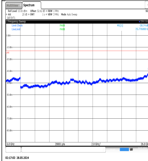
NTNV-N77-3450-3550-PC3-30-60-L-DFT-QPSK- Edge_1RB_Left-6000-26000-Ant1-PASS
