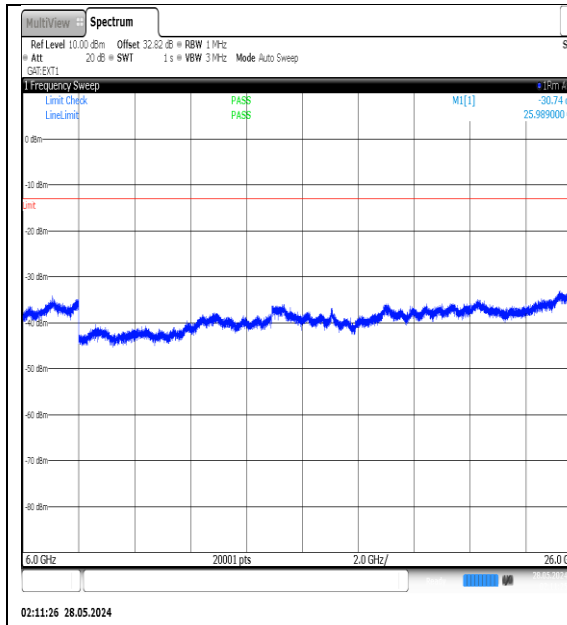
NTVN-N77-3450-3550-PC3-30-50-M-DFT-QPSK-Edge_1RB_Left-6000-26000-Ant1-PASS
