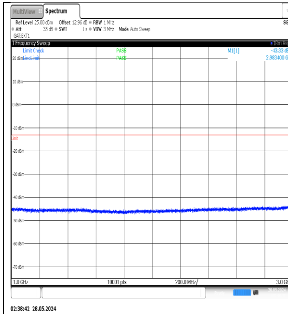
NTNV-N77-3450-3550-PC3-30-80-H-DFT-QPSK-Edge_1RB_Left-1000-3000-Ant1-PASS
