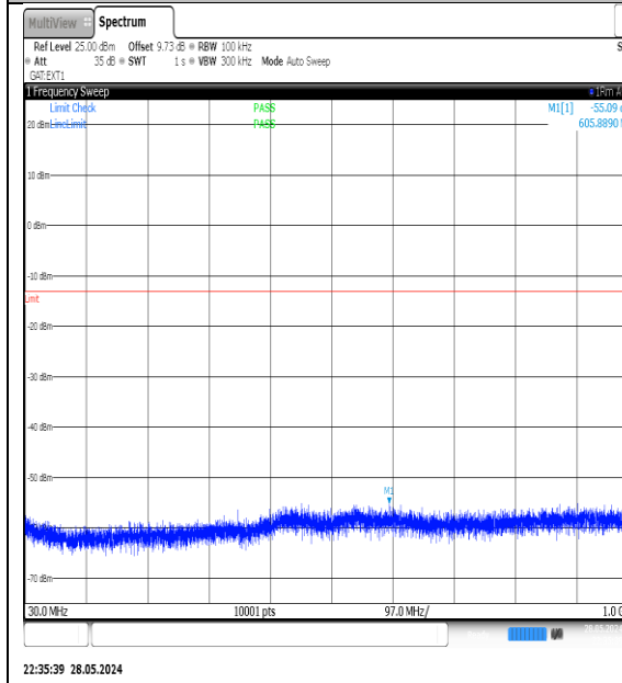
NTNV-N78-3700-3800-PC3-30-10-L-DFT-QPSK- Edge_1RB_Left-30-1000-Ant1-PASS
