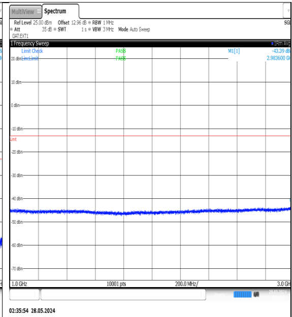
NTNV-N77-3450-3550-PC3-30-80-M-DFT-QPSK- Edge_1RB_Left-1000-3000-Ant1-PASS
