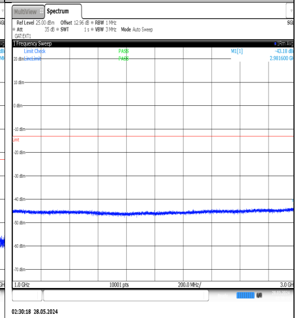
NTNV-N77-3450-3550-PC3-30-70-H-DFT-QPSK- Edge_1RB_Left-1000-3000-Ant1-PASS
