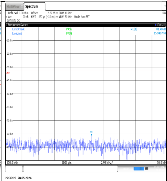
NTNV-N78-3700-3800-PC3-30-10-H-DFT-QPSK- Edge_1RB_Left-0.15-30-Ant1-PASS
