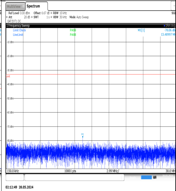
NTVN-N77-3450-3550-PC3-30-50-H-DFT-QPSK-Edge_1RB_Left-0.15-30-Ant1-PASS
