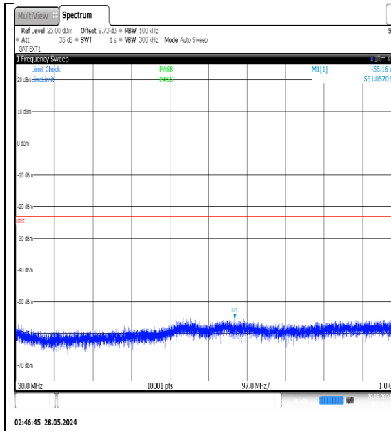
NTNV-N77-3450-3550-PC3-30-90-H-DFT-QPSK- Edge_1RB_Left-30-1000-Ant1-PASS
