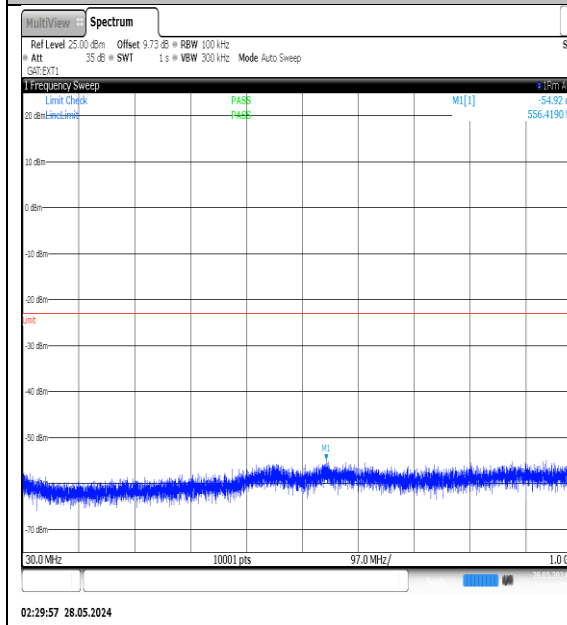
NTNV-N77-3450-3550-PC3-30-70-H-DFT-QPSK- Edge_1RB_Left-30-1000-Ant1-PASS
