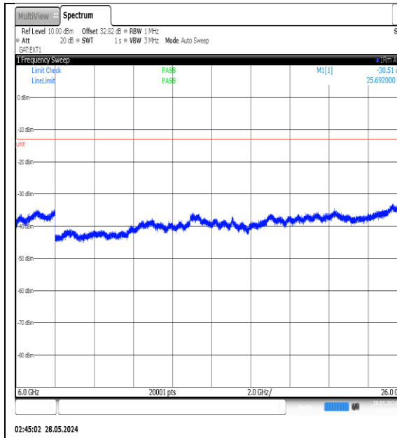
NTVN-N77-3450-3550-PC3-30-90-M-DFT-QPSK-Edge_1RB_Left-6000-26000-Ant1-PASS
