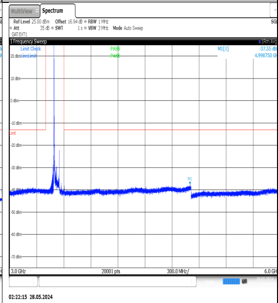
NTNV-N77-3450-3550-PC3-30-60-H-DFT-QPSK- Edge_1RB_Left-3000-6000-Ant1-PASS
