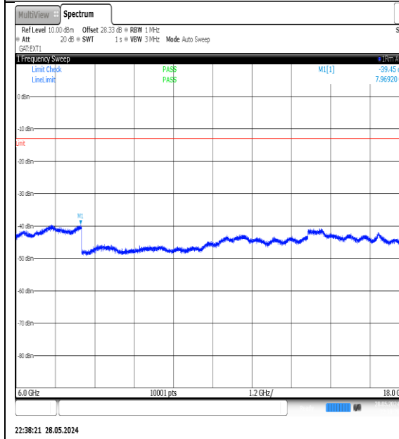
NTNV-N78-3700-3800-PC3-30-10-M-DFT-QPSK-Edge_1RB_Left-6000-18000-Ant1-PASS
