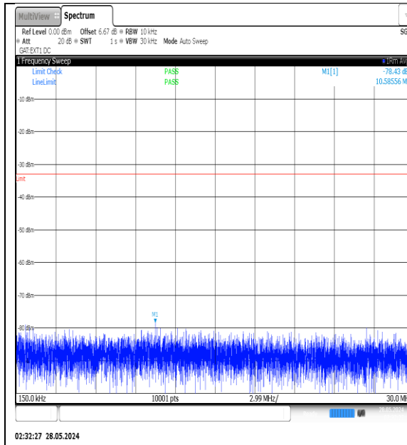
NTNV-N77-3450-3550-PC3-30-80-L-DFT-QPSK- Edge_1RB_Left-0.15-30-Ant1-PASS
