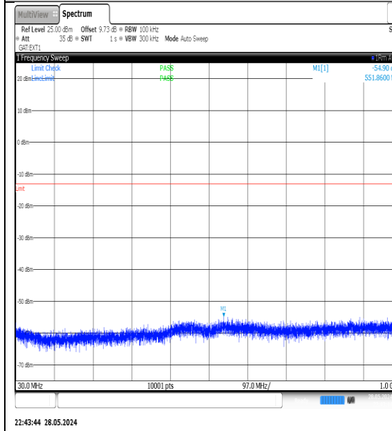
NTVN-N78-3700-3800-PC3-30-15-M-DFT-QPSK-Edge_1RB_Left-30-1000-Ant1-PASS
