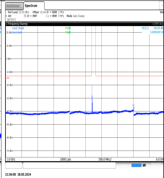
NTNV-N78-3700-3800-PC3-30-10-L-DFT-QPSK- Edge_1RB_Left-1000-6000-Ant1-PASS
