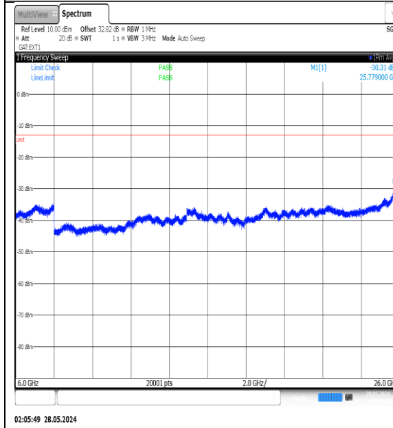
NTNV-N77-3450-3550-PC3-30-40-H-DFT-QPSK-Edge_1RB_Left-6000-26000-Ant1-PASS
