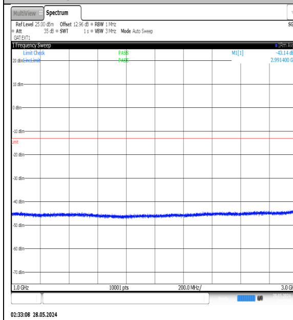
NTNV-N77-3450-3550-PC3-30-80-L-DFT-QPSK- Edge_1RB_Left-1000-3000-Ant1-PASS
