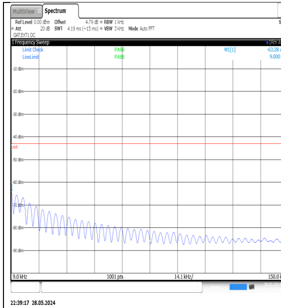
NTNV-N78-3700-3800-PC3-30-10-H-DFT-QPSK- Edge_1RB_Left-0.009-0.15-Ant1-PASS
