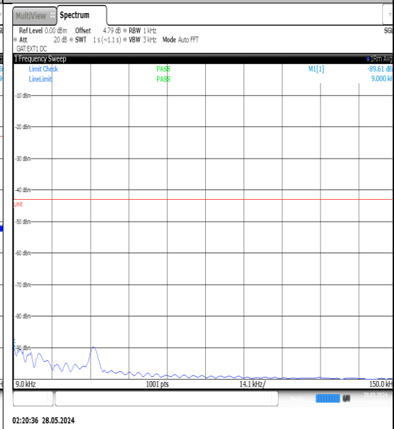
NTVN-N77-3450-3550-PC3-30-60-H-DFT-QPSK-Edge_1RB_Left-0.009-0.15-Ant1-PASS
