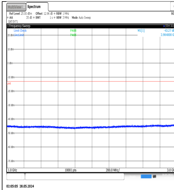
NTNV-N77-3450-3550-PC3-30-40-H-DFT-QPSK-Edge_1RB_Left-1000-3000-Ant1-PASS
