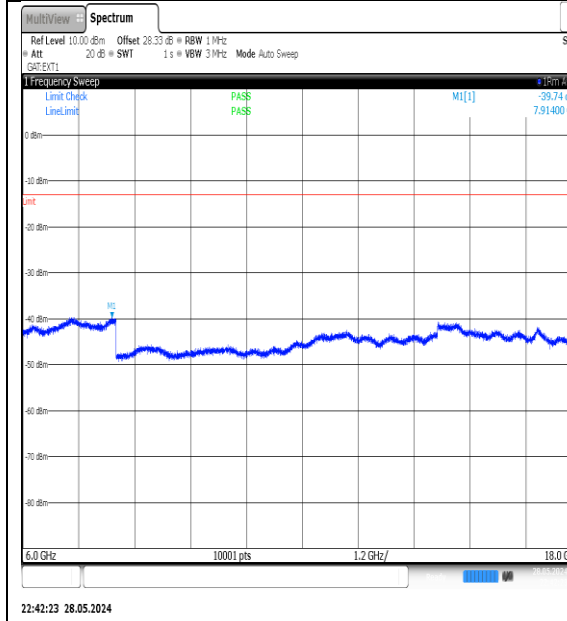
NTNV-N78-3700-3800-PC3-30-15-L-DFT-QPSK- Edge_1RB_Left-6000-18000-Ant1-PASS
