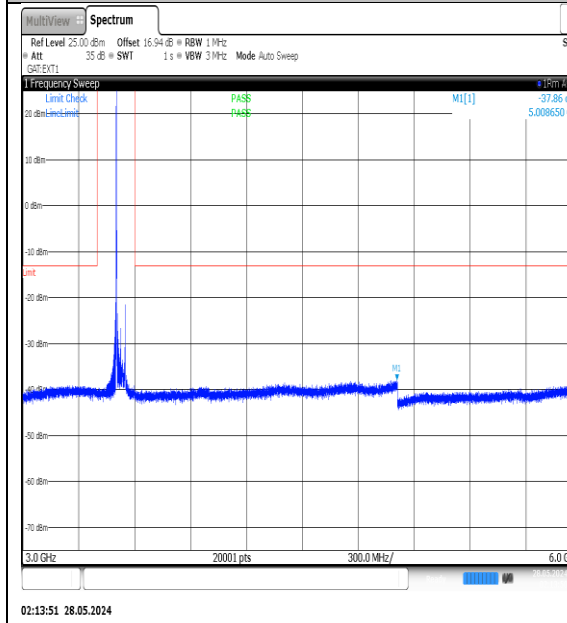
NTNV-N77-3450-3550-PC3-30-50-H-DFT-QPSK- Edge_1RB_Left-3000-6000-Ant1-PASS
