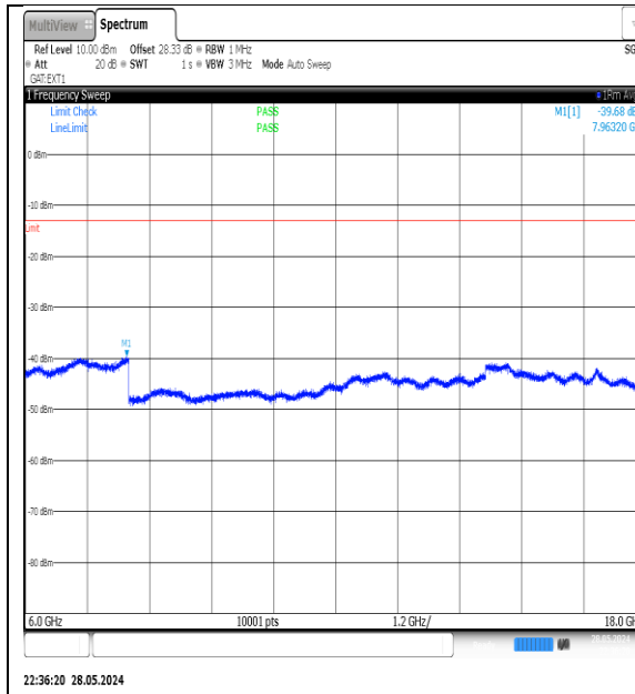
NTNV-N78-3700-3800-PC3-30-10-L-DFT-QPSK- Edge_1RB_Left-6000-18000-Ant1-PASS
