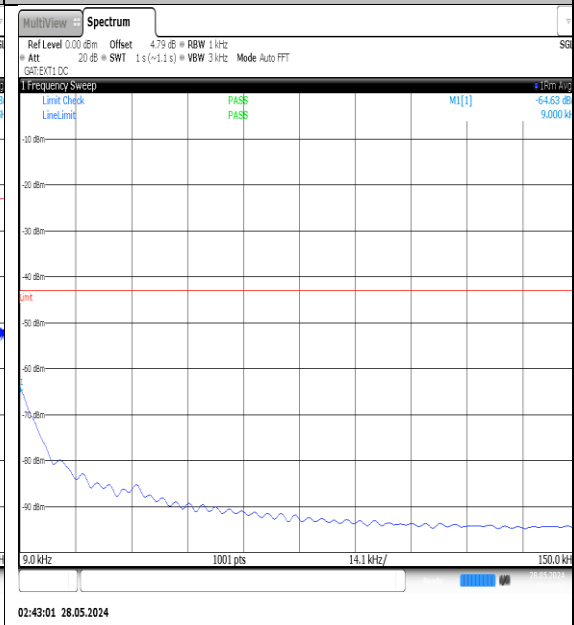
NTNV-N77-3450-3550-PC3-30-90-M-DFT-QPSK- Edge_1RB_Left-0.009-0.15-Ant1-PASS
