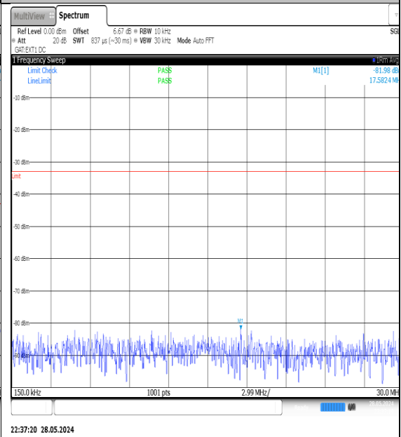
NTNV-N78-3700-3800-PC3-30-10-M-DFT-QPSK- Edge_1RB_Left-0.15-30-Ant1-PASS
