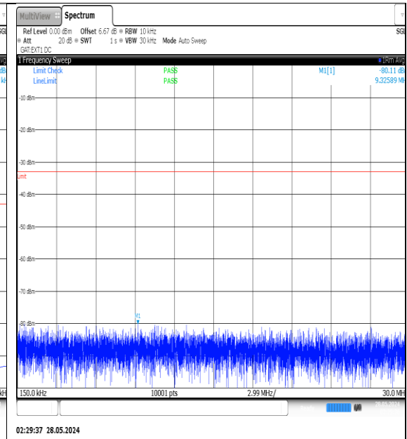
NTNV-N77-3450-3550-PC3-30-70-H-DFT-QPSK- Edge_1RB_Left-0.15-30-Ant1-PASS
