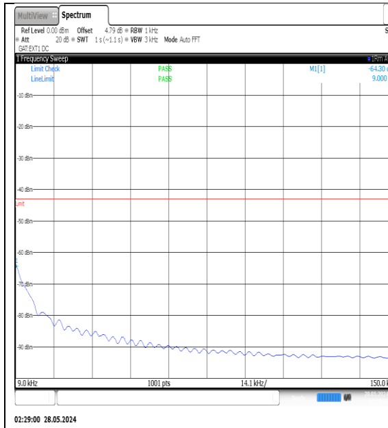
NTNV-N77-3450-3550-PC3-30-70-H-DFT-QPSK- Edge_1RB_Left-0.009-0.15-Ant1-PASS
