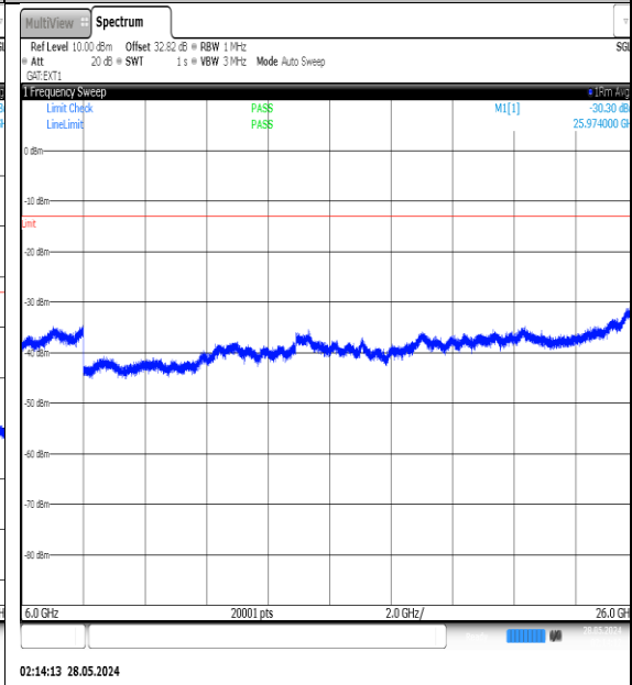
NTNV-N77-3450-3550-PC3-30-50-H-DFT-QPSK- Edge_1RB_Left-6000-26000-Ant1-PASS
