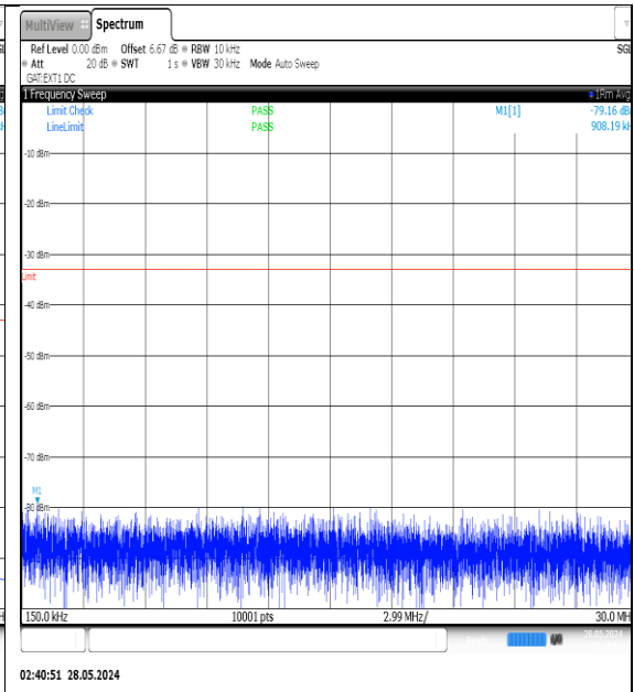
NTNV-N77-3450-3550-PC3-30-90-L-DFT-QPSK-Edge_1RB_Left-0.15-30-Ant1-PASS
