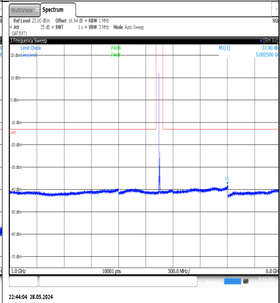
NTVN-N78-3700-3800-PC3-30-15-M-DFT-QPSK-Edge_1RB_Left-1000-6000-Ant1-PASS
