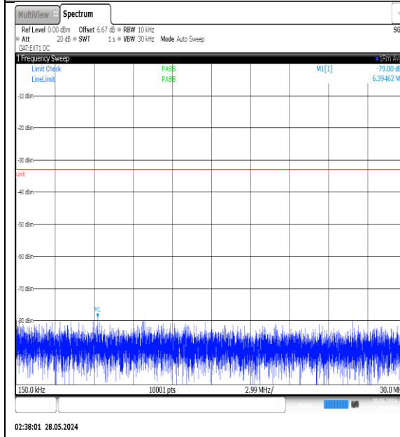
NTVN-N77-3450-3550-PC3-30-80-H-DFT-QPSK-Edge_1RB_Left-0.15-30-Ant1-PASS
