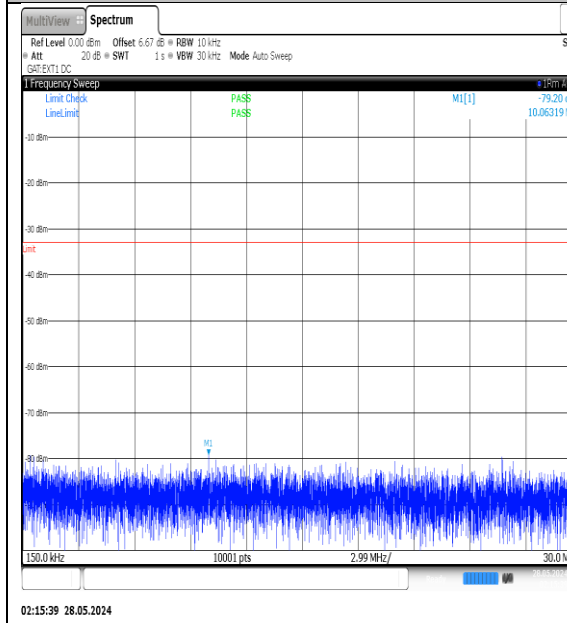
NTNV-N77-3450-3550-PC3-30-60-L-DFT-QPSK-Edge_1RB_Left-0.15-30-Ant1-PASS
