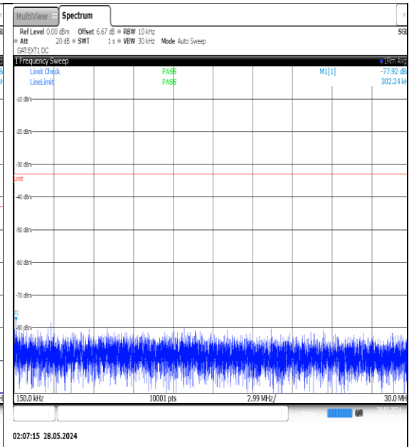
NTNV-N77-3450-3550-PC3-30-50-L-DFT-QPSK-Edge_1RB_Left-0.15-30-Ant1-PASS
