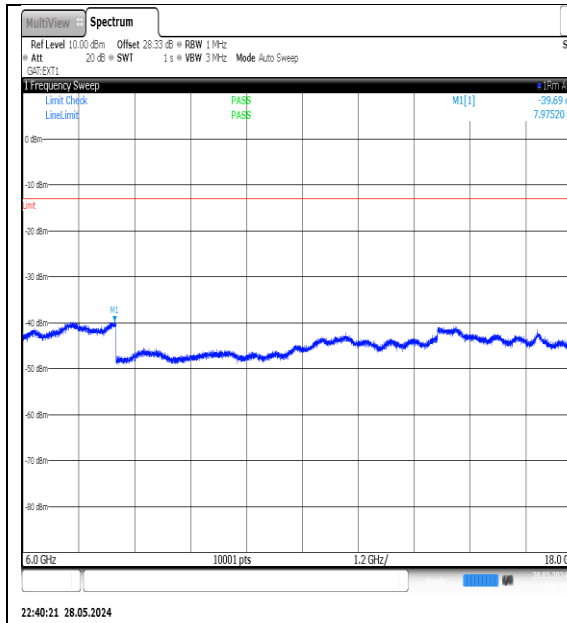
NTVN-N78-3700-3800-PC3-30-10-H-DFT-QPSK-Edge_1RB_Left-6000-18000-Ant1-PASS
