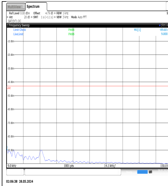
NTNV-N77-3450-3550-PC3-30-50-L-DFT-QPSK-Edge_1RB_Left-0.009-0.15-Ant1-PASS
