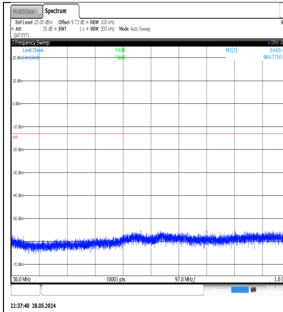
NTNV-N78-3700-3800-PC3-30-10-M-DFT-QPSK-Edge_1RB_Left-30-1000-Ant1-PASS
