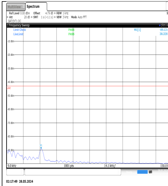
NTVN-N77-3450-3550-PC3-30-60-M-DFT-QPSK-Edge_1RB_Left-0.009-0.15-Ant1-PASS
