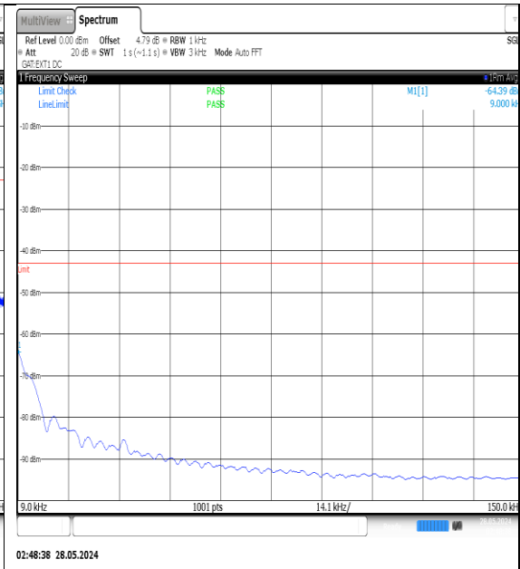
NTNV-N77-3450-3550-PC3-30-100-M-DFT-QPSK-Edge_1RB_Left-0.009-0.15-Ant1-PASS
