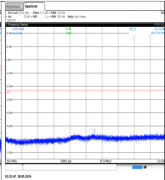
NTNV-N77-3450-3550-PC3-30-80-L-DFT-QPSK- Edge_1RB_Left-30-1000-Ant1-PASS
