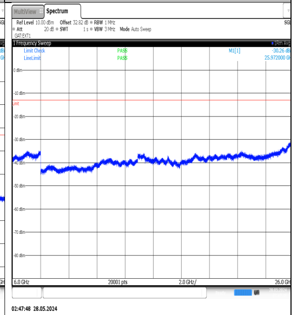
NTNV-N77-3450-3550-PC3-30-90-H-DFT-QPSK- Edge_1RB_Left-6000-26000-Ant1-PASS
