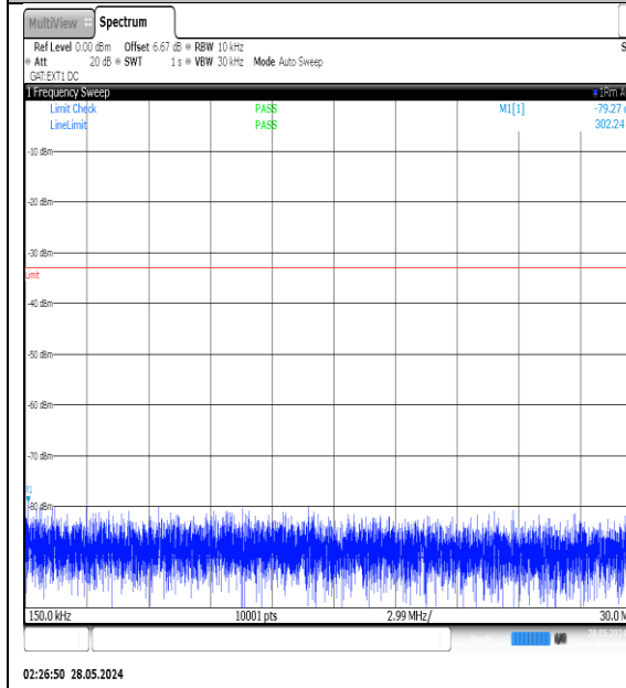
NTNV-N77-3450-3550-PC3-30-70-M-DFT-QPSK-Edge_1RB_Left-0.15-30-Ant1-PASS
