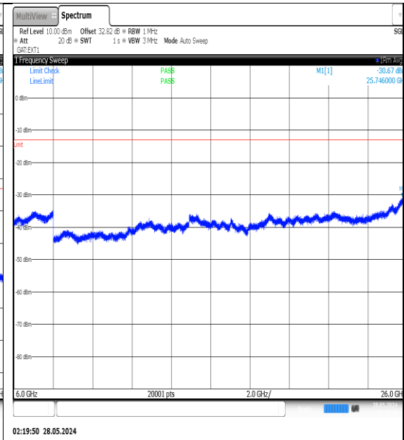
NTVN-N77-3450-3550-PC3-30-60-M-DFT-QPSK-Edge_1RB_Left-6000-26000-Ant1-PASS
