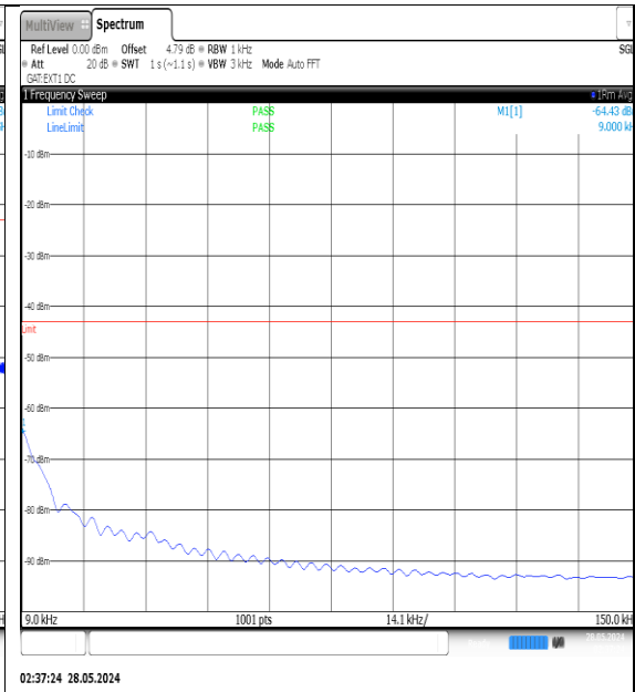
NTVN-N77-3450-3550-PC3-30-80-H-DFT-QPSK-Edge_1RB_Left-0.009-0.15-Ant1-PASS
