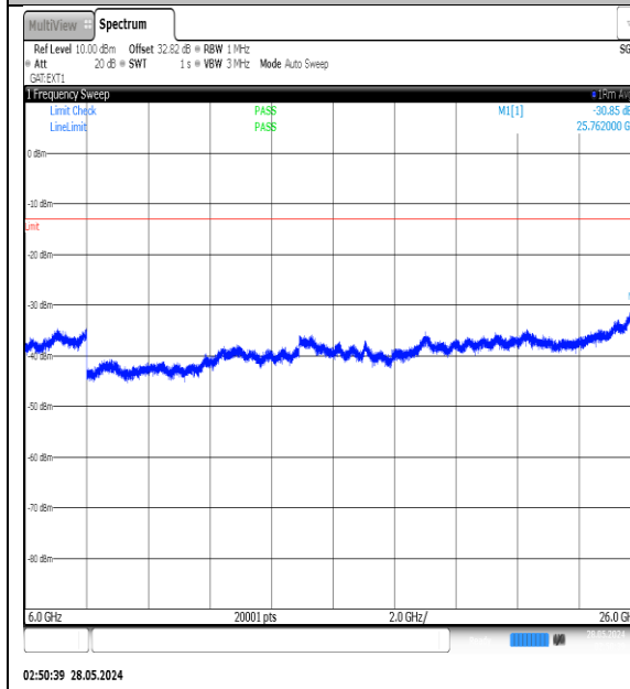
N77-3450-3550-PC3-30-100-M-DFT- QPSK-Edge_1RB_Left-6000-26000-Ant1-PASS
