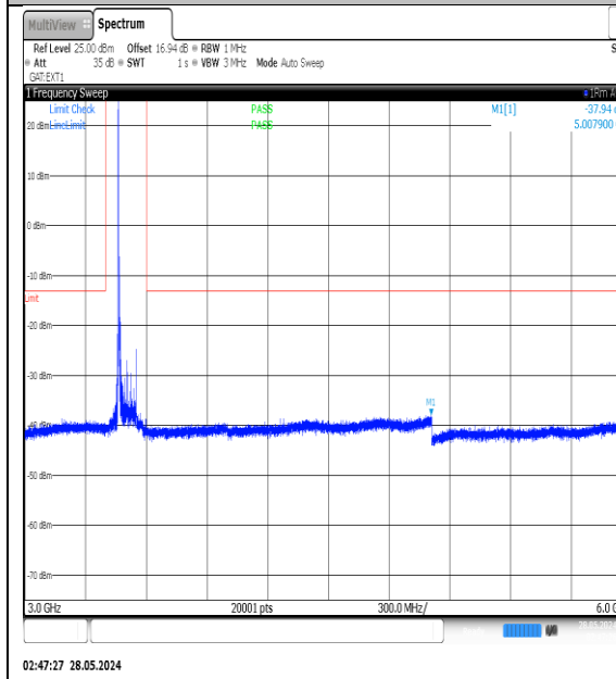
NTNV-N77-3450-3550-PC3-30-90-H-DFT-QPSK- Edge_1RB_Left-3000-6000-Ant1-PASS
