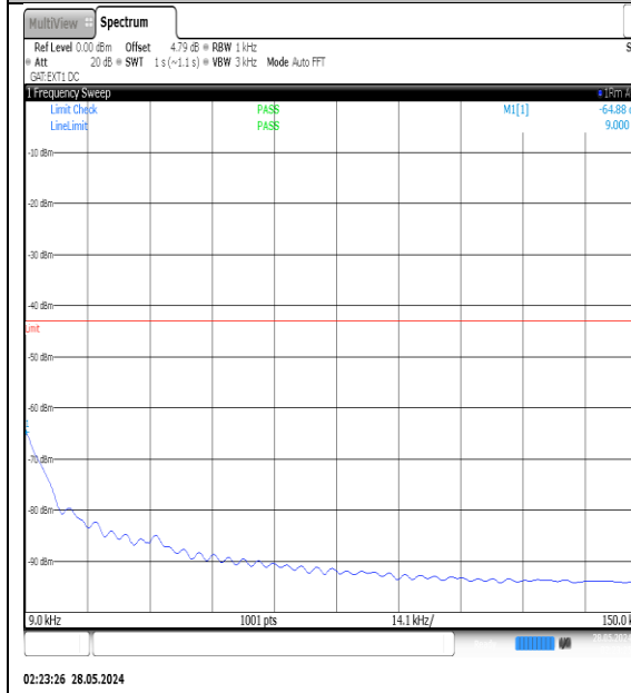
NTNV-N77-3450-3550-PC3-30-70-L-DFT-QPSK-Edge_1RB_Left-0.009-0.15-Ant1-PASS
