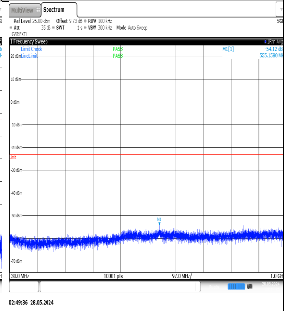
NTNV-N77-3450-3550-PC3-30-100-M-DFT-QPSK-Edge_1RB_Left-30-1000-Ant1-PASS
