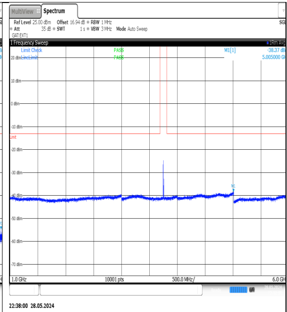
NTNV-N78-3700-3800-PC3-30-10-M-DFT-QPSK-Edge_1RB_Left-1000-6000-Ant1-PASS
