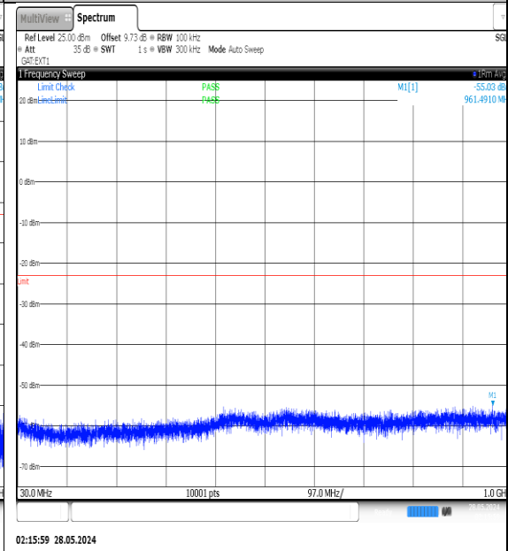
NTNV-N77-3450-3550-PC3-30-60-L-DFT-QPSK-Edge_1RB_Left-30-1000-Ant1-PASS
