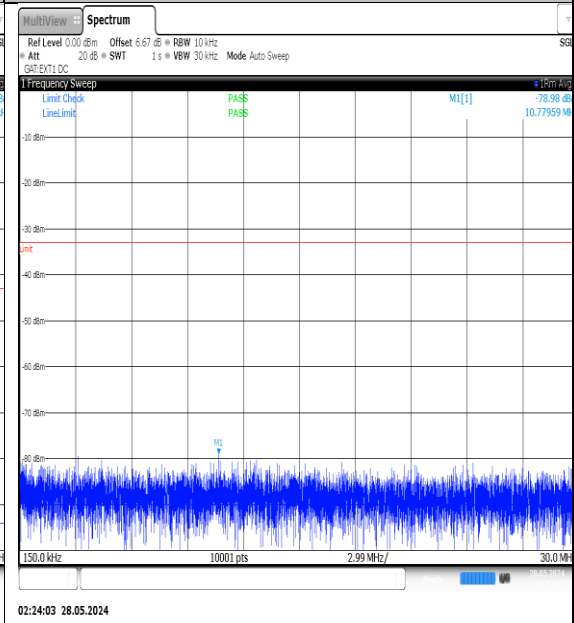
NTNV-N77-3450-3550-PC3-30-70-L-DFT-QPSK-Edge_1RB_Left-0.15-30-Ant1-PASS
