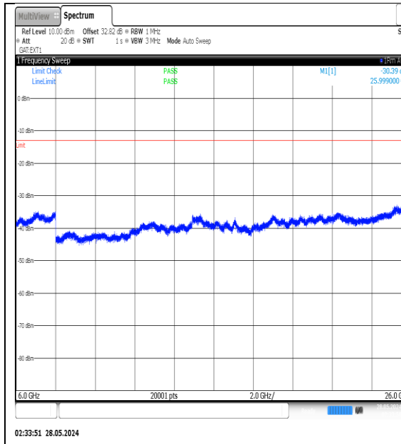
NTNV-N77-3450-3550-PC3-30-80-L-DFT-QPSK- Edge_1RB_Left-6000-26000-Ant1-PASS
