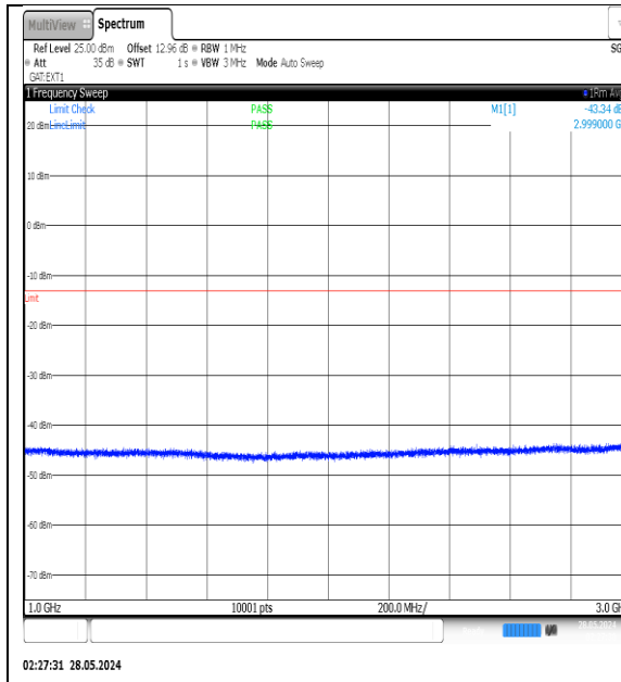
NTNV-N77-3450-3550-PC3-30-70-M-DFT-QPSK-Edge_1RB_Left-1000-3000-Ant1-PASS
