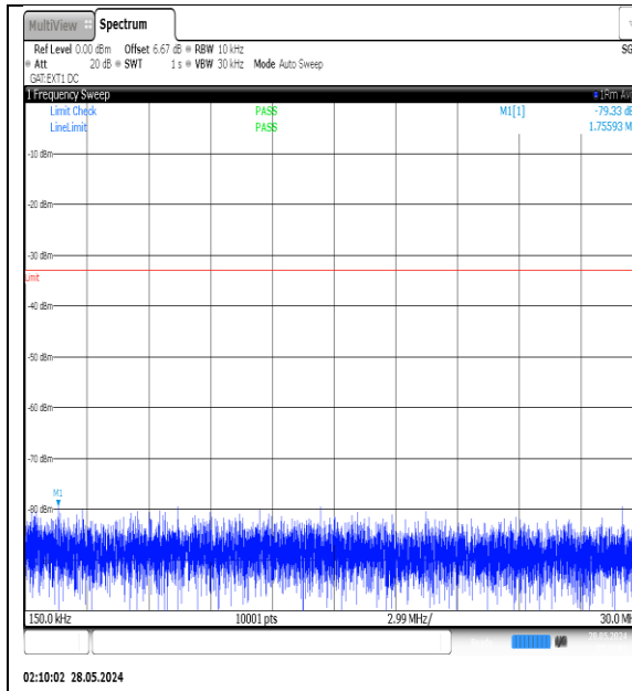
NTNV-N77-3450-3550-PC3-30-50-M-DFT-QPSK-Edge_1RB_Left-0.15-30-Ant1-PASS
