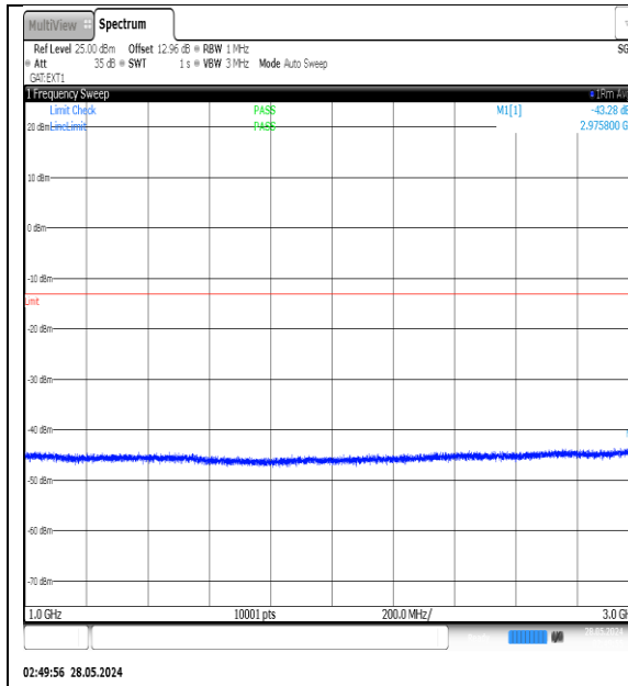
N77-3450-3550-PC3-30-100-M-DFT- QPSK-Edge_1RB_Left-1000-3000-Ant1-PASS
