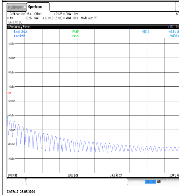
NTNV-N78-3700-3800-PC3-30-10-M-DFT-QPSK- Edge_1RB_Left-0.009-0.15-Ant1-PASS
