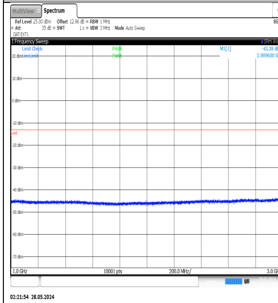
NTNV-N77-3450-3550-PC3-30-60-H-DFT-QPSK- Edge_1RB_Left-1000-3000-Ant1-PASS
