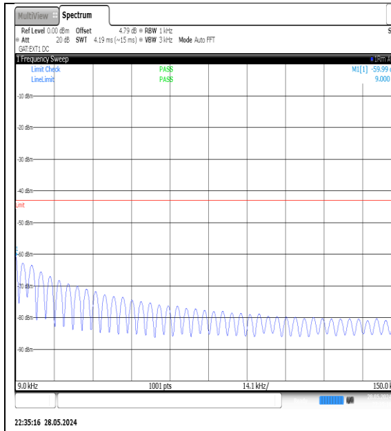
NTNV-N78-3700-3800-PC3-30-10-L-DFT-QPSK- Edge_1RB_Left-0.009-0.15-Ant1-PASS
