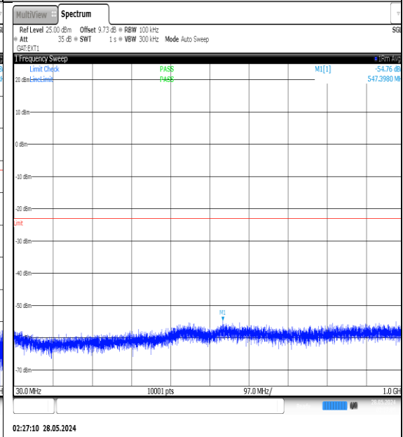
NTNV-N77-3450-3550-PC3-30-70-M-DFT-QPSK-Edge_1RB_Left-30-1000-Ant1-PASS
