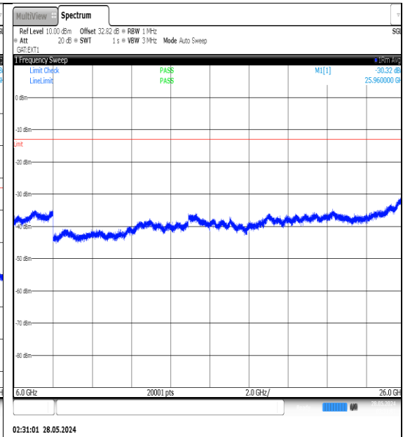
NTNV-N77-3450-3550-PC3-30-70-H-DFT-QPSK- Edge_1RB_Left-6000-26000-Ant1-PASS
