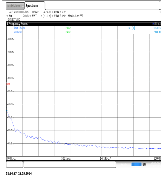
NTNV-N77-3450-3550-PC3-30-80-M-DFT-QPSK- Edge_1RB_Left-0.009-0.15-Ant1-PASS
