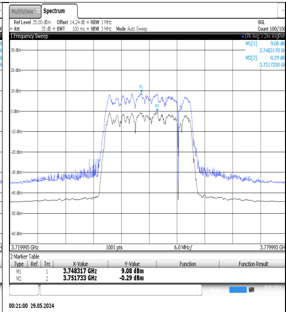
NTNV-N78-3700-3800-PC3-30-20-M-DFT-QPSK- Outer_Full-Ant1-PASS
