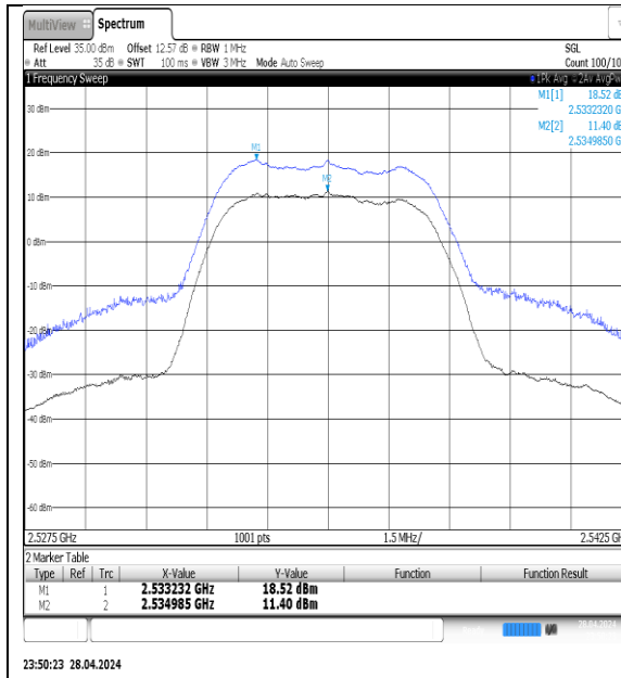
NTNV-N7-PC3-15-5-M-DFT-QPSK-Outer_Full-Ant1-PASS
