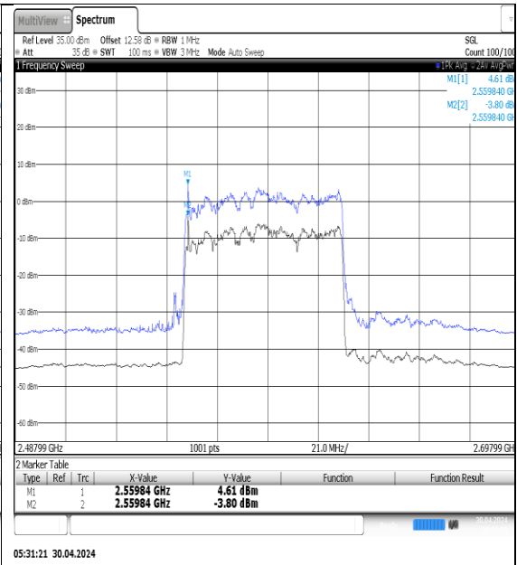
NTVN-N41-PC3-30-70-M-DFT-QPSK-Outer_Full-Ant1-PASS
