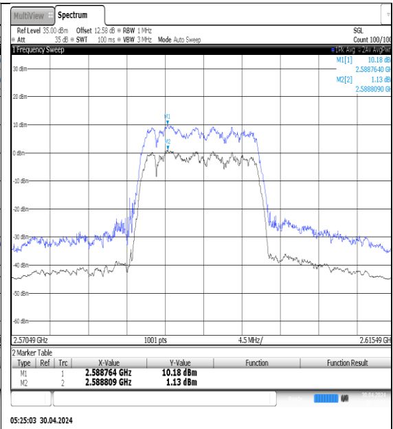
NTVN-N41-PC3-30-15-M-DFT-QPSK-Outer_Full-Ant1-PASS
