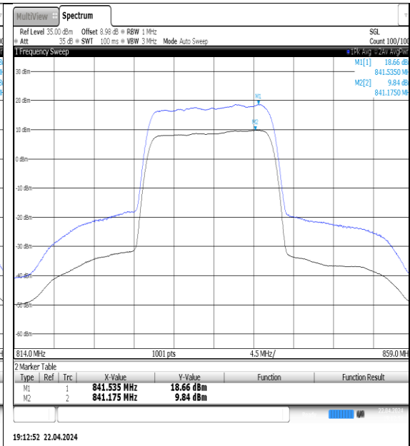
NTNV-N5-PC3-15-15-M-DFT-16QAM-Outer_Full-Ant1-PASS
