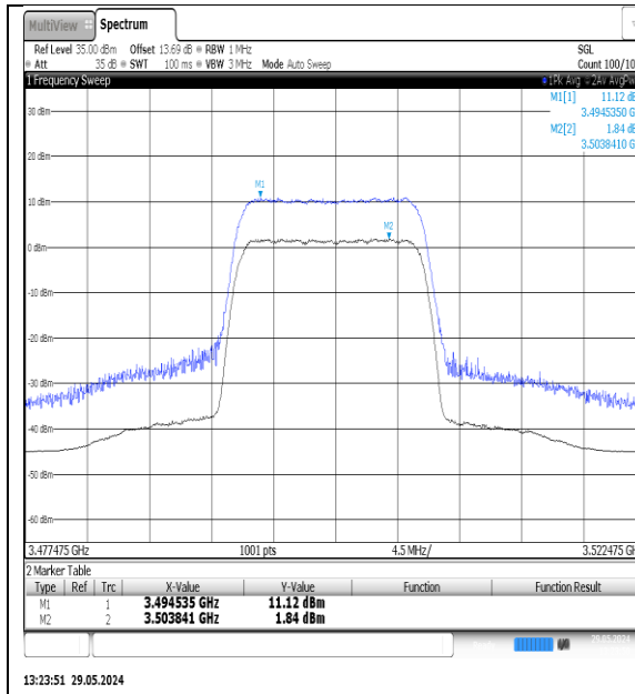
NTNV-N77-3450-3550-PC3-30-15-M-DFT-16QAM-Outer_Full-Ant1-PASS
