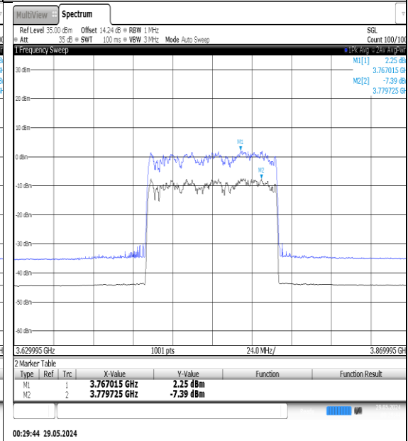
NTNV-N78-3700-3800-PC3-30-80-M-DFT-QPSK- Outer_Full-Ant1-PASS
