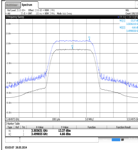
NTNV-N77-3450-3550-PC3-30-10-M-DFT-16QAM-Outer_Full-Ant1-PASS
