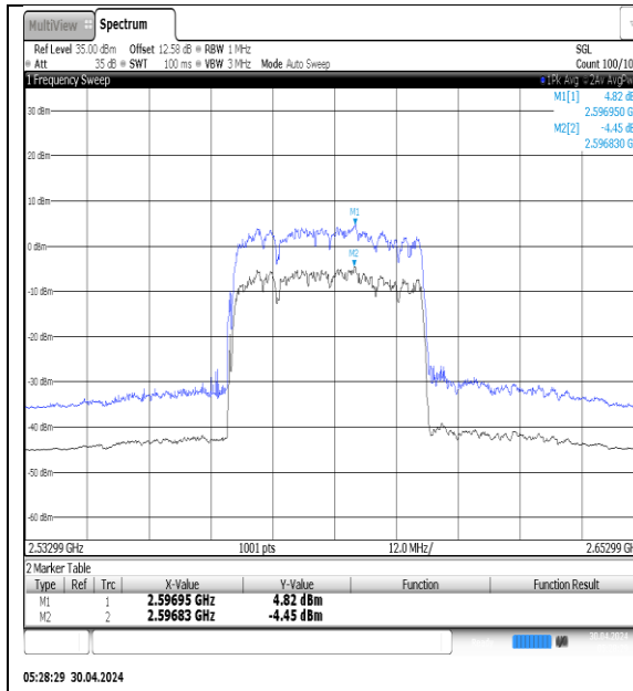
NTVN-N41-PC3-30-40-M-DFT-16QAM-Outer_Full-Ant1-PASS
