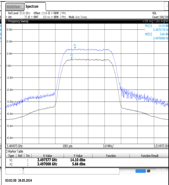
NTNV-N77-3450-3550-PC3-30-10-M-DFT-QPSK-Outer_Full-Ant1-PASS
