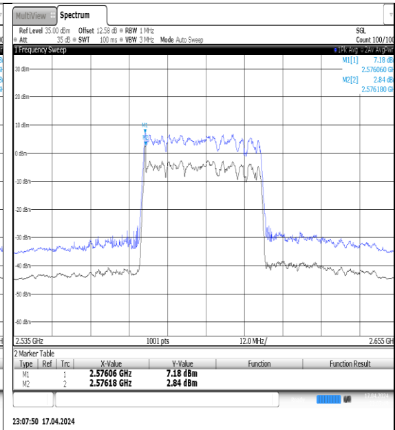
NTVN-N38-PC3-30-40-M-DFT-QPSK-Outer_Full-Ant1-PASS
