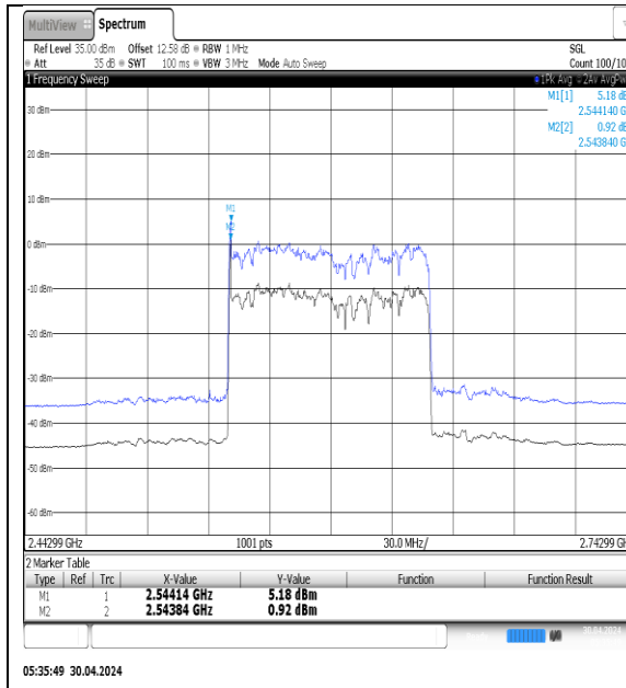
NTNV-N41-PC3-30-100-M-DFT-16QAM-Outer_Full-Ant1-PASS
