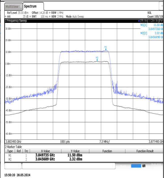
NTNV-N77-3700-3980-PC3-30-25-M-DFT-QPSK- Outer_Full-Ant1-PASS
