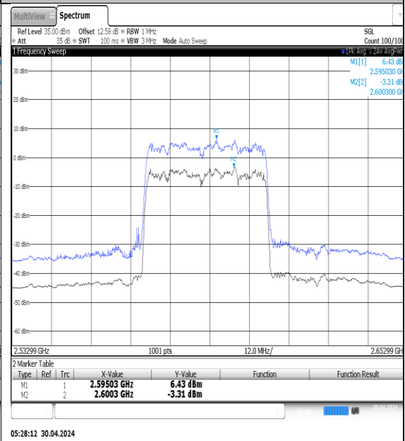
NTVN-N41-PC3-30-40-M-DFT-QPSK-Outer_Full-Ant1-PASS
