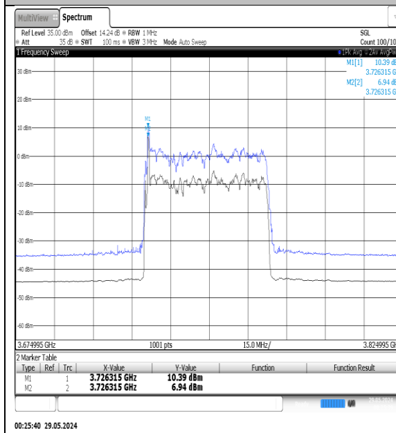
NTNV-N78-3700-3800-PC3-30-50-M-DFT- 16QAM-Outer_Full-Ant1-PASS
