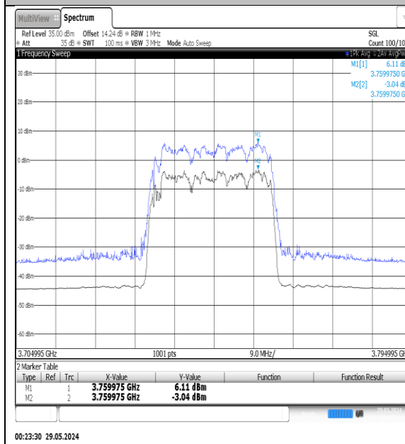
NTNV-N78-3700-3800-PC3-30-30-M-DFT- 16QAM-Outer_Full-Ant1-PASS
