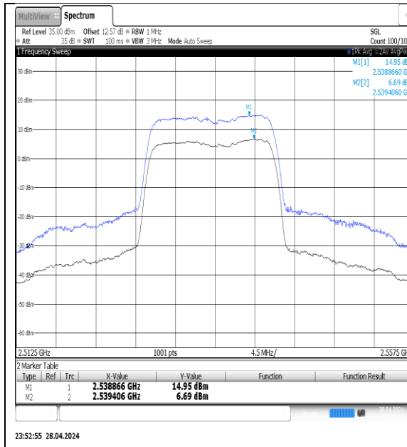
NTNV-N7-PC3-15-15-M-DFT-QPSK-Outter_Full-Ant1-PASS
