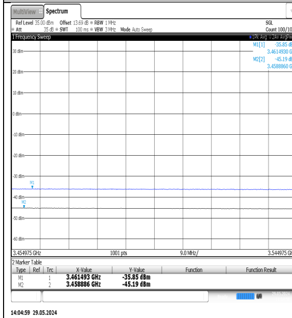
NTNV-N77-3450-3550-PC3-30-30-M-DFT-16QAM-Outer_Full-Ant1-PASS
