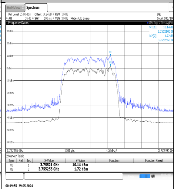
NTNV-N78-3700-3800-PC3-30-15-M-DFT-QPSK- Outer_Full-Ant1-PASS
