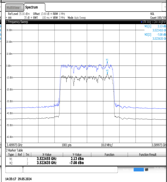
NTNV-N77-3450-3550-PC3-30-60-M-DFT-QPSK- Outer_Full-Ant1-PASS
