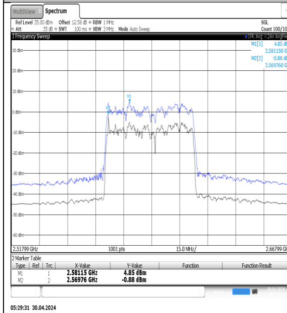
NTVN-N41-PC3-30-50-M-DFT-16QAM-Outer_Full-Ant1-PASS
