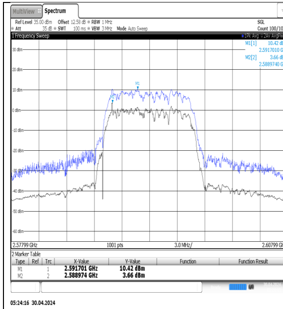
NTVN-N41-PC3-30-10-M-DFT-16QAM-Outer_Full-Ant1-PASS
