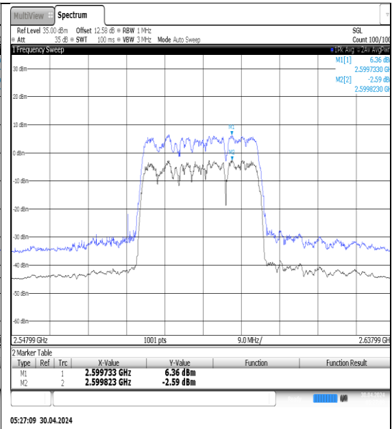
NTVN-N41-PC3-30-30-M-DFT-QPSK-Outer_Full-Ant1-PASS
