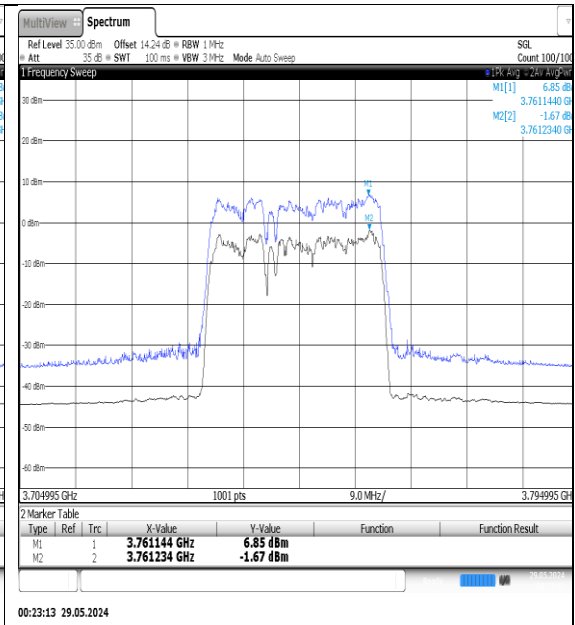
NTNV-N78-3700-3800-PC3-30-30-M-DFT-QPSK- Outer_Full-Ant1-PASS
