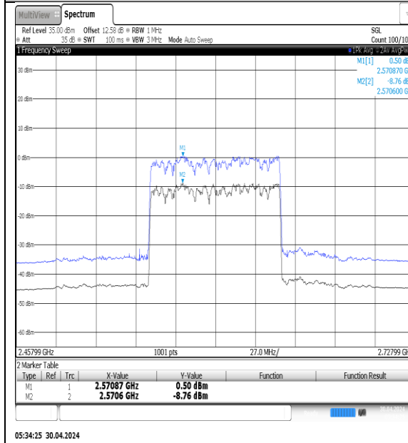
NTVN-N41-PC3-30-90-M-DFT-16QAM-Outer_Full-Ant1-PASS
