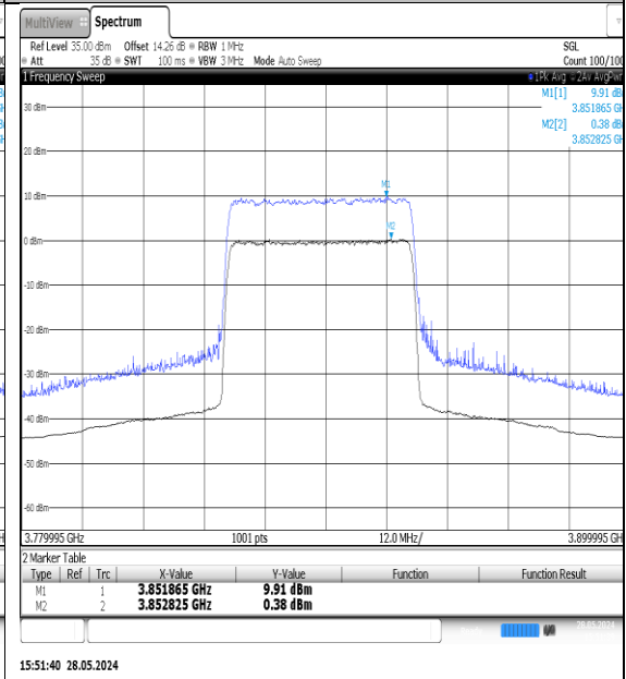
NTNV-N77-3700-3980-PC3-30-40-M-DFT-QPSK- Outer_Full-Ant1-PASS
