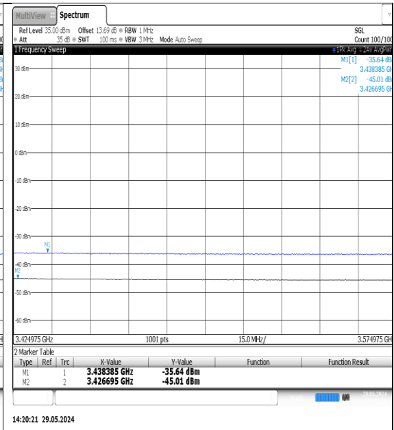
NTNV-N77-3450-3550-PC3-30-50-M-DFT-QPSK- Outer_Full-Ant1-PASS
