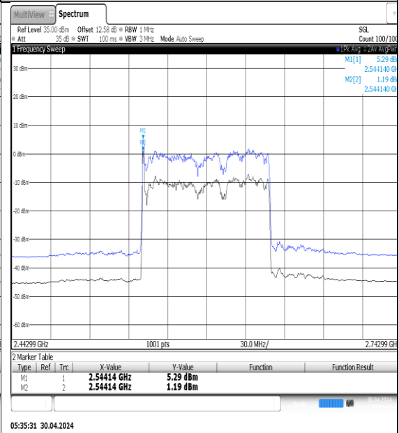
NTVN-N41-PC3-30-100-M-DFT-QPSK-Outer_Full-Ant1-PASS
