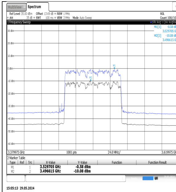
NTNV-N77-3450-3550-PC3-30-80-M-DFT- 16QAM-Outer_Full-Ant1-PASS
