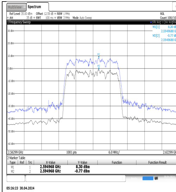
NTVN-N41-PC3-30-20-M-DFT-16QAM-Outer_Full-Ant1-PASS
