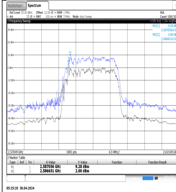
NTVN-N41-PC3-30-15-M-DFT-16QAM-Outer_Full-Ant1-PASS
