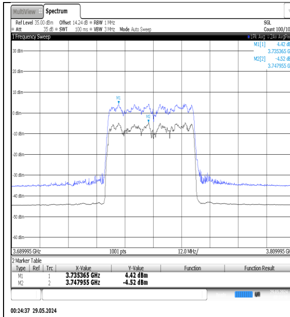
NTNV-N78-3700-3800-PC3-30-40-M-DFT- 16QAM-Outer_Full-Ant1-PASS
