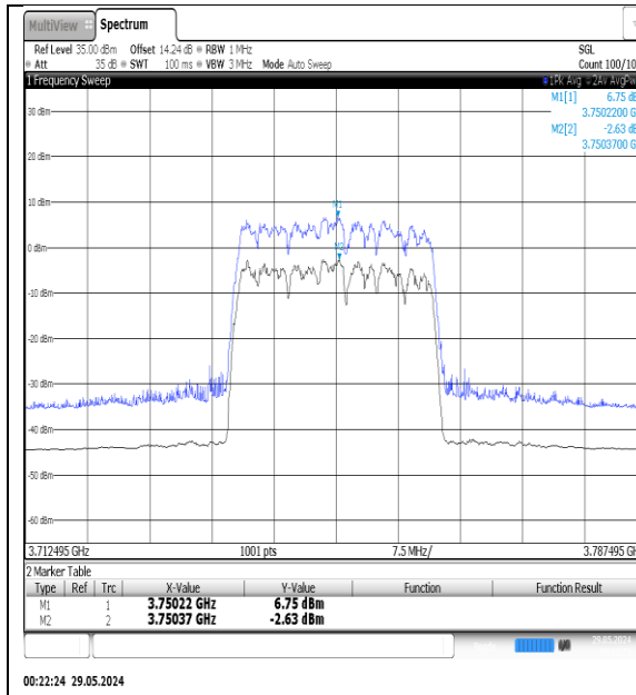
NTNV-N78-3700-3800-PC3-30-25-M-DFT- 16QAM-Outer_Full-Ant1-PASS
