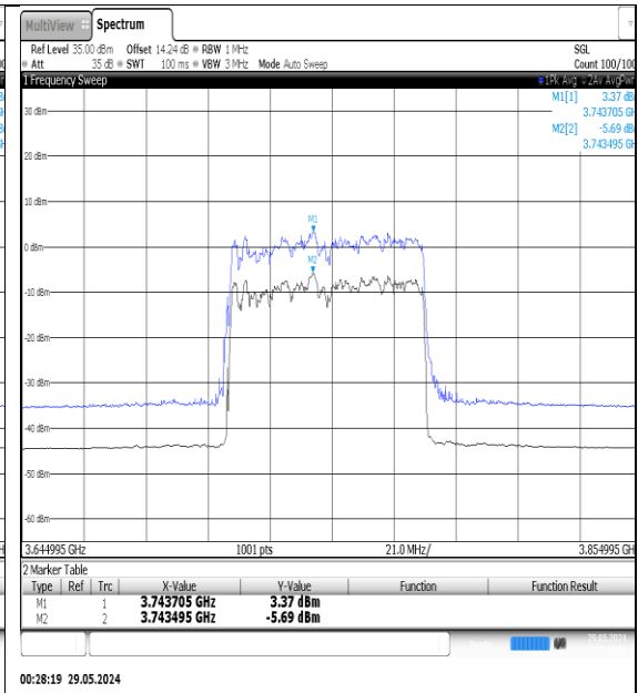
NTNV-N78-3700-3800-PC3-30-70-M-DFT-QPSK- Outer_Full-Ant1-PASS
