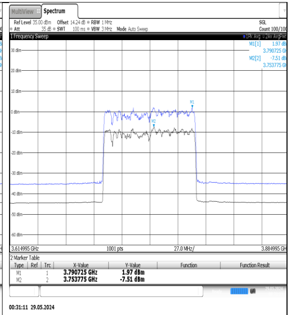
NTNV-N78-3700-3800-PC3-30-90-M-DFT-QPSK- Outer_Full-Ant1-PASS
