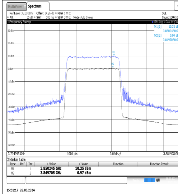
NTNV-N77-3700-3980-PC3-30-30-M-DFT- 16QAM-Outer_Full-Ant1-PASS
