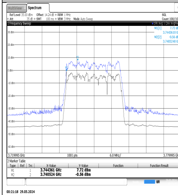
NTNV-N78-3700-3800-PC3-30-20-M-DFT- 16QAM-Outer_Full-Ant1-PASS
