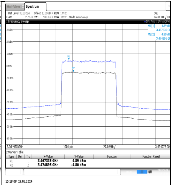
NTNV-N77-3450-3550-PC3-30-90-M-DFT-QPSK- Outer_Full-Ant1-PASS
