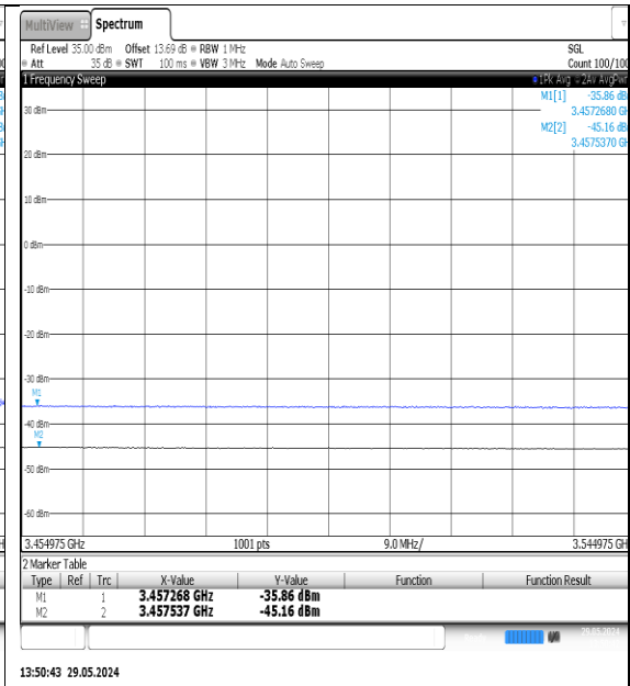
NTNV-N77-3450-3550-PC3-30-30-M-DFT-QPSK-Outer_Full-Ant1-PASS
