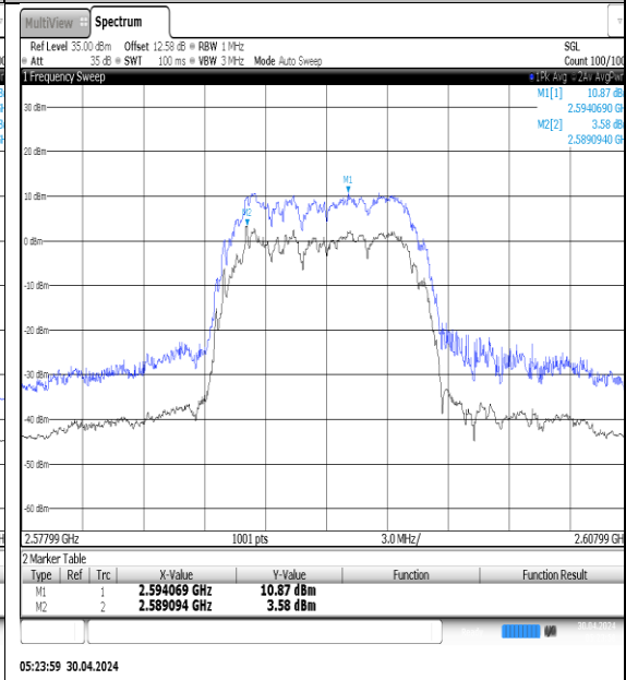
NTVN-N41-PC3-30-10-M-DFT-QPSK-Outer_Full-Ant1-PASS
