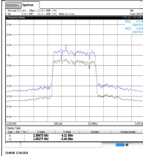
NTVN-N38-PC3-30-40-M-DFT-16QAM-Outer_Full-Ant1-PASS
