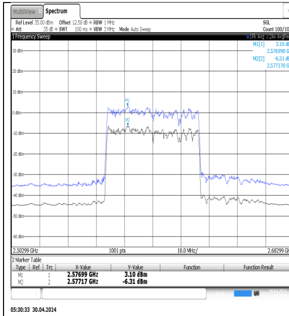
NTVN-N41-PC3-30-60-M-DFT-16QAM-Outer_Full-Ant1-PASS
