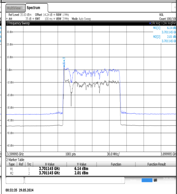
NTNV-N78-3700-3800-PC3-30-100-M-DFT- QPSK-Outer_Full-Ant1-PASS
