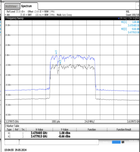
NTNV-N77-3450-3550-PC3-30-80-M-DFT-QPSK- Outer_Full-Ant1-PASS
