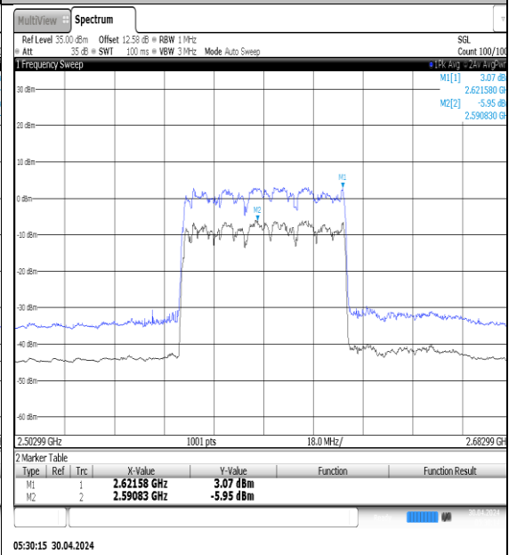
NTVN-N41-PC3-30-60-M-DFT-QPSK-Outer_Full-Ant1-PASS
