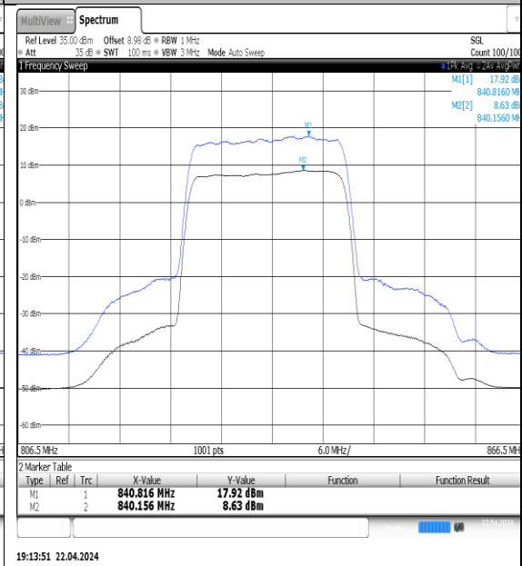
NTNV-N5-PC3-15-20-M-DFT-16QAM-Outer_Full-Ant1-PASS
