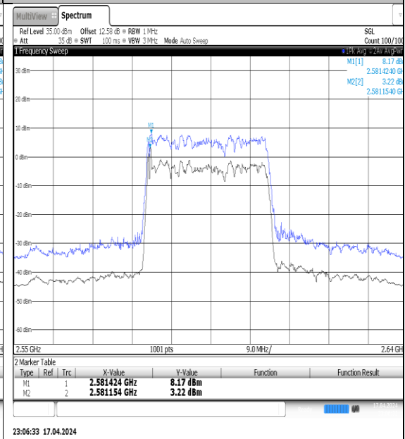
NTVN-N38-PC3-30-30-M-DFT-QPSK-Outer_Full-Ant1-PASS
