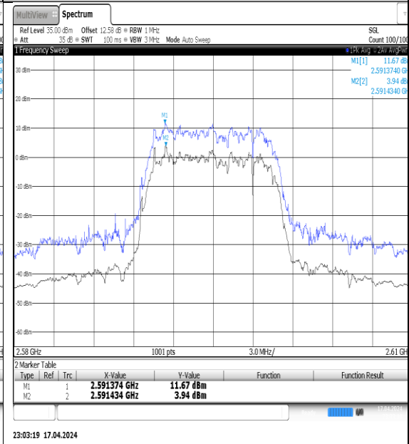
NTNV-N38-PC3-30-10-M-DFT-16QAM-Outter_Full-Ant1-PASS
