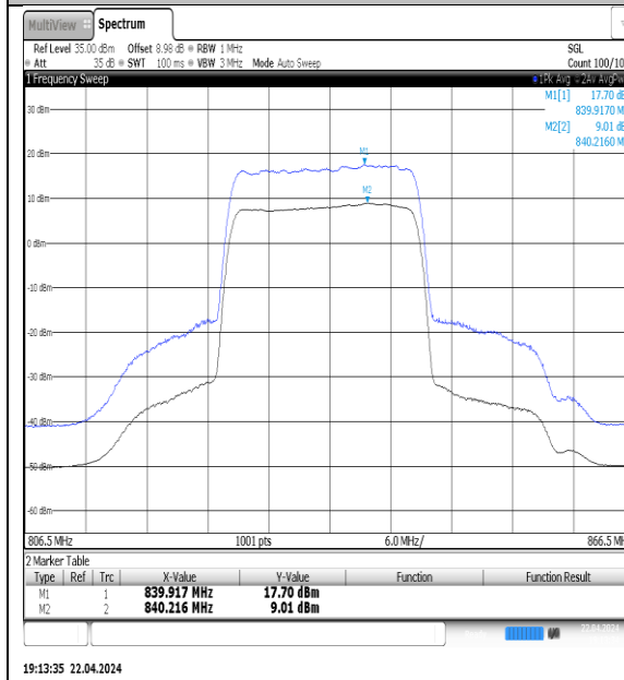
NTNV-N5-PC3-15-20-M-DFT-QPSK-Outer_Full-Ant1-PASS
