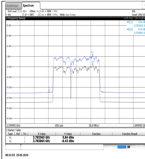
NTNV-N78-3700-3800-PC3-30-100-M-DFT- 16QAM-Outer_Full-Ant1-PASS
