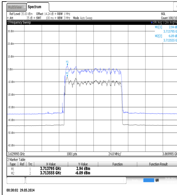
NTNV-N78-3700-3800-PC3-30-80-M-DFT- 16QAM-Outer_Full-Ant1-PASS
