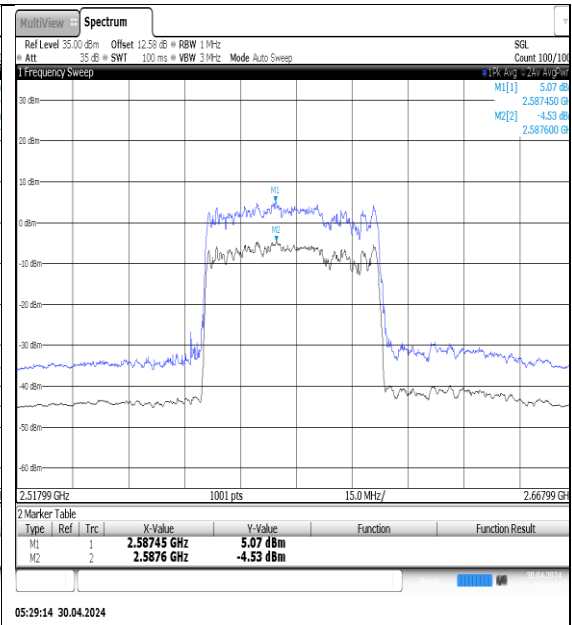
NTVN-N41-PC3-30-50-M-DFT-QPSK-Outer_Full-Ant1-PASS
