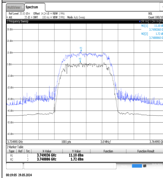
NTNV-N78-3700-3800-PC3-30-10-M-DFT- 16QAM-Outer_Full-Ant1-PASS
