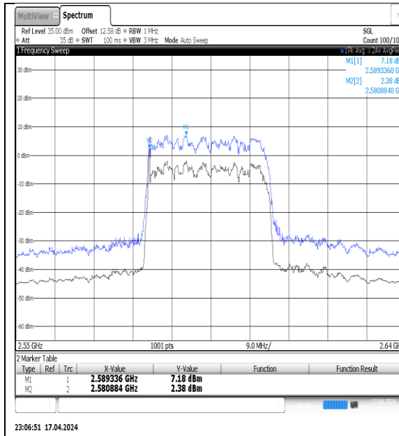
NTVN-N38-PC3-30-30-M-DFT-16QAM-Outer_Full-Ant1-PASS
