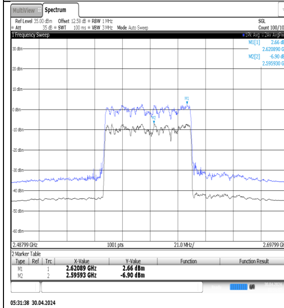
NTVN-N41-PC3-30-70-M-DFT-16QAM-Outer_Full-Ant1-PASS
