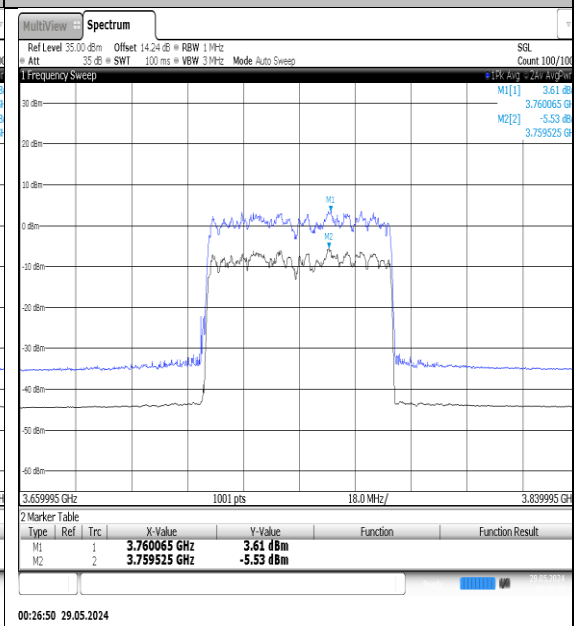
NTNV-N78-3700-3800-PC3-30-60-M-DFT-QPSK- Outer_Full-Ant1-PASS
