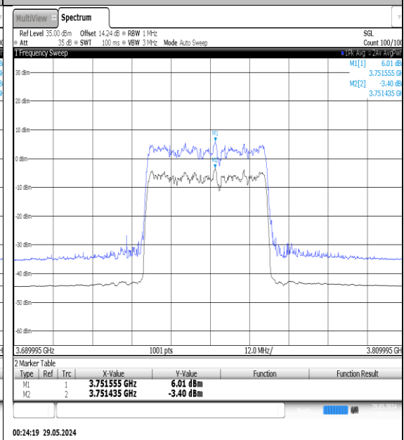
NTNV-N78-3700-3800-PC3-30-40-M-DFT-QPSK- Outer_Full-Ant1-PASS
