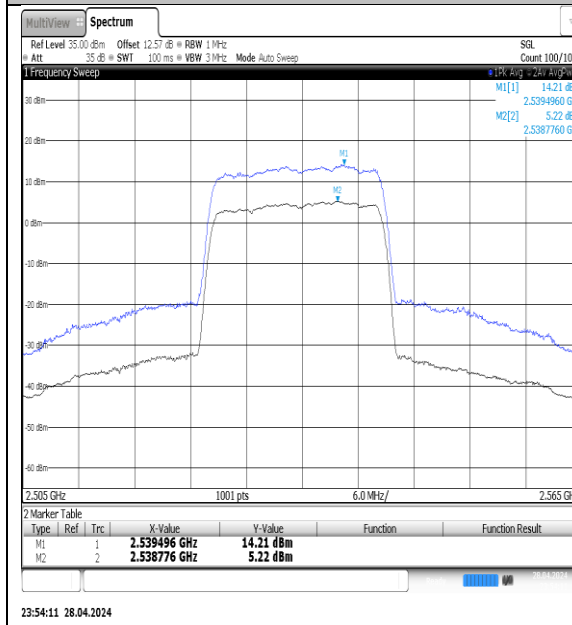
NTNV-N7-PC3-15-20-M-DFT-QPSK-Outter_Full-Ant1-PASS
