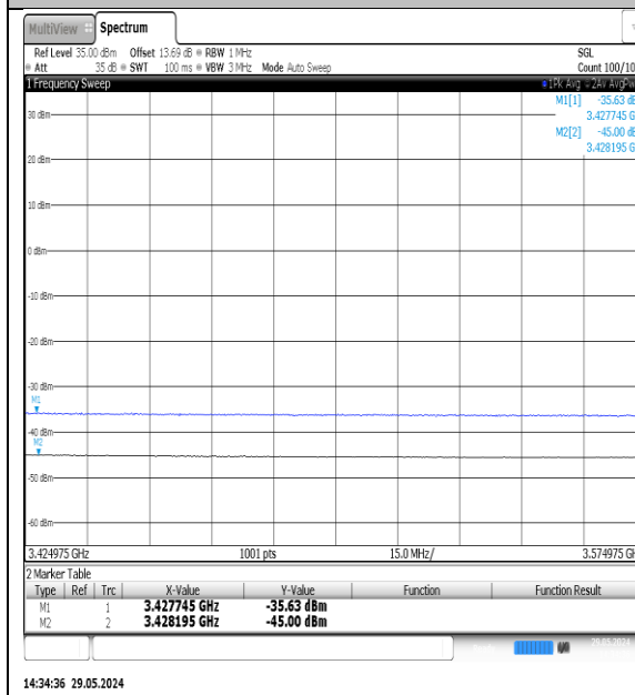
NTNV-N77-3450-3550-PC3-30-50-M-DFT- 16QAM-Outer_Full-Ant1-PASS
