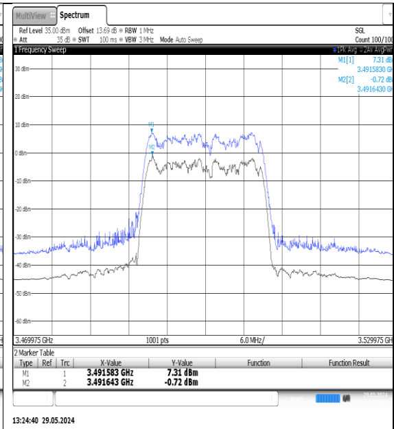
NTNV-N77-3450-3550-PC3-30-20-M-DFT-QPSK-Outer_Full-Ant1-PASS
