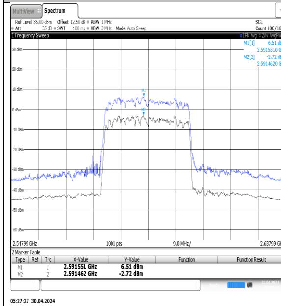
NTVN-N41-PC3-30-30-M-DFT-16QAM-Outer_Full-Ant1-PASS
