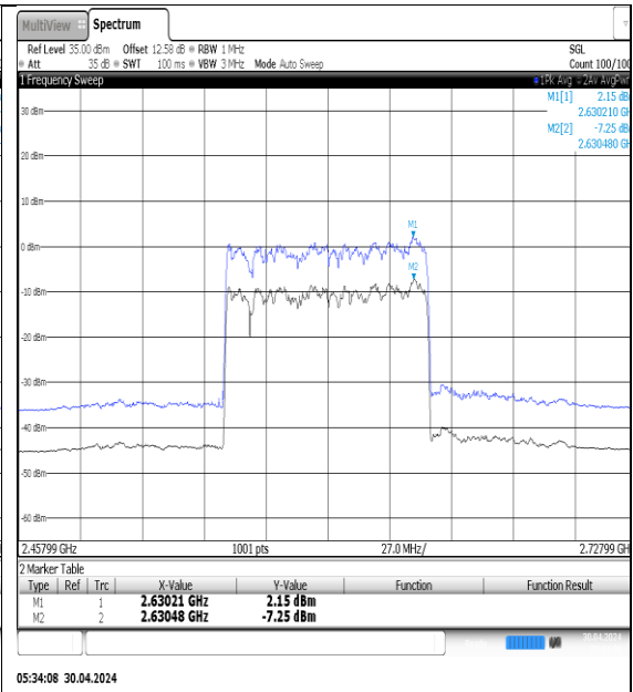
NTVN-N41-PC3-30-90-M-DFT-QPSK-Outer_Full-Ant1-PASS
