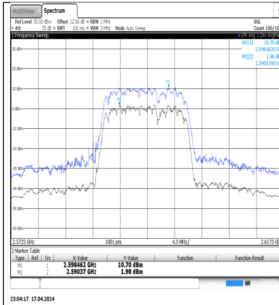
NTVN-N38-PC3-30-15-M-DFT-QPSK-Outer_Full-Ant1-PASS
