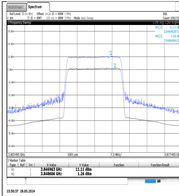
NTNV-N77-3700-3980-PC3-30-25-M-DFT- 16QAM-Outer_Full-Ant1-PASS
