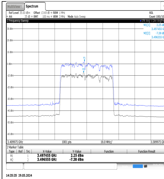
NTNV-N77-3450-3550-PC3-30-60-M-DFT- 16QAM-Outer_Full-Ant1-PASS
