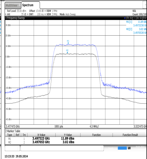
NTNV-N77-3450-3550-PC3-30-15-M-DFT-QPSK-Outer_Full-Ant1-PASS
