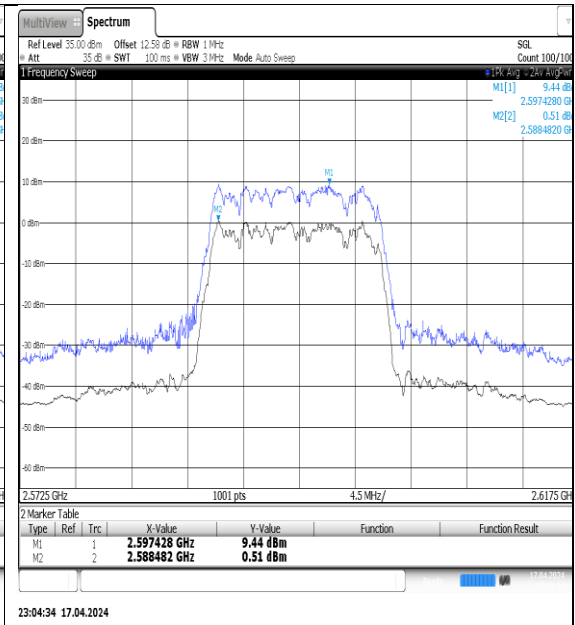
NTVN-N38-PC3-30-15-M-DFT-16QAM-Outer_Full-Ant1-PASS
