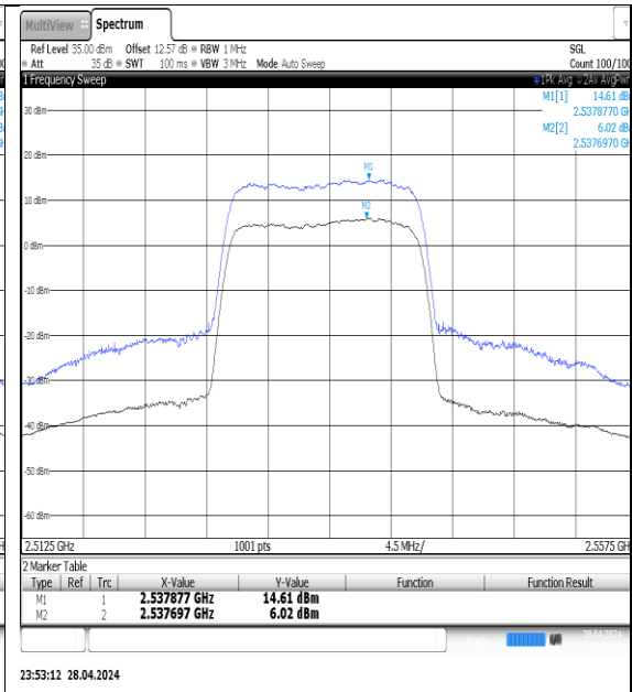
NTNV-N7-PC3-15-15-M-DFT-16QAM-Outter_Full-Ant1-PASS
