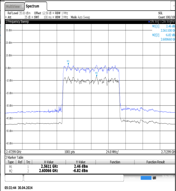
NTVN-N41-PC3-30-80-M-DFT-QPSK-Outer_Full-Ant1-PASS
