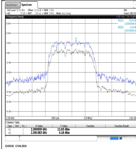
NTNV-N38-PC3-30-10-M-DFT-QPSK-Outter_Full-Ant1-PASS
