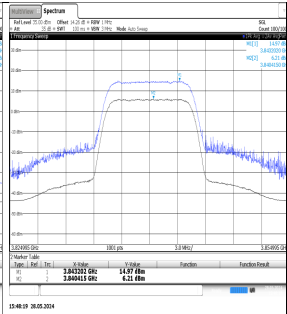
NTNV-N77-3700-3980-PC3-30-10-M-DFT-QPSK- Outer_Full-Ant1-PASS
