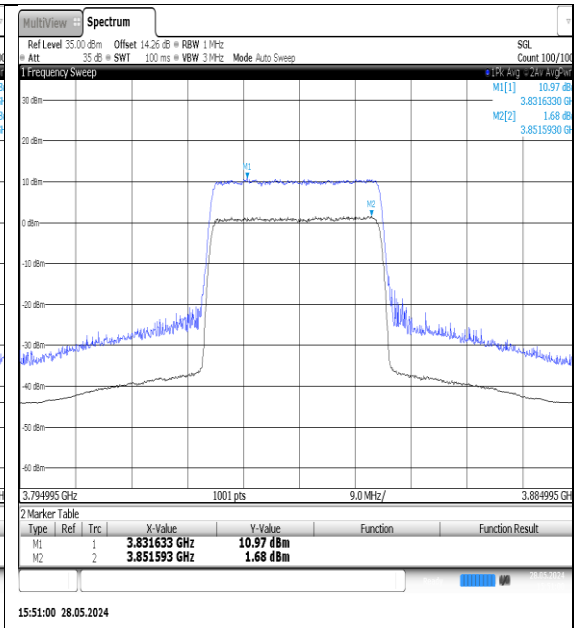
NTNV-N77-3700-3980-PC3-30-30-M-DFT-QPSK- Outer_Full-Ant1-PASS
