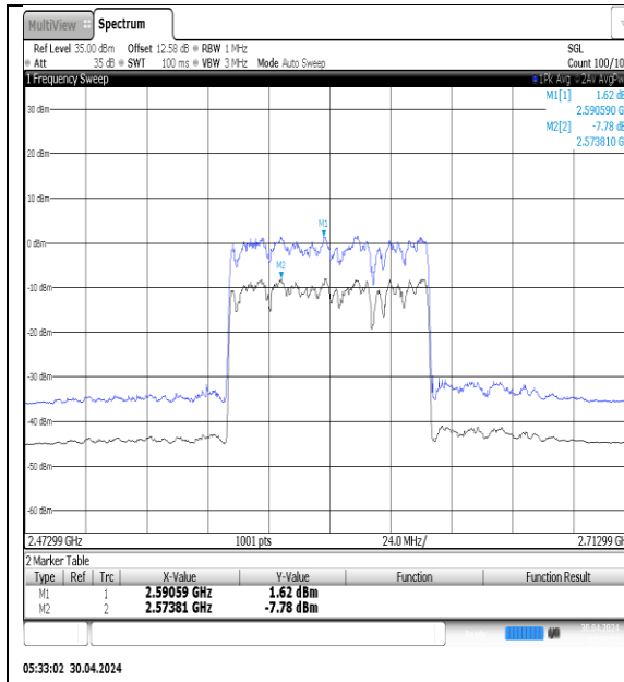
NTVN-N41-PC3-30-80-M-DFT-16QAM-Outer_Full-Ant1-PASS
