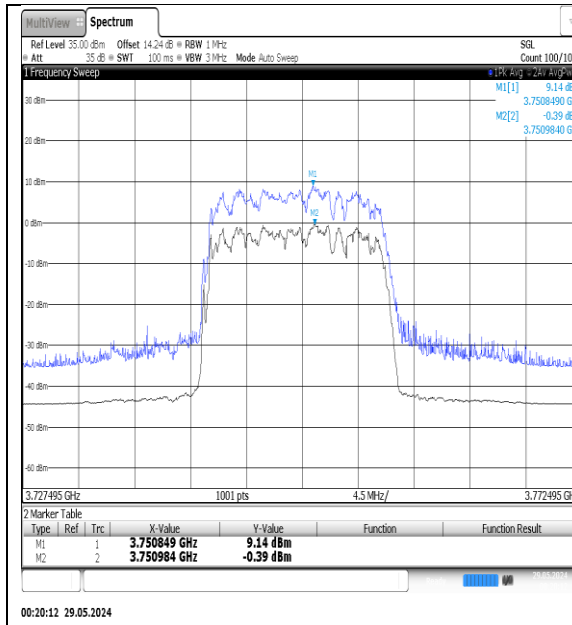
NTNV-N78-3700-3800-PC3-30-15-M-DFT- 16QAM-Outer_Full-Ant1-PASS
