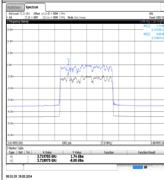
NTNV-N78-3700-3800-PC3-30-90-M-DFT- 16QAM-Outer_Full-Ant1-PASS
