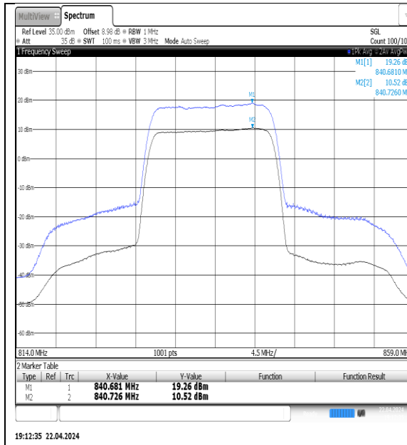
NTNV-N5-PC3-15-15-M-DFT-QPSK-Outer_Full-Ant1-PASS
