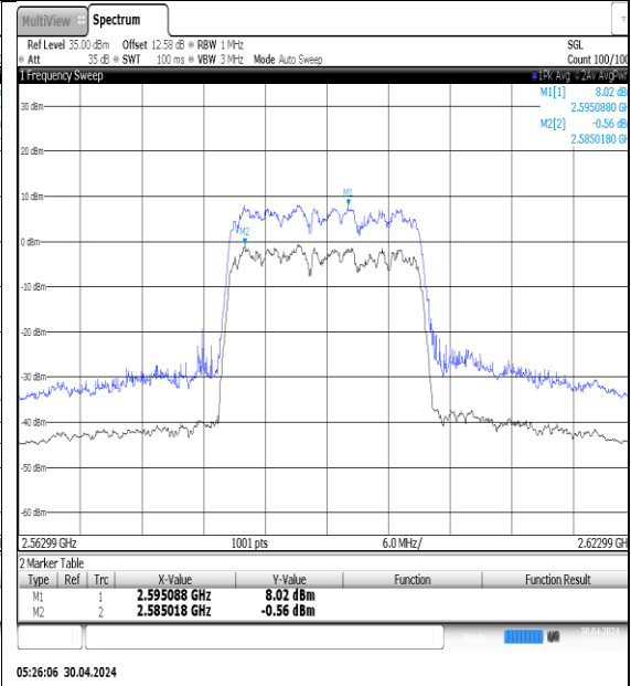
NTVN-N41-PC3-30-20-M-DFT-QPSK-Outer_Full-Ant1-PASS
