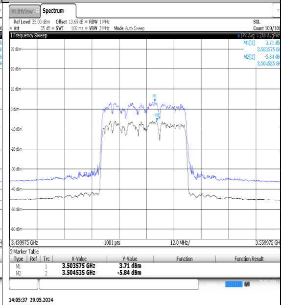
NTNV-N77-3450-3550-PC3-30-40-M-DFT-QPSK-Outer_Full-Ant1-PASS
