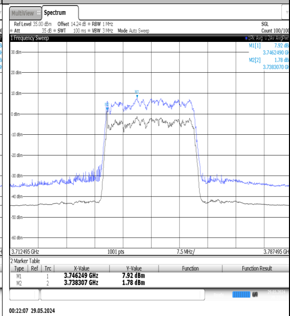
NTNV-N78-3700-3800-PC3-30-25-M-DFT-QPSK- Outer_Full-Ant1-PASS
