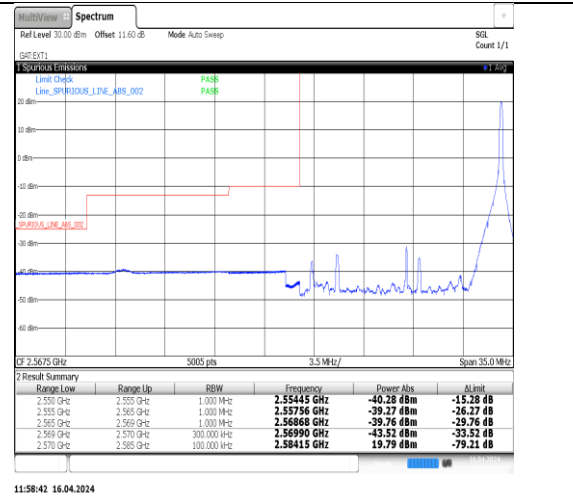
Band38_15MHz_16QAM_38175_1RB#0
