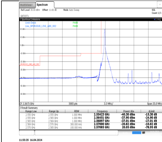
Band38_15MHz_16QAM_37825_75RB#0
