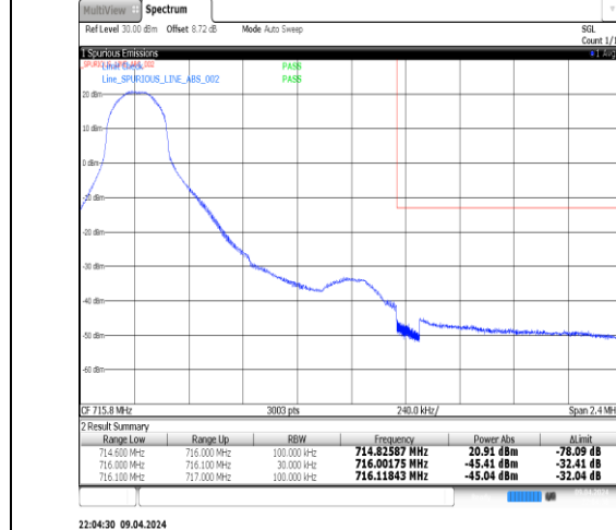
Band12 1.4MHz QPSK 23173 6RB#0
