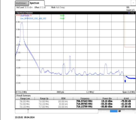
Band12_10MHz_16QAM_23130_50RB#0
