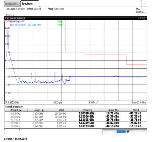
Band38_15MHz_16QAM_38175_75RB#0
