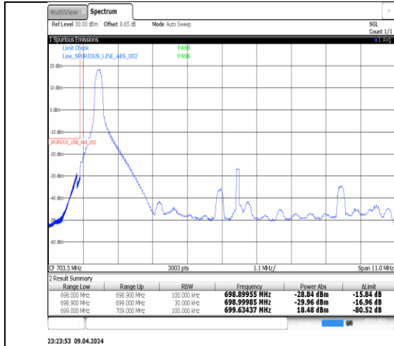
Band12_10MHz_16QAM_23060_50RB#0
