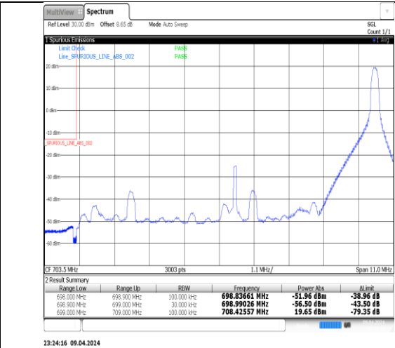
Band12_10MHz_16QAM_23130_1RB#0
