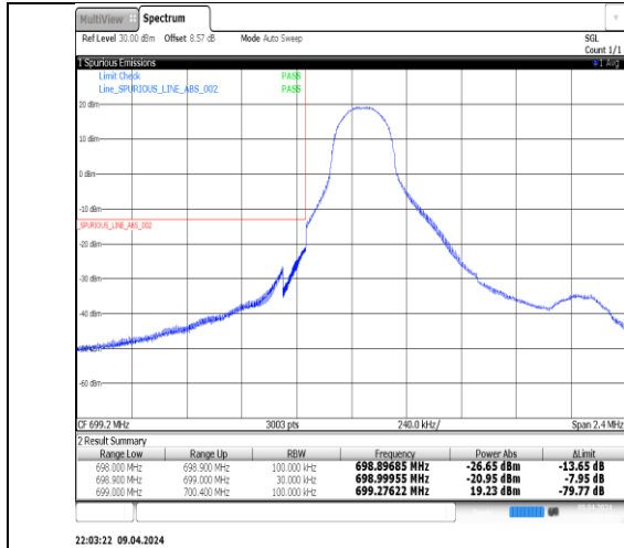
Band12 1.4MHz QPSK 23017 6RB#0
