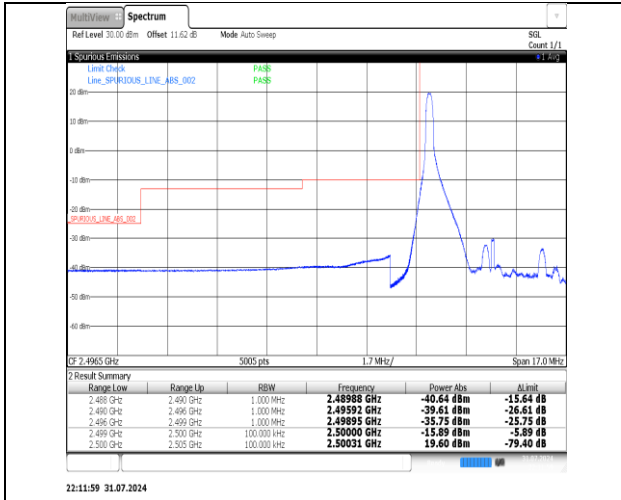
Band7-5MHz-QPSK-20775-1RB#24-PASS
