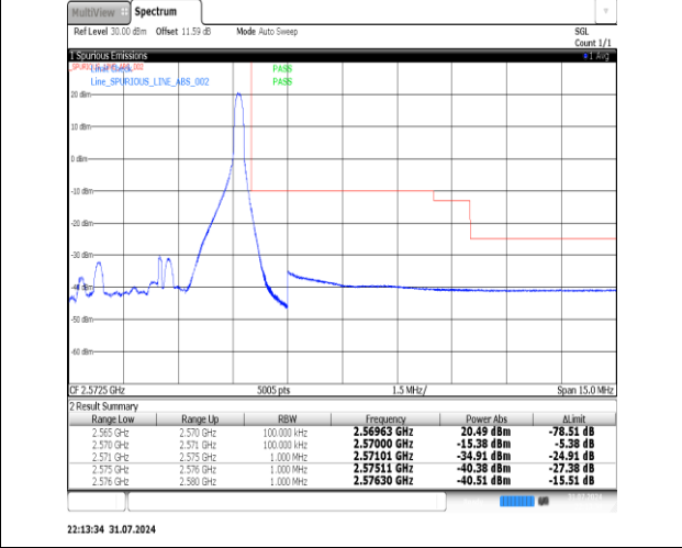
Band7-5MHz-16QAM-20775-25RB#0-PASS
