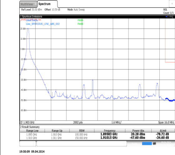
Band2_15MHz_QPSK_19125_1RB#0
