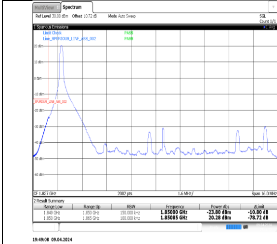
Band2_15MHz_QPSK_18675_75RB#0
