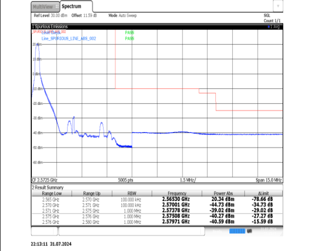
Band7-5MHz-QPSK-21425-1RB#24-PASS
