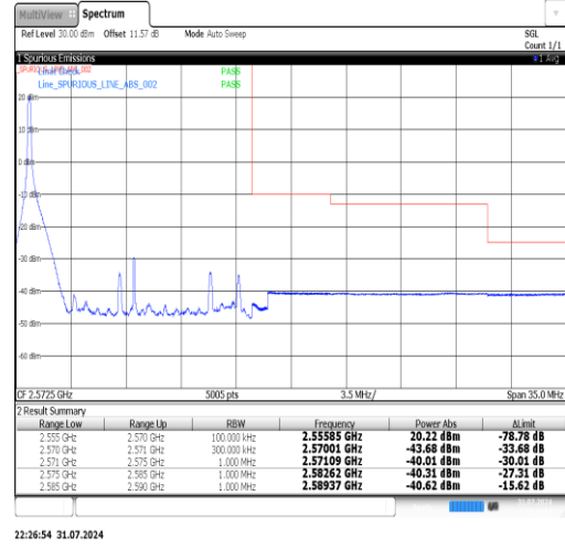
Band7-15MHz-QPSK-21375-1RB#74-PASS
