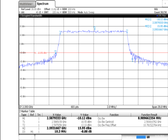
Band41-10MHz-QPSK-40620-50RB#0-PASS
