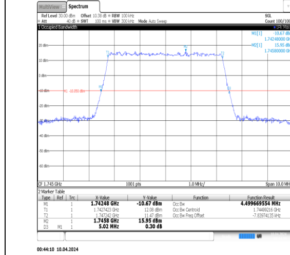
00:44:10 10.04.2024 Band66-5MHz-QPSK-132322-25RB#0-PASS
