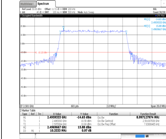
Band41-10MHz-QPSK-39700-50RB#0-PASS
