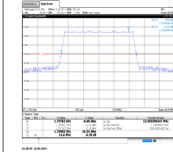
01:38:20 10.04.2024 Band66-15MHz-QPSK-132322-75RB#0-PASS
