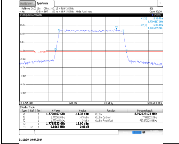
01:11:09 10.04.2024 Band66-10MHz-16QAM-132022-50RB#0-PASS
