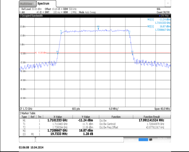
Band66-20MHz-16QAM-132572-100RB#0-PASS
