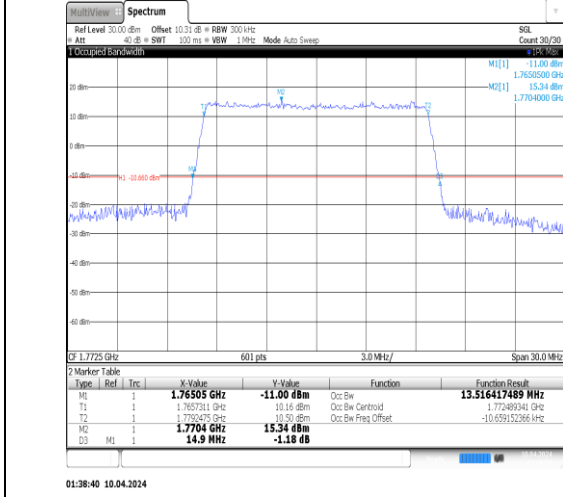
01:38:40 10.04.2024 Band66-15MHz-16QAM-132047-75RB#0-PASS
