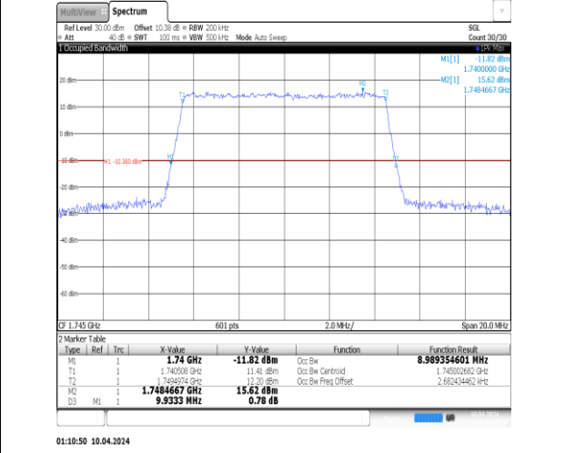
01:10:50 10.04.2024 Band66-10MHz-QPSK-132322-50RB#0-PASS
