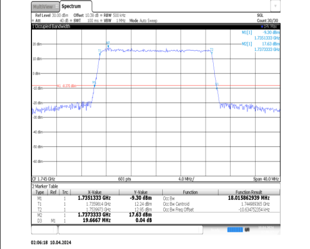
Band66-20MHz-16QAM-132072-100RB#0-PASS
