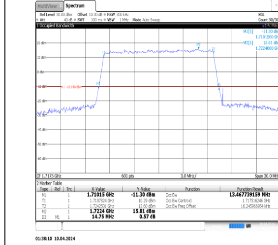
01:38:10 10.04.2024 Band66-15MHz-16QAM-132322-75RB#0-PASS
