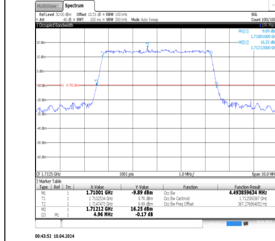
00:43:52 10.04.2024 Band66-5MHz-16QAM-132322-25RB#0-PASS
