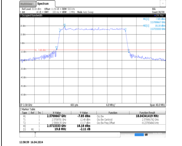
Band38-20MHz-QPSK-38150-100RB#0-PASS
