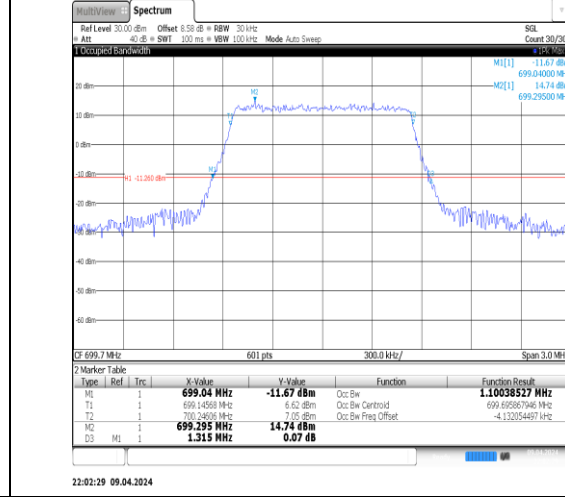
Band12-1.4MHz-16QAM-23095-6RB#0-PASS
