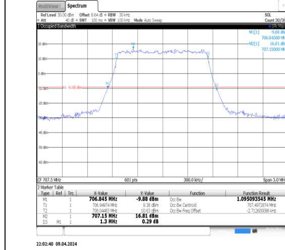
Band12-1.4MHz-QPSK-23095-6RB#0-PASS
