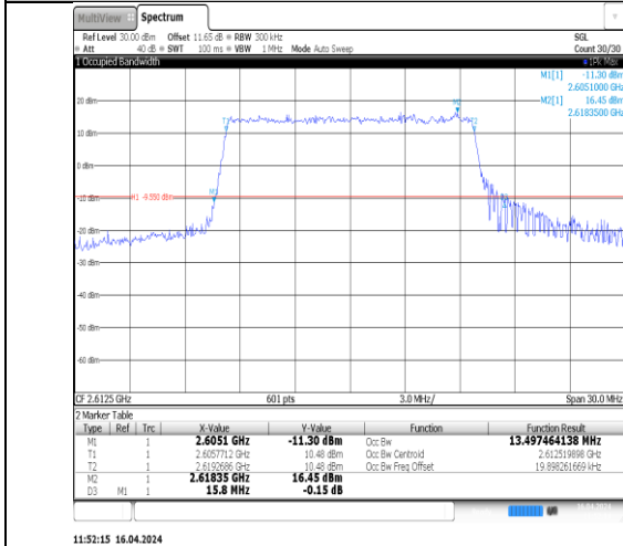
Band38-15MHz-16QAM-38175-75RB#0-PASS
