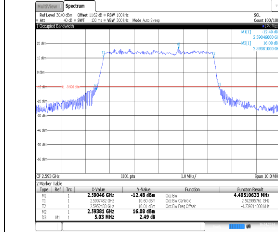
Band41-5MHz-QPSK-40620-25RB#0-PASS
