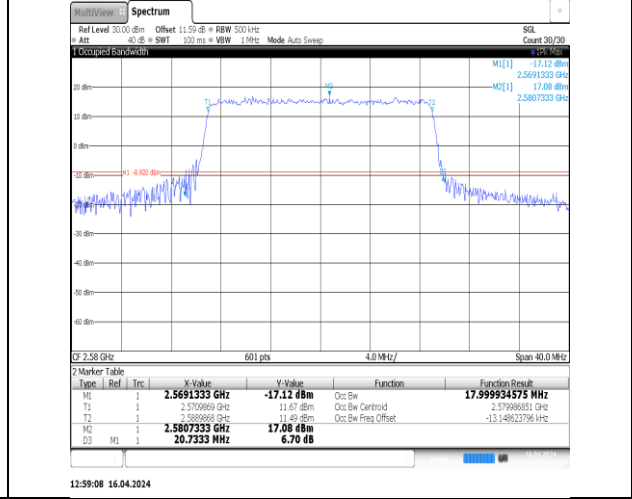
Band38-20MHz-16QAM-38150-100RB#0-PASS
