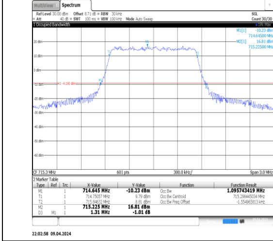
Band12-1.4MHz-16QAM-23173-6RB#0-PASS
