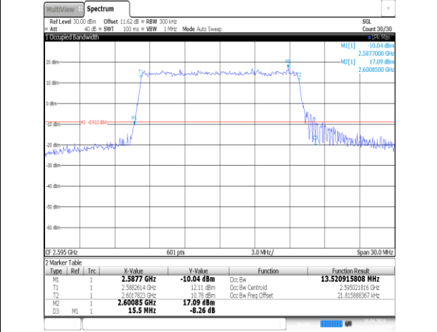
Band38-15MHz-16QAM-38000-75RB#0-PASS
