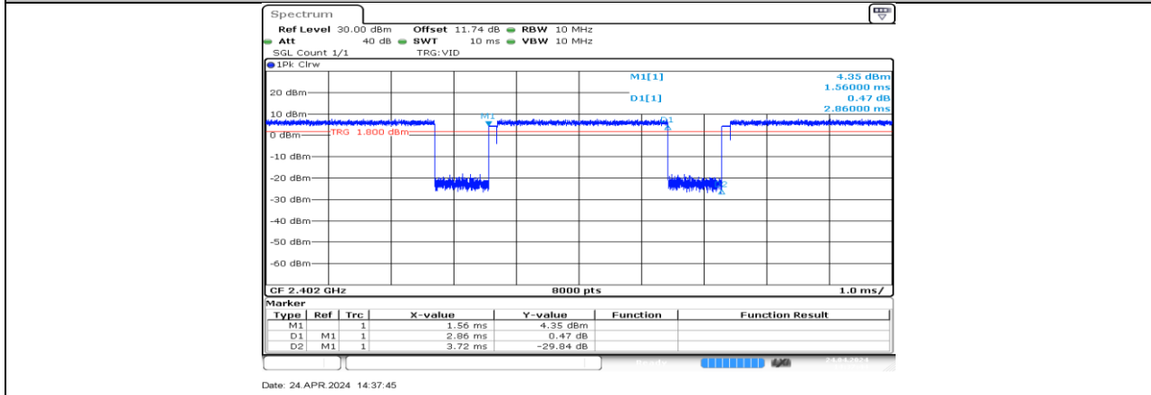
3DH5_Ant7_2402
