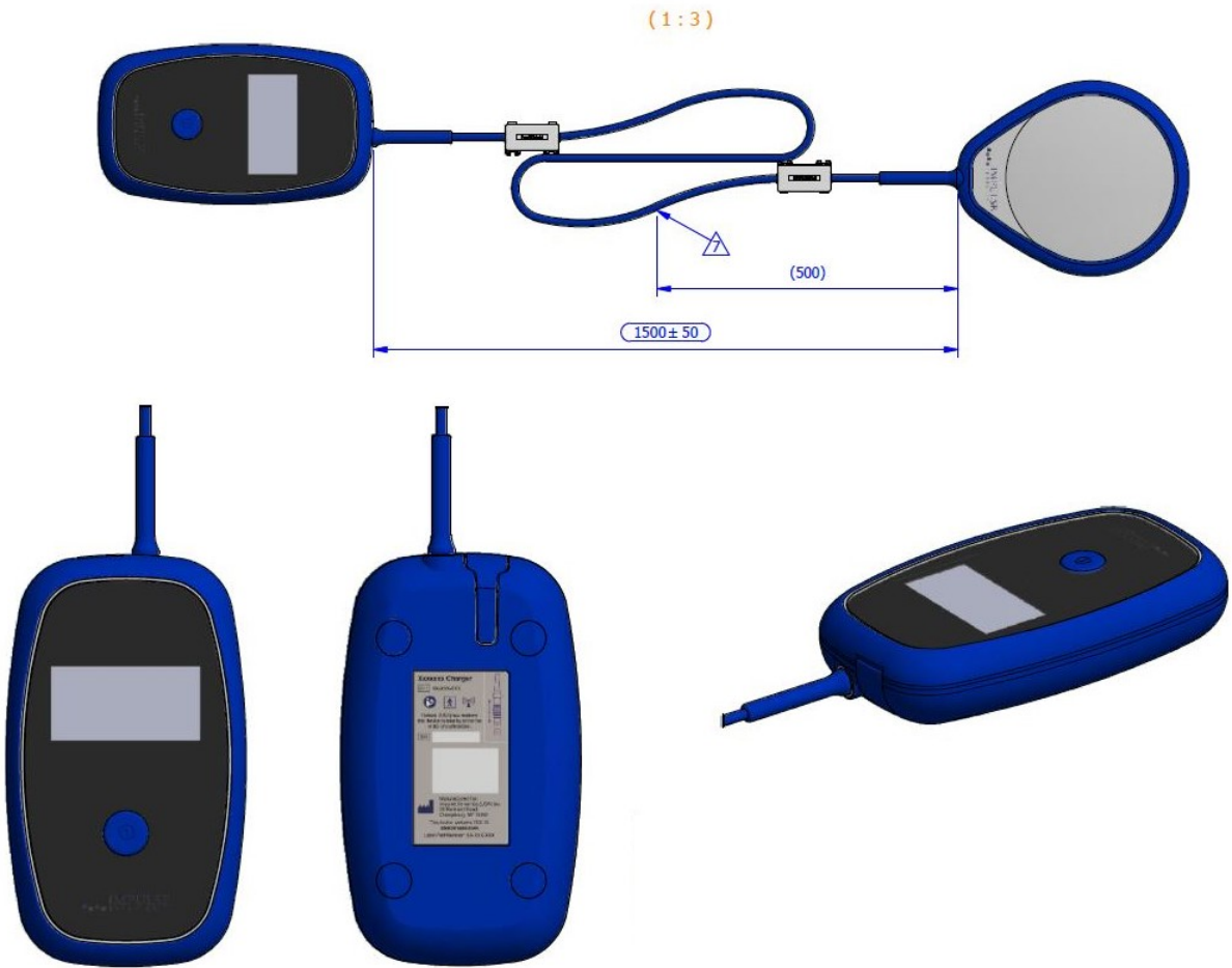
External Picture 2: Mechanical model used for assembly.
