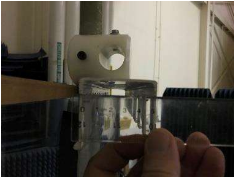
EUT Surface Spacing Measurement
