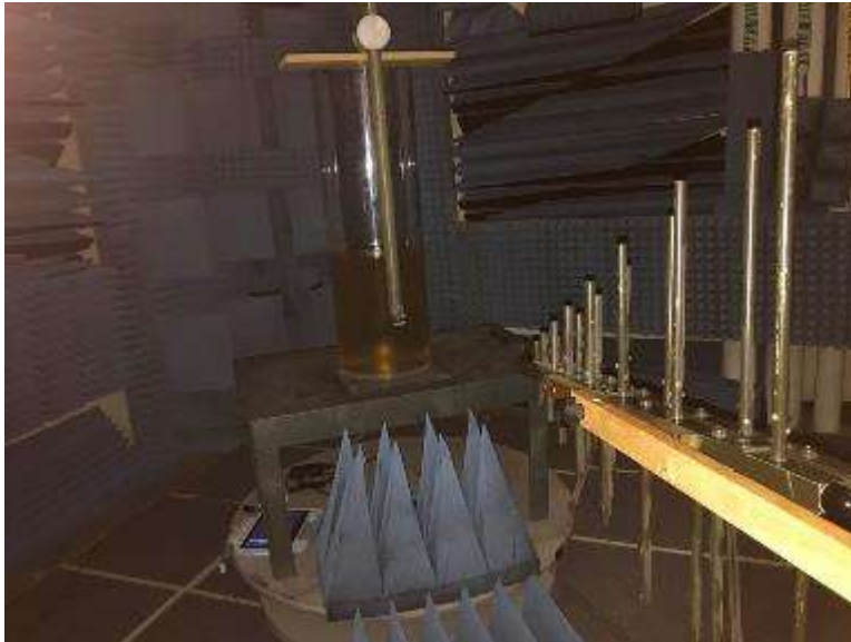
EUT Outside Torso Simulator for Reference Measurement
