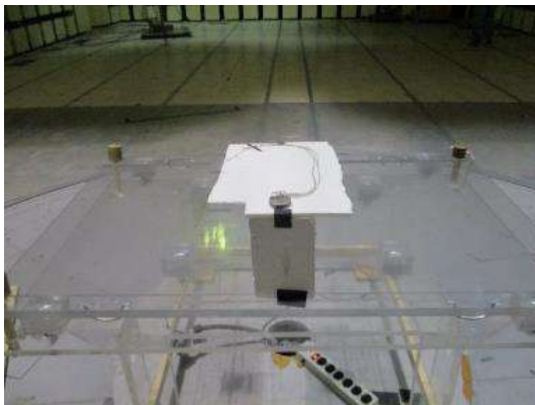
Radiated Emissions, Rear
