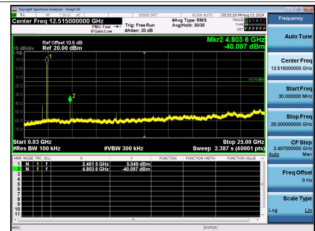
BLE_1M-Ant1-2402-30~25000-PASS
