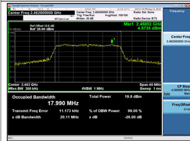
11N20SISO-Ant1-2462
