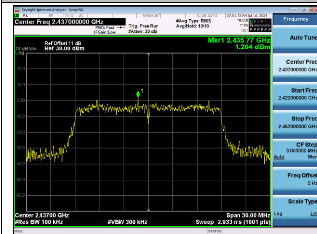
11N20SISO-Ant1-2437-0~Reference-PASS
