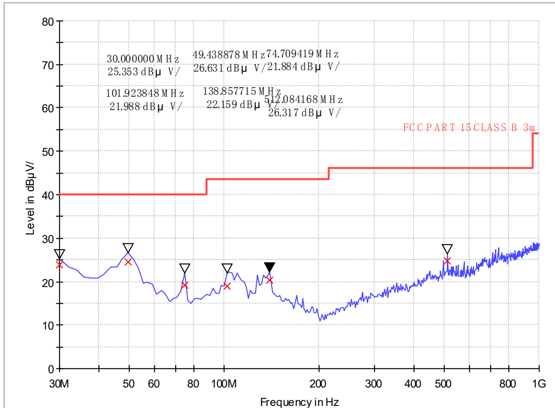
EMI Sweep-3M(30-1G)
