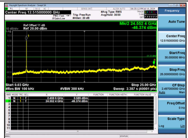
11G-Ant1-2462-30~25000-PASS
