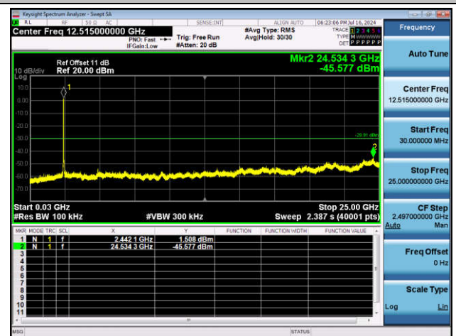
11G-Ant1-2437-30~25000-PASS
