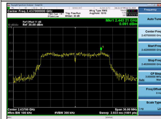
11G-Ant1-2437-0~Reference-PASS
