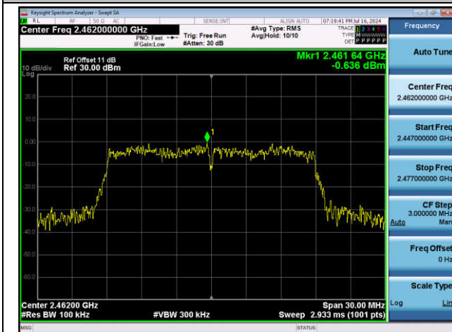
11N20SISO-Ant1-2462-0~Reference-PASS
