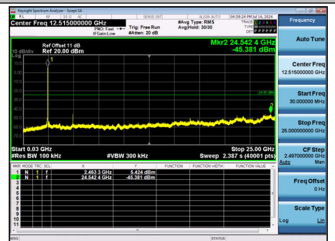
11B-Ant1-2462-30~25000-PASS
