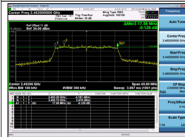
11N20SISO-Ant1-2462-PASS
