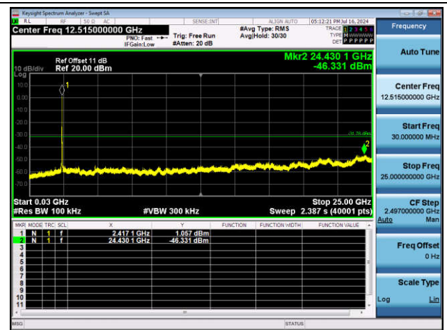
11G-Ant1-2412-30~25000-PASS
