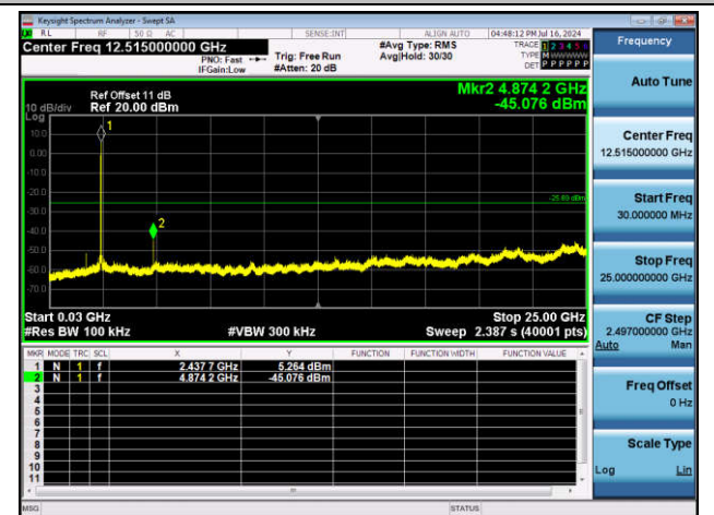
11B-Ant1-2437-30~25000-PASS
