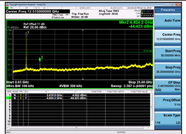
11B-Ant1-2412-30~25000-PASS
