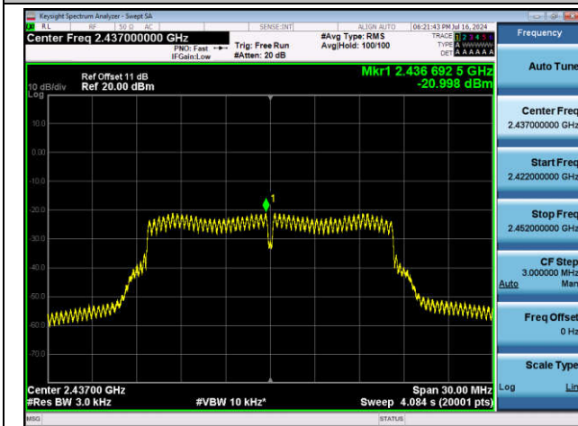
11G-Ant1-2437-PASS
