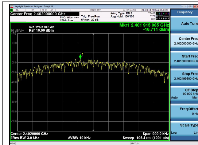
BLE_1M-Ant1-2402-PASS
