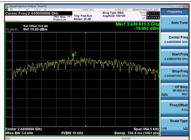
BLE_1M-Ant1-2440-PASS
