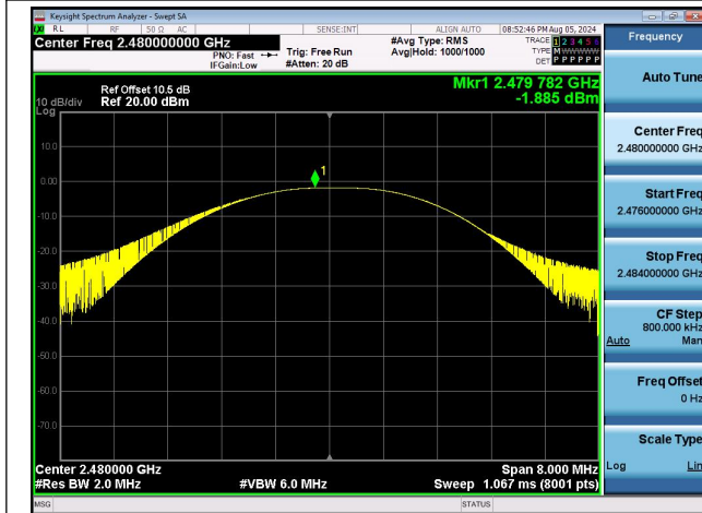
BLE_1M-Ant1-2480-PASS
