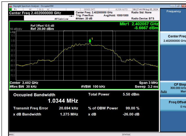
BLE_1M-Ant1-2402
