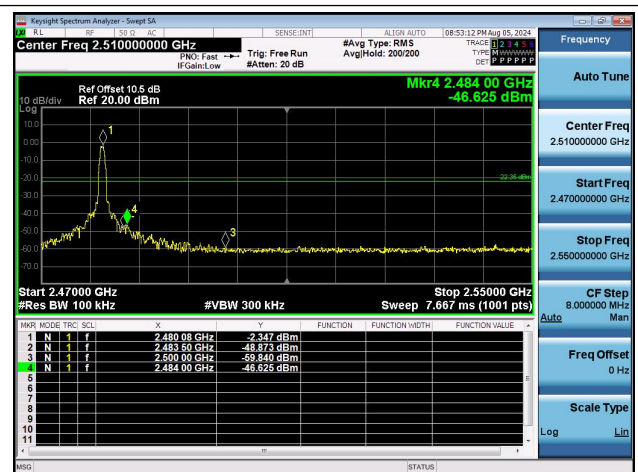
BLE_1M-Ant1-2480-PASS
