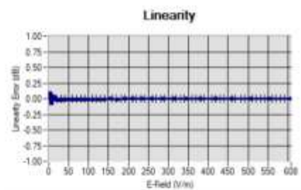
Linearity +/-1.87% (+/-0.08dB)
