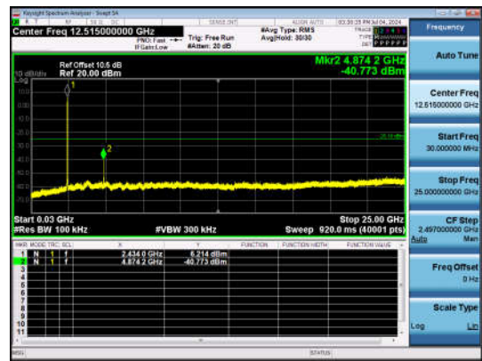
11B-Ant1-2437-30~25000-PASS
