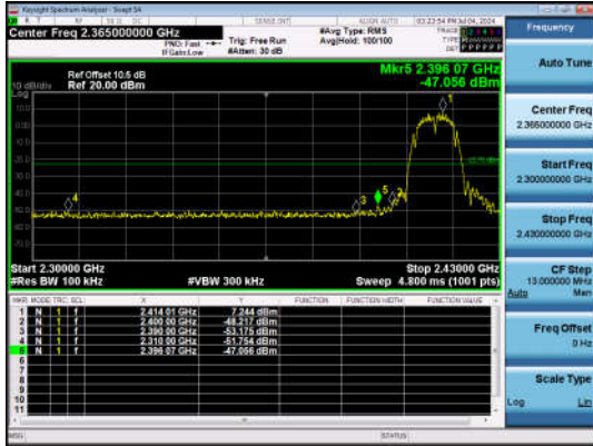
11B-Ant1-2412-PASS
