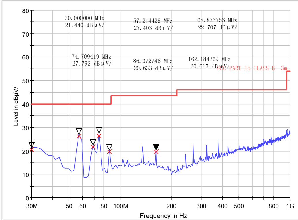
EMI Sweep-3M(30-1G)
