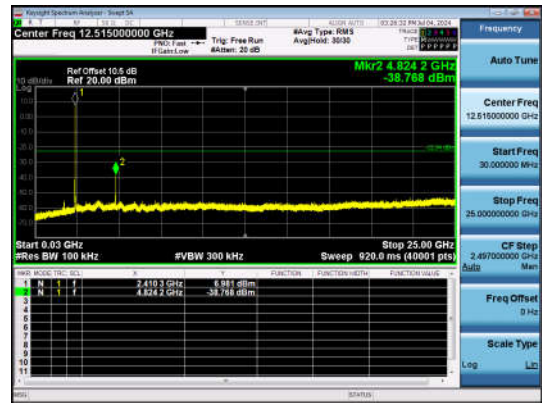
11B-Ant1-2412-30~25000-PASS
