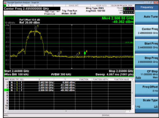
11B-Ant1-2462-PASS
