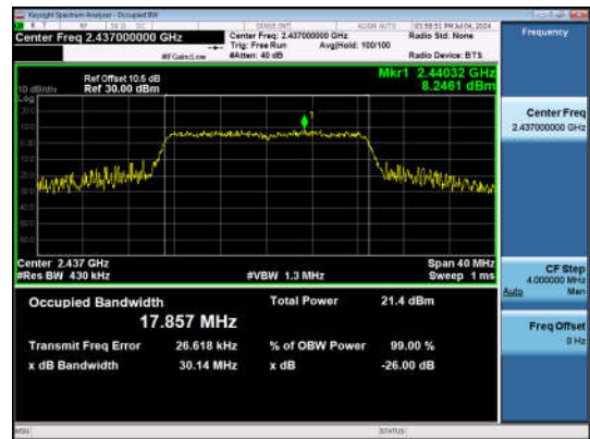
11N20SISO-Ant1-2437
