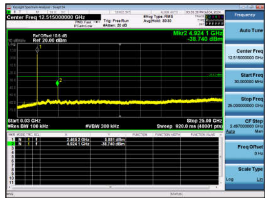
11B-Ant1-2462-30~25000-PASS
