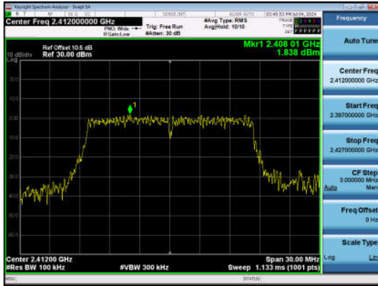
11G-Ant1-2412-0~Reference-PASS
