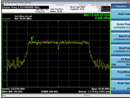
11N20SISO-Ant1-2437-0~Reference-PASS
