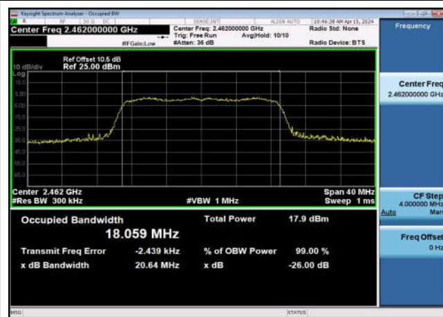
99% Bandwidth-802.11n(20MHz),2462MHz ,Ant0
