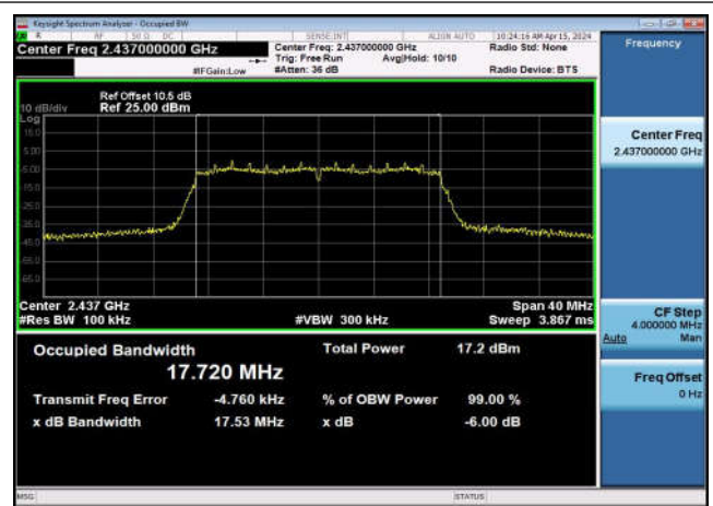
6dB Bandwidth-802.11n(20MHz),2437MHz ,Ant0
