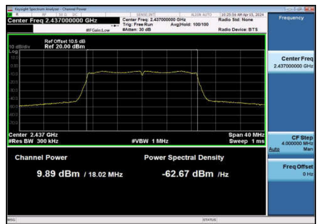
Output Power-802.11n(20MHz),2437MHz ,Ant0
