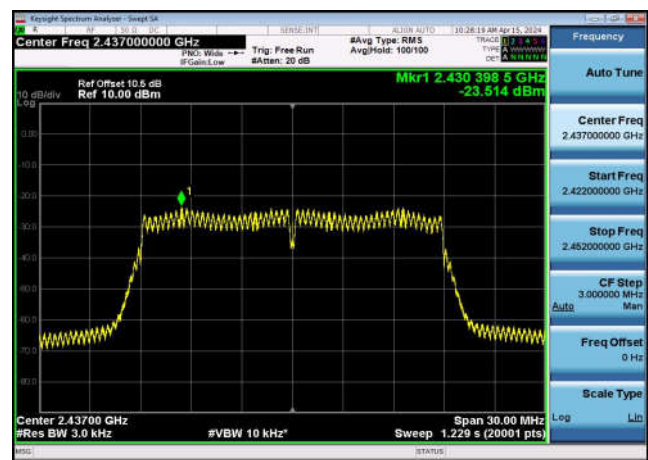
Power spectral density-802.11n(20MHz) ,2437MHz,Ant0
