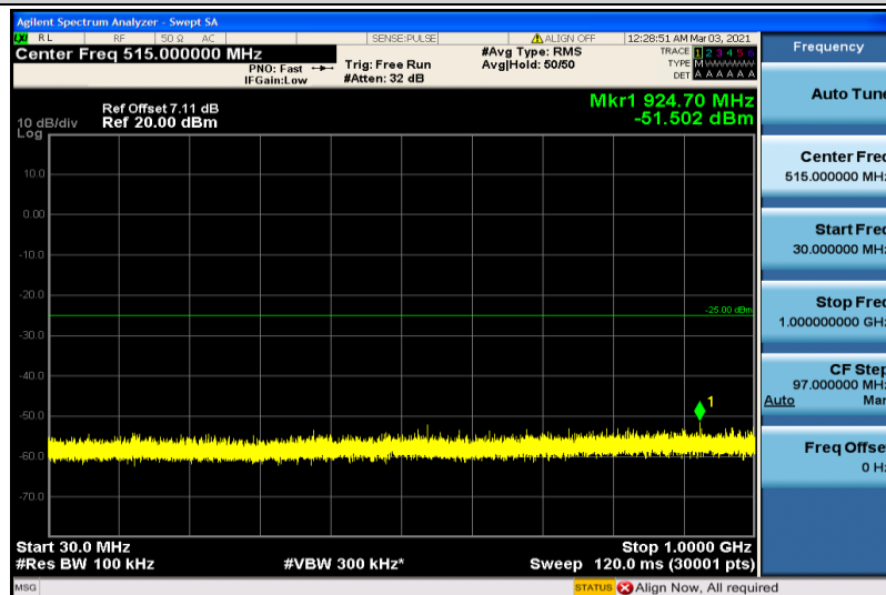
Band38-15MHz-QPSK-38000-1RB#0-30~1000MHz
