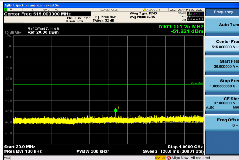
Band38-15MHz-QPSK-37825-1RB#0-30~1000MHz
