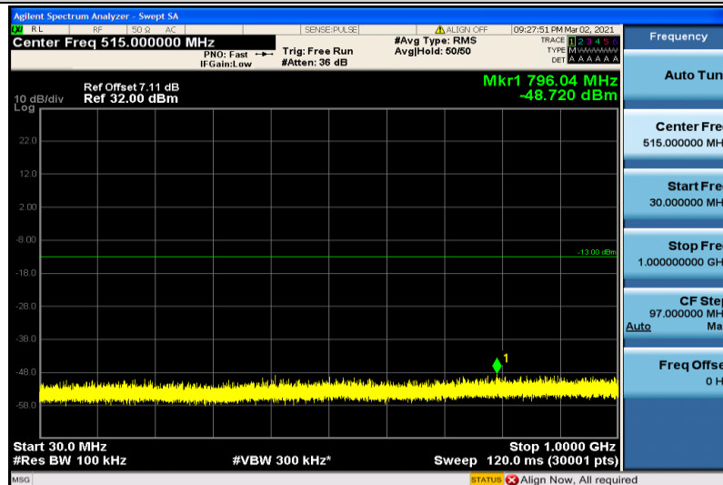
Band4-15MHz-QPSK-20025-1RB#0-30~1000MHz
