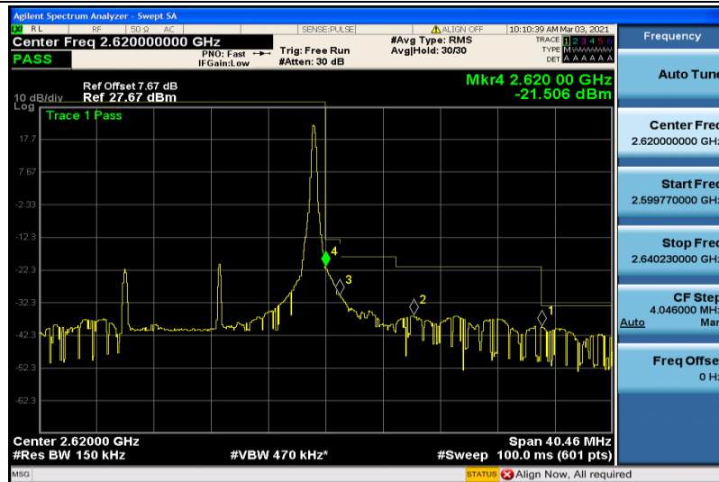
Band38-15MHz-16QAM-38175-1RB#74
